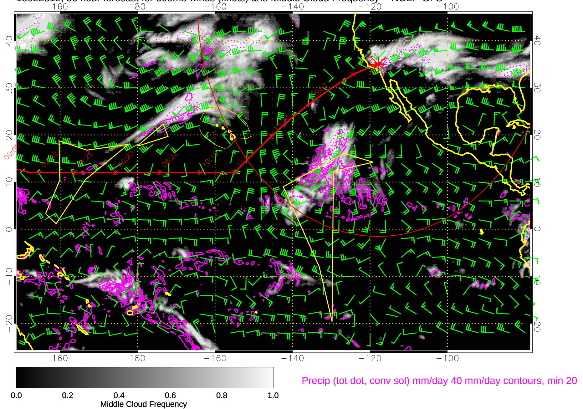
15022312, 36 hour forecast for 500mb winds (knots) and Middle Cloud Frequency -- NCEP GFS
