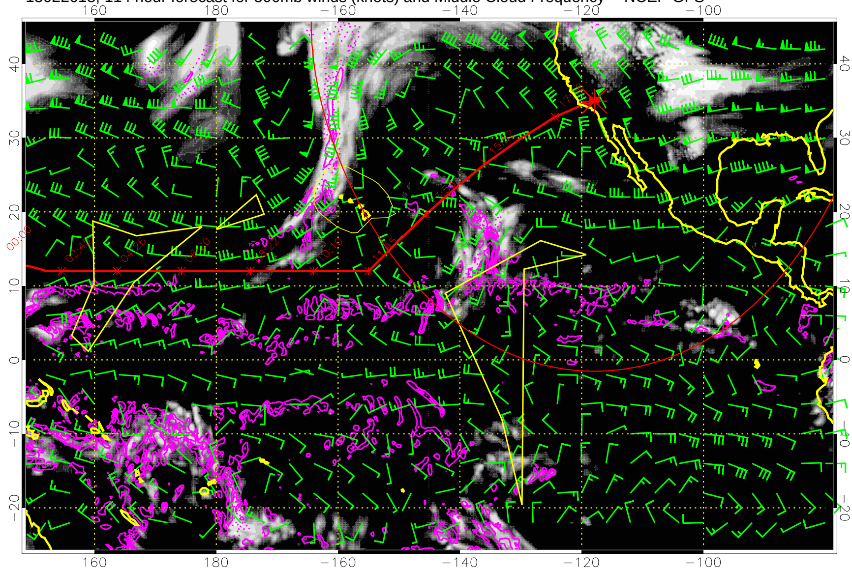
15022618, 114 hour forecast for 500mb winds (knots) and Middle Cloud Frequency -- NCEP GFS
