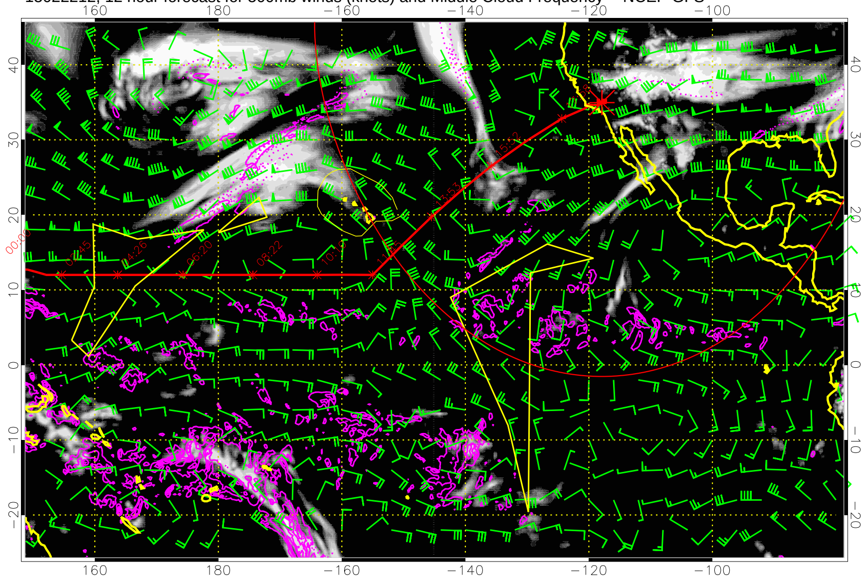
15022212, 12 hour forecast for 500mb winds (knots) and Middle Cloud Frequency -- NCEP GFS
