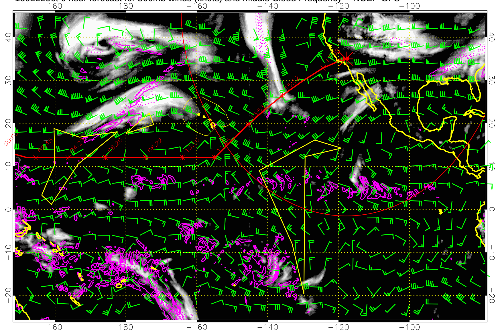
15022206, 6 hour forecast for 500mb winds (knots) and Middle Cloud Frequency -- NCEP GFS
