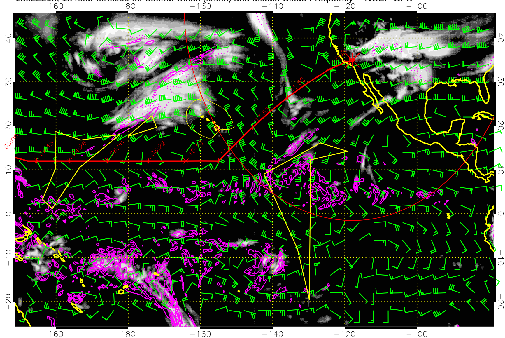
15022218, 18 hour forecast for 500mb winds (knots) and Middle Cloud Frequency -- NCEP GFS
