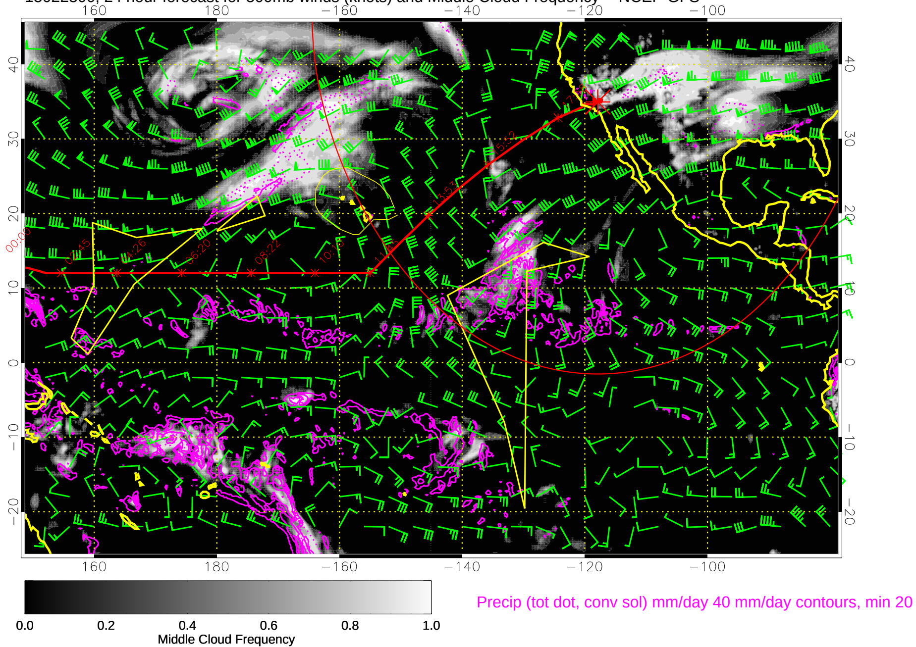
15022300, 24 hour forecast for 500mb winds (knots) and Middle Cloud Frequency -- NCEP GFS
