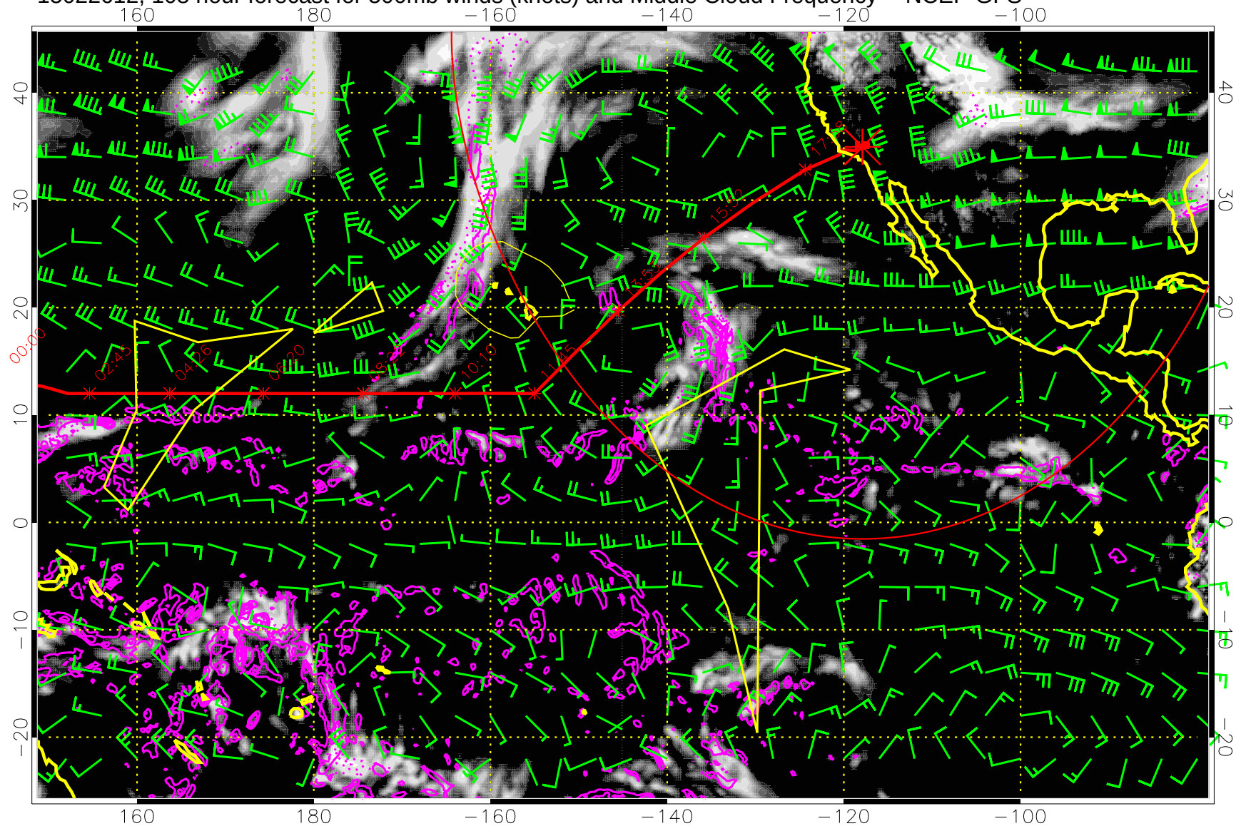
15022612, 108 hour forecast for 500mb winds (knots) and Middle Cloud Frequency -- NCEP GFS
