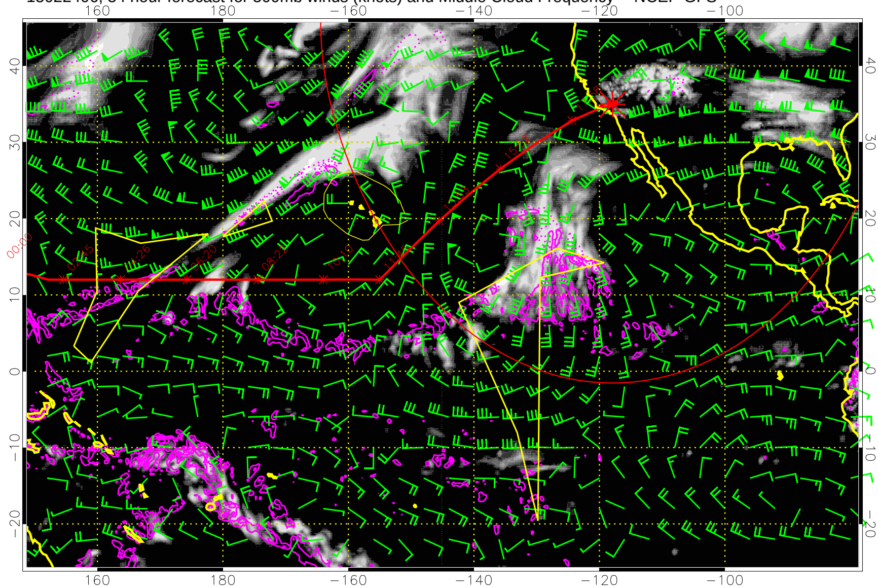
15022406, 54 hour forecast for 500mb winds (knots) and Middle Cloud Frequency -- NCEP GFS
