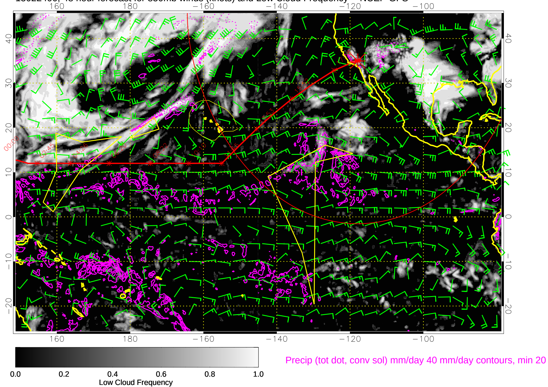
15022400, 48 hour forecast for 850mb winds (knots) and Low Cloud Frequency -- NCEP GFS
