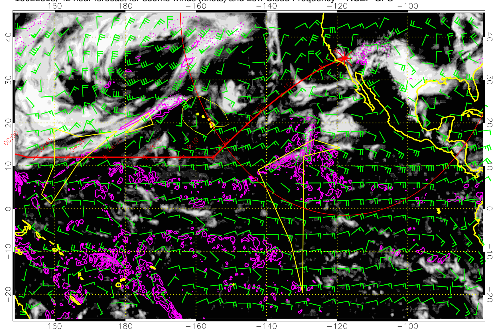
15022318, 42 hour forecast for 850mb winds (knots) and Low Cloud Frequency -- NCEP GFS
