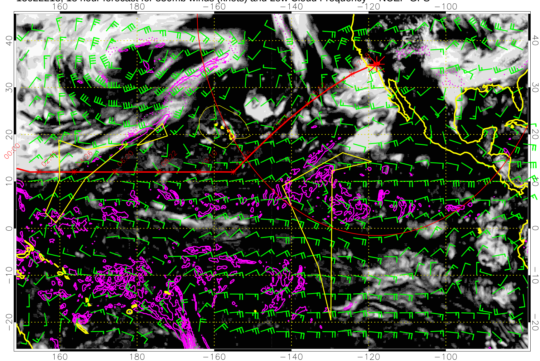
15022218, 18 hour forecast for 850mb winds (knots) and Low Cloud Frequency -- NCEP GFS
