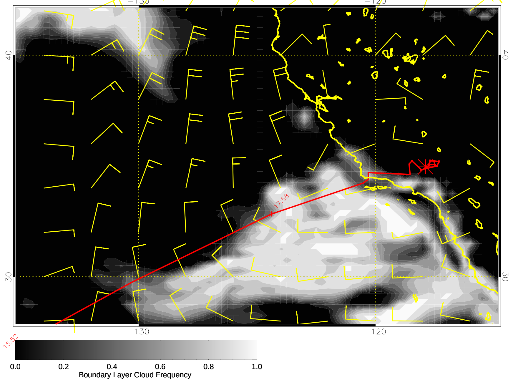
15022206, 6 hour forecast for surface winds (knots) and Boundary Layer Cloud Frequency -- NCEP GFS
