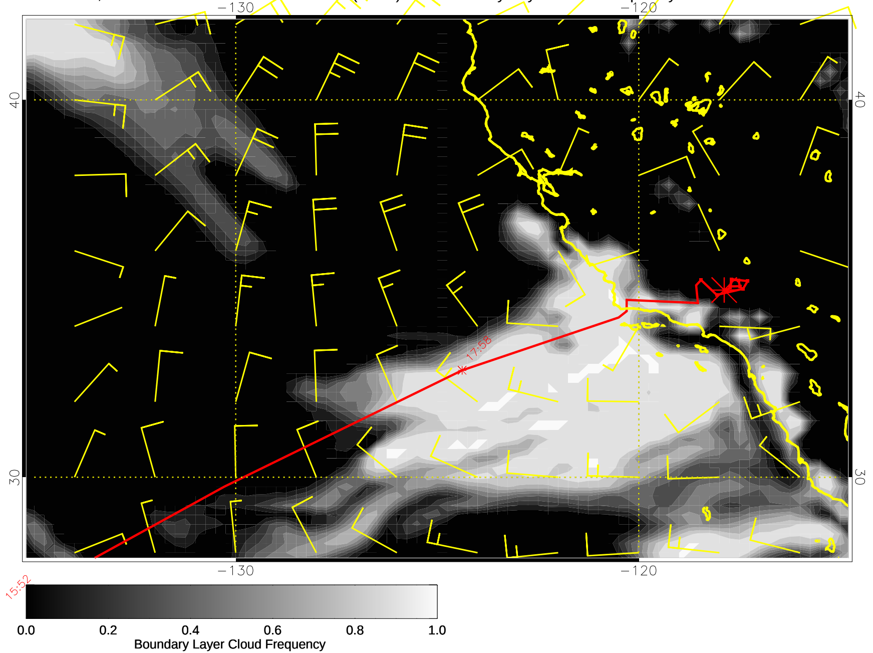
15022212, 12 hour forecast for surface winds (knots) and Boundary Layer Cloud Frequency -- NCEP GFS
