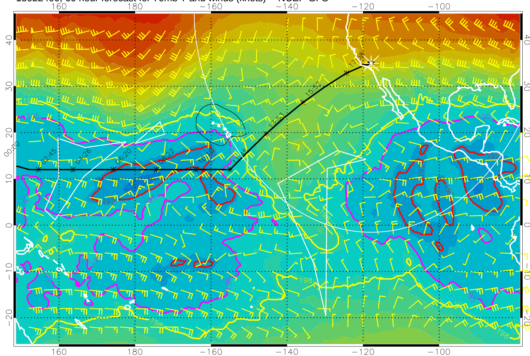
15022400, 60 hour forecast for 70mb T and winds (knots) -- NCEP GFS
