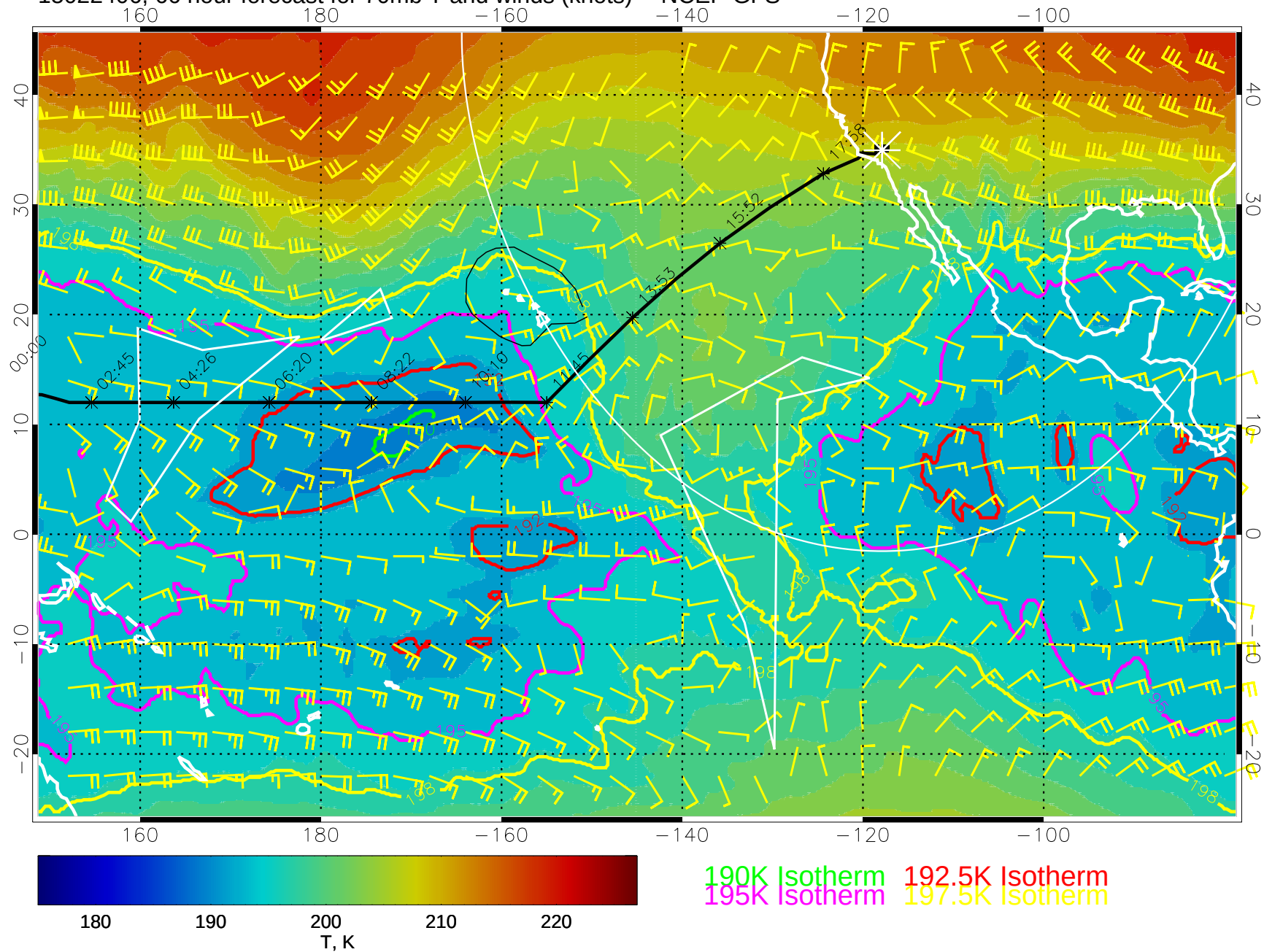
15022406, 66 hour forecast for 70mb T and winds (knots) -- NCEP GFS
