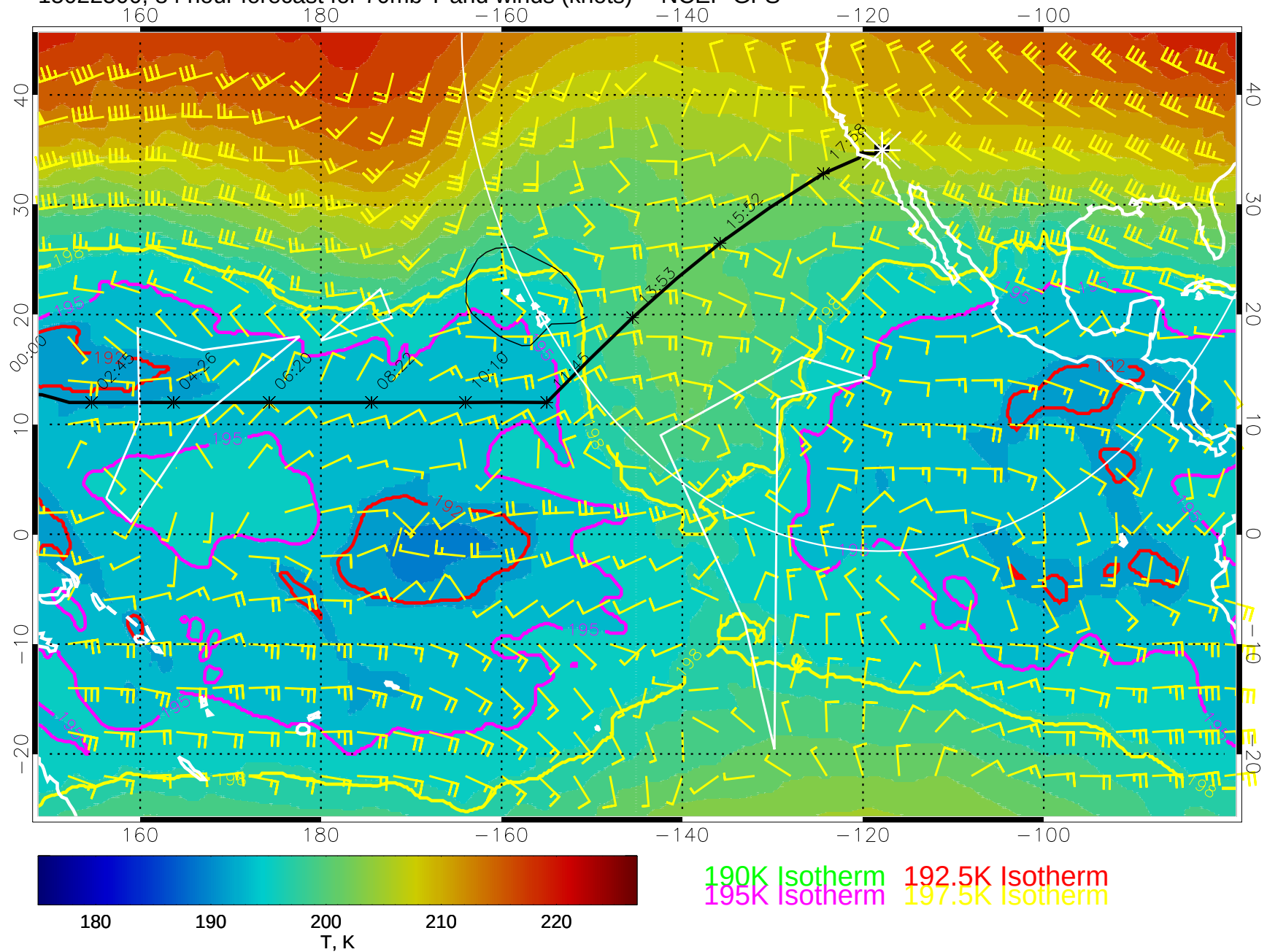
15022500, 84 hour forecast for 70mb T and winds (knots) -- NCEP GFS
