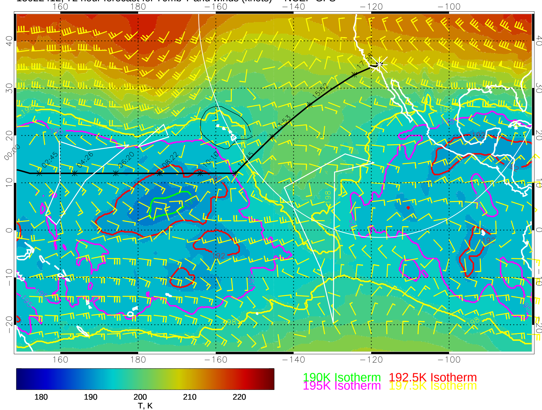
15022412, 72 hour forecast for 70mb T and winds (knots) -- NCEP GFS
