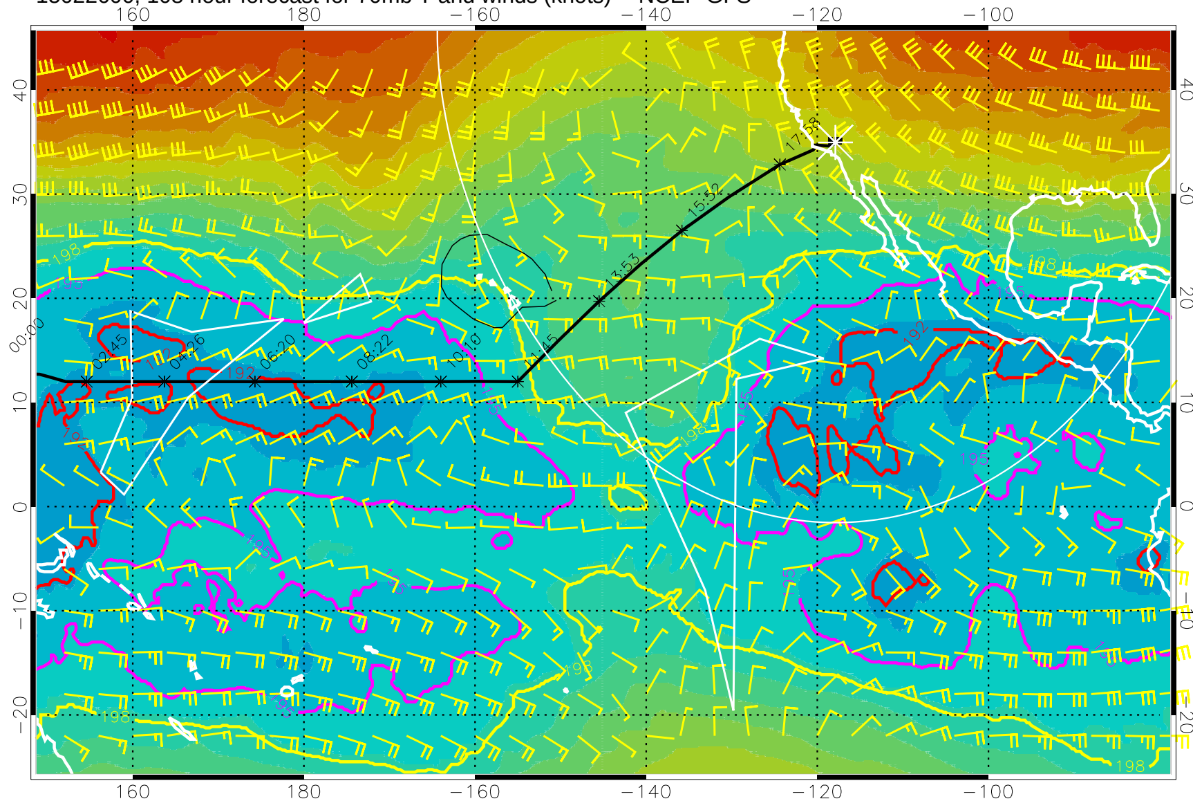
15022600, 108 hour forecast for 70mb T and winds (knots) -- NCEP GFS
