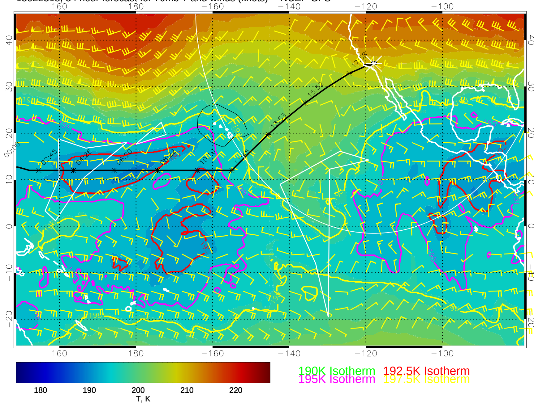
15022318, 54 hour forecast for 70mb T and winds (knots) -- NCEP GFS
