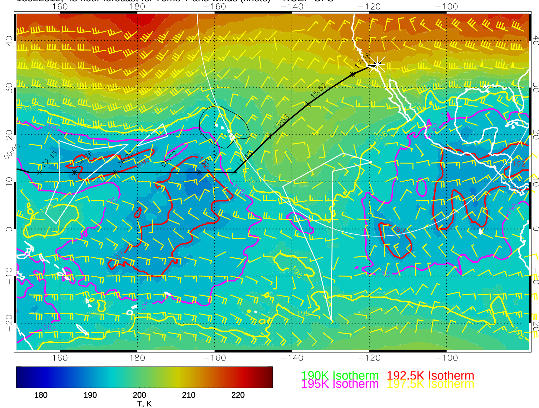
15022312, 48 hour forecast for 70mb T and winds (knots) -- NCEP GFS
