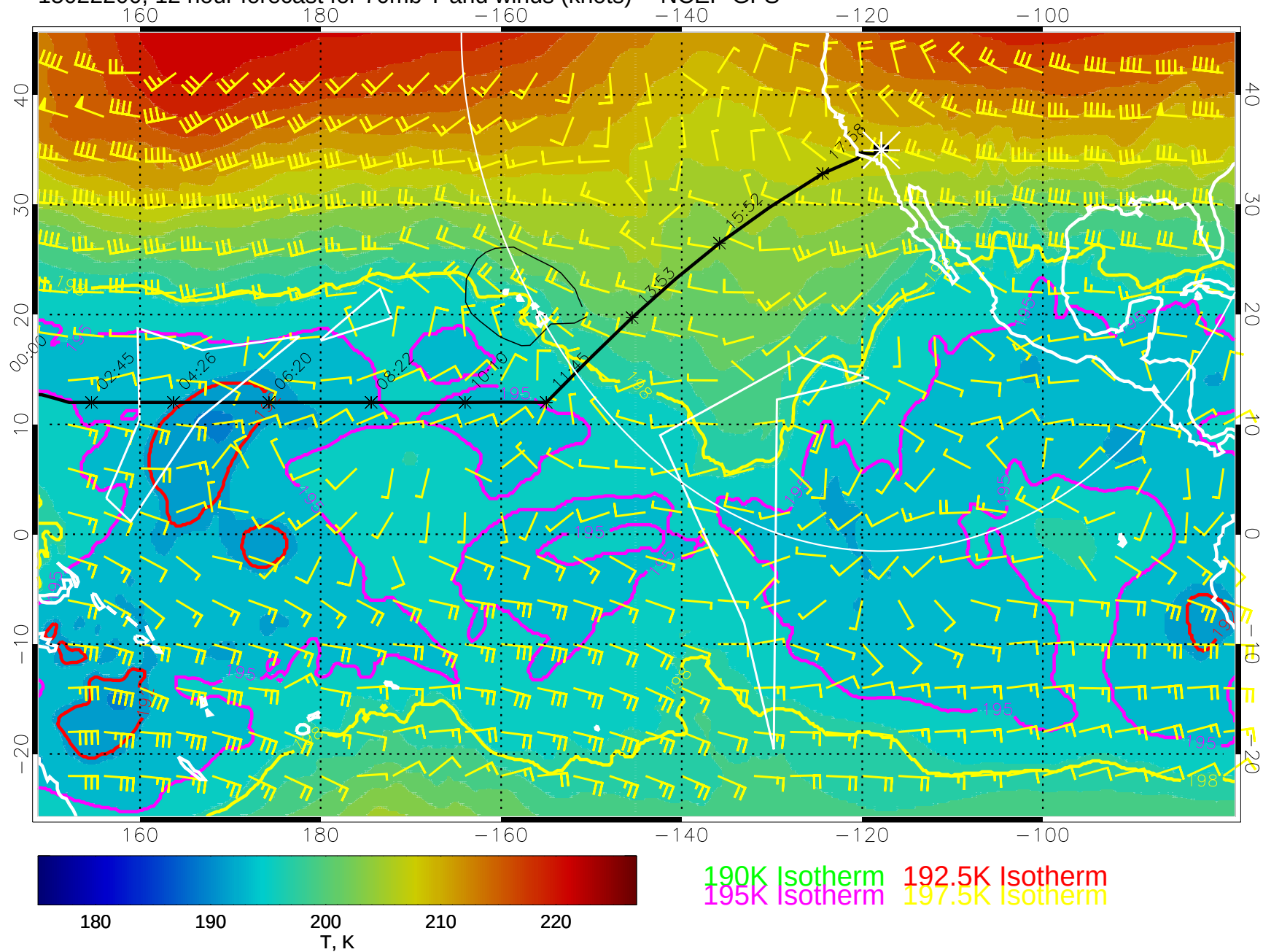
15022200, 12 hour forecast for 70mb T and winds (knots) -- NCEP GFS
