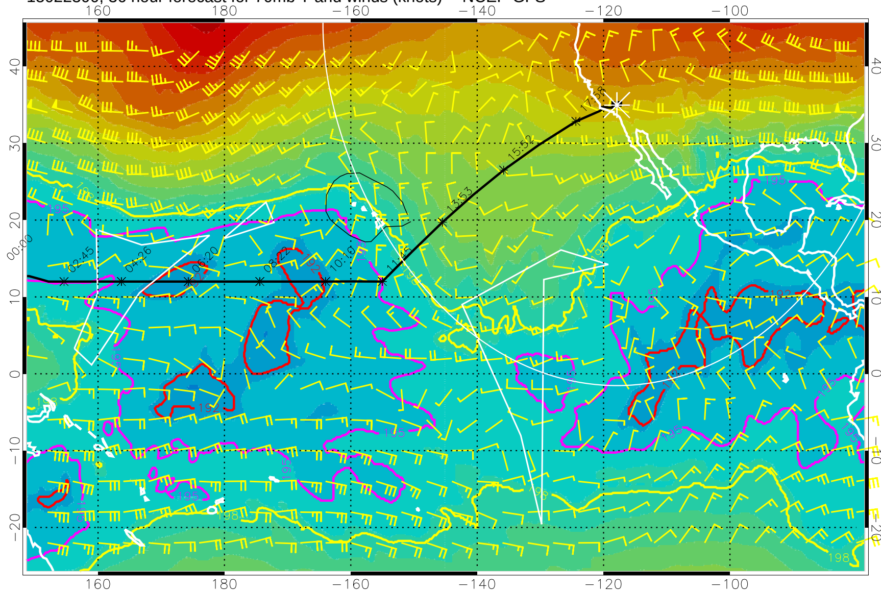
15022300, 36 hour forecast for 70mb T and winds (knots) -- NCEP GFS
