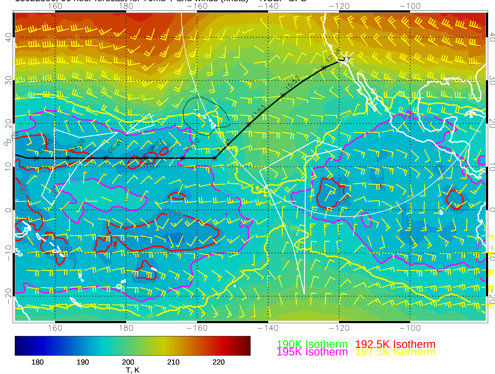
15022506, 90 hour forecast for 70mb T and winds (knots) -- NCEP GFS
