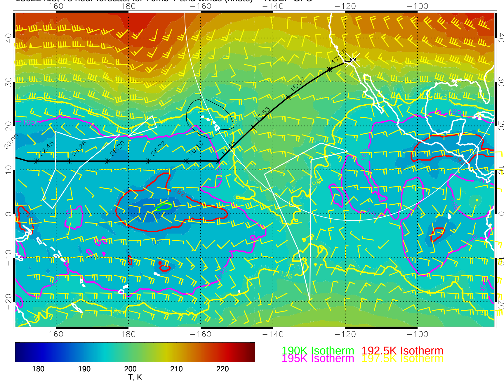
15022418, 78 hour forecast for 70mb T and winds (knots) -- NCEP GFS
