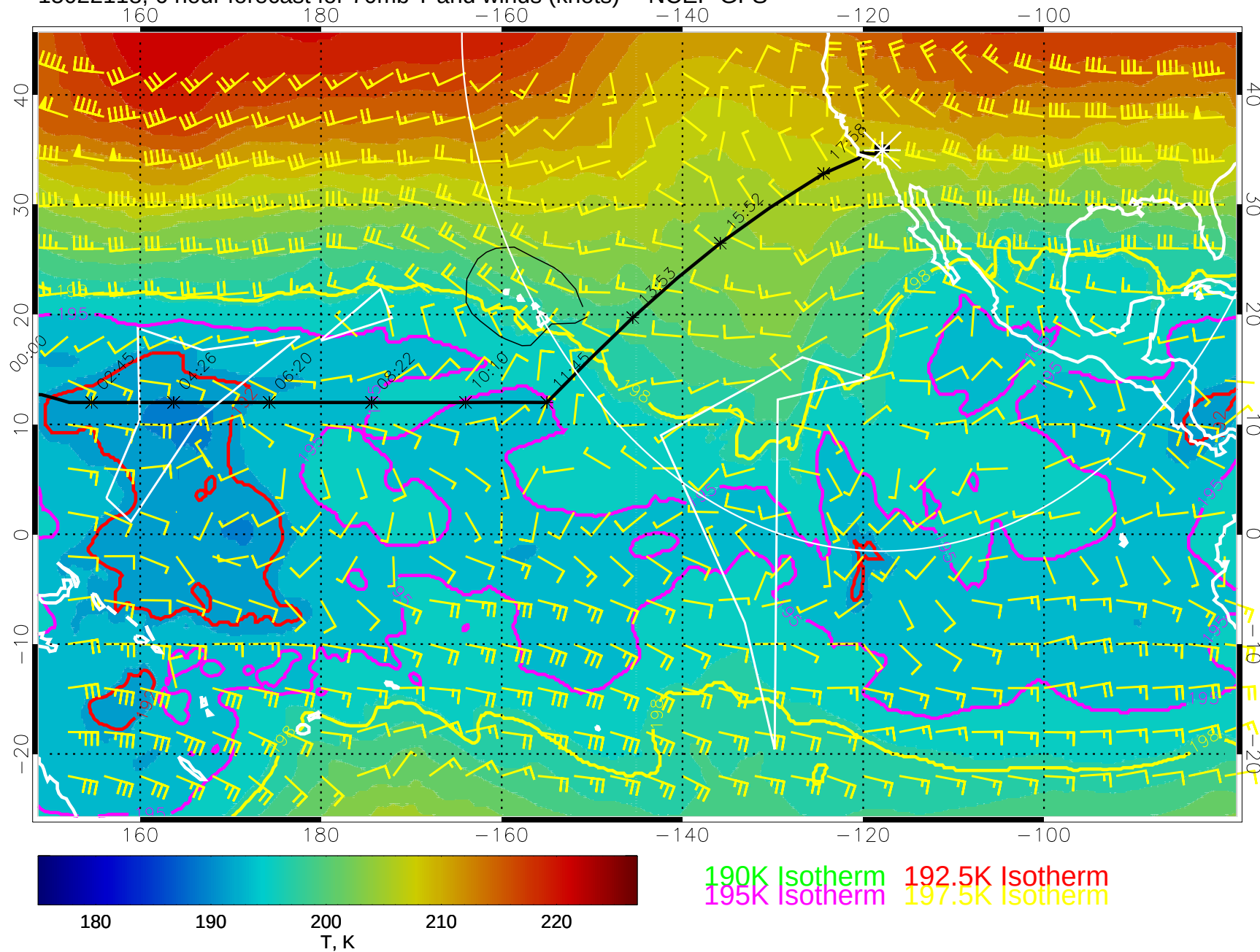
15022118, 6 hour forecast for 70mb T and winds (knots) -- NCEP GFS
