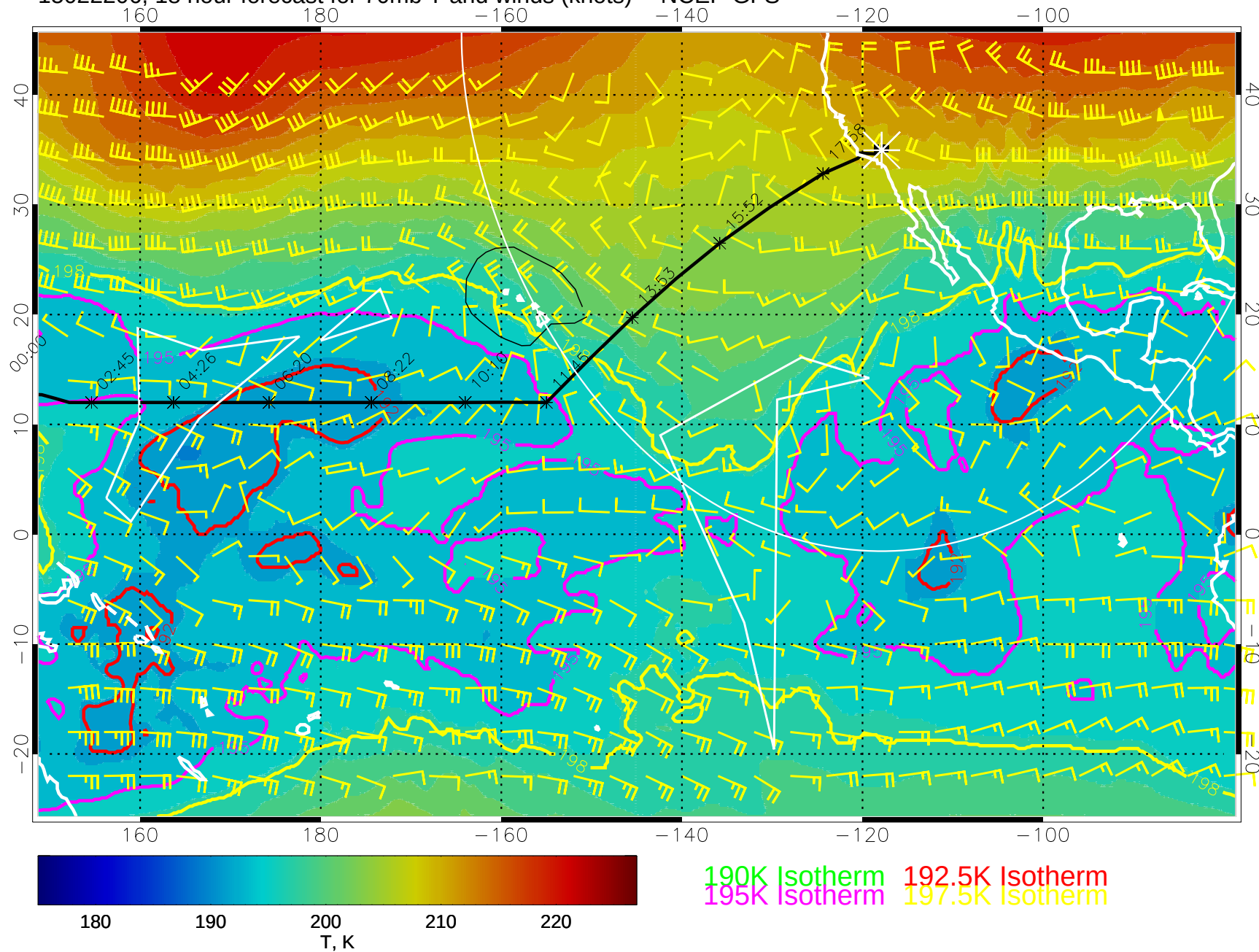
15022206, 18 hour forecast for 70mb T and winds (knots) -- NCEP GFS
