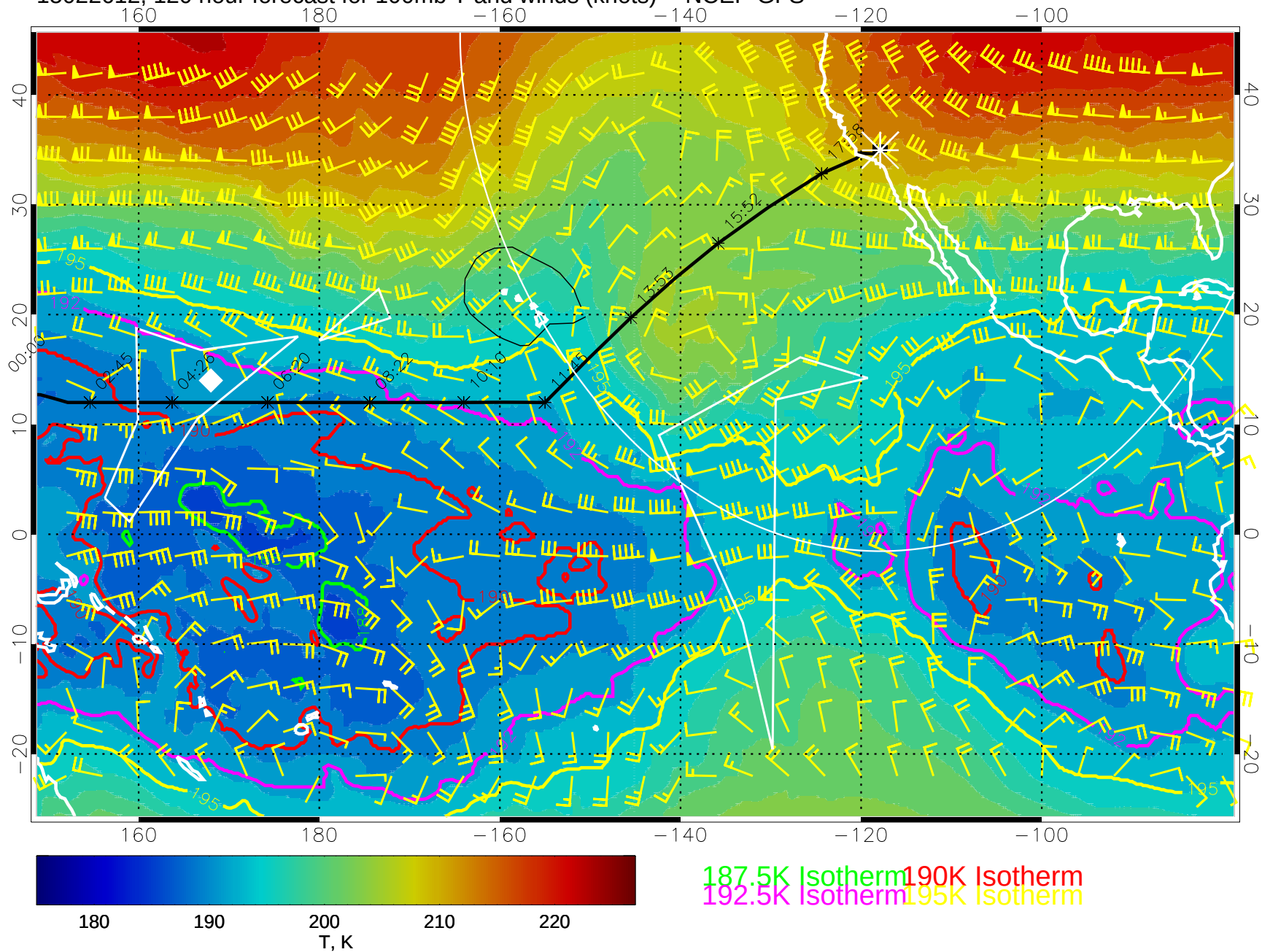
15022612, 120 hour forecast for 100mb T and winds (knots) -- NCEP GFS
