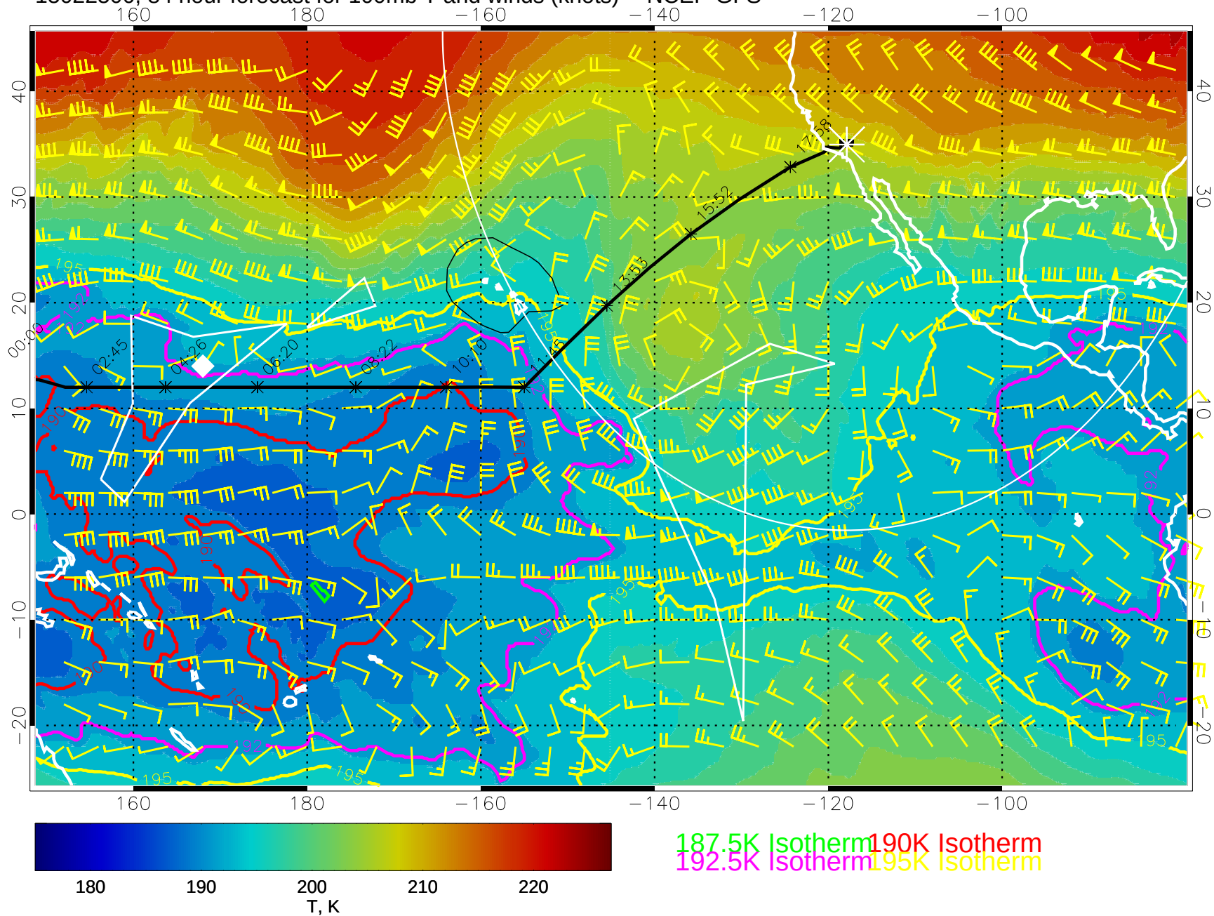
15022500, 84 hour forecast for 100mb T and winds (knots) -- NCEP GFS
