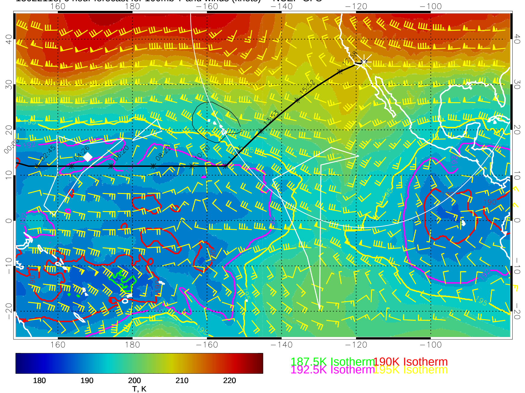
15022118, 6 hour forecast for 100mb T and winds (knots) -- NCEP GFS
