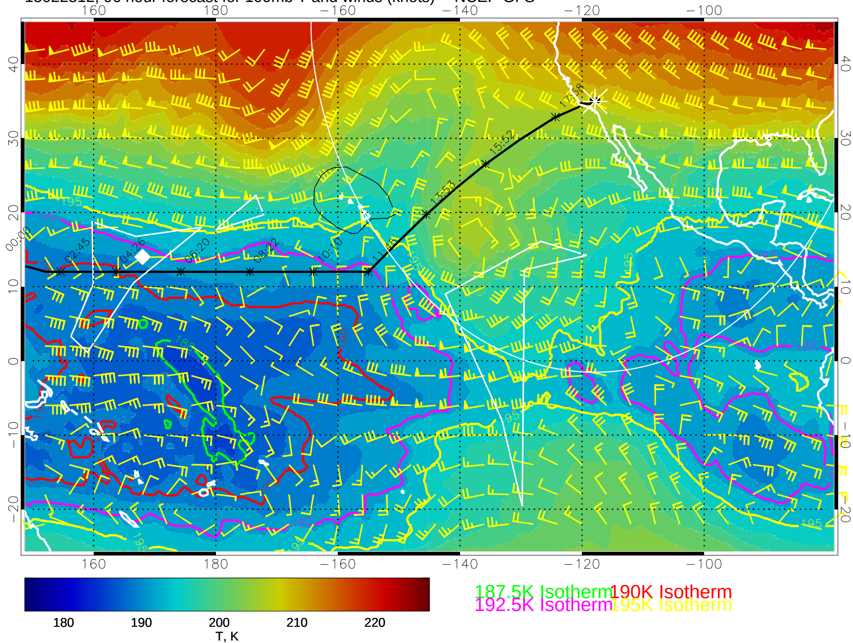
15022512, 96 hour forecast for 100mb T and winds (knots) -- NCEP GFS
