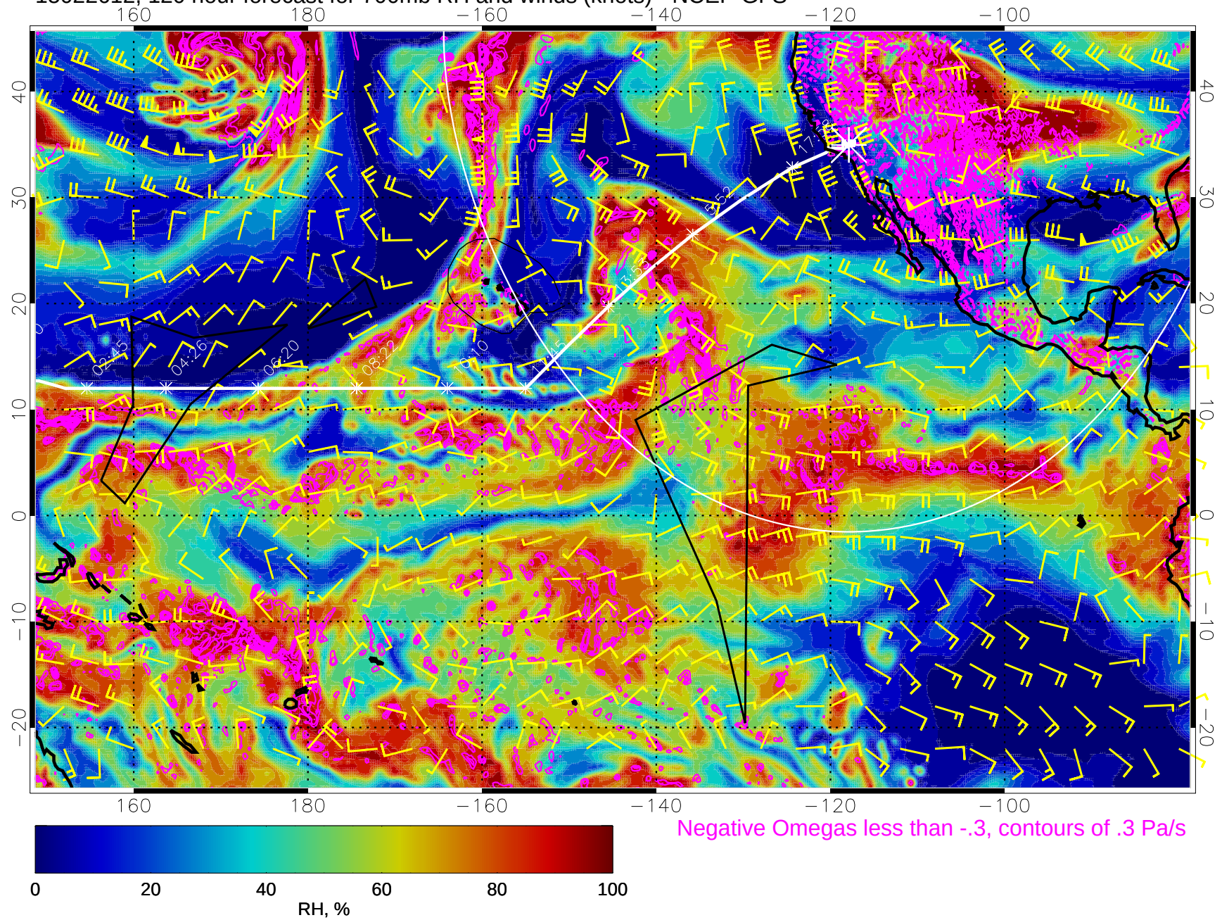
15022612, 120 hour forecast for 700mb RH and winds (knots) - NCEP GFS
