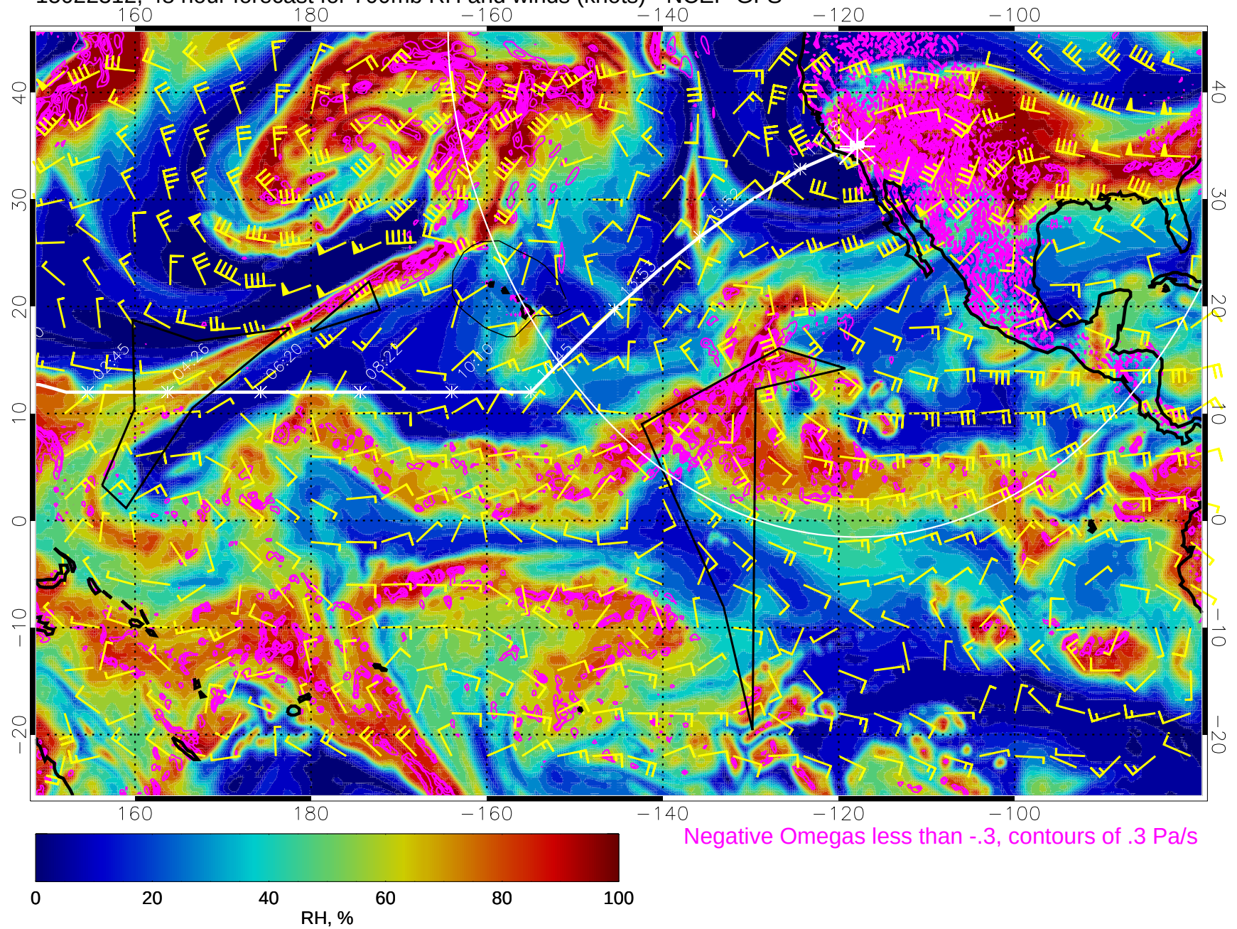
15022312, 48 hour forecast for 700mb RH and winds (knots) - NCEP GFS
