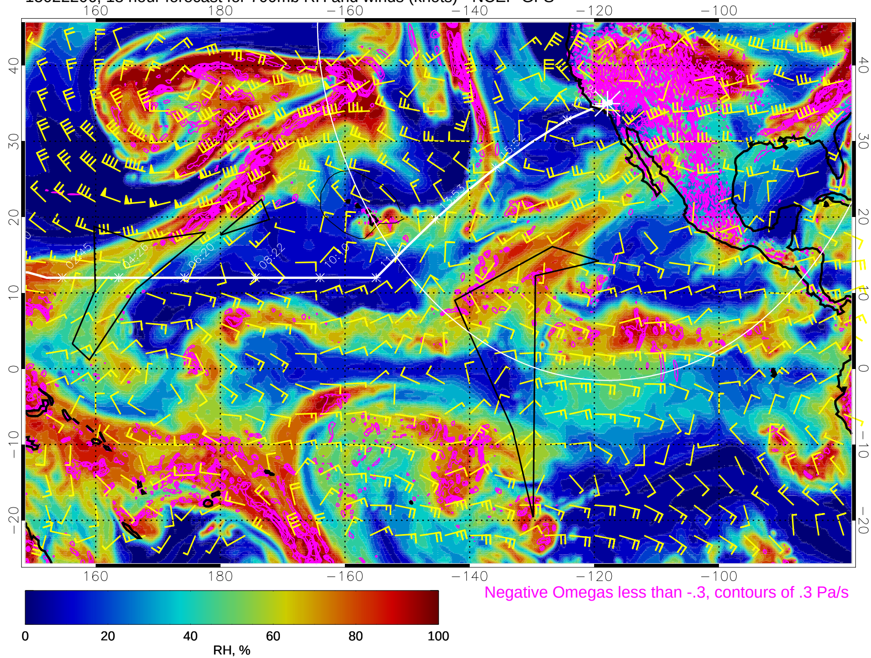
15022206, 18 hour forecast for 700mb RH and winds (knots) - NCEP GFS
