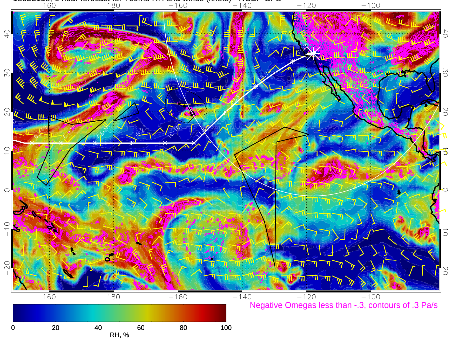
15022118, 6 hour forecast for 700mb RH and winds (knots) - NCEP GFS
