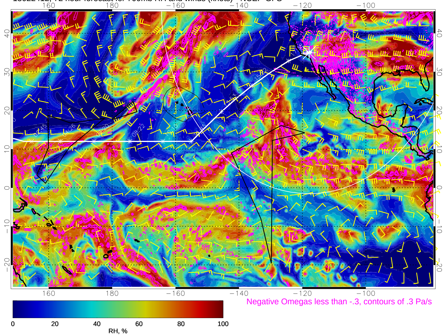
15022412, 72 hour forecast for 700mb RH and winds (knots) - NCEP GFS
