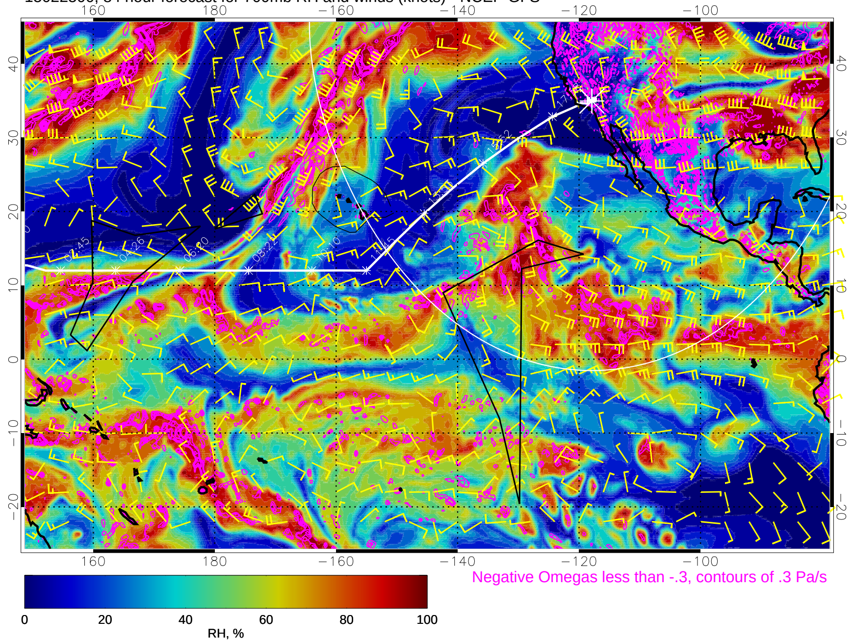
15022500, 84 hour forecast for 700mb RH and winds (knots) - NCEP GFS
