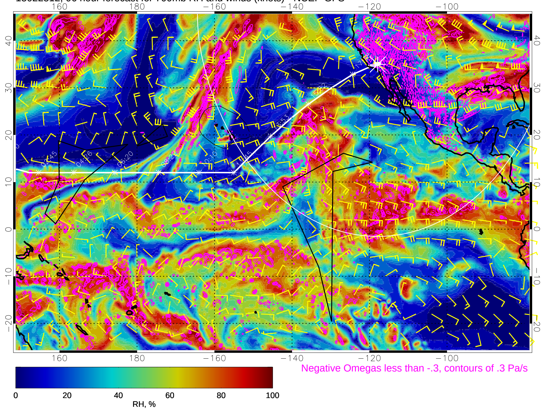
15022512, 96 hour forecast for 700mb RH and winds (knots) - NCEP GFS
