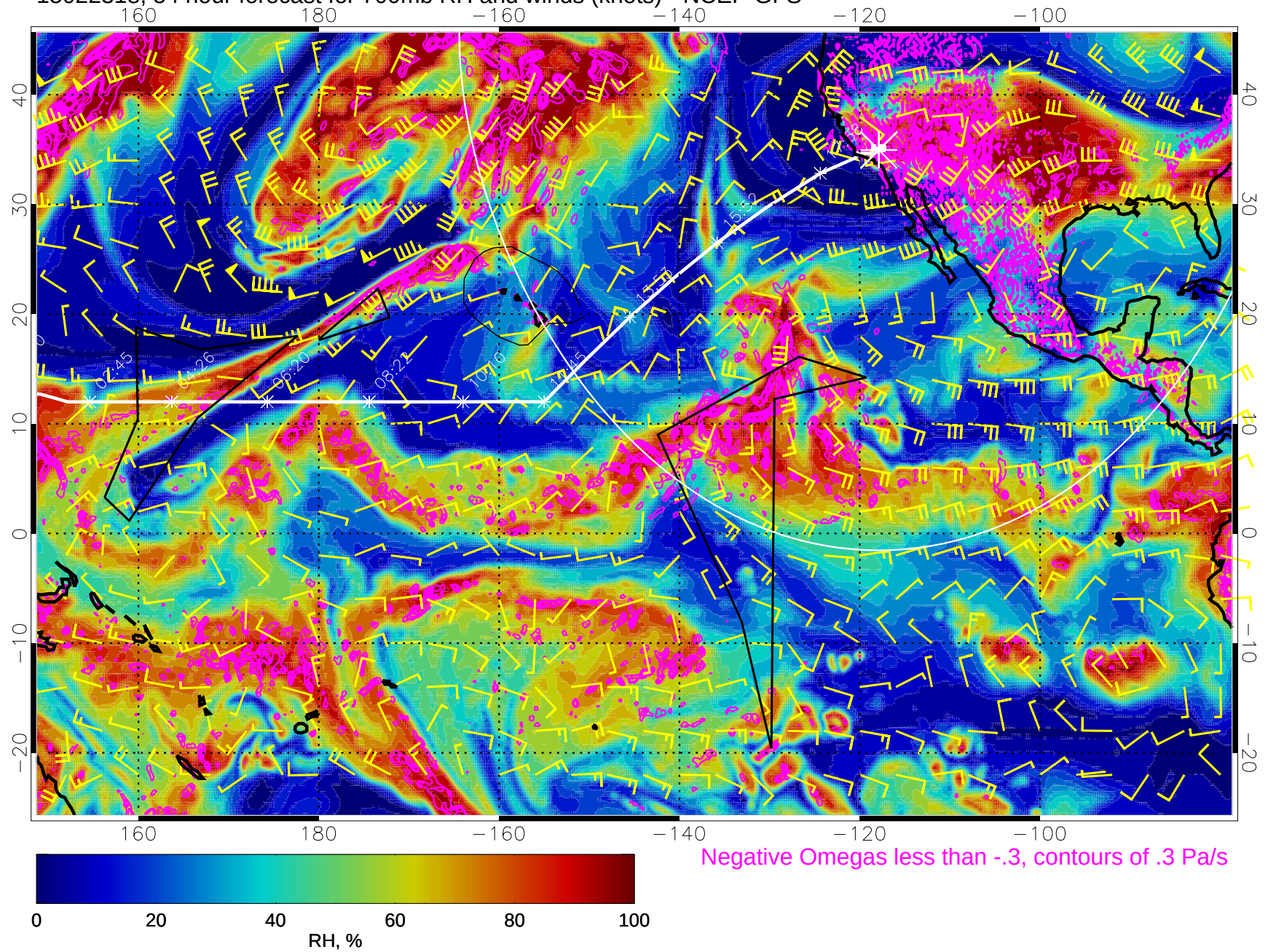
15022318, 54 hour forecast for 700mb RH and winds (knots) - NCEP GFS
