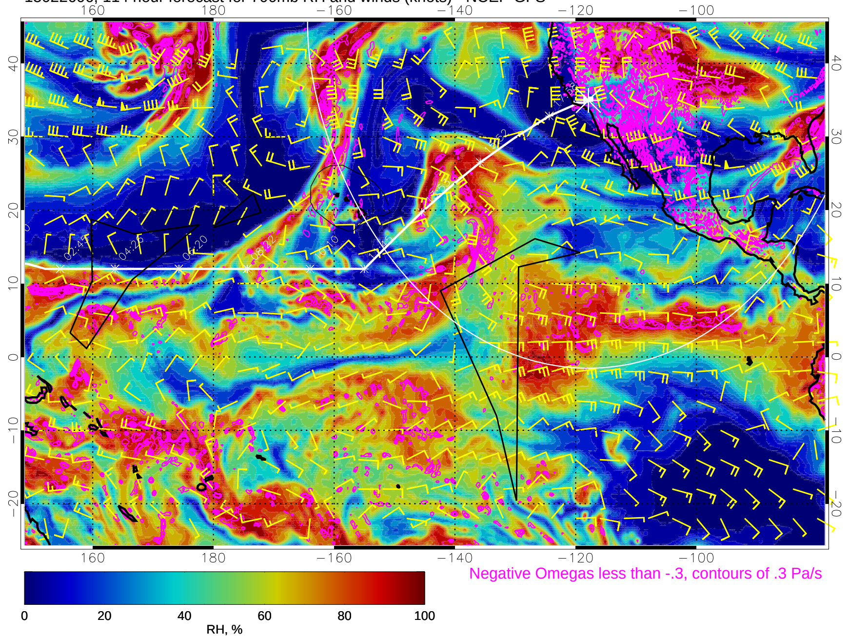
15022606, 114 hour forecast for 700mb RH and winds (knots) - NCEP GFS
