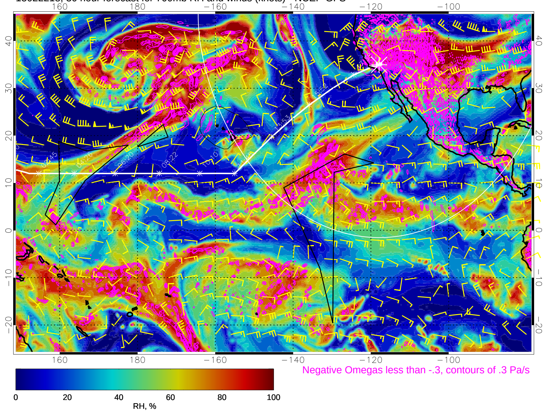
15022218, 30 hour forecast for 700mb RH and winds (knots) - NCEP GFS
