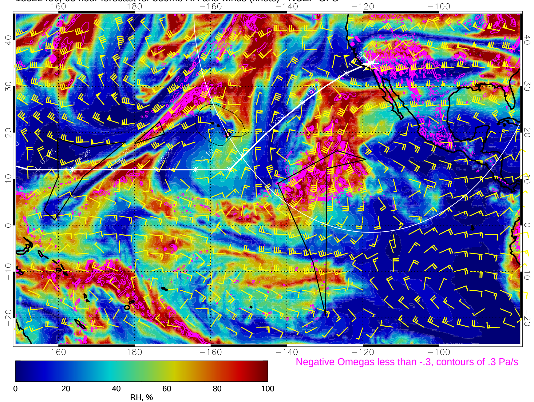
15022406, 66 hour forecast for 500mb RH and winds (knots) - NCEP GFS
