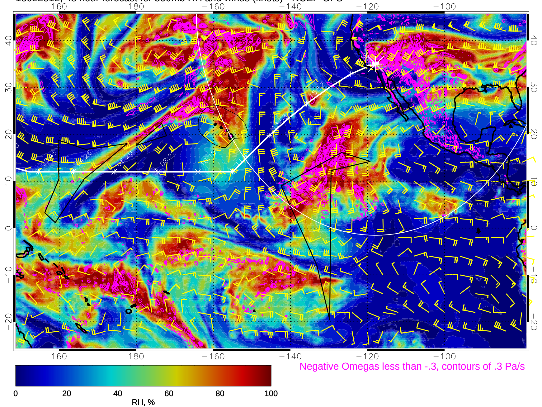
15022312, 48 hour forecast for 500mb RH and winds (knots) - NCEP GFS
