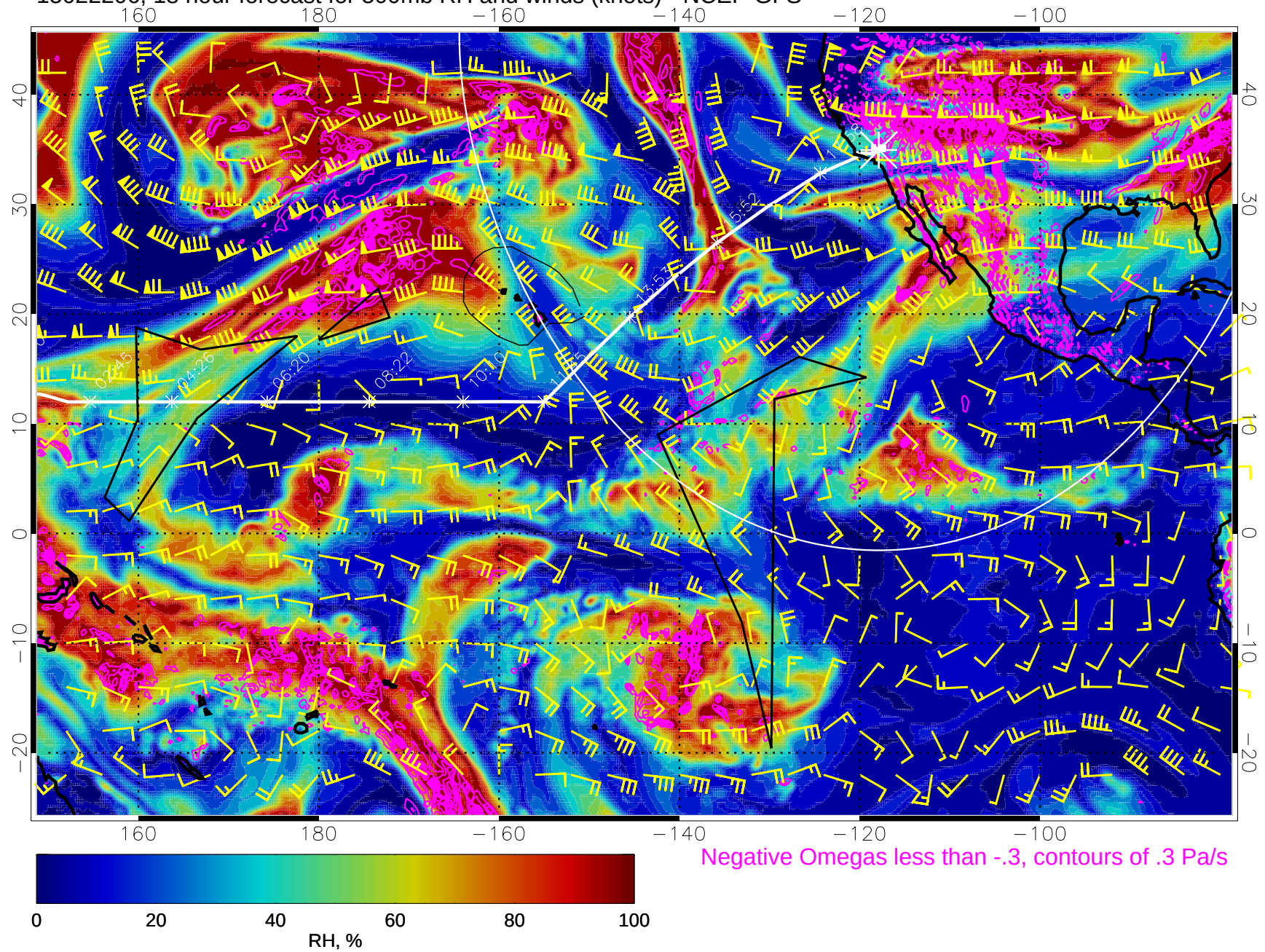
15022206, 18 hour forecast for 500mb RH and winds (knots) - NCEP GFS
