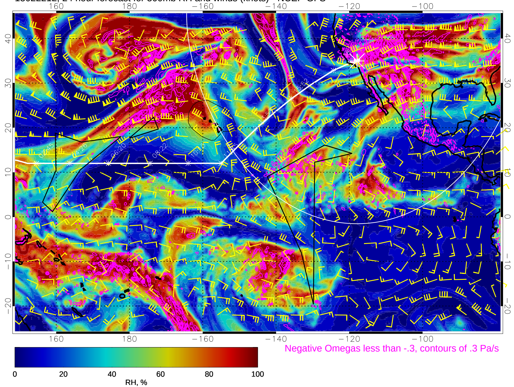
15022212, 24 hour forecast for 500mb RH and winds (knots) - NCEP GFS
