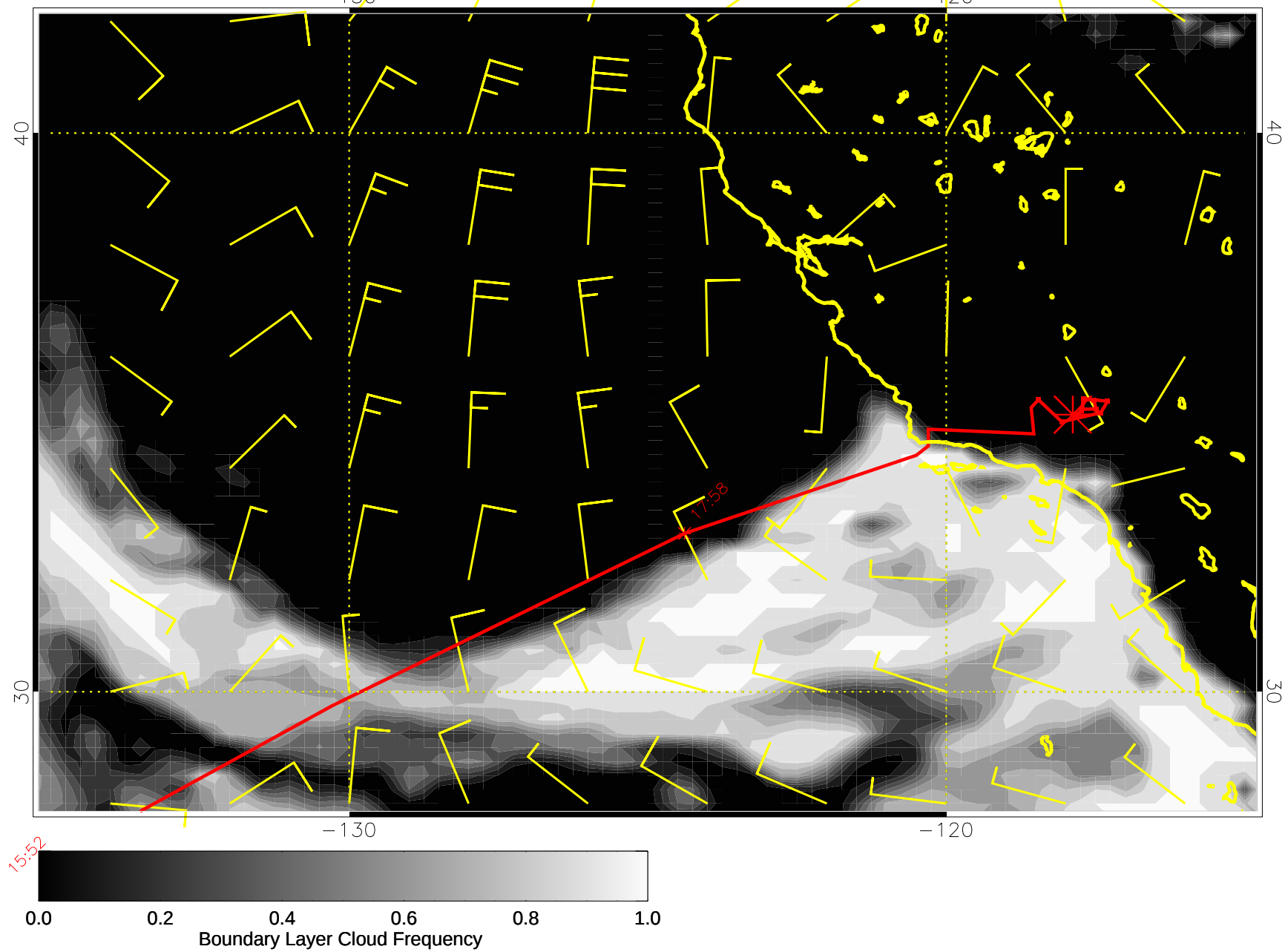
15022118, 6 hour forecast for surface winds (knots) and Boundary Layer Cloud Frequency -- NCEP GFS
