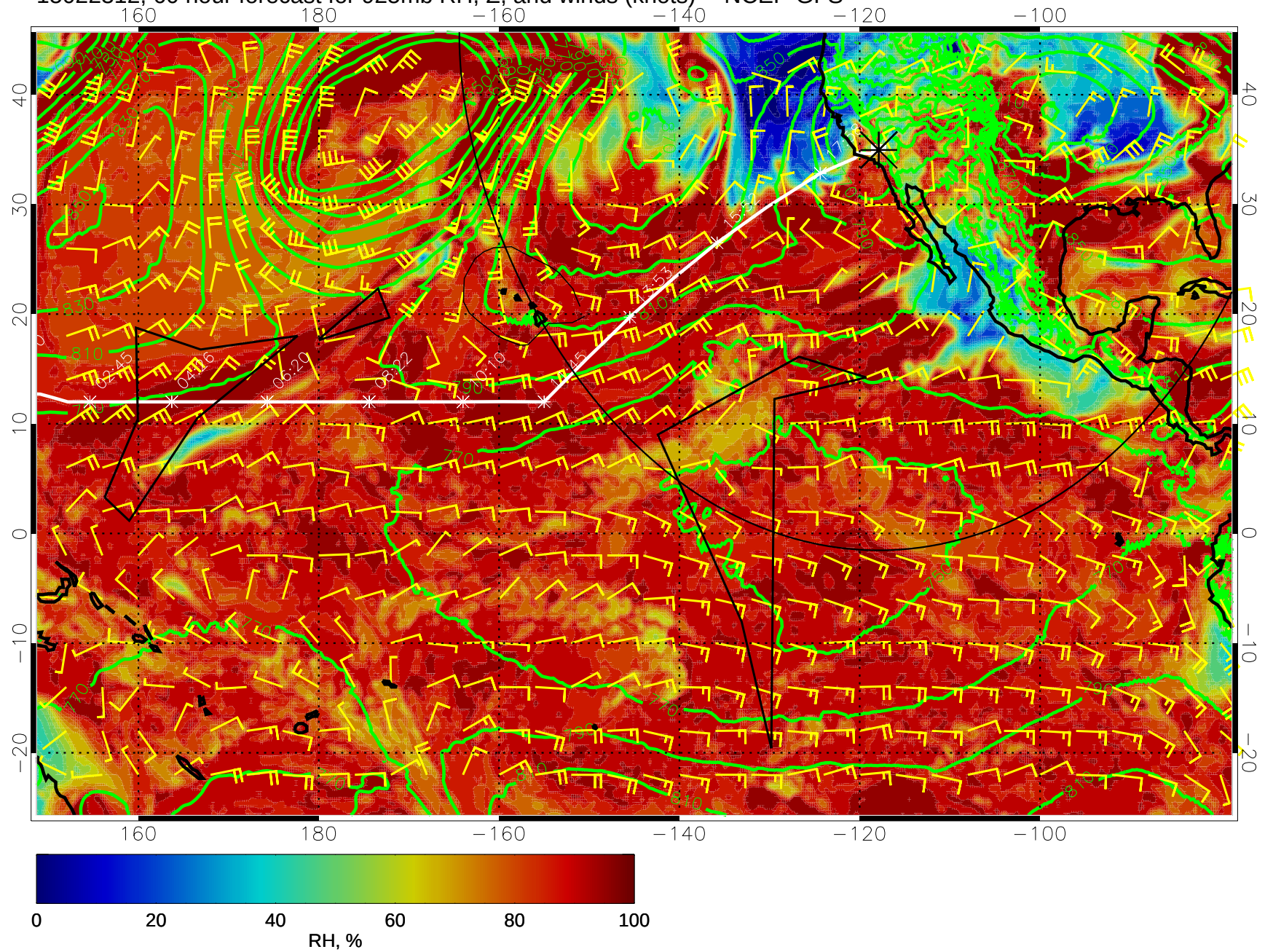
15022312, 60 hour forecast for 925mb RH, Z, and winds (knots) -- NCEP GFS
