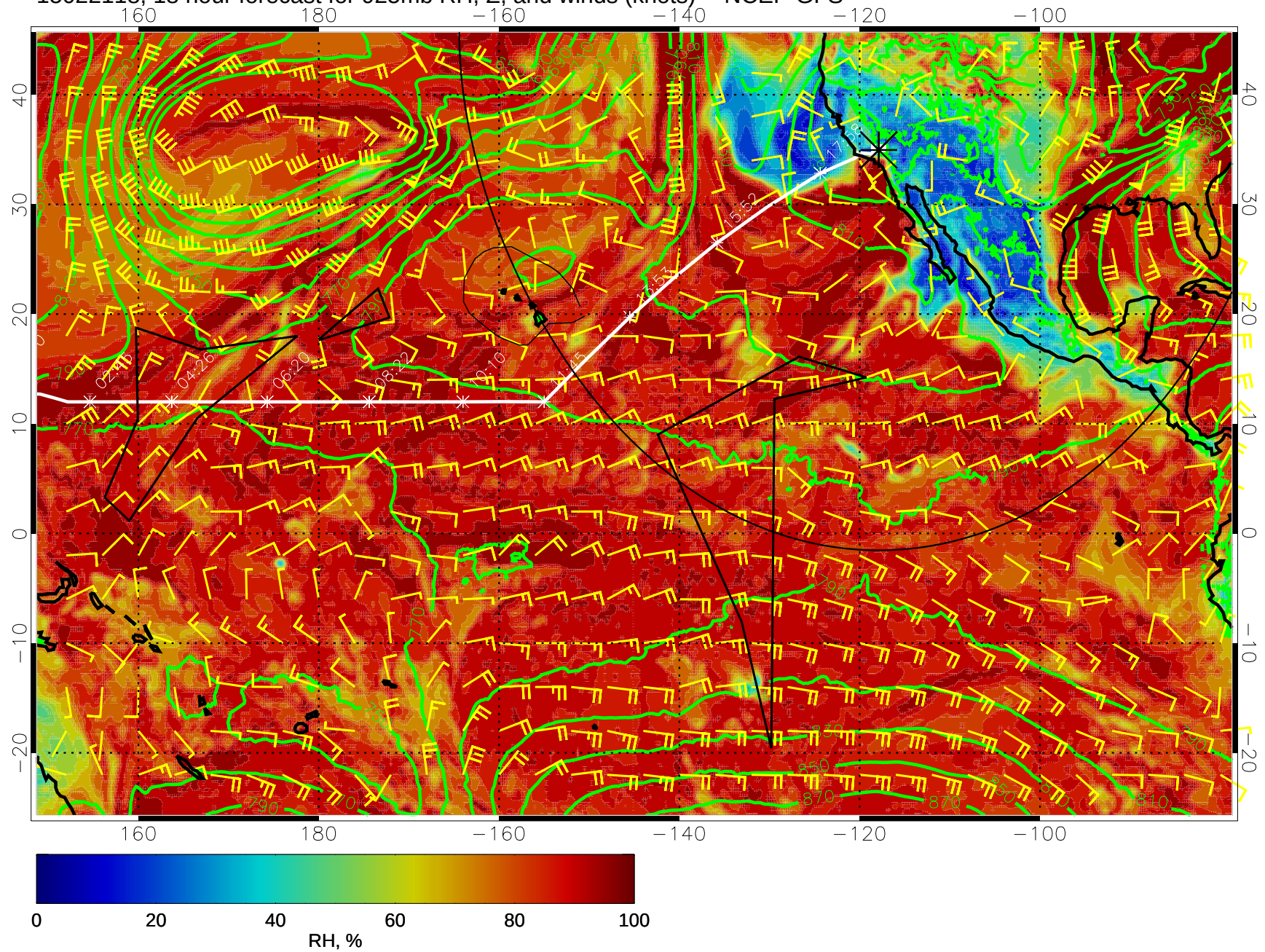
15022118, 18 hour forecast for 925mb RH, Z, and winds (knots) -- NCEP GFS
