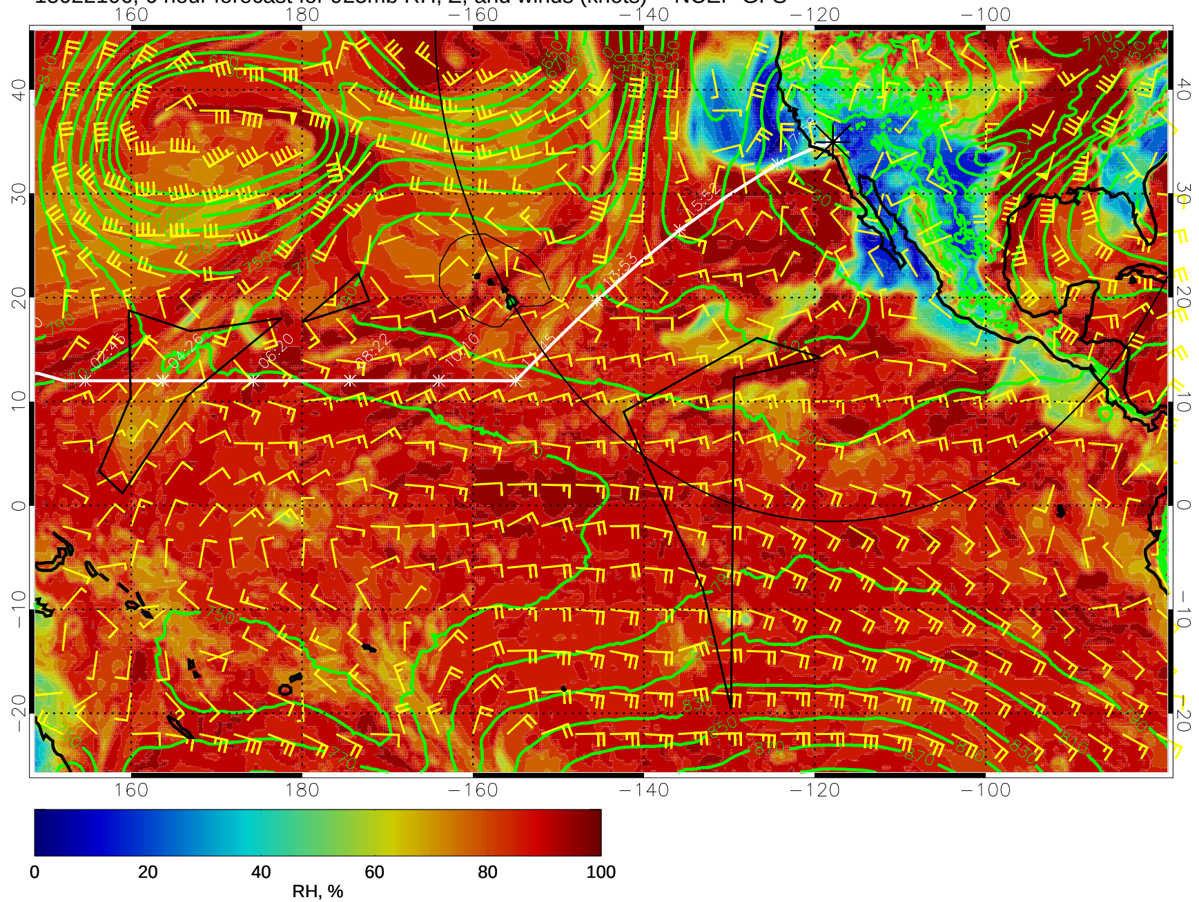
15022106, 6 hour forecast for 925mb RH, Z, and winds (knots) -- NCEP GFS
