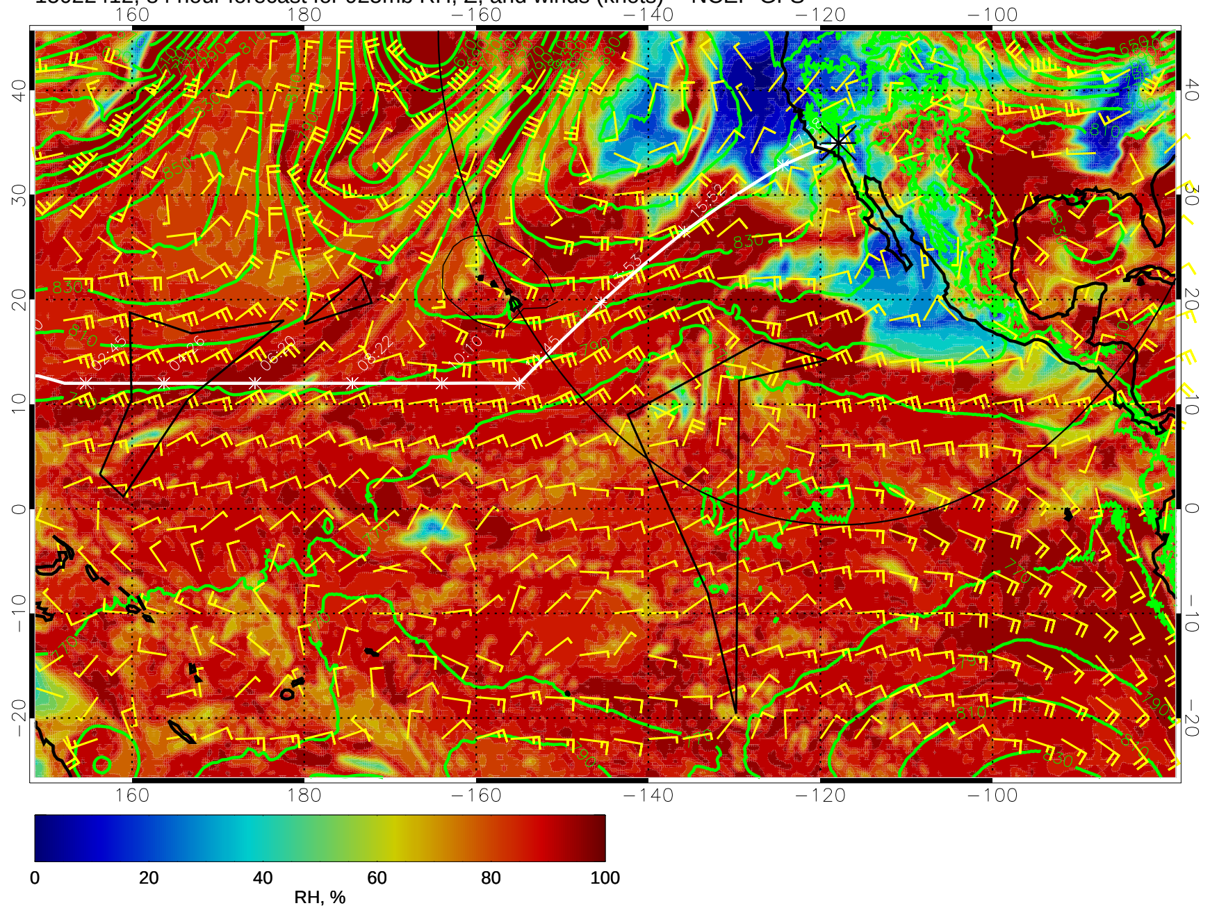
15022412, 84 hour forecast for 925mb RH, Z, and winds (knots) -- NCEP GFS
