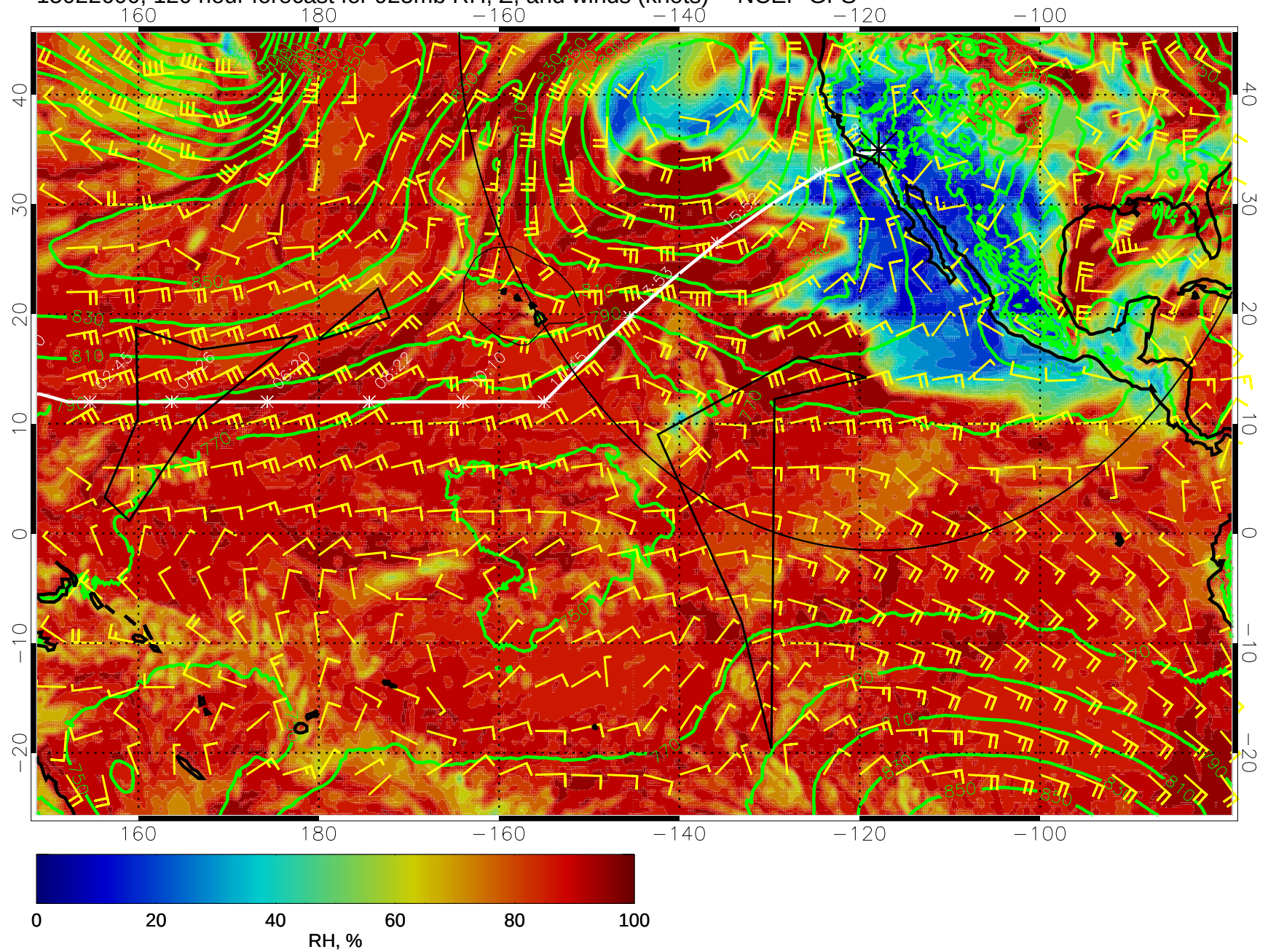
15022600, 120 hour forecast for 925mb RH, Z, and winds (knots) -- NCEP GFS
