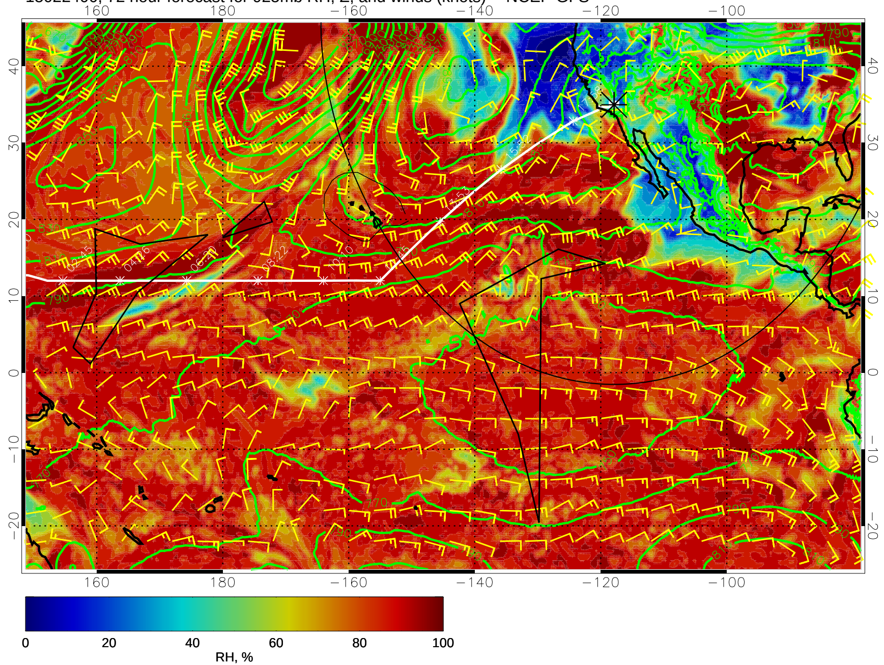
15022400, 72 hour forecast for 925mb RH, Z, and winds (knots) -- NCEP GFS
