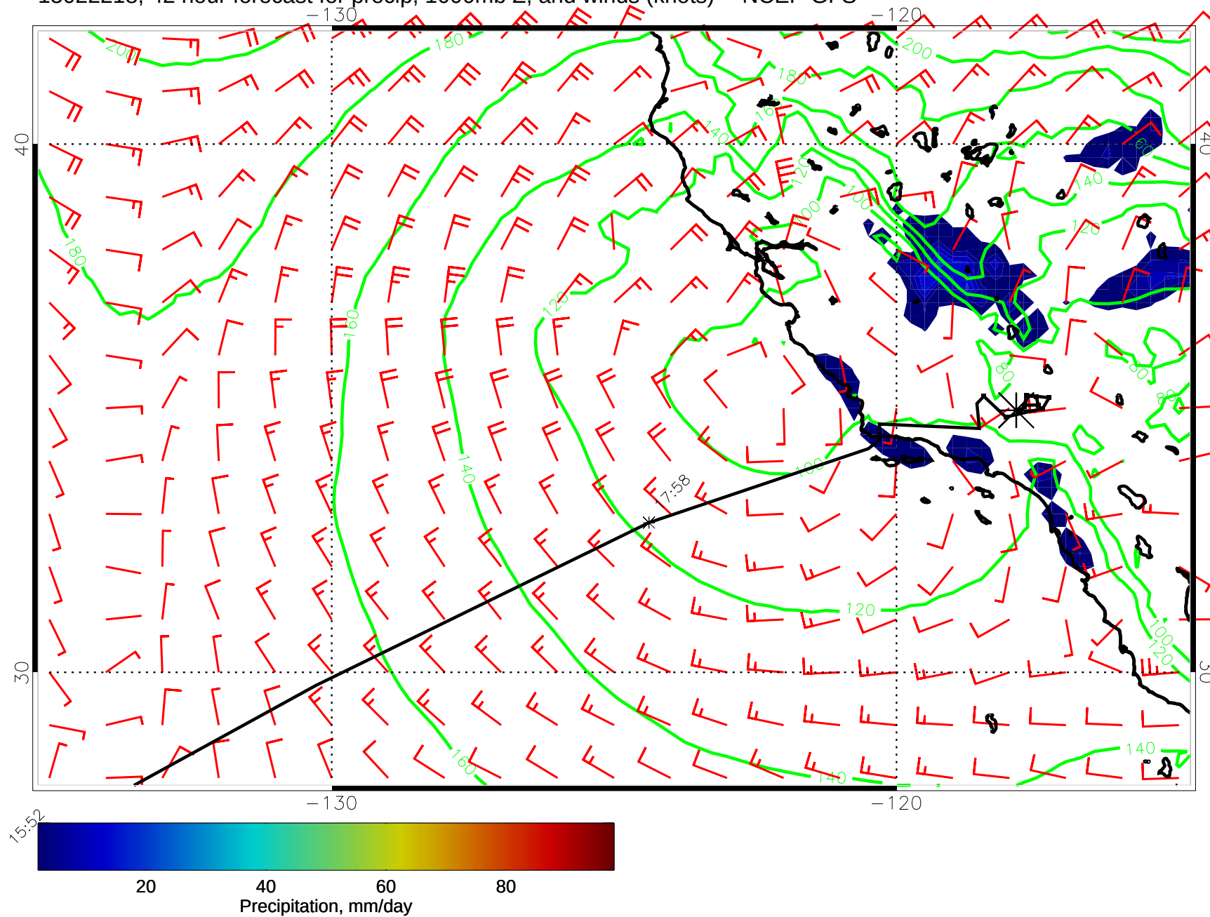
15022218, 42 hour forecast for precip, 1000mb Z, and winds (knots) -- NCEP GFS
