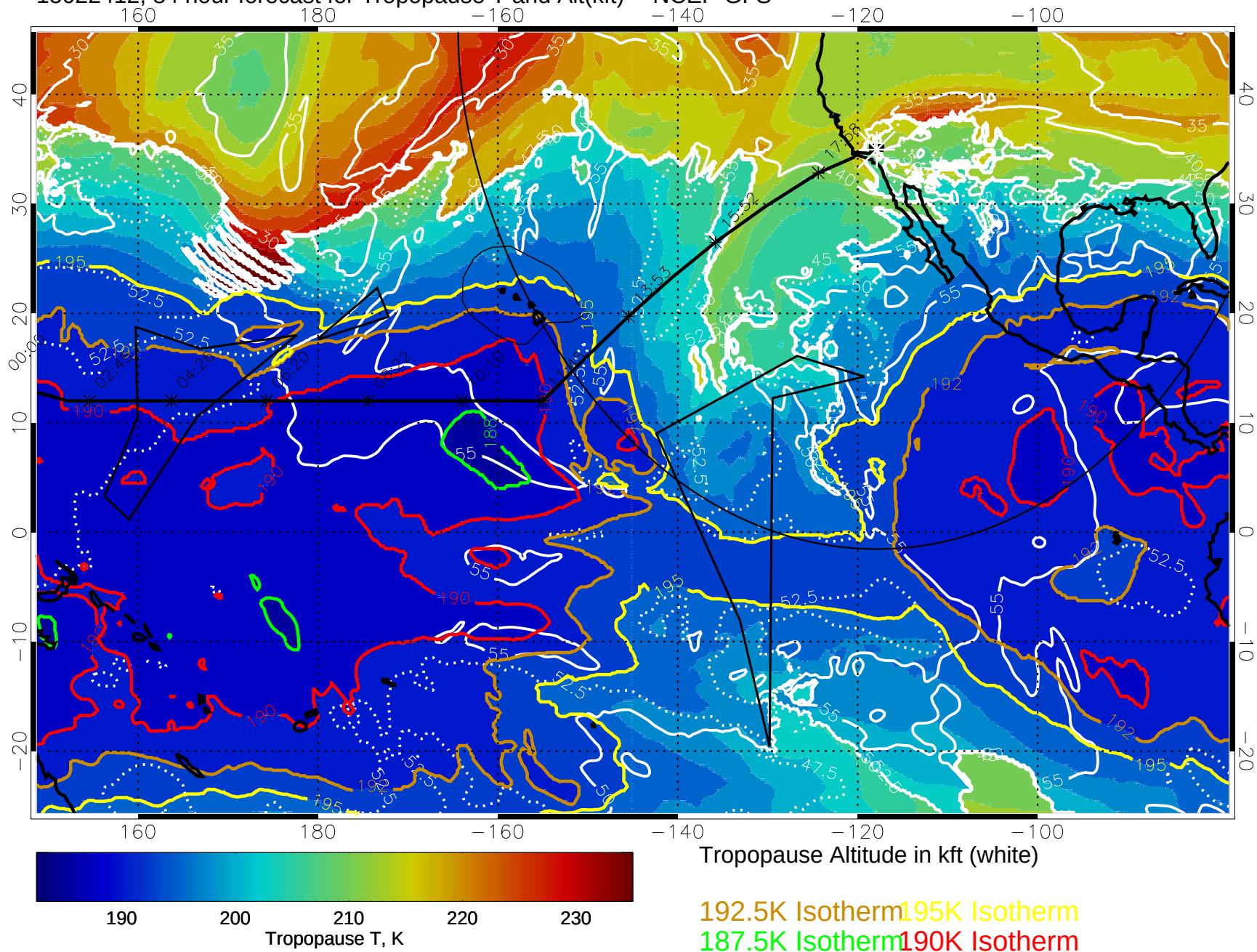
15022412, 84 hour forecast for Tropopause T and Alt(kft) -- NCEP GFS
