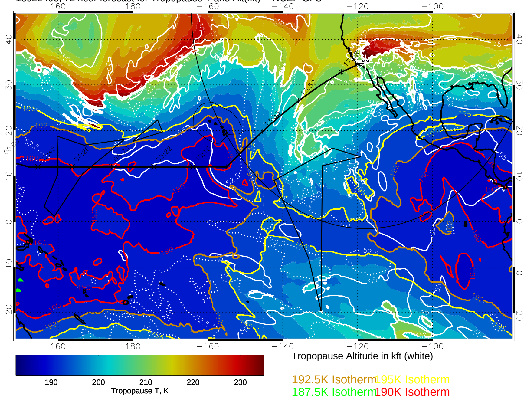
15022400, 72 hour forecast for Tropopause T and Alt(kft) -- NCEP GFS
