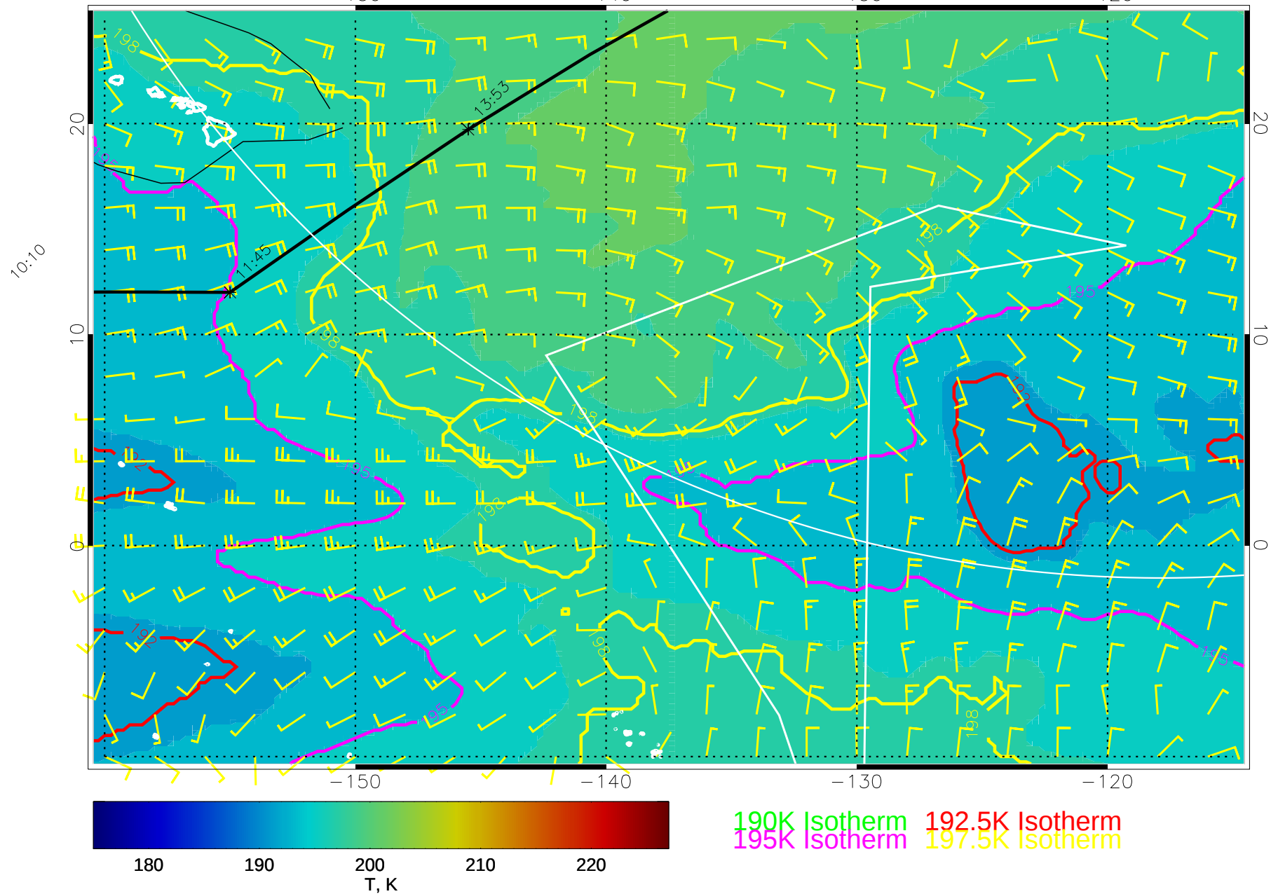
15022506, 102 hour forecast for 70mb T and winds (knots) -- NCEP GFS
