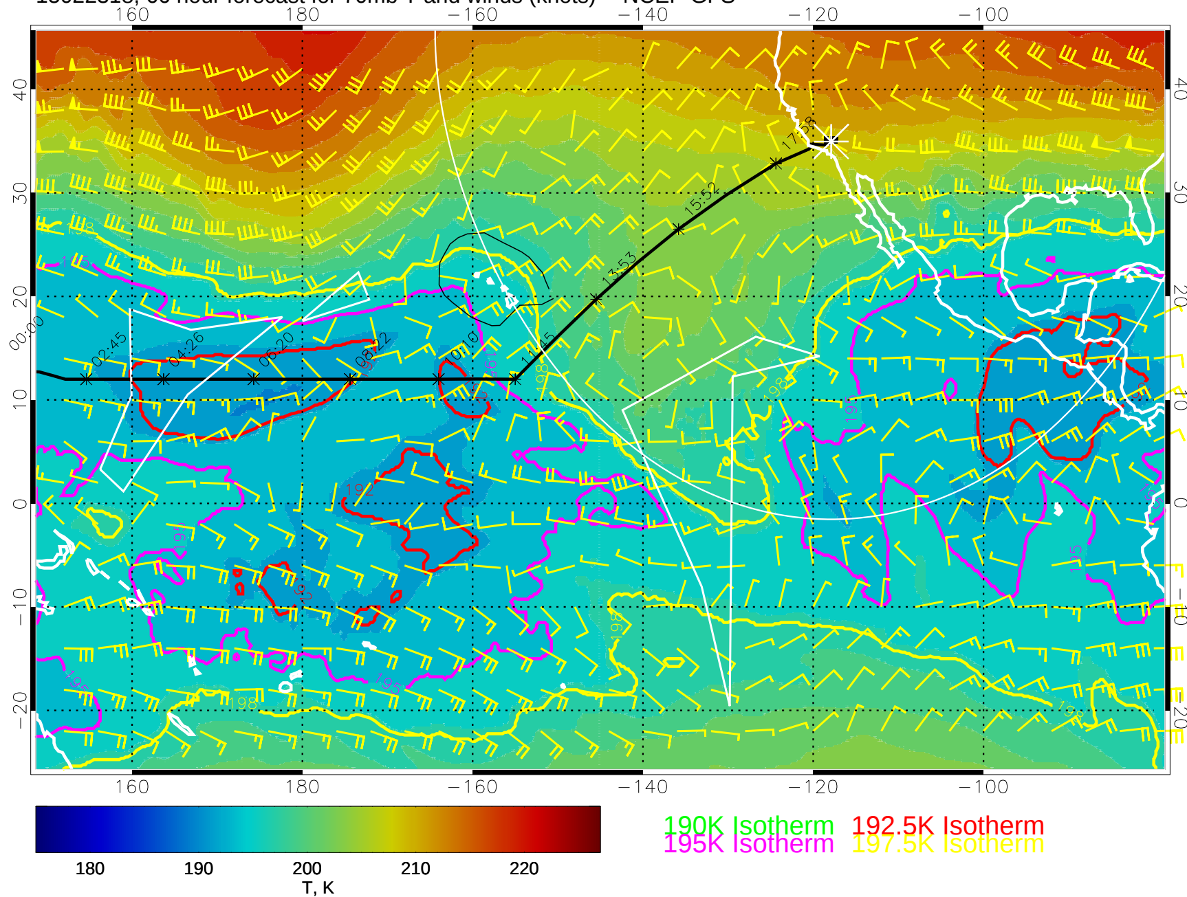
15022318, 66 hour forecast for 70mb T and winds (knots) -- NCEP GFS
