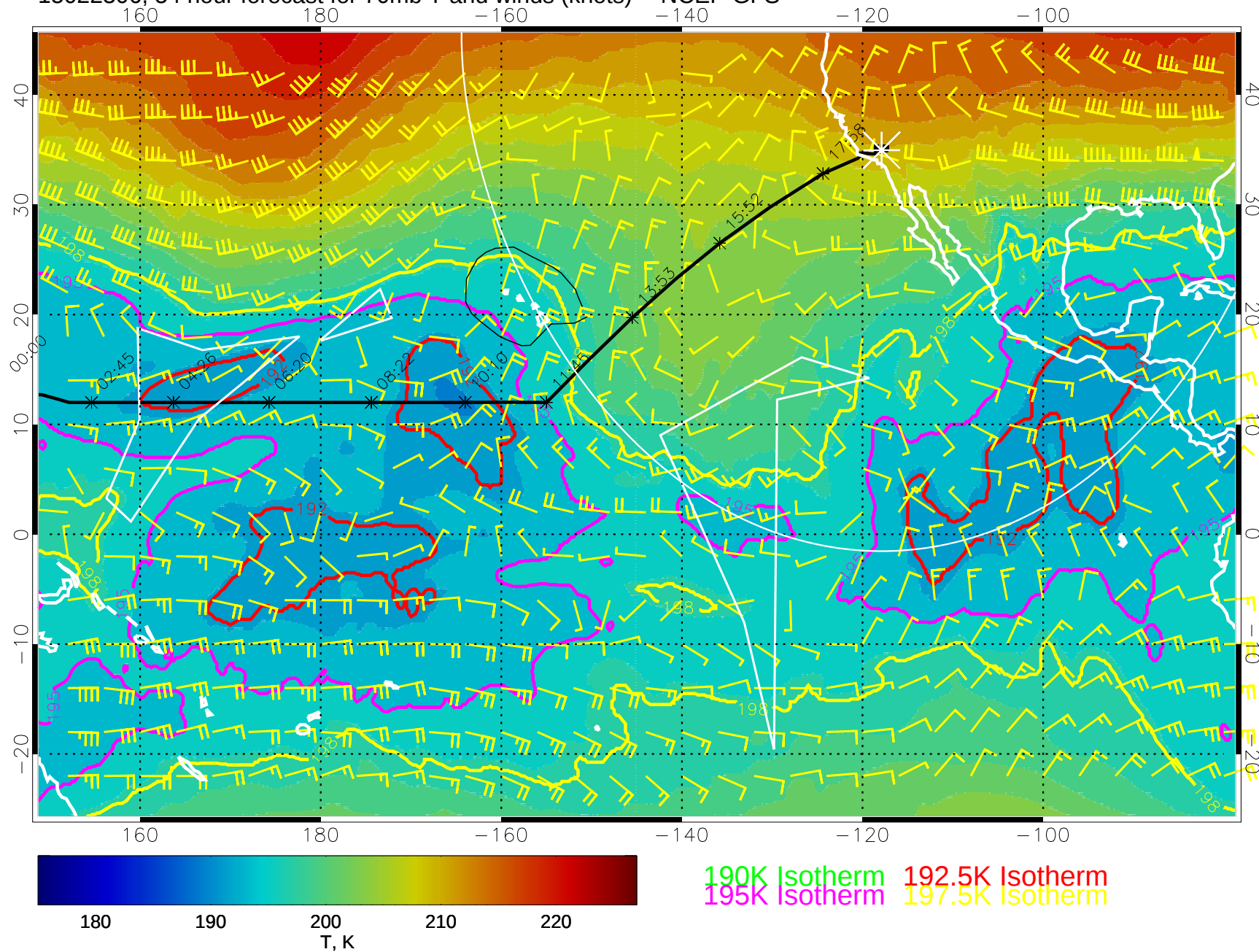
15022306, 54 hour forecast for 70mb T and winds (knots) -- NCEP GFS
