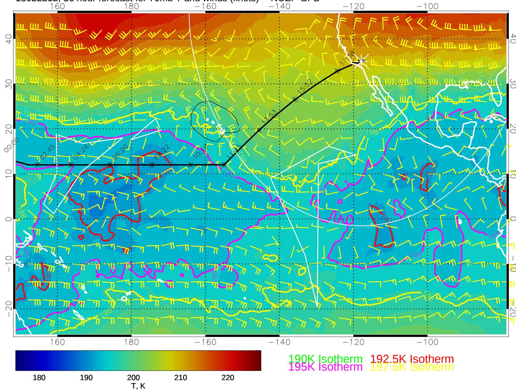
15022212, 36 hour forecast for 70mb T and winds (knots) -- NCEP GFS
