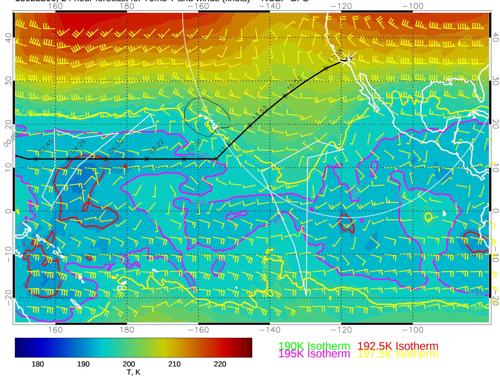
15022200, 24 hour forecast for 70mb T and winds (knots) -- NCEP GFS
