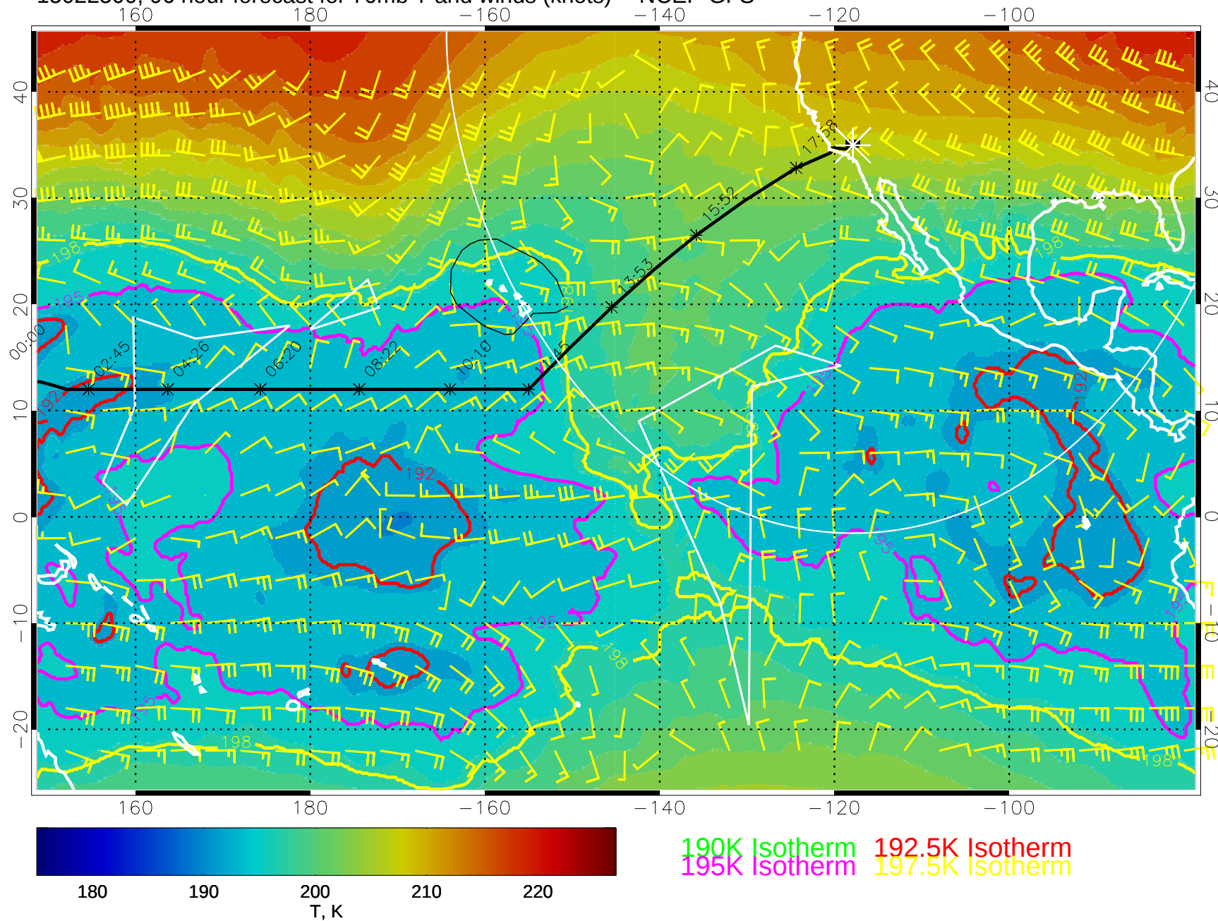
15022500, 96 hour forecast for 70mb T and winds (knots) -- NCEP GFS
