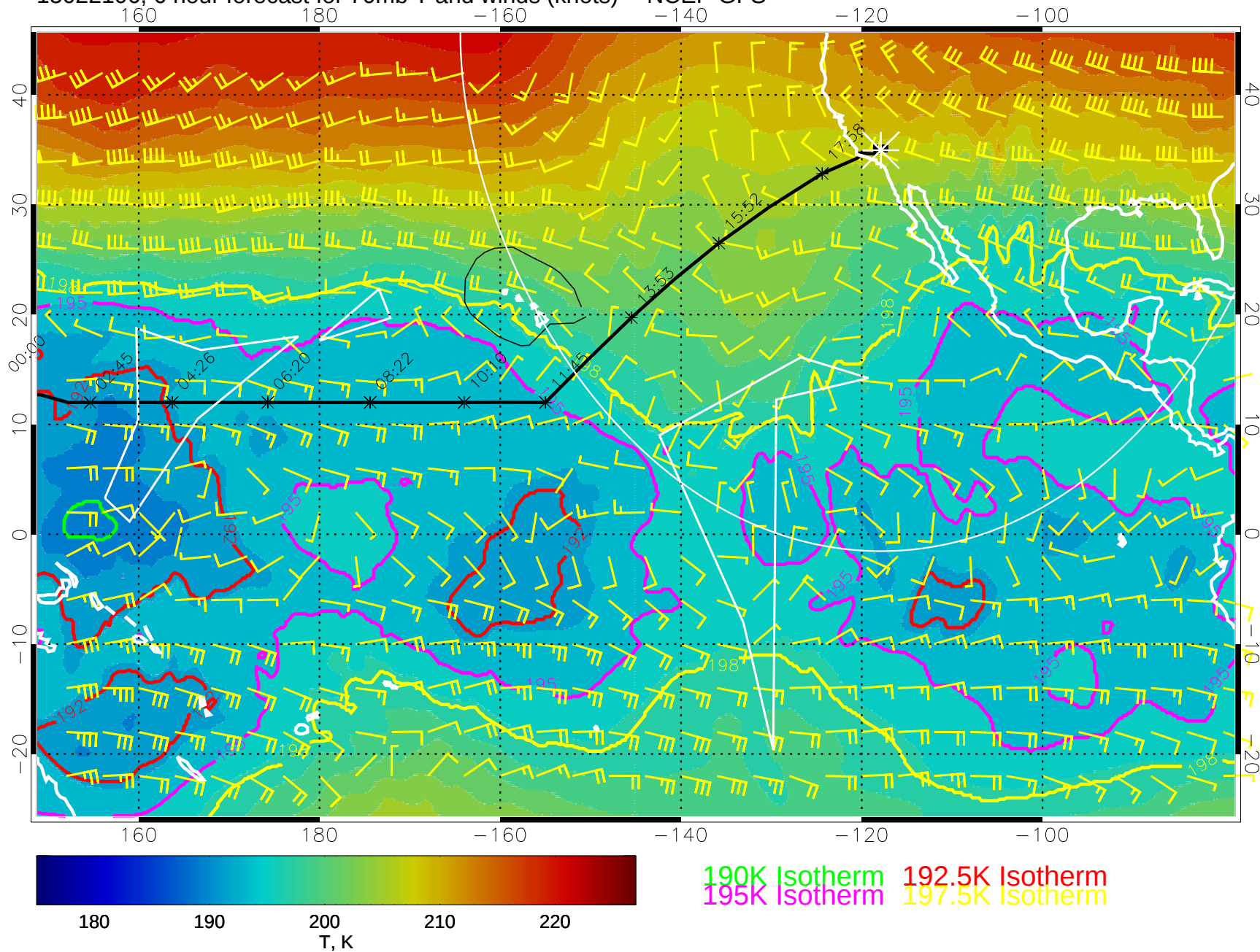
15022106, 6 hour forecast for 70mb T and winds (knots) -- NCEP GFS
