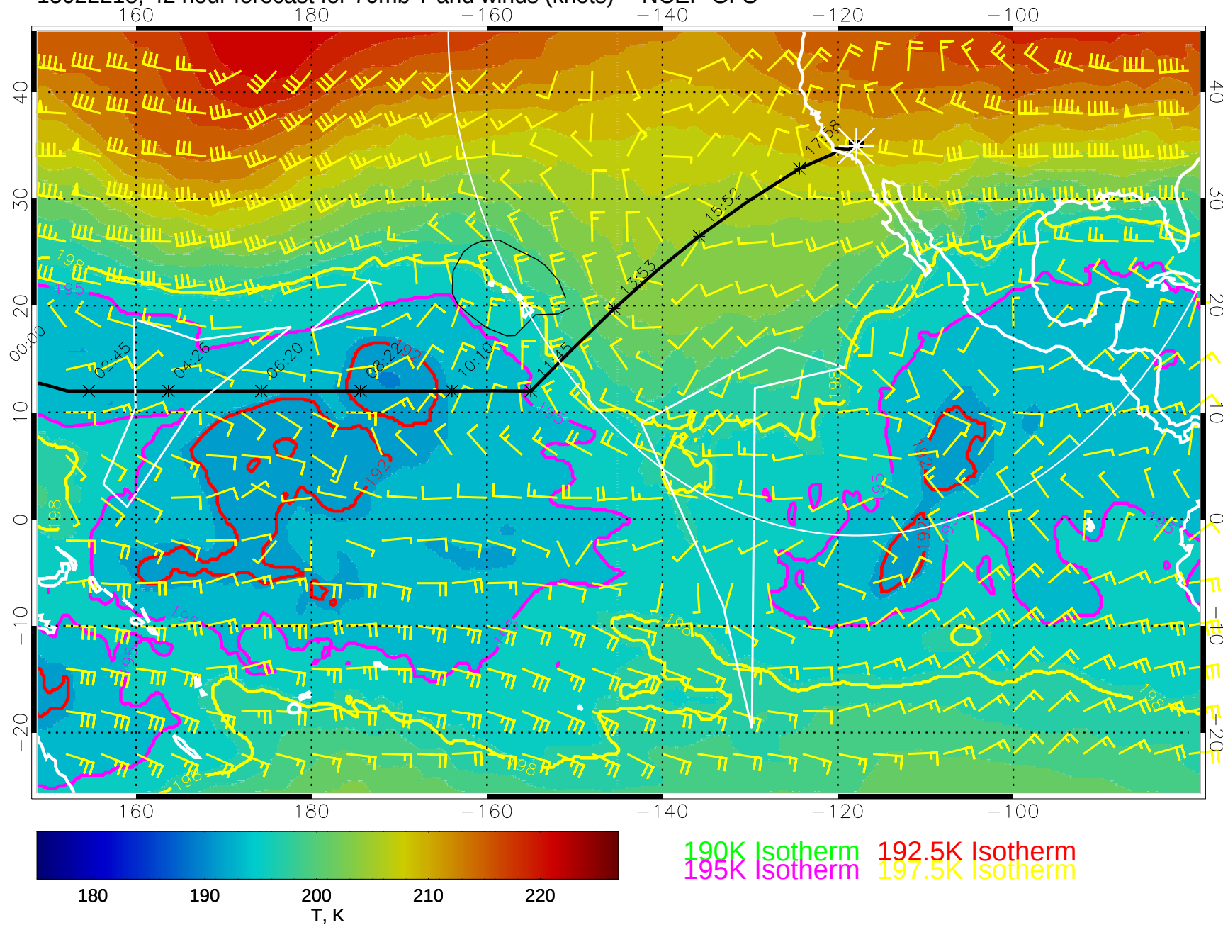
15022218, 42 hour forecast for 70mb T and winds (knots) -- NCEP GFS
