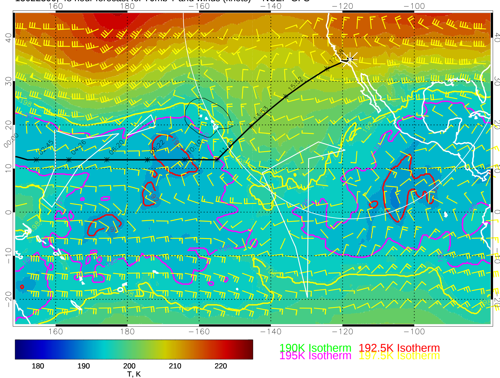
15022300, 48 hour forecast for 70mb T and winds (knots) -- NCEP GFS
