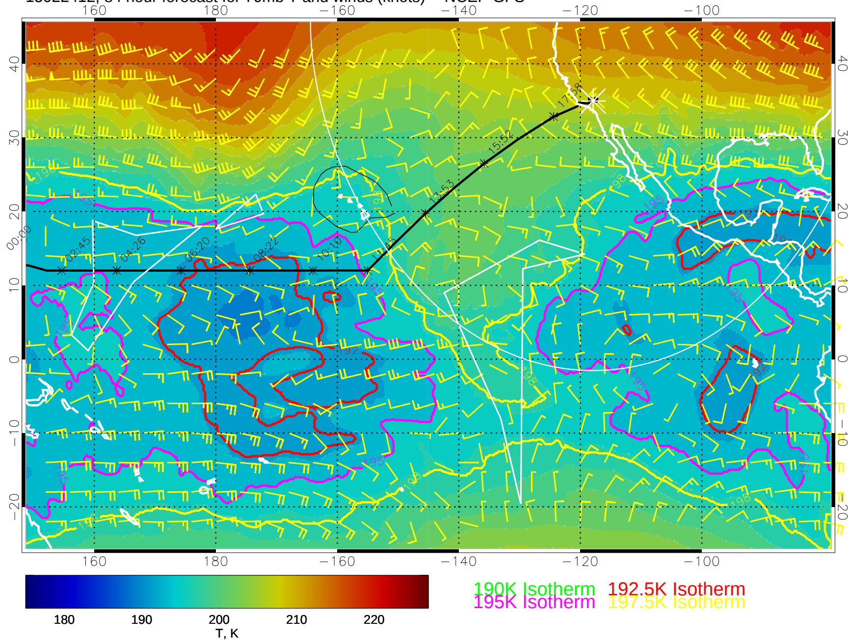
15022412, 84 hour forecast for 70mb T and winds (knots) -- NCEP GFS
