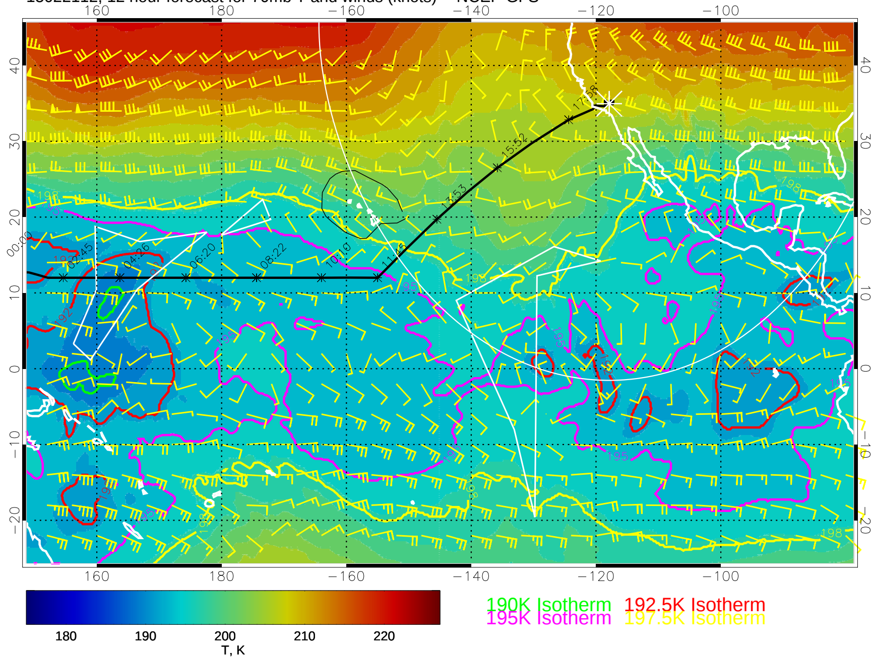
15022112, 12 hour forecast for 70mb T and winds (knots) -- NCEP GFS
