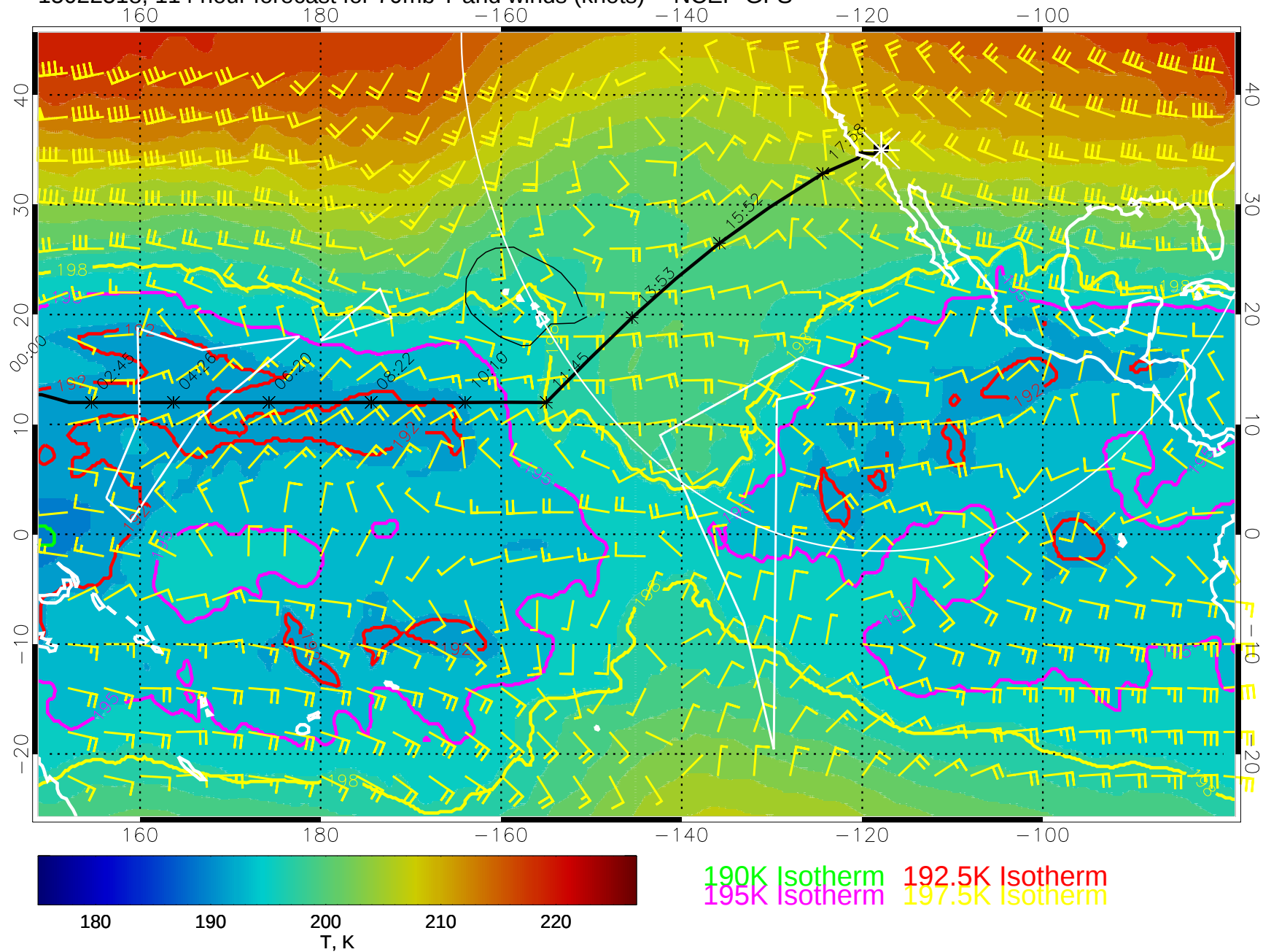
15022518, 114 hour forecast for 70mb T and winds (knots) -- NCEP GFS
