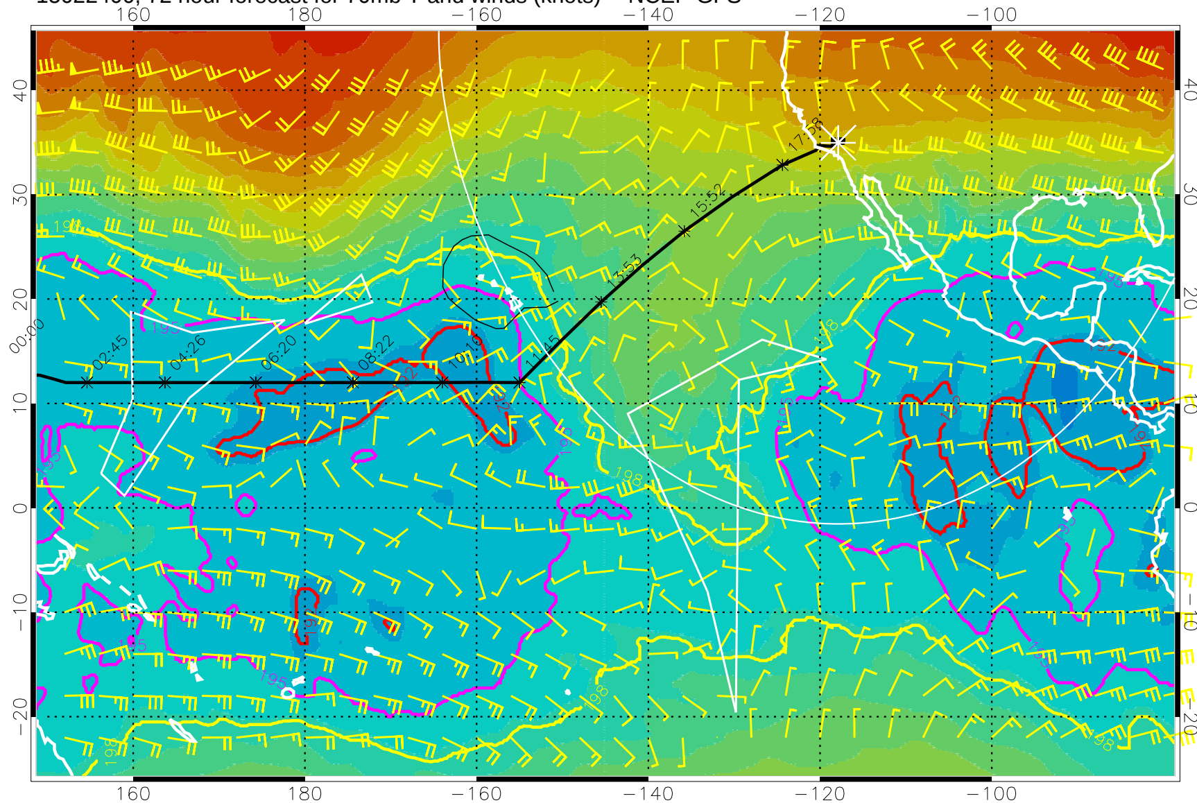
15022400, 72 hour forecast for 70mb T and winds (knots) -- NCEP GFS
