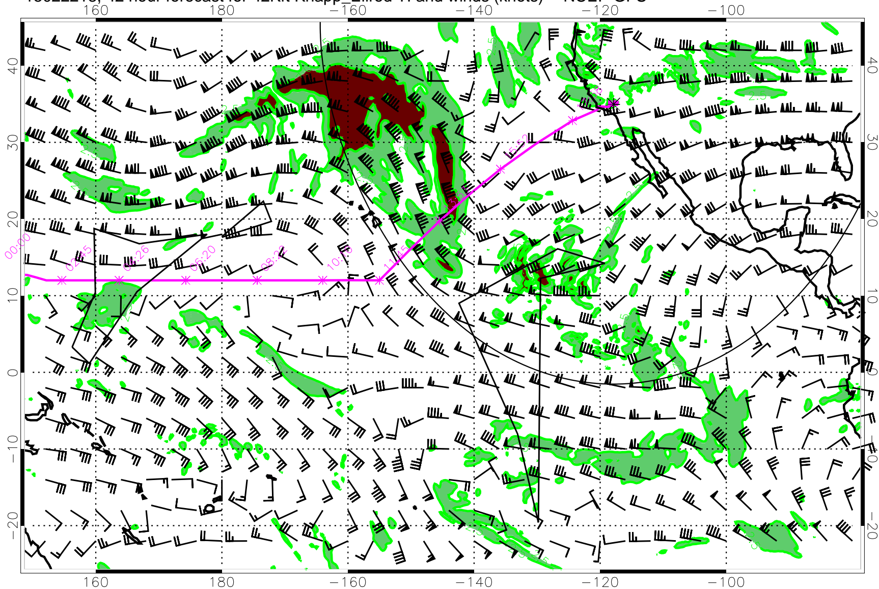
15022218, 42 hour forecast for 42Kft Knapp_Ellrod TI and winds (knots) -- NCEP GFS
