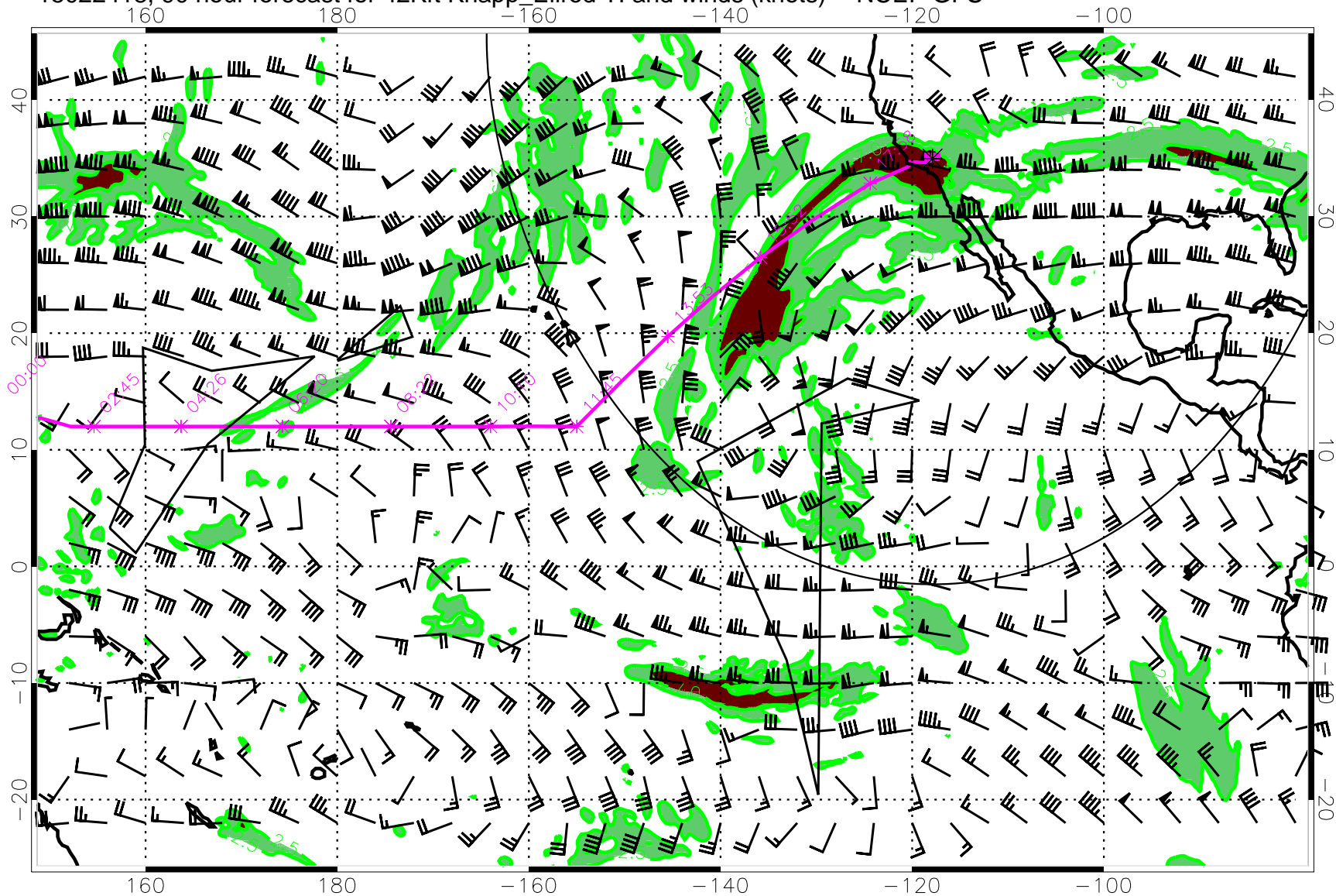
15022418, 90 hour forecast for 42Kft Knapp_Ellrod TI and winds (knots) -- NCEP GFS
