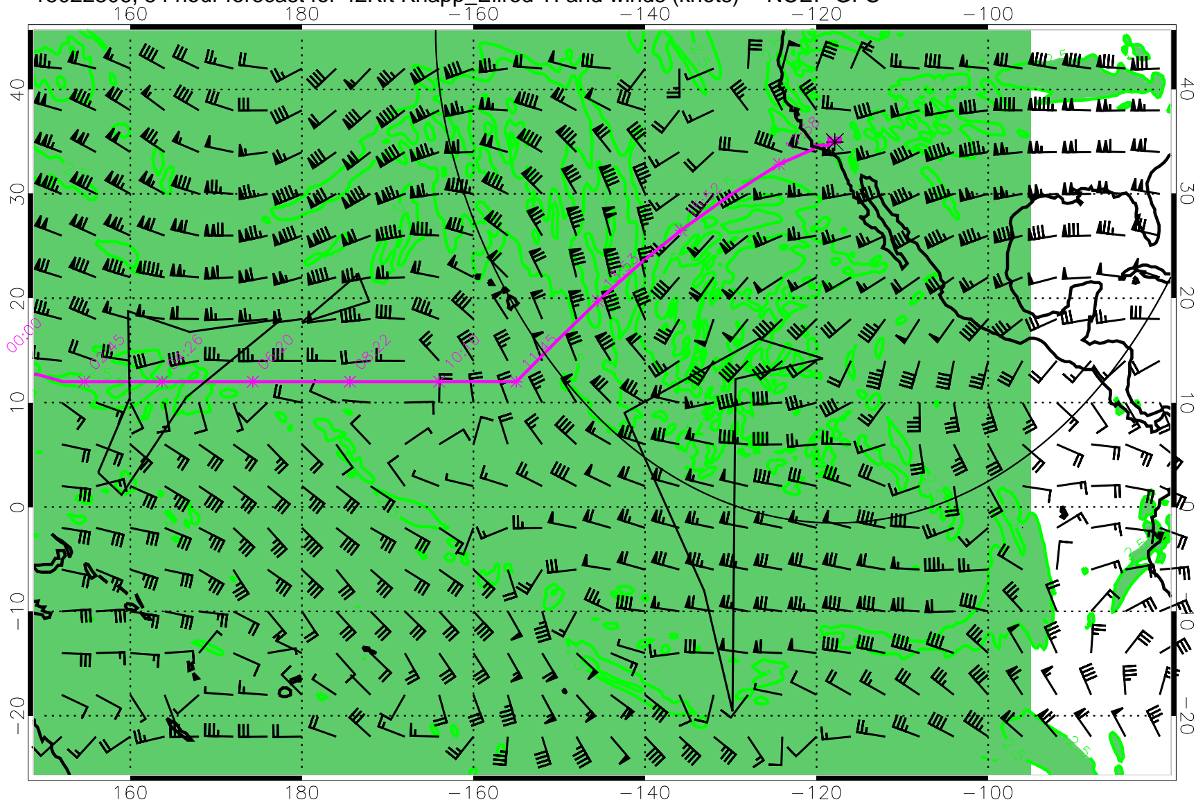
15022306, 54 hour forecast for 42Kft Knapp_Ellrod TI and winds (knots) -- NCEP GFS
