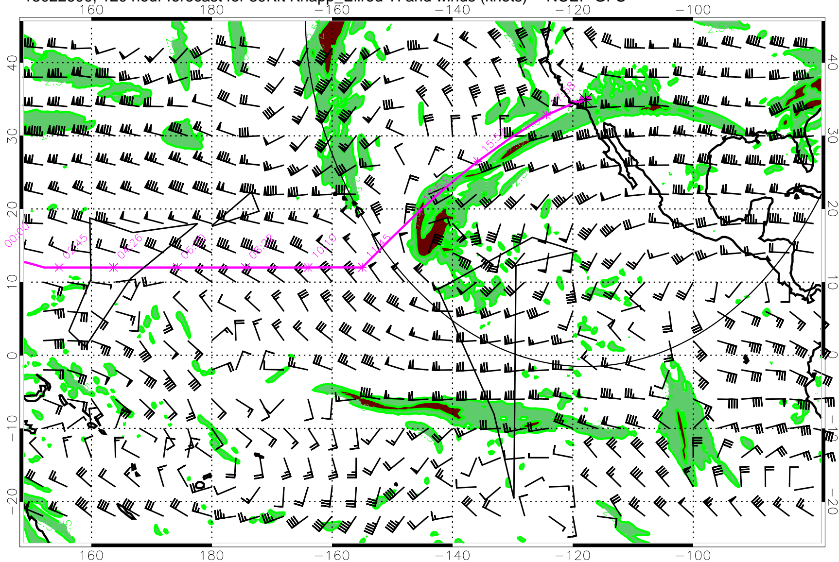
15022600, 120 hour forecast for 39Kft Knapp_Ellrod TI and winds (knots) -- NCEP GFS
