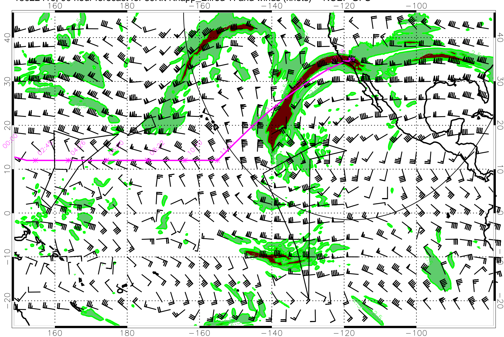
15022418, 90 hour forecast for 39Kft Knapp_Ellrod TI and winds (knots) -- NCEP GFS
