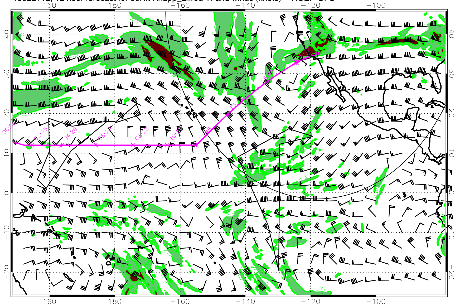
15022112, 12 hour forecast for 39Kft Knapp_Ellrod TI and winds (knots) -- NCEP GFS
