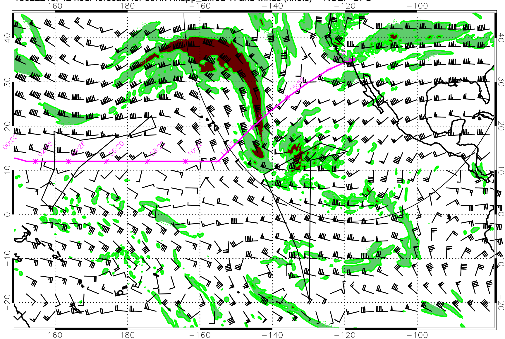
15022218, 42 hour forecast for 39Kft Knapp_Ellrod TI and winds (knots) -- NCEP GFS
