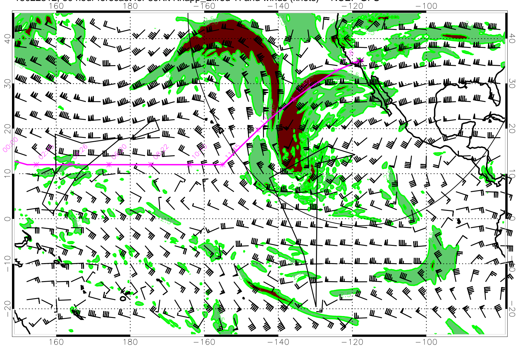
15022312, 60 hour forecast for 39Kft Knapp_Ellrod TI and winds (knots) -- NCEP GFS
