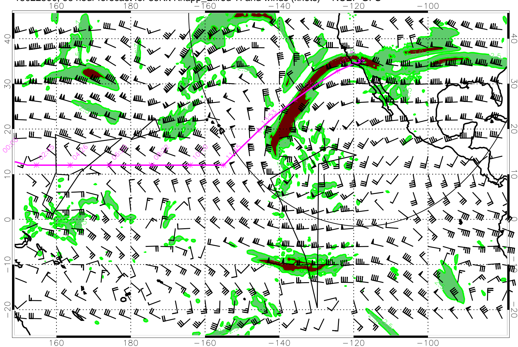
15022500, 96 hour forecast for 39Kft Knapp_Ellrod TI and winds (knots) -- NCEP GFS
