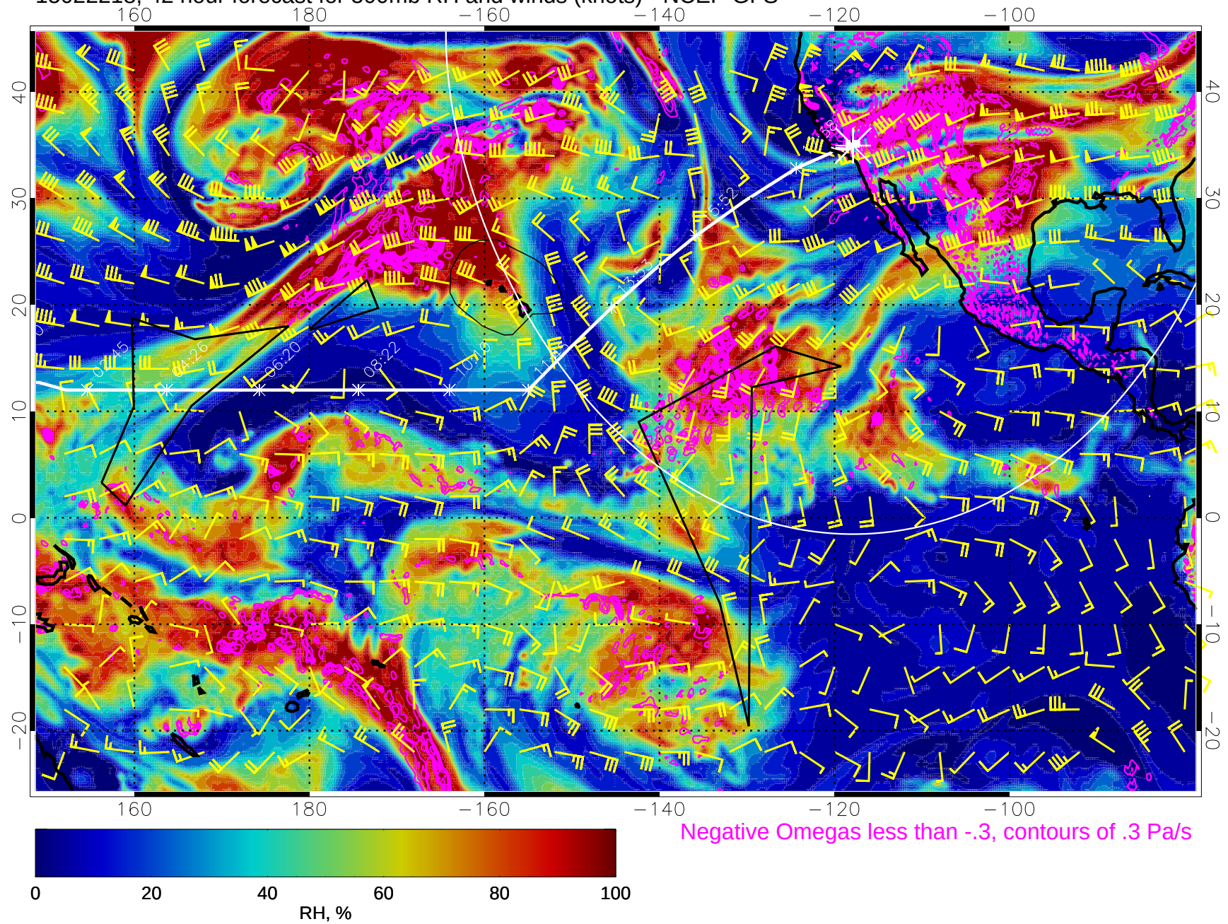
15022218, 42 hour forecast for 500mb RH and winds (knots) - NCEP GFS
