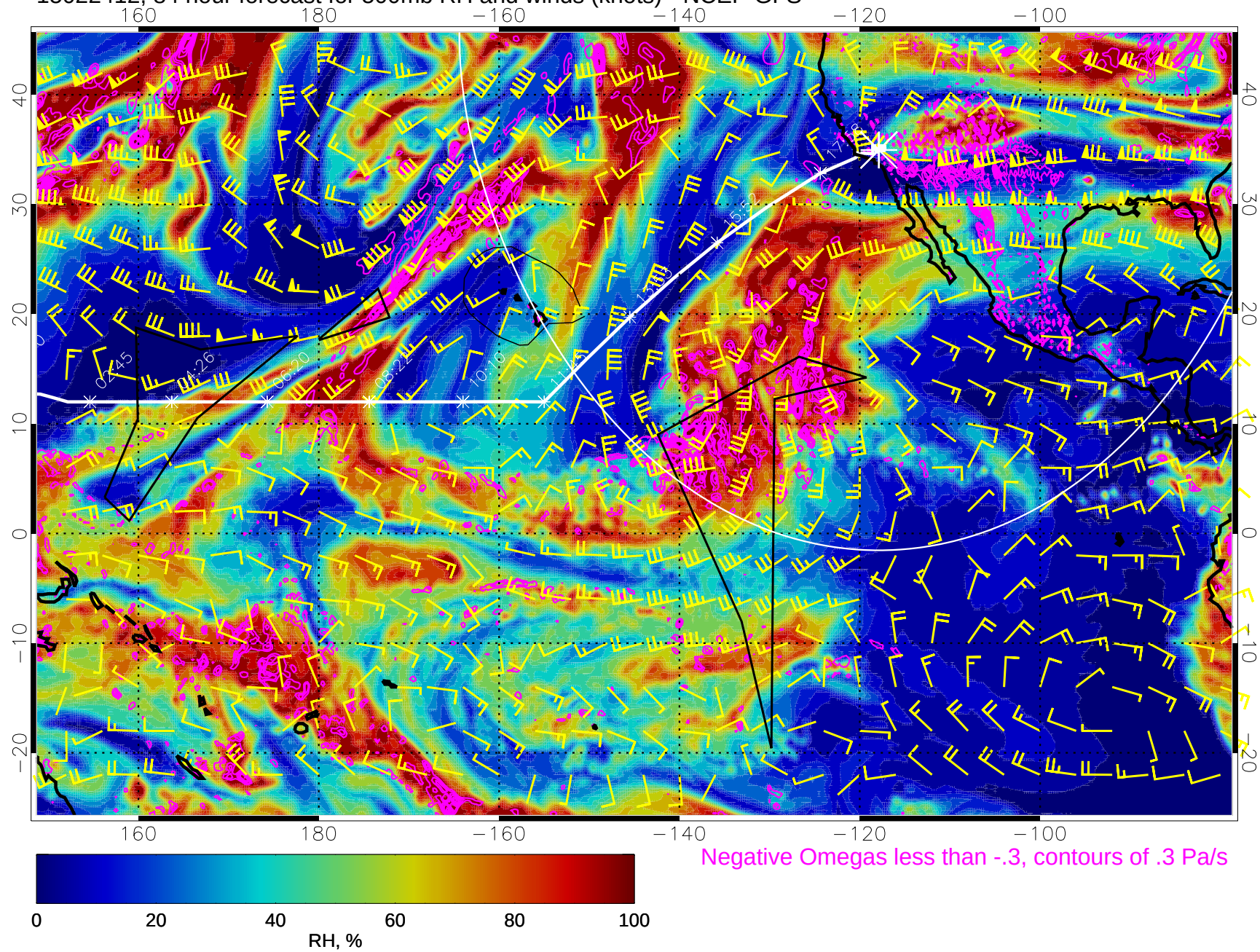
15022412, 84 hour forecast for 500mb RH and winds (knots) - NCEP GFS
