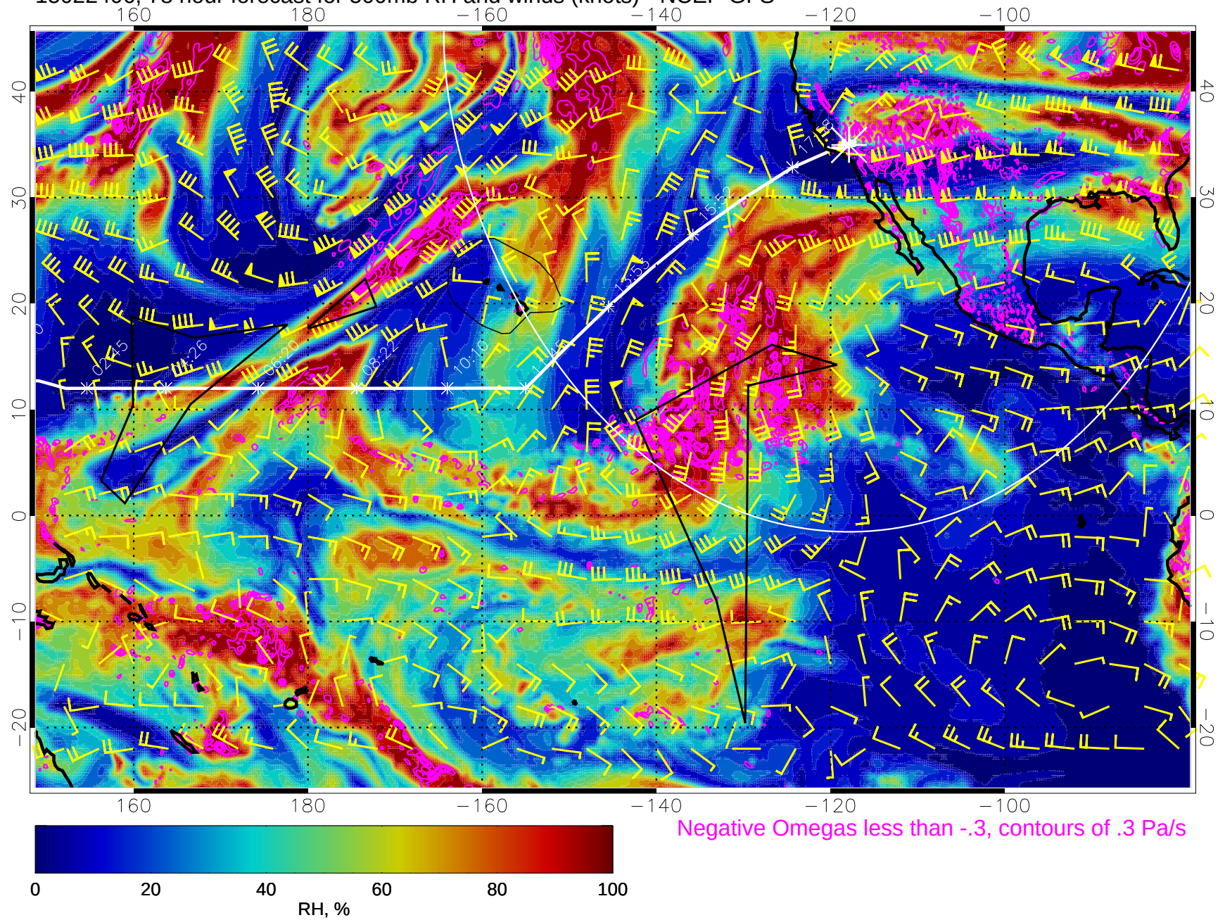
15022406, 78 hour forecast for 500mb RH and winds (knots) - NCEP GFS
