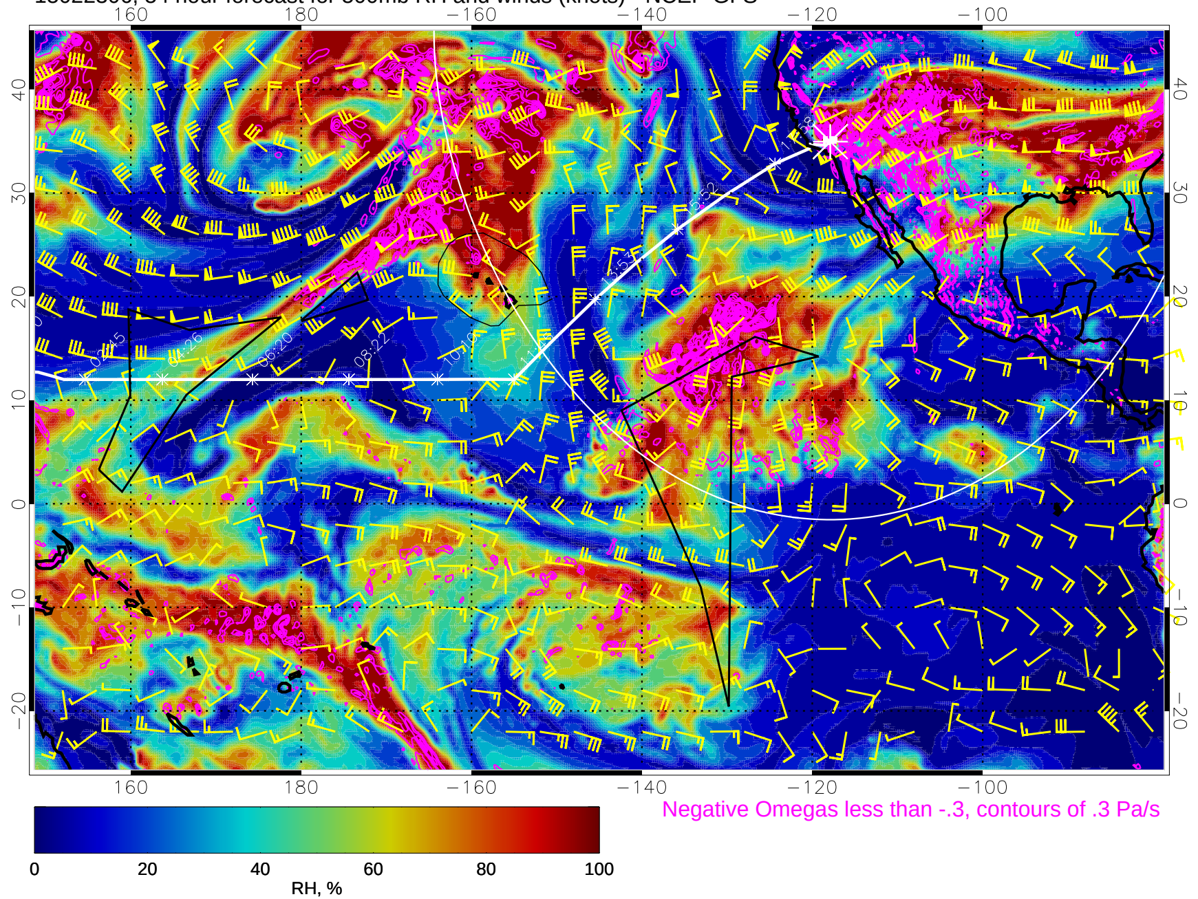
15022306, 54 hour forecast for 500mb RH and winds (knots) - NCEP GFS
