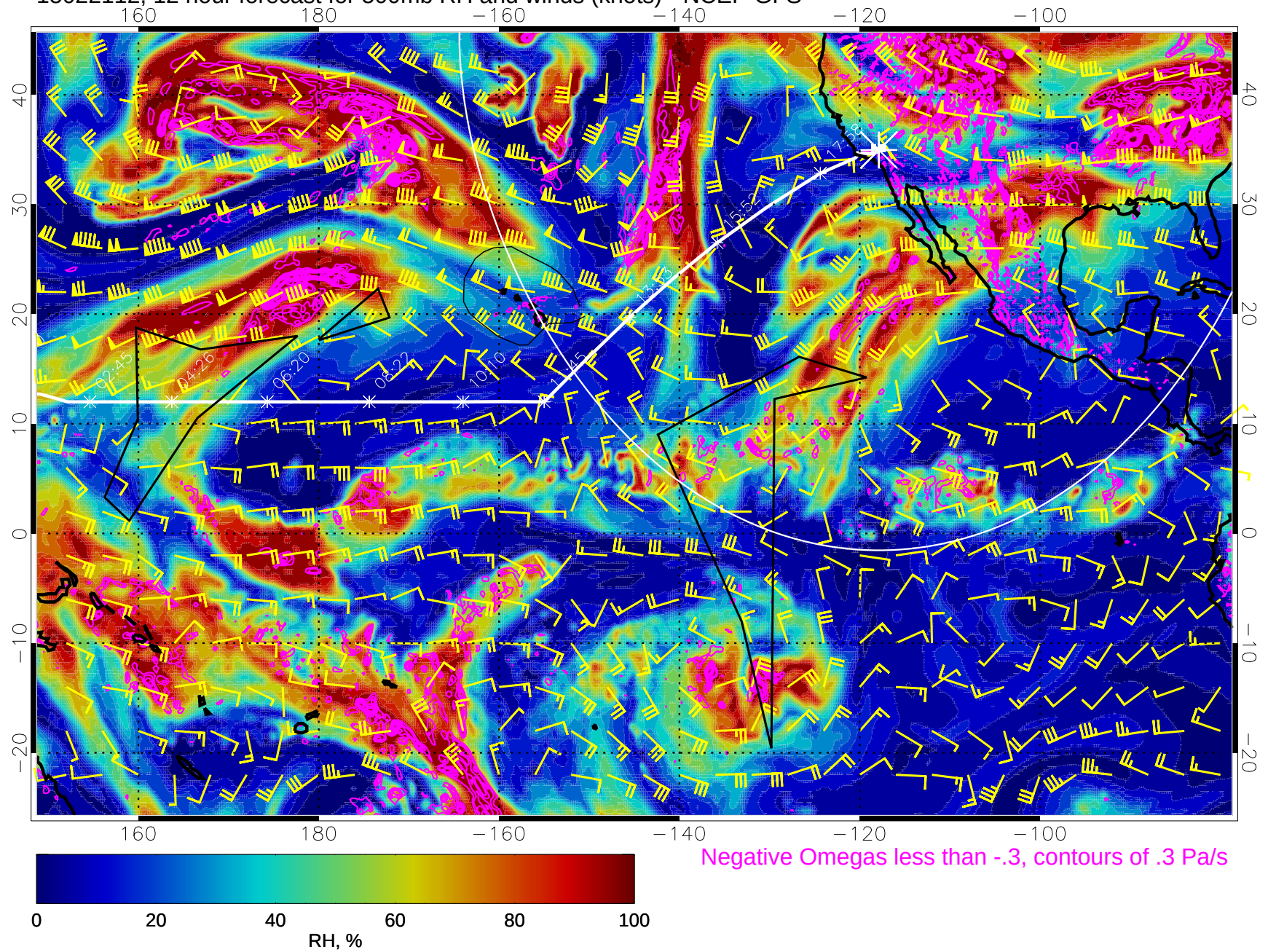
15022112, 12 hour forecast for 500mb RH and winds (knots) - NCEP GFS
