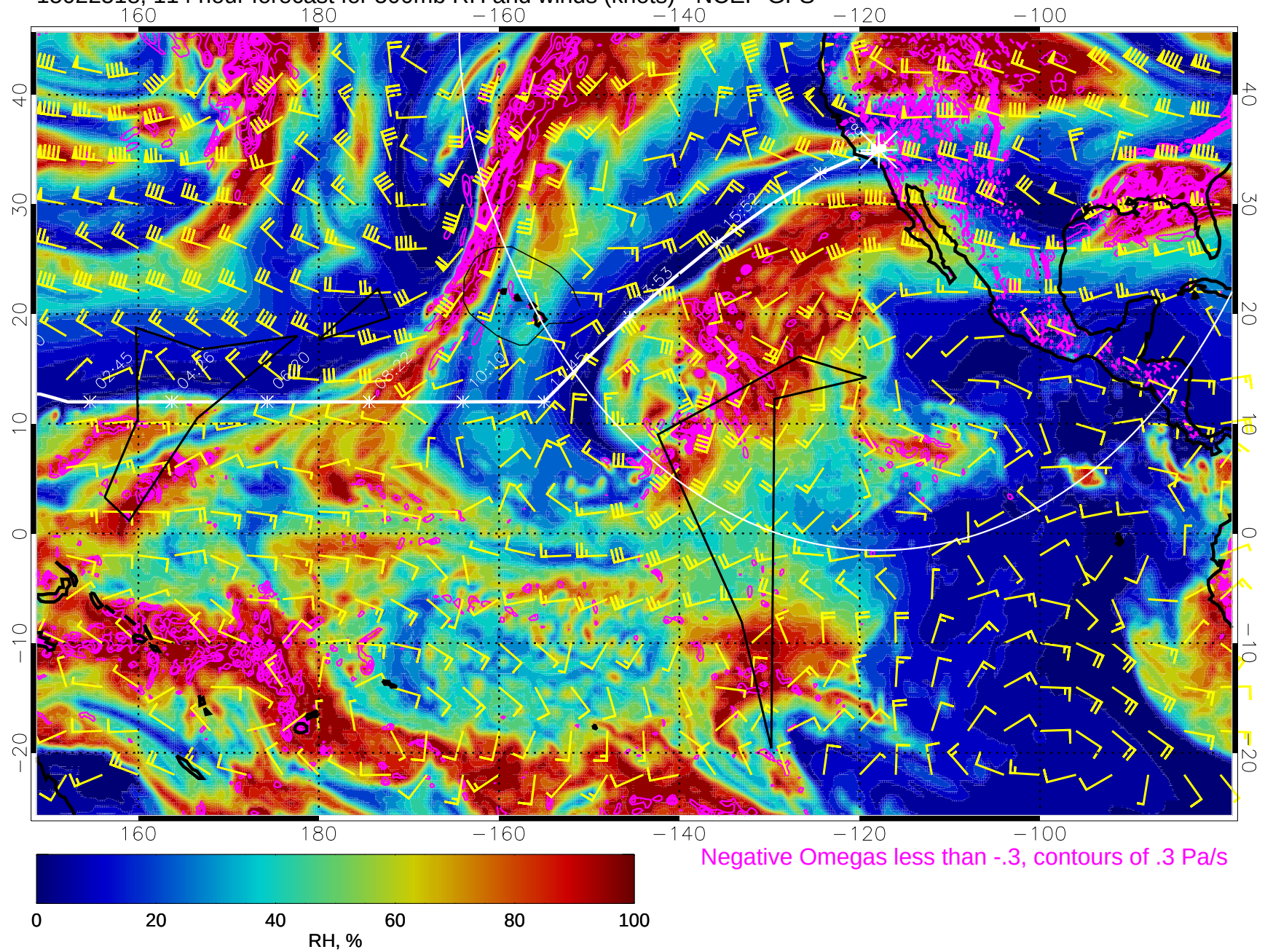
15022518, 114 hour forecast for 500mb RH and winds (knots) - NCEP GFS
