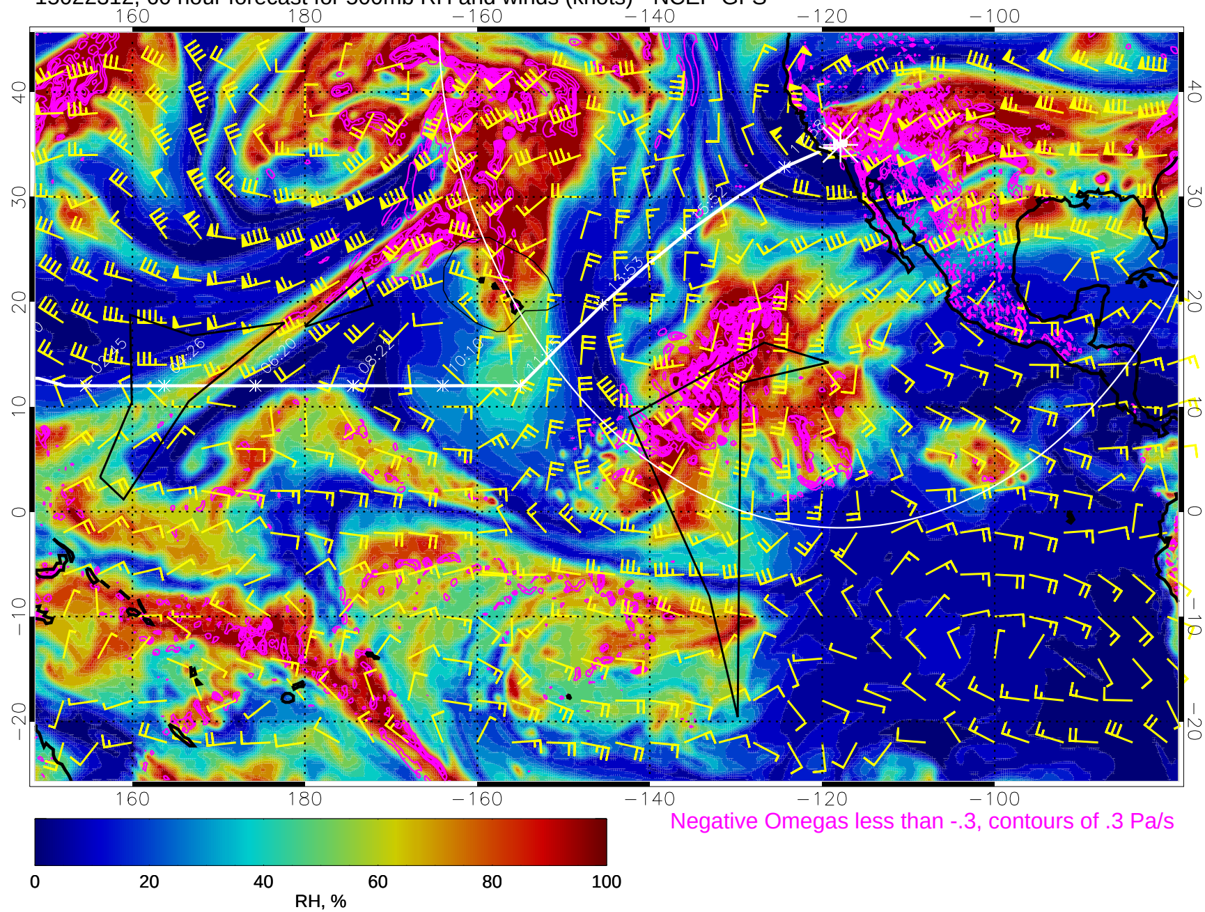
15022312, 60 hour forecast for 500mb RH and winds (knots) - NCEP GFS
