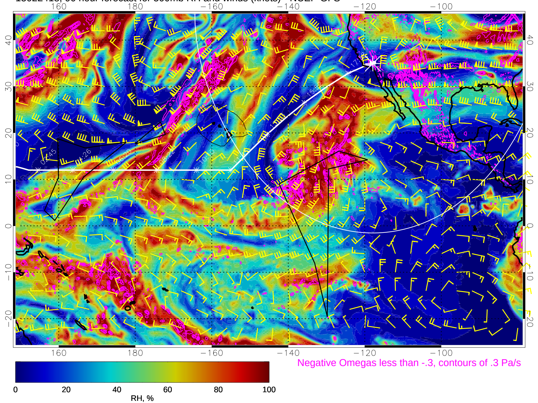
15022418, 90 hour forecast for 500mb RH and winds (knots) - NCEP GFS
