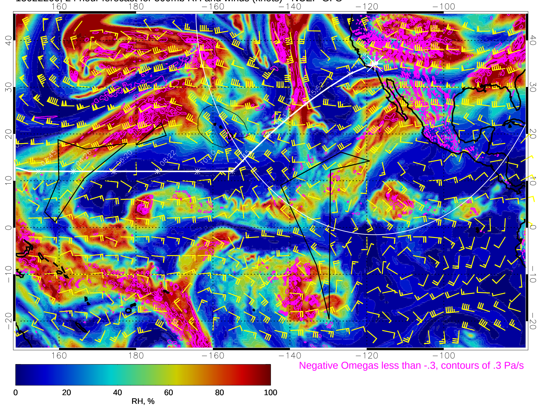
15022200, 24 hour forecast for 500mb RH and winds (knots) - NCEP GFS
