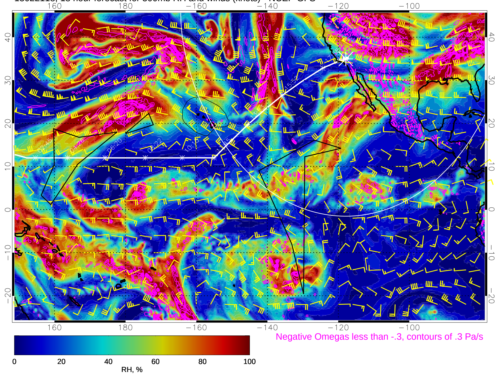
15022118, 18 hour forecast for 500mb RH and winds (knots) - NCEP GFS
