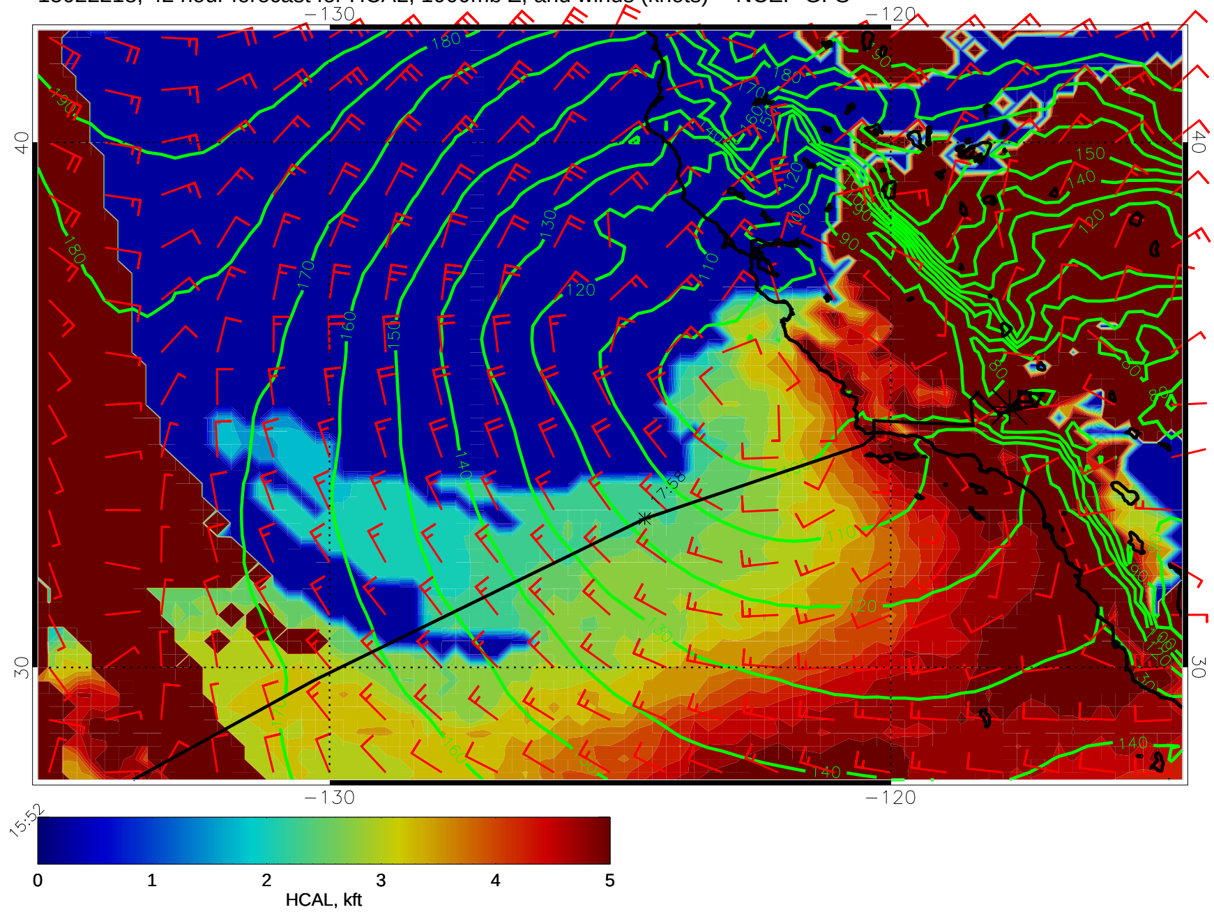
15022218, 42 hour forecast for HCAL, 1000mb Z, and winds (knots) -- NCEP GFS
