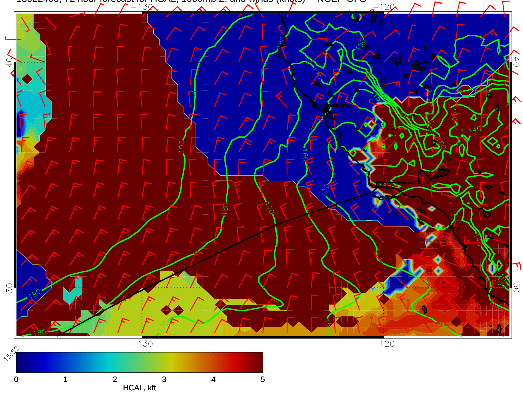
15022400, 72 hour forecast for HCAL, 1000mb Z, and winds (knots) -- NCEP GFS
