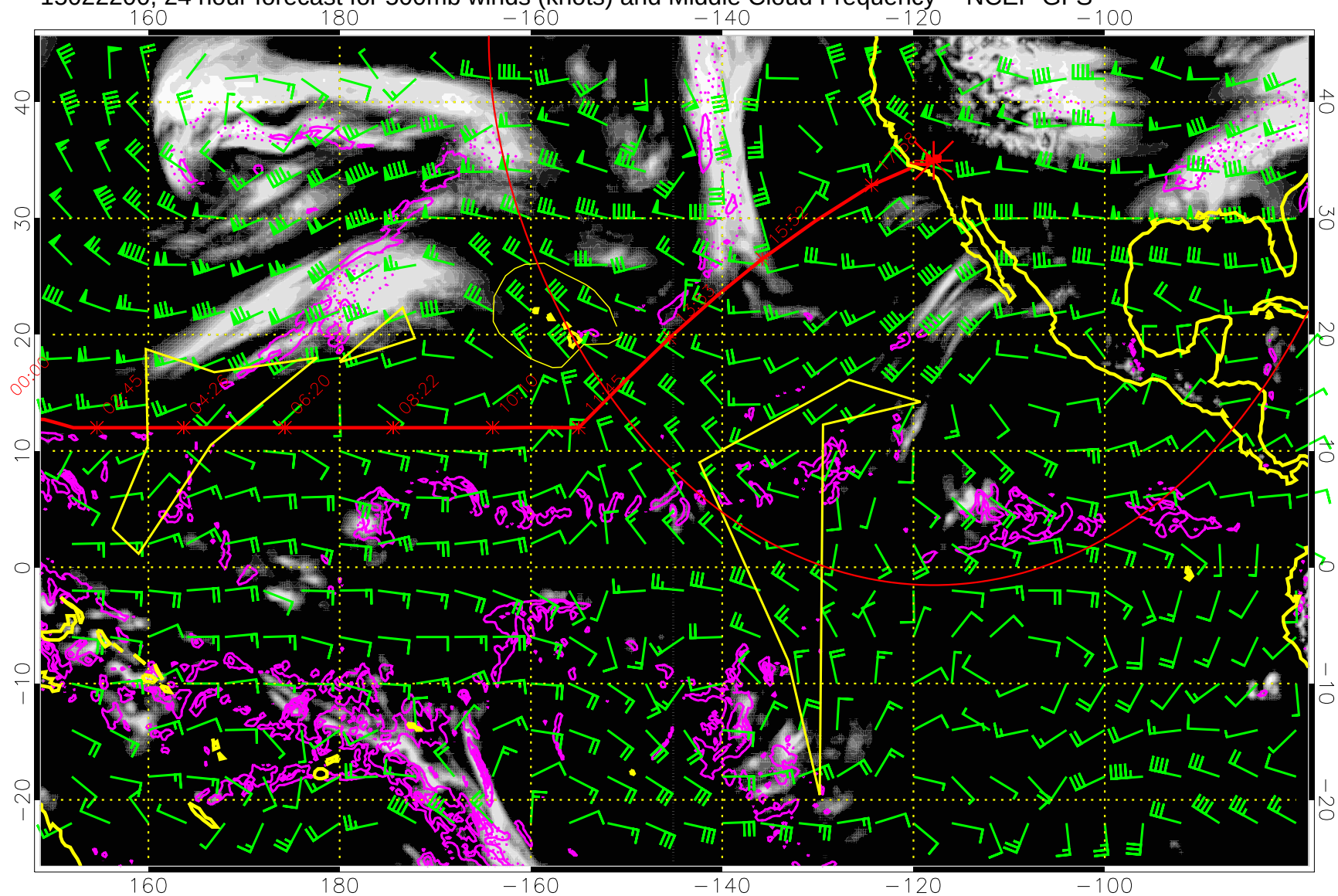
15022200, 24 hour forecast for 500mb winds (knots) and Middle Cloud Frequency -- NCEP GFS
