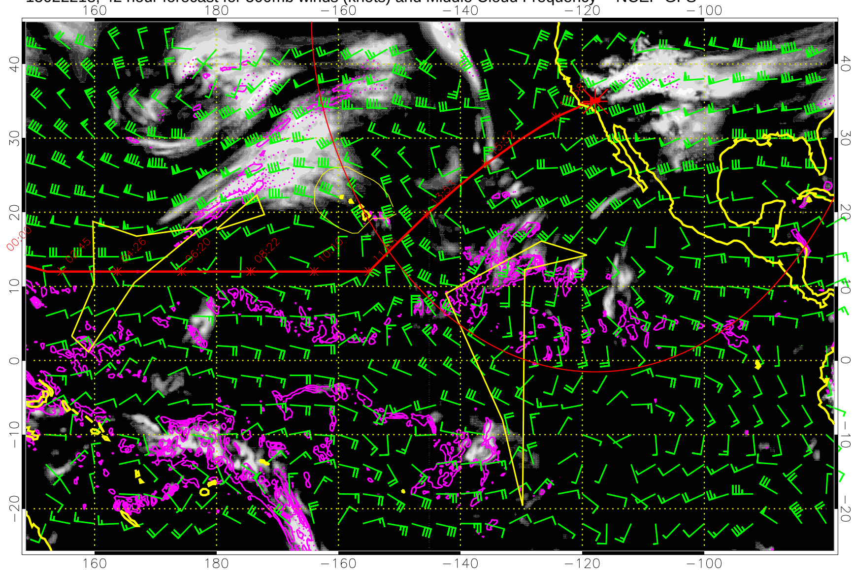
15022218, 42 hour forecast for 500mb winds (knots) and Middle Cloud Frequency -- NCEP GFS
