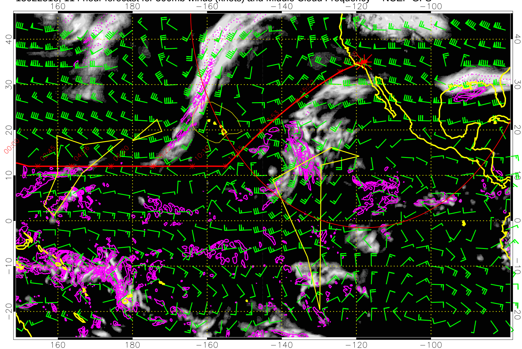
15022518, 114 hour forecast for 500mb winds (knots) and Middle Cloud Frequency -- NCEP GFS
