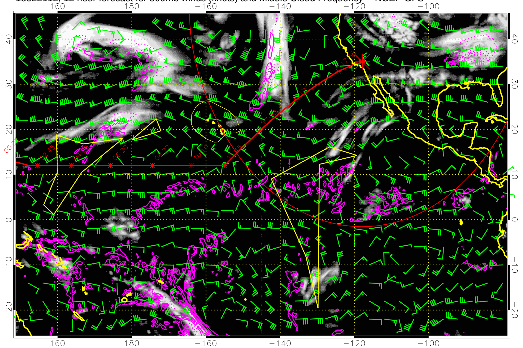
15022112, 12 hour forecast for 500mb winds (knots) and Middle Cloud Frequency -- NCEP GFS
