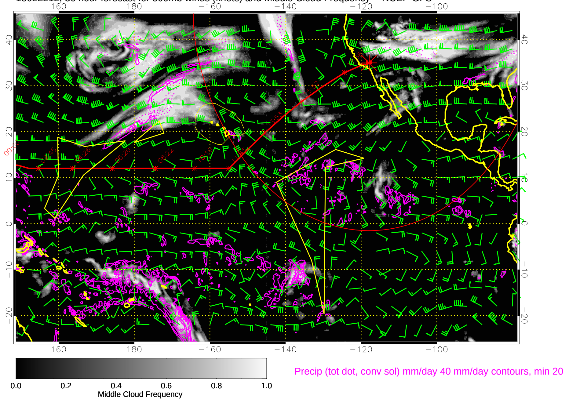
15022212, 36 hour forecast for 500mb winds (knots) and Middle Cloud Frequency -- NCEP GFS
