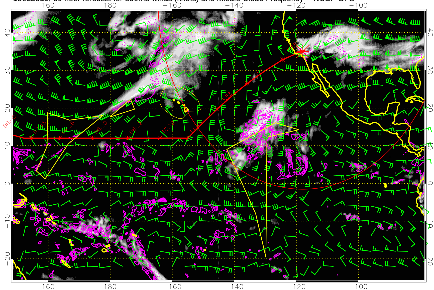
15022312, 60 hour forecast for 500mb winds (knots) and Middle Cloud Frequency -- NCEP GFS
