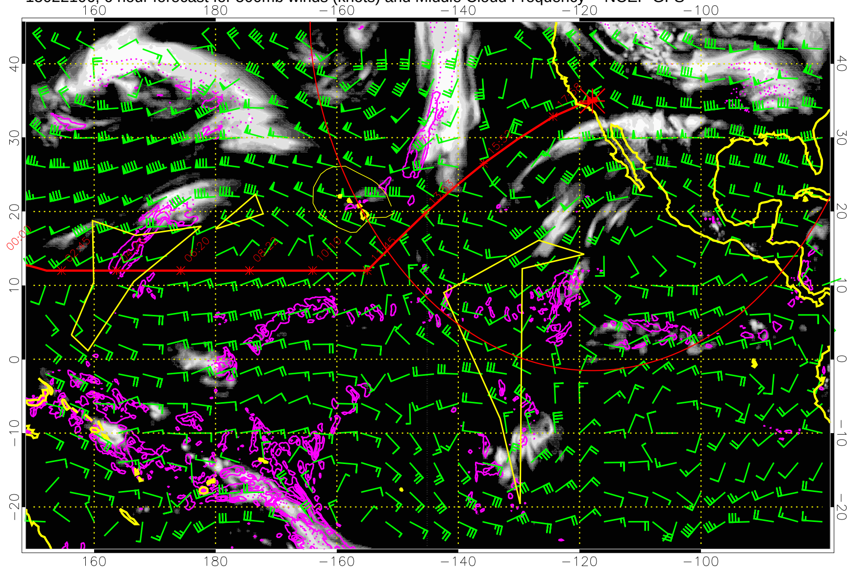
15022106, 6 hour forecast for 500mb winds (knots) and Middle Cloud Frequency -- NCEP GFS
