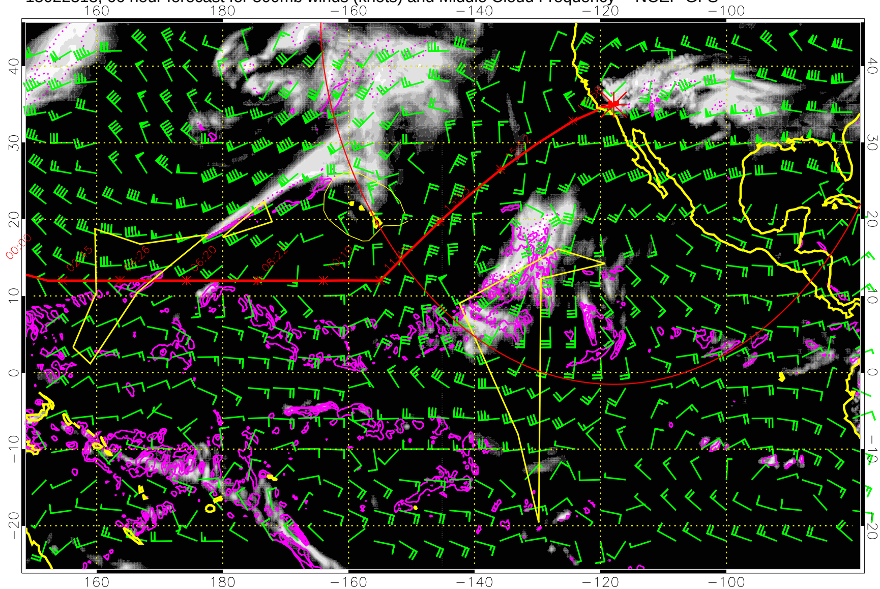
15022318, 66 hour forecast for 500mb winds (knots) and Middle Cloud Frequency -- NCEP GFS
