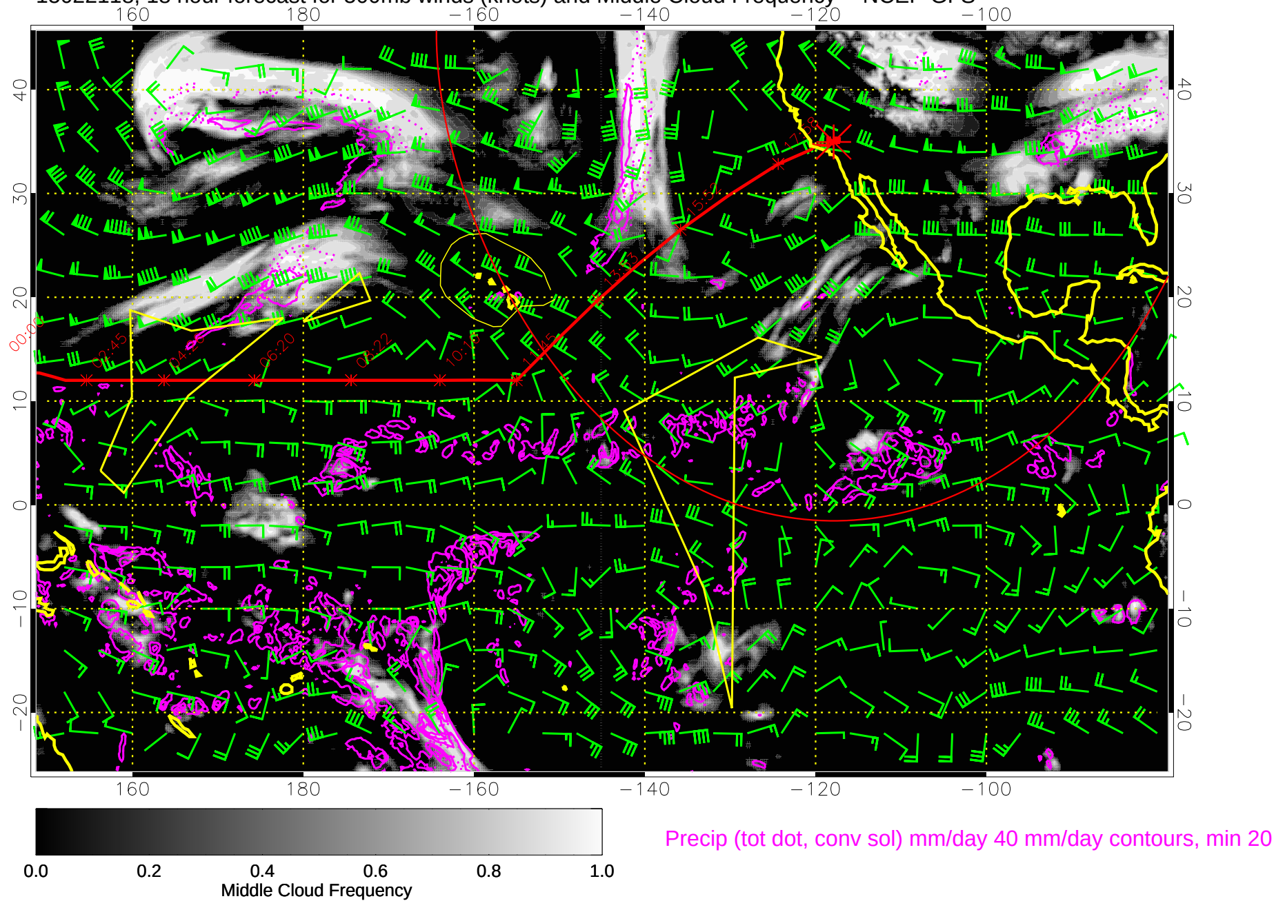
15022118, 18 hour forecast for 500mb winds (knots) and Middle Cloud Frequency -- NCEP GFS
