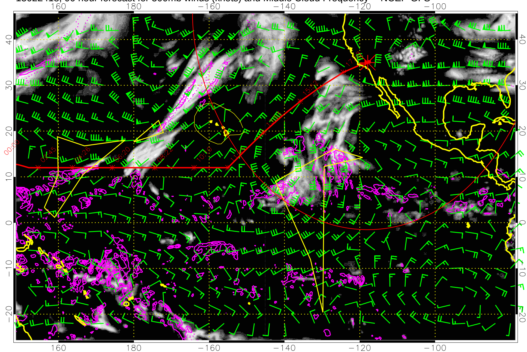
15022418, 90 hour forecast for 500mb winds (knots) and Middle Cloud Frequency -- NCEP GFS
