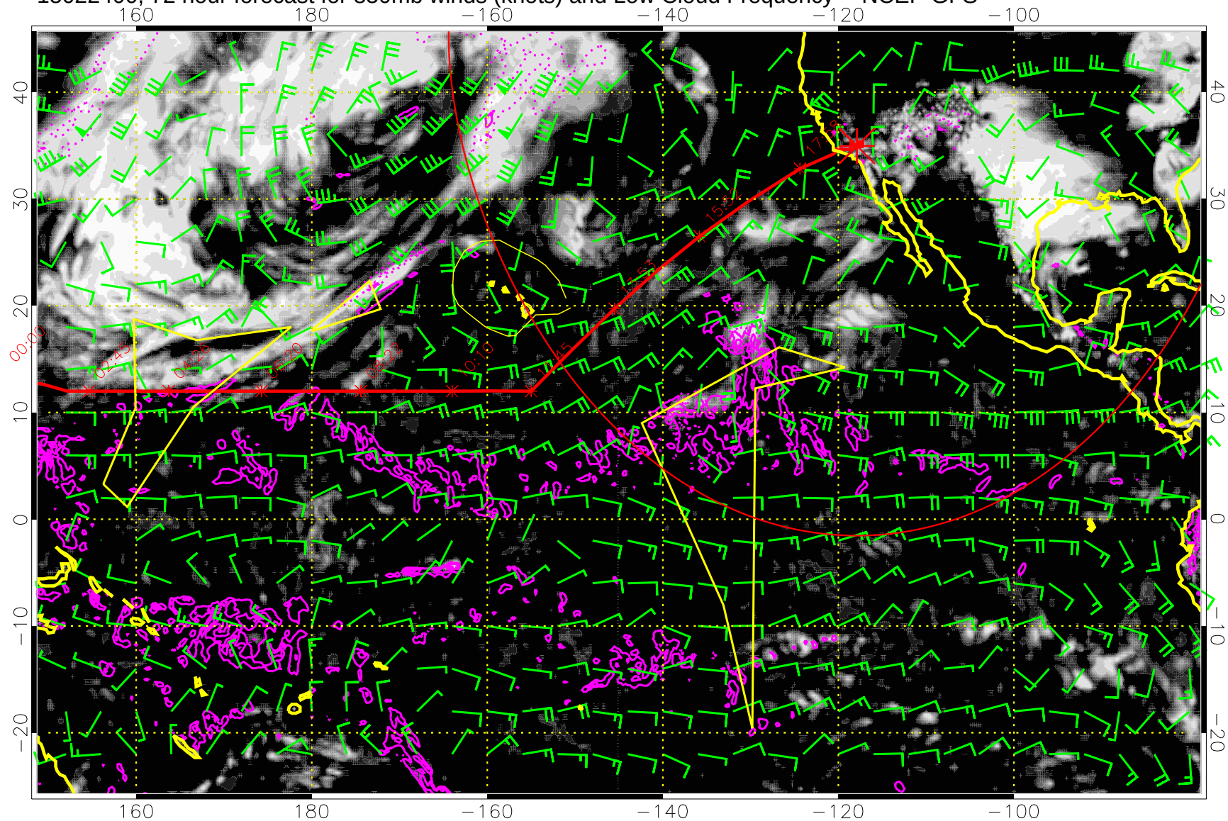
15022400, 72 hour forecast for 850mb winds (knots) and Low Cloud Frequency -- NCEP GFS
