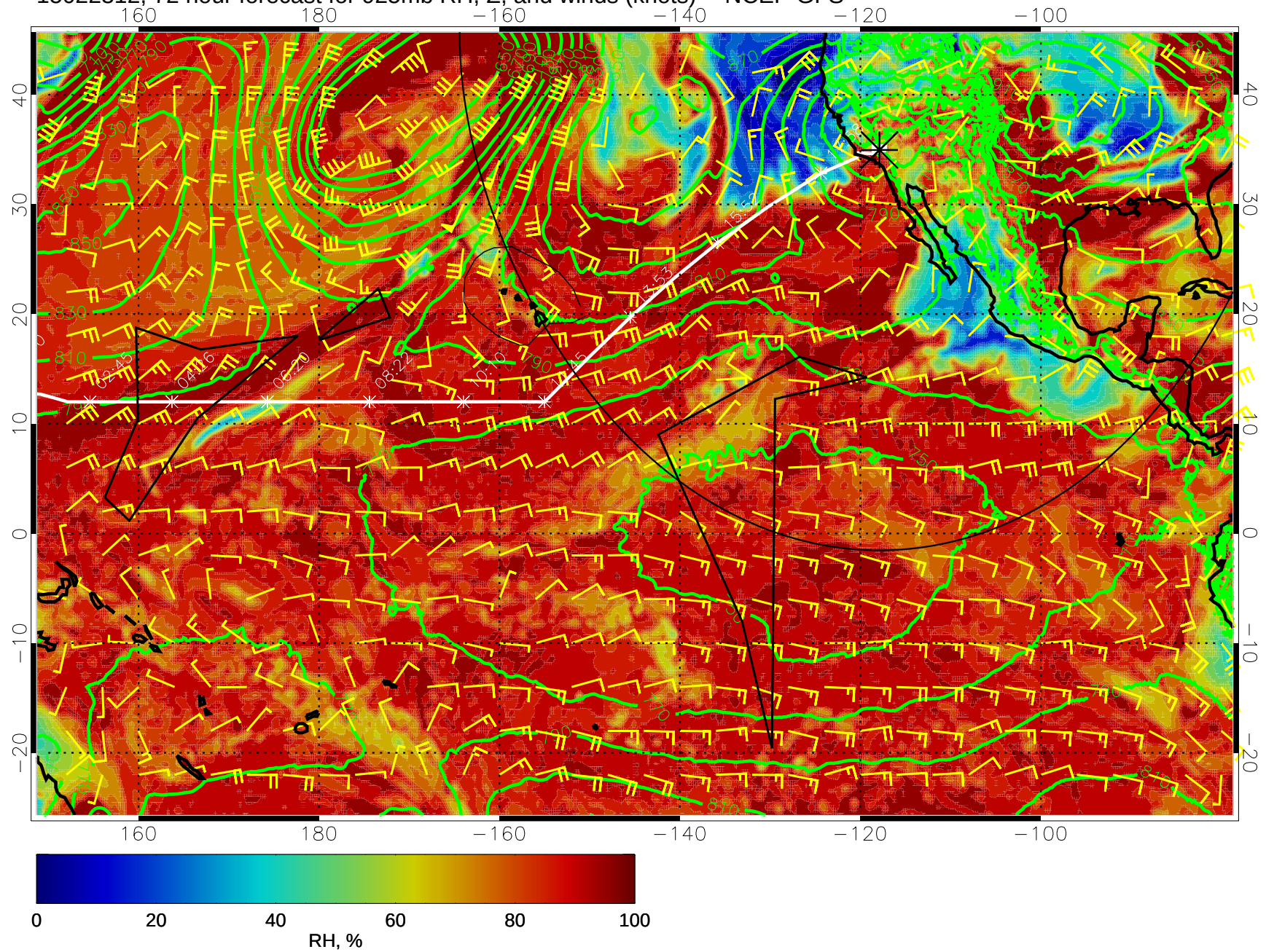
15022312, 72 hour forecast for 925mb RH, Z, and winds (knots) -- NCEP GFS
