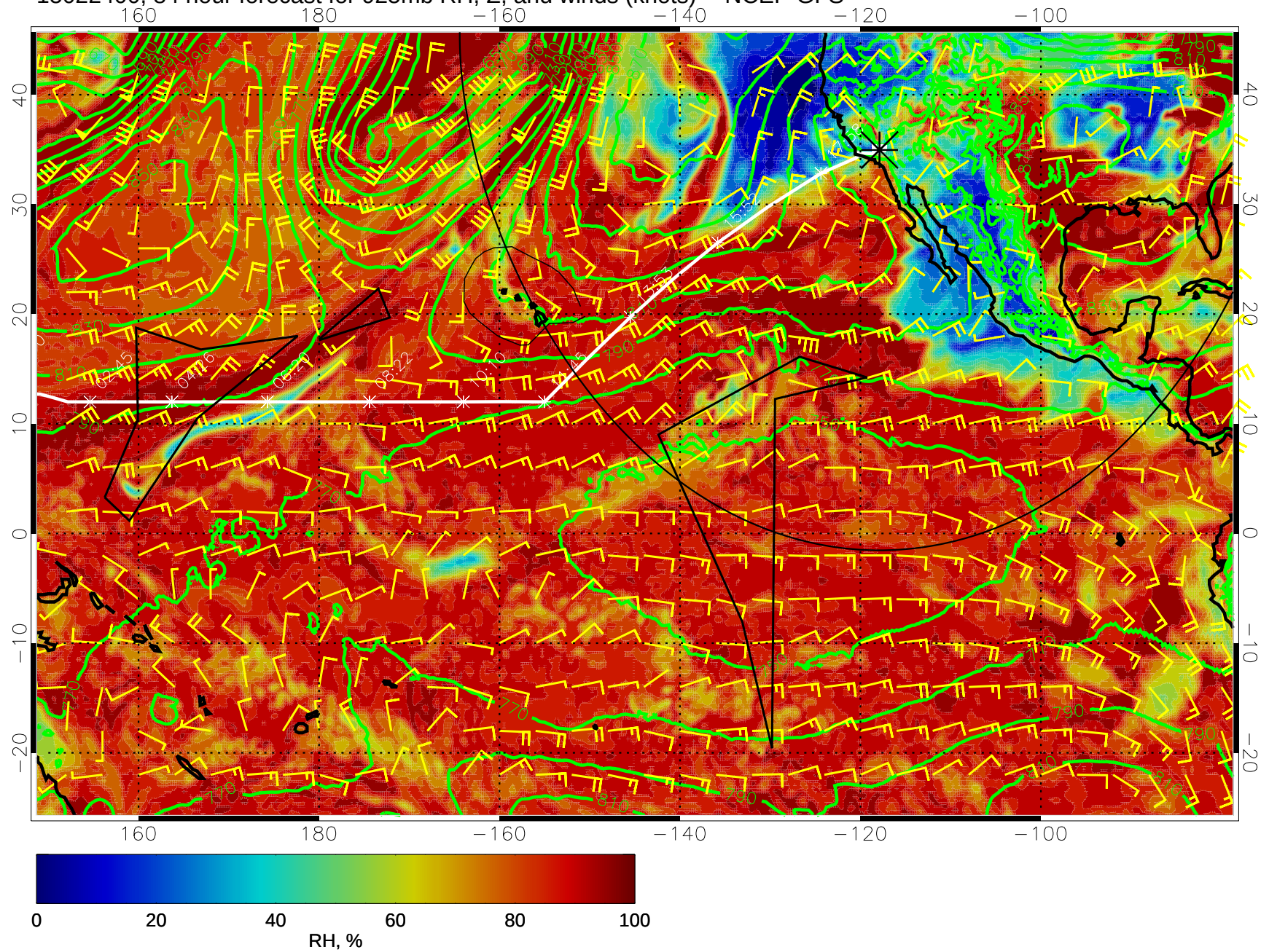
15022400, 84 hour forecast for 925mb RH, Z, and winds (knots) -- NCEP GFS
