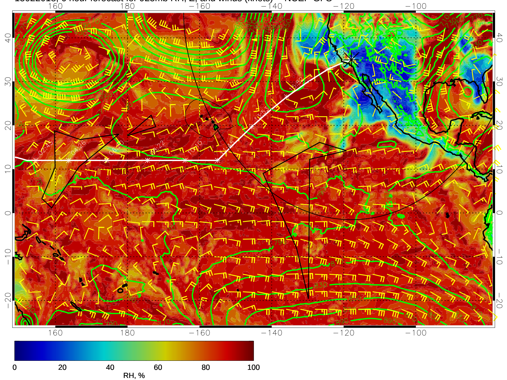
15022018, 6 hour forecast for 925mb RH, Z, and winds (knots) -- NCEP GFS
