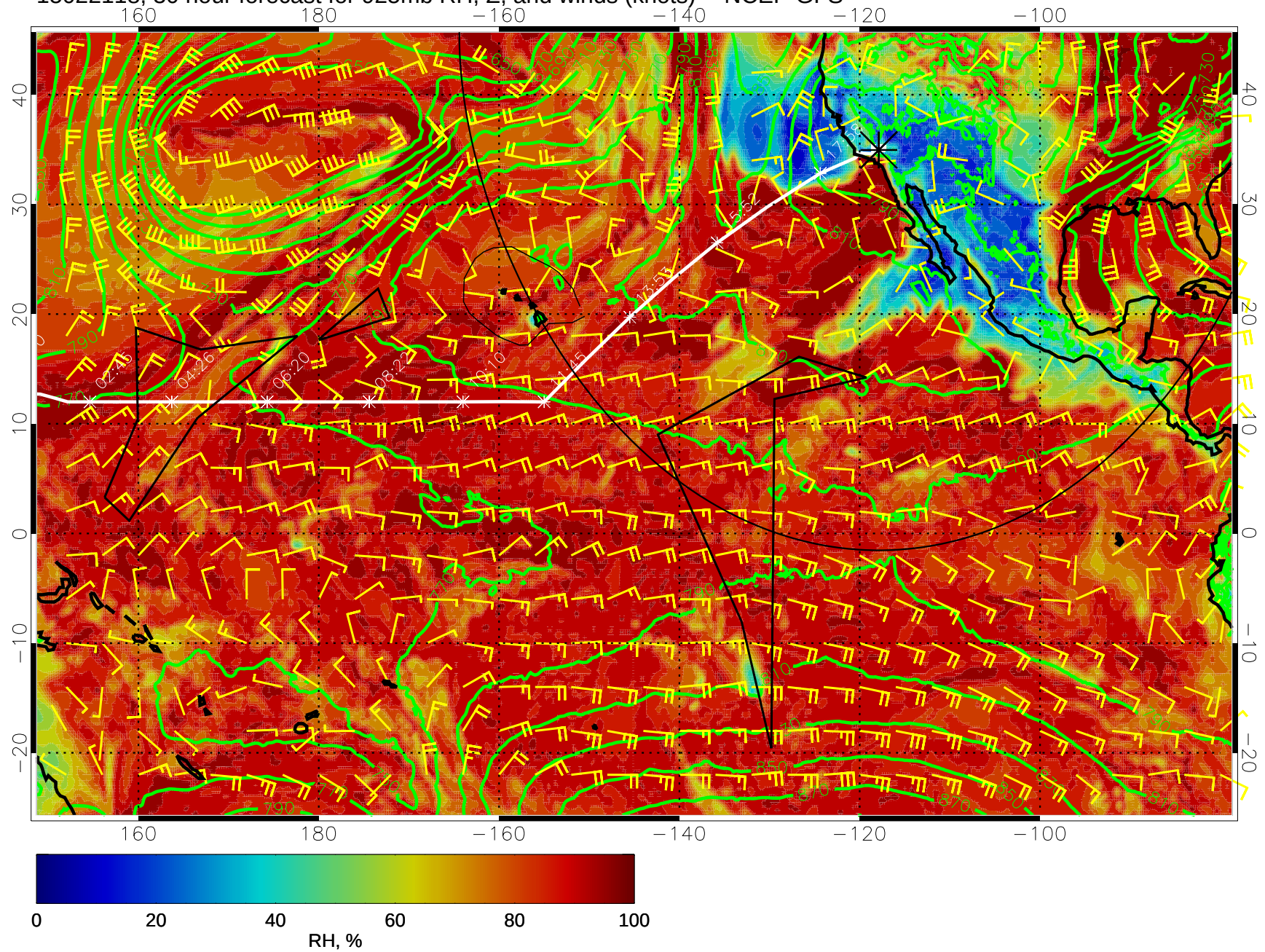
15022118, 30 hour forecast for 925mb RH, Z, and winds (knots) -- NCEP GFS
