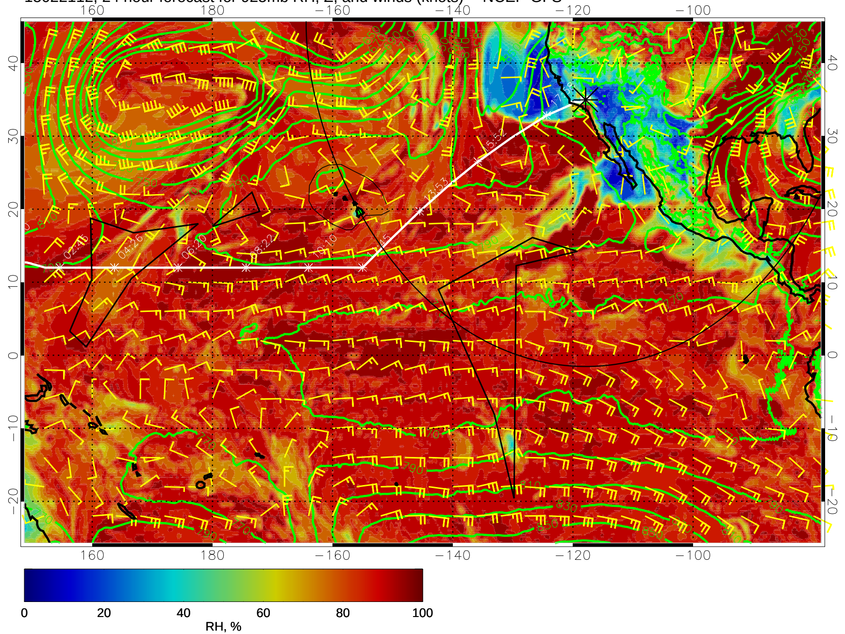
15022112, 24 hour forecast for 925mb RH, Z, and winds (knots) -- NCEP GFS
