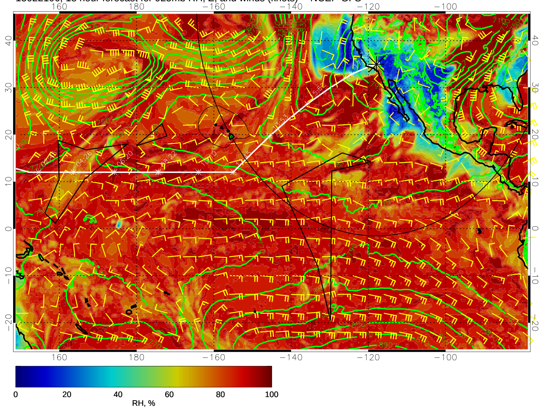
15022106, 18 hour forecast for 925mb RH, Z, and winds (knots) -- NCEP GFS
