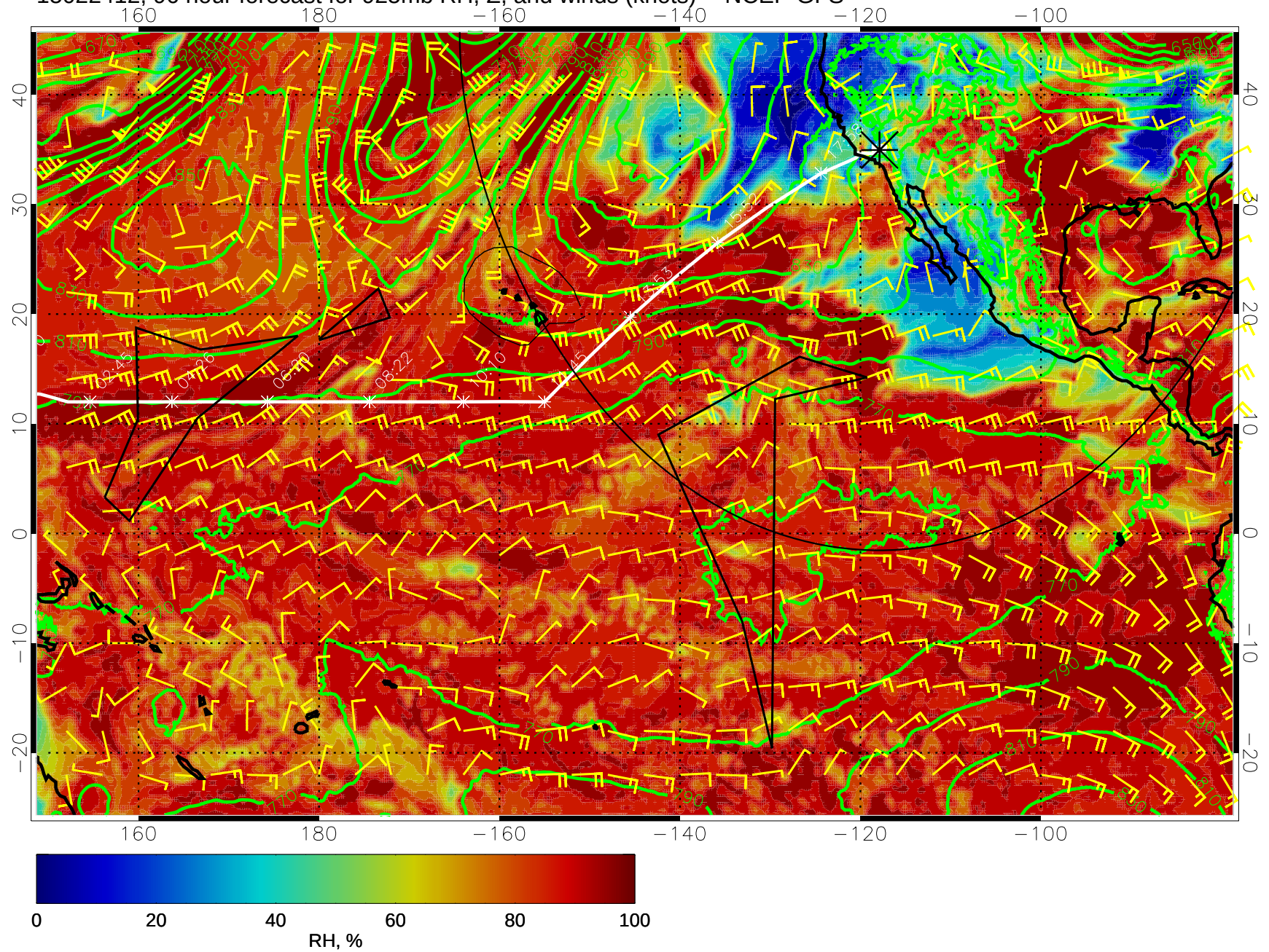
15022412, 96 hour forecast for 925mb RH, Z, and winds (knots) -- NCEP GFS
