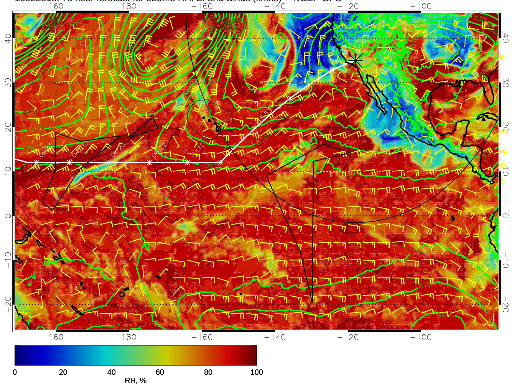
15022318, 78 hour forecast for 925mb RH, Z, and winds (knots) -- NCEP GFS
