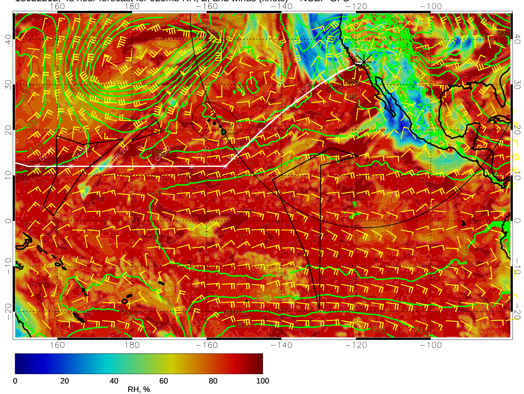
15022212, 48 hour forecast for 925mb RH, Z, and winds (knots) -- NCEP GFS
