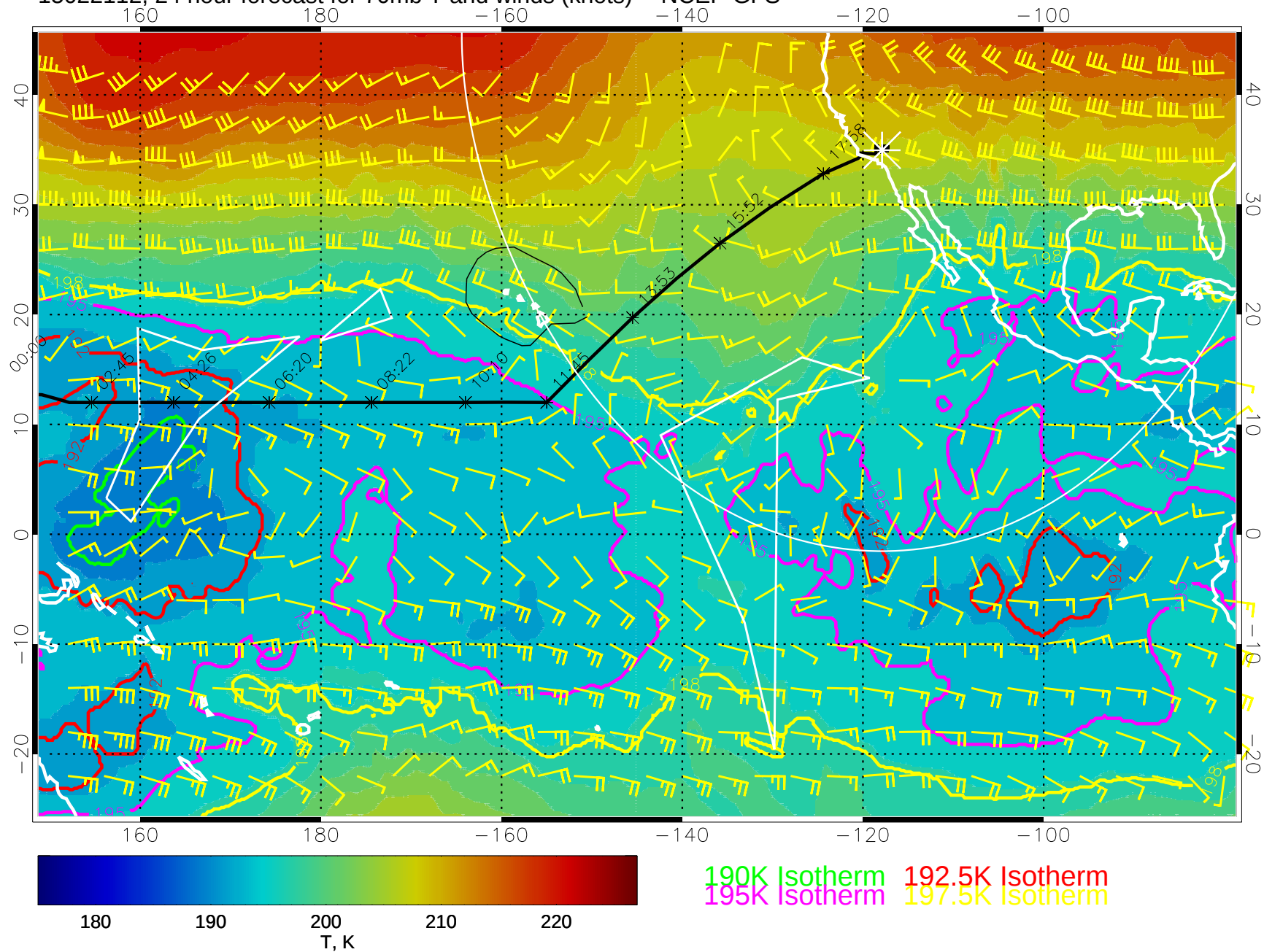
15022112, 24 hour forecast for 70mb T and winds (knots) -- NCEP GFS
