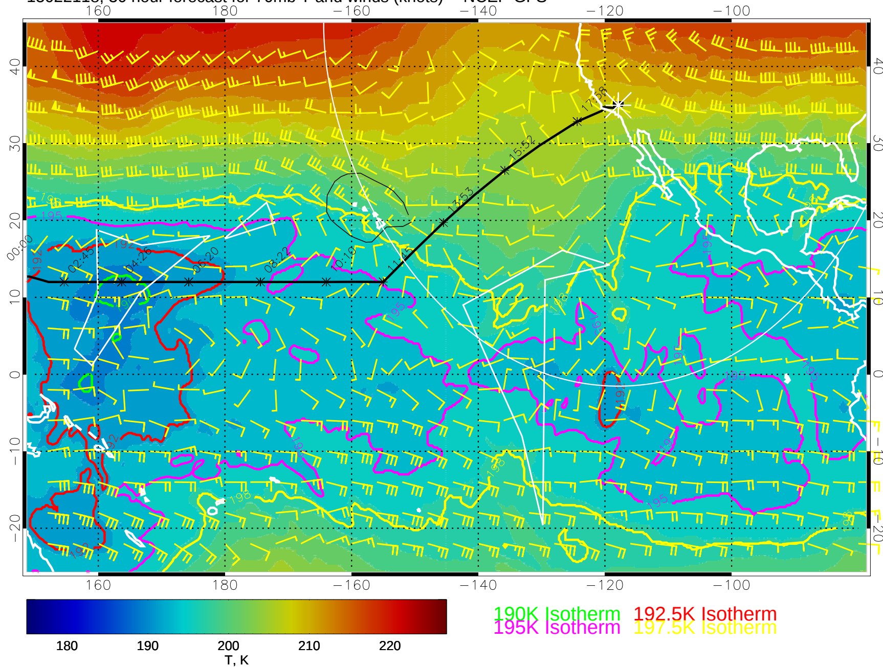
15022118, 30 hour forecast for 70mb T and winds (knots) -- NCEP GFS
