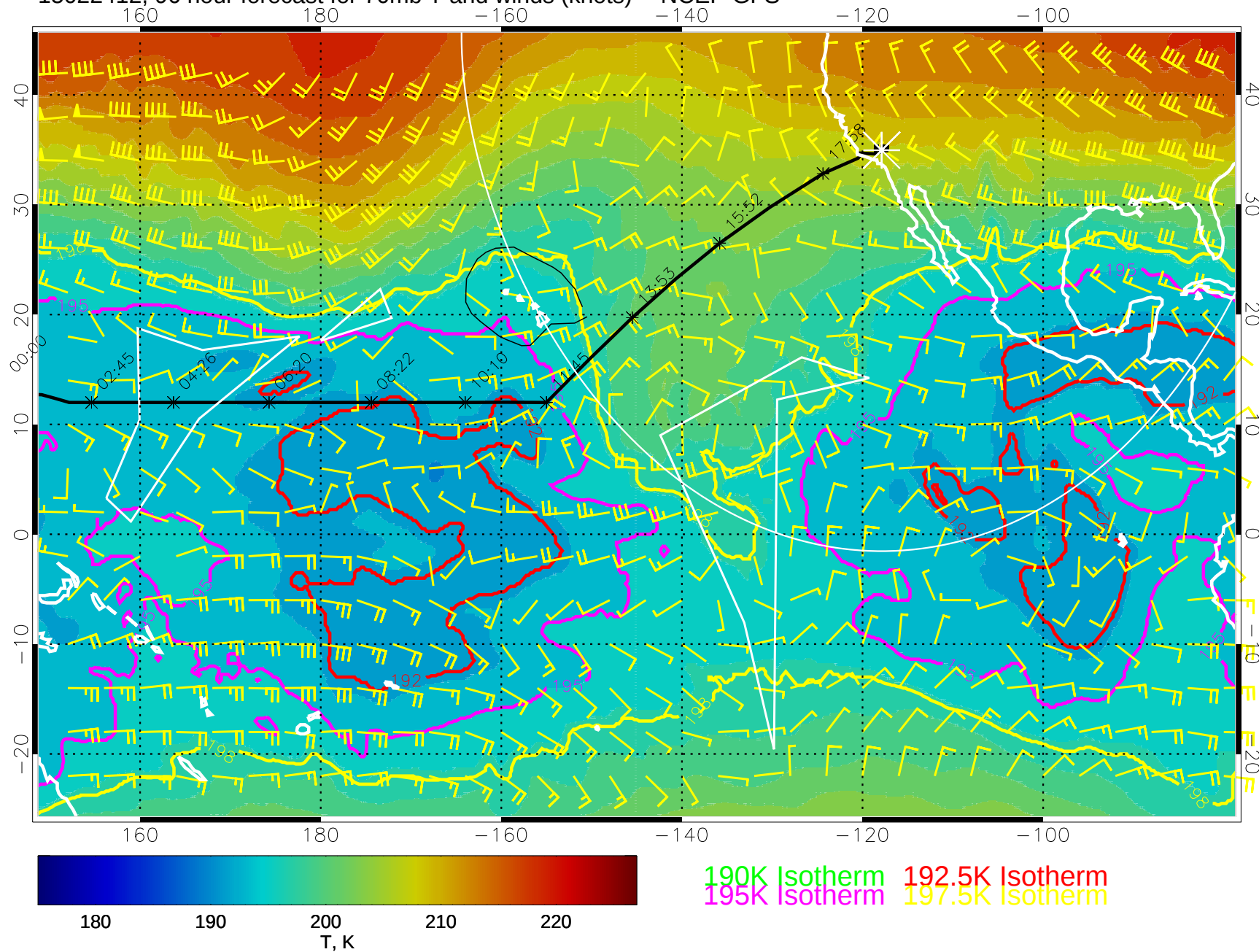
15022412, 96 hour forecast for 70mb T and winds (knots) -- NCEP GFS
