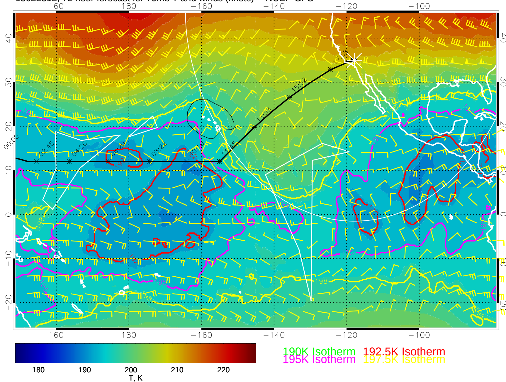
15022312, 72 hour forecast for 70mb T and winds (knots) -- NCEP GFS
