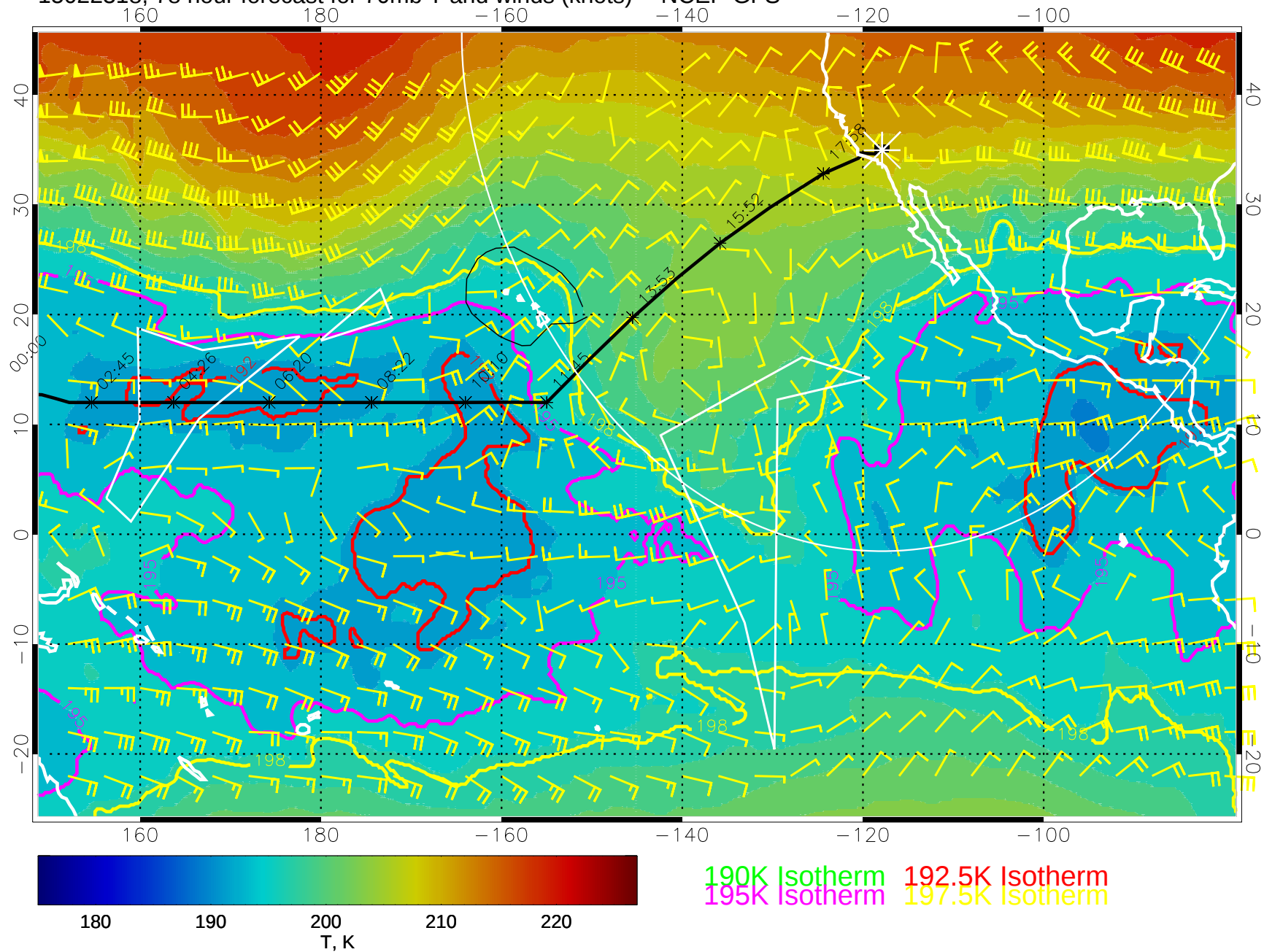
15022318, 78 hour forecast for 70mb T and winds (knots) -- NCEP GFS
