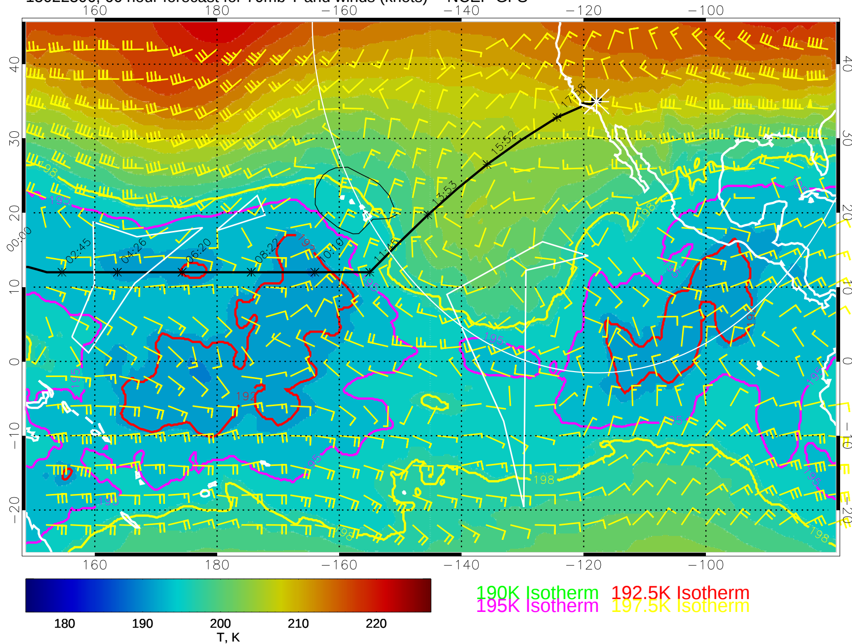
15022306, 66 hour forecast for 70mb T and winds (knots) -- NCEP GFS
