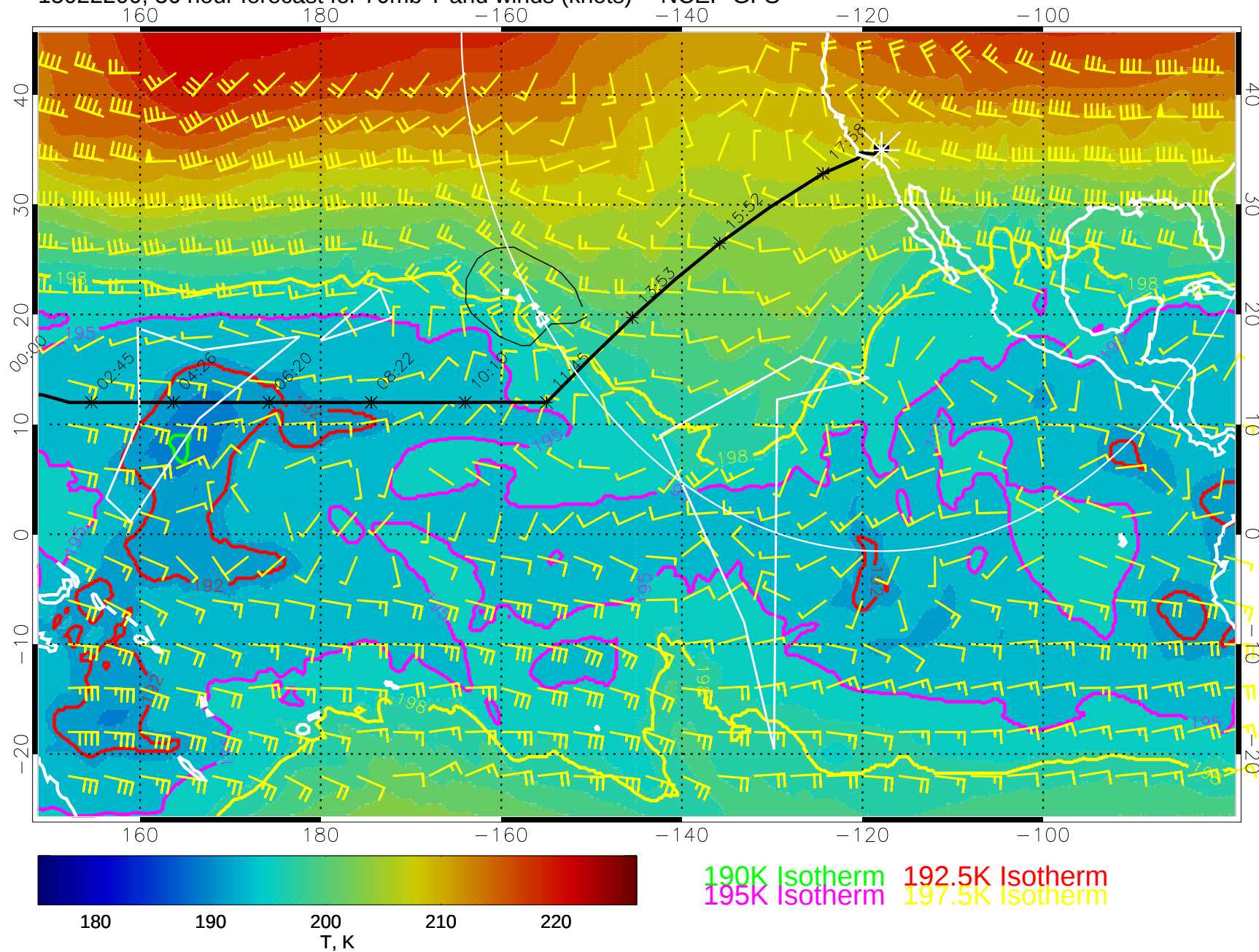
15022200, 36 hour forecast for 70mb T and winds (knots) -- NCEP GFS
