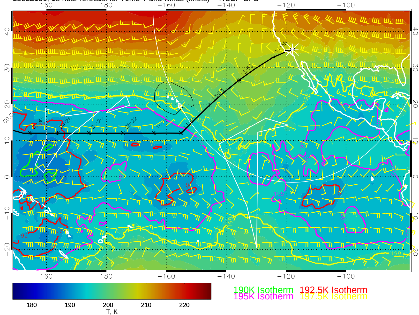
15022106, 18 hour forecast for 70mb T and winds (knots) -- NCEP GFS
