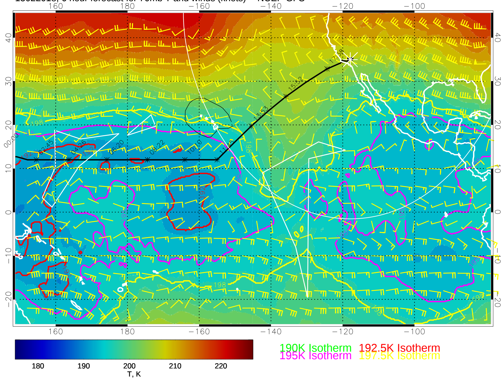
15022018, 6 hour forecast for 70mb T and winds (knots) -- NCEP GFS
