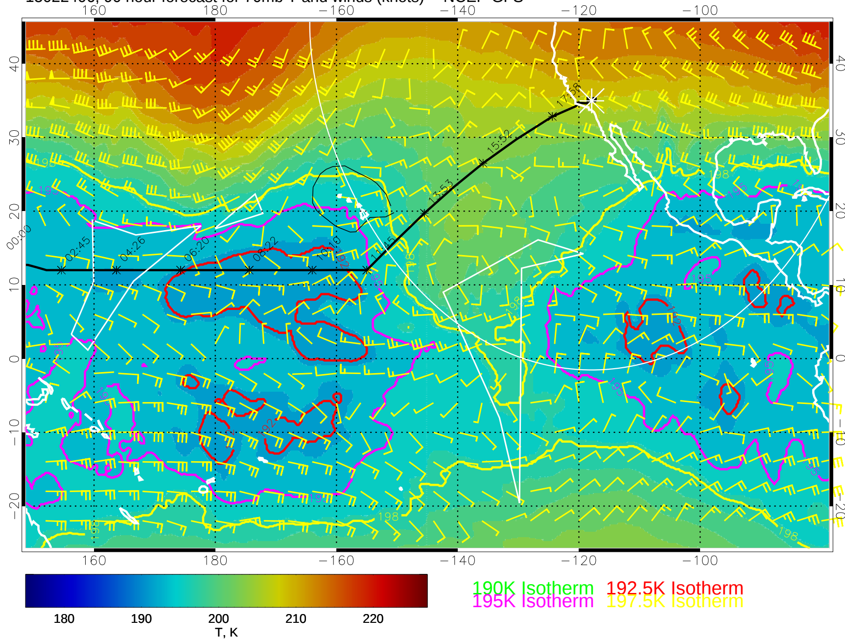
15022406, 90 hour forecast for 70mb T and winds (knots) -- NCEP GFS
