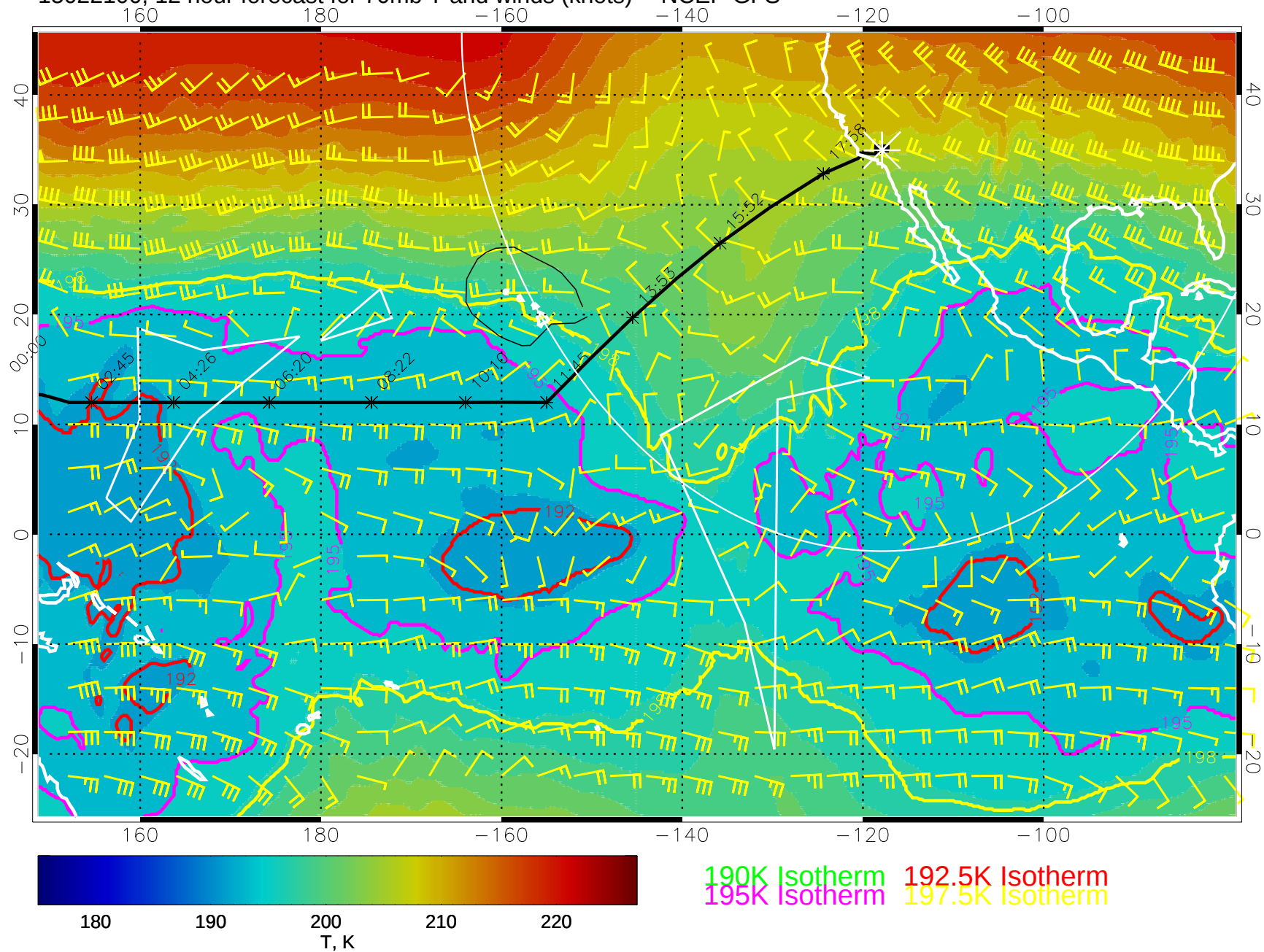
15022100, 12 hour forecast for 70mb T and winds (knots) -- NCEP GFS
