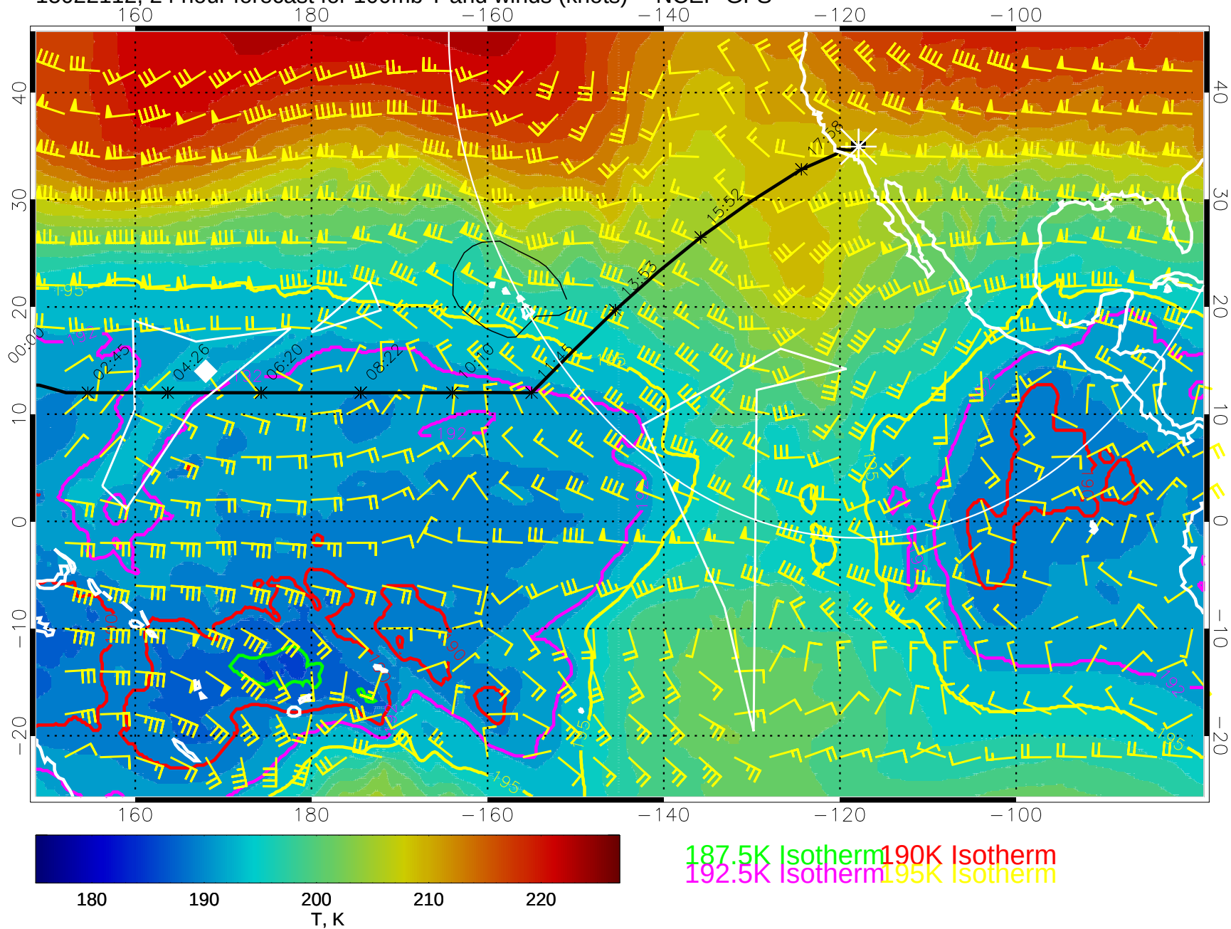
15022112, 24 hour forecast for 100mb T and winds (knots) -- NCEP GFS
