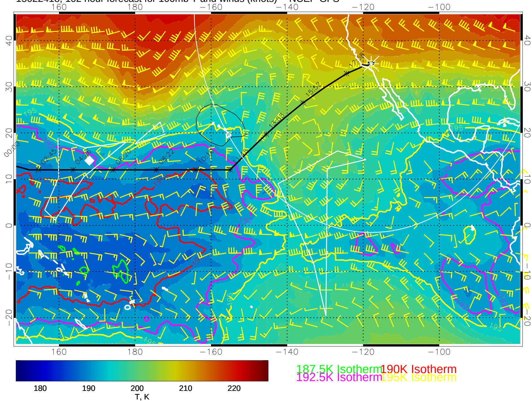
15022418, 102 hour forecast for 100mb T and winds (knots) -- NCEP GFS
