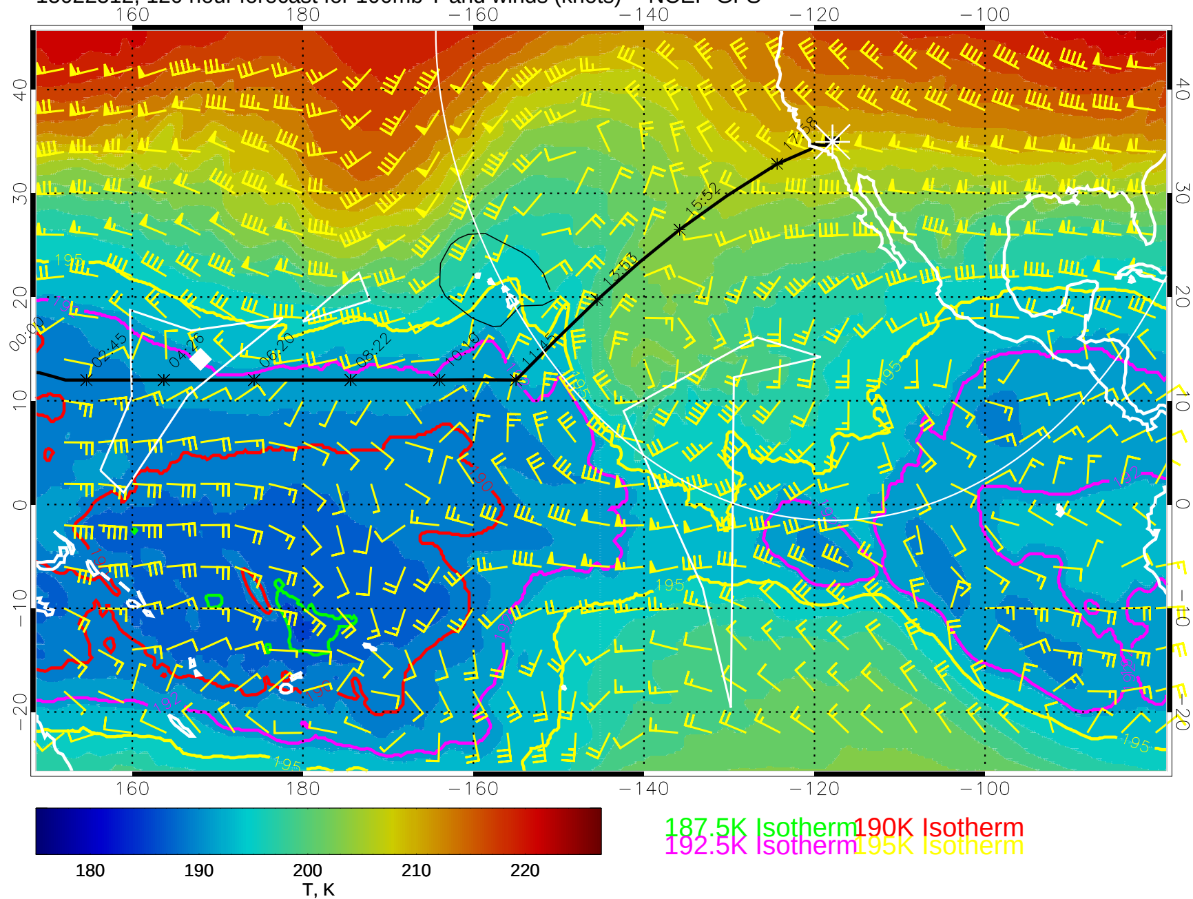
15022512, 120 hour forecast for 100mb T and winds (knots) -- NCEP GFS
