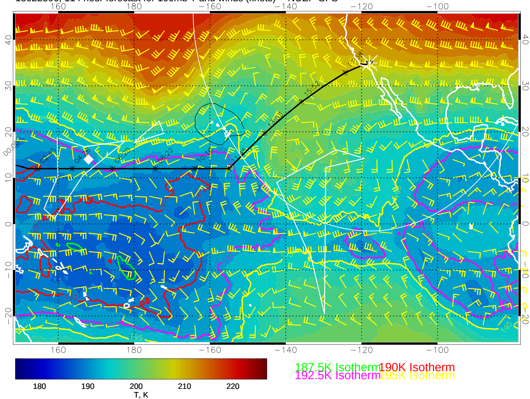
15022506, 114 hour forecast for 100mb T and winds (knots) -- NCEP GFS
