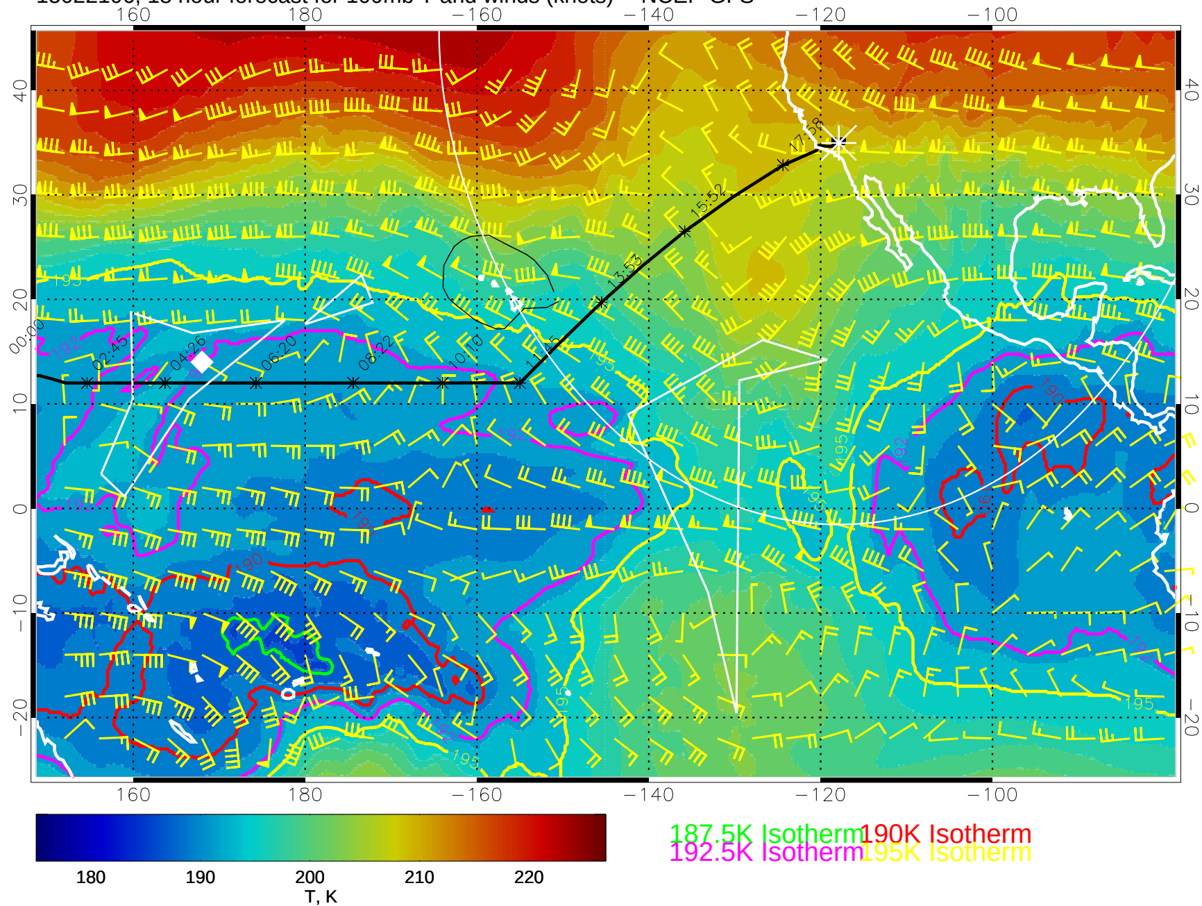
15022106, 18 hour forecast for 100mb T and winds (knots) -- NCEP GFS
