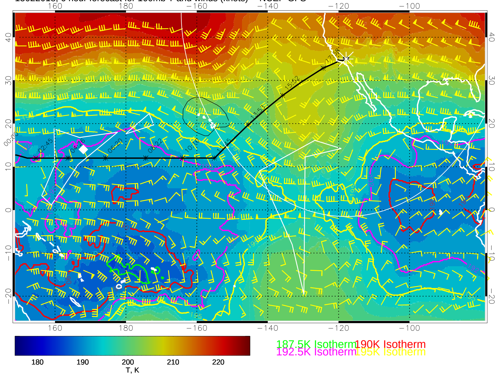
15022018, 6 hour forecast for 100mb T and winds (knots) -- NCEP GFS
