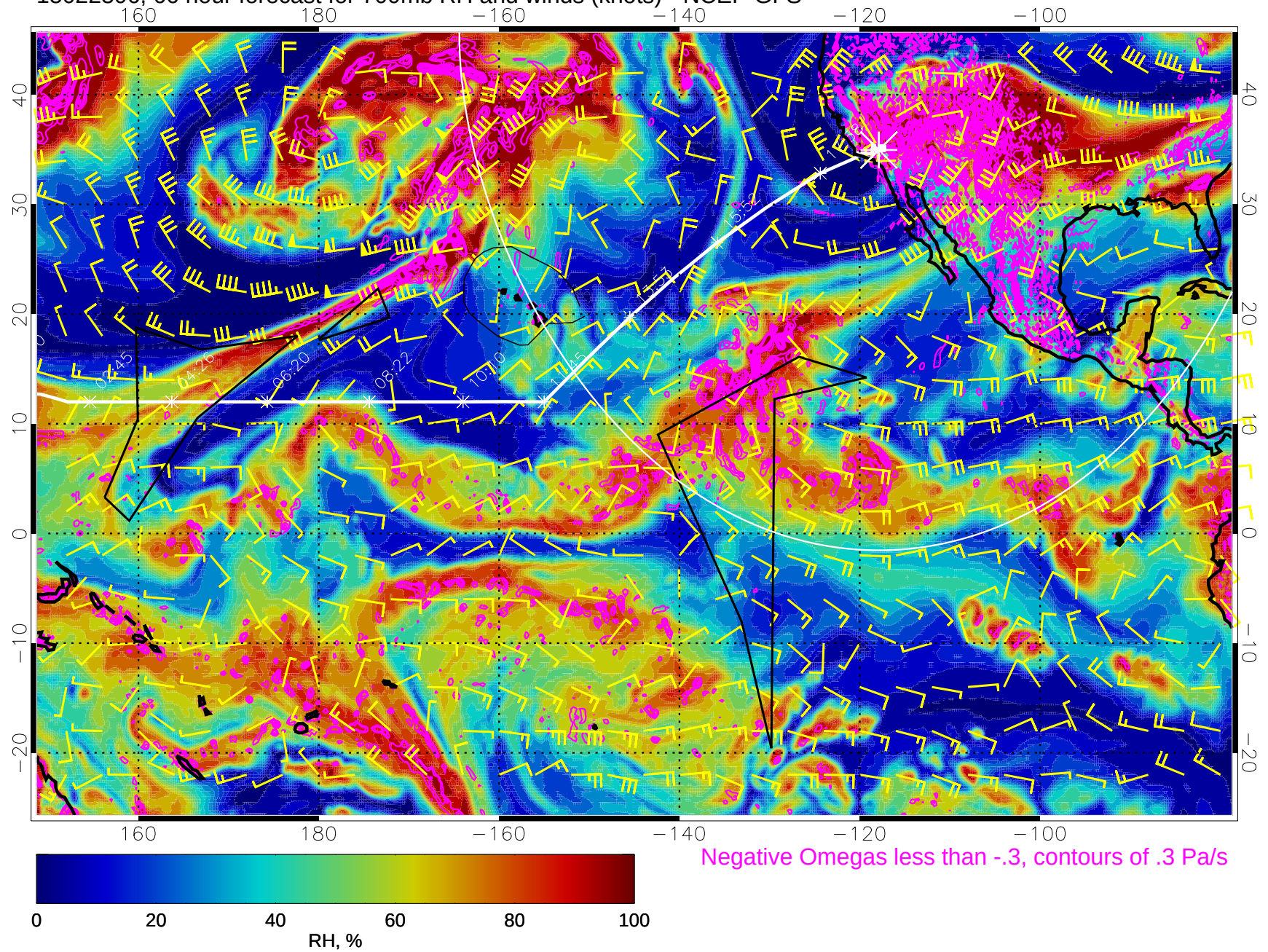
15022306, 66 hour forecast for 700mb RH and winds (knots) - NCEP GFS
