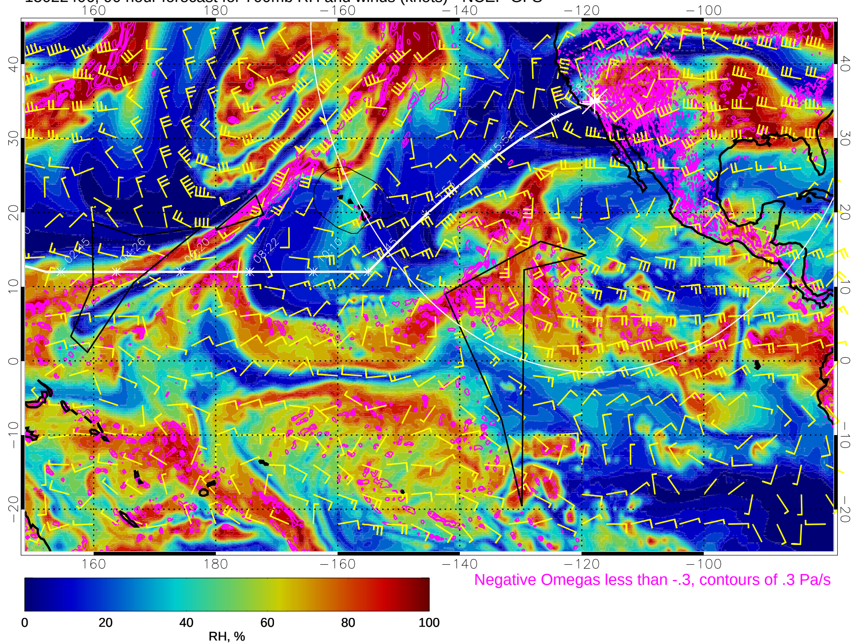
15022406, 90 hour forecast for 700mb RH and winds (knots) - NCEP GFS
