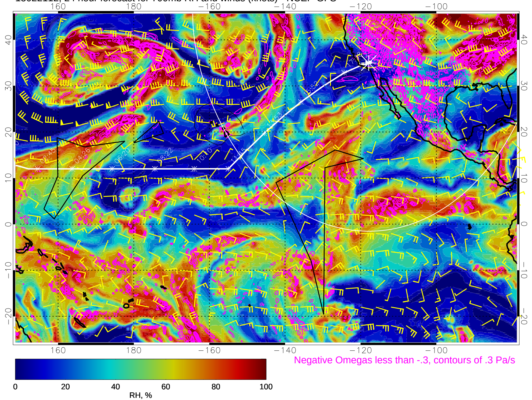
15022112, 24 hour forecast for 700mb RH and winds (knots) - NCEP GFS
