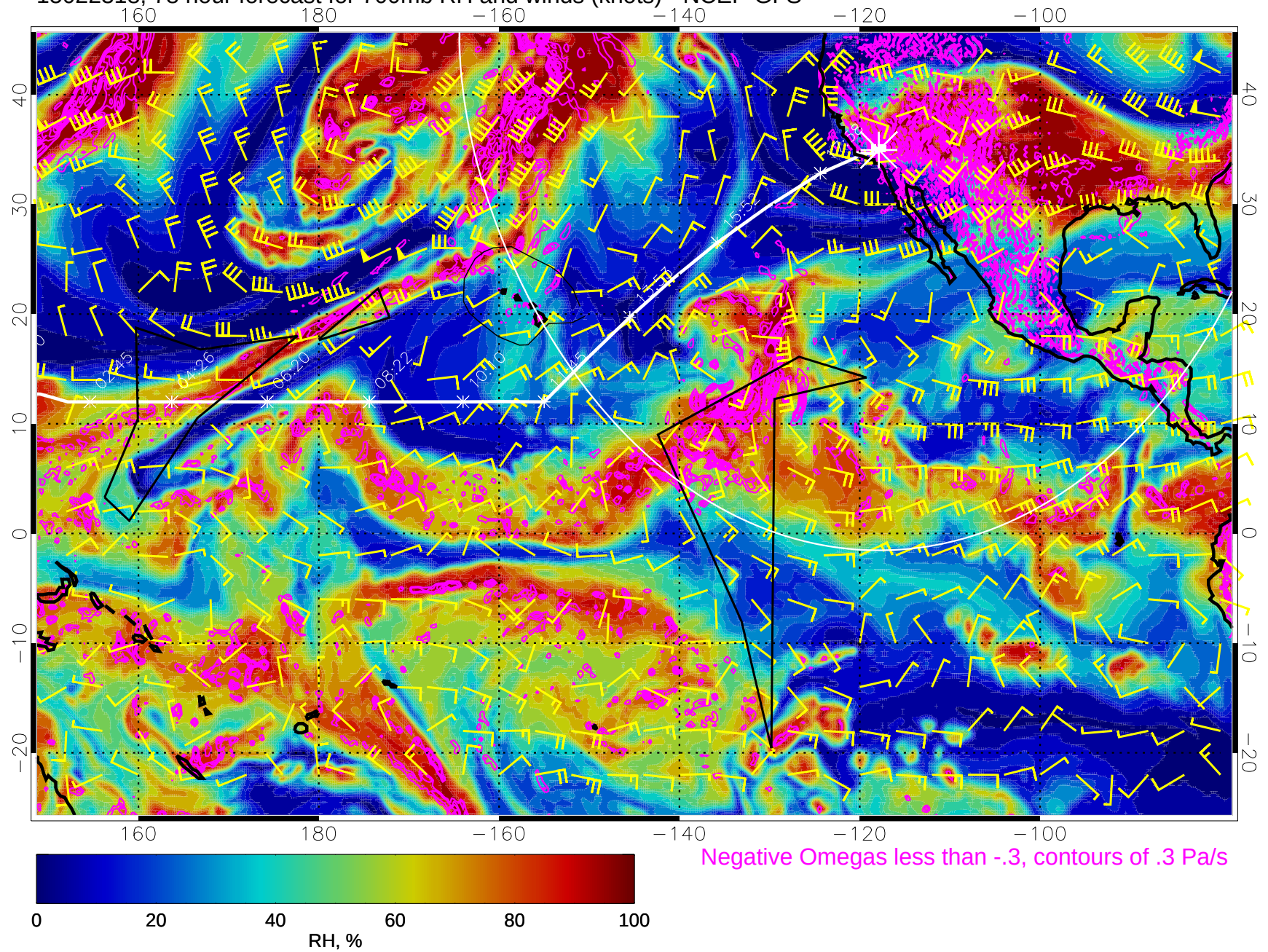
15022318, 78 hour forecast for 700mb RH and winds (knots) - NCEP GFS
