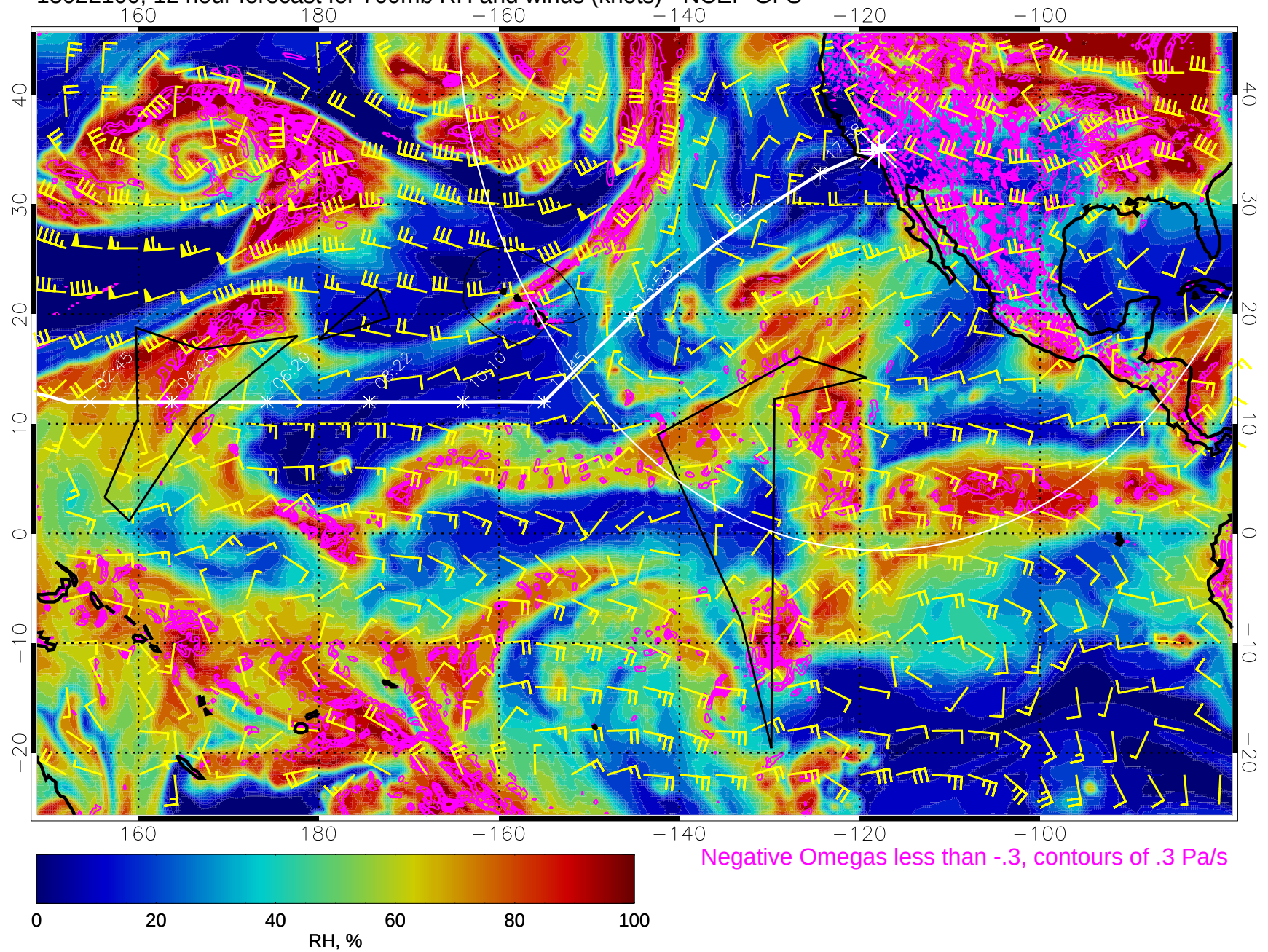
15022100, 12 hour forecast for 700mb RH and winds (knots) - NCEP GFS
