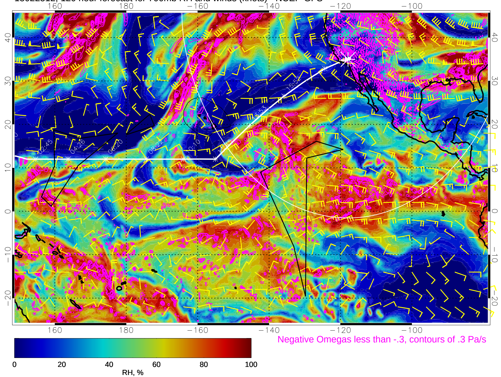
15022512, 120 hour forecast for 700mb RH and winds (knots) - NCEP GFS
