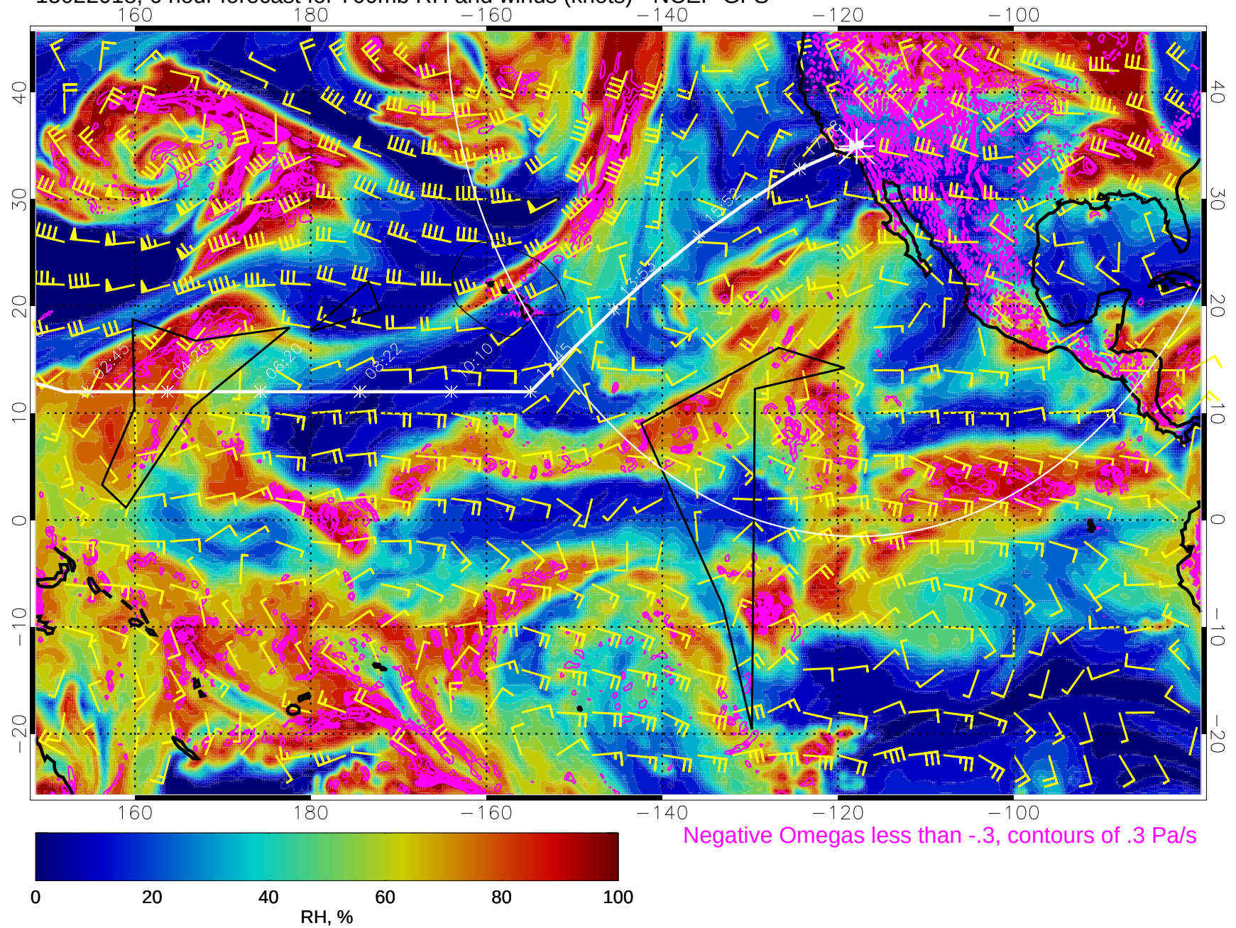
15022018, 6 hour forecast for 700mb RH and winds (knots) - NCEP GFS
