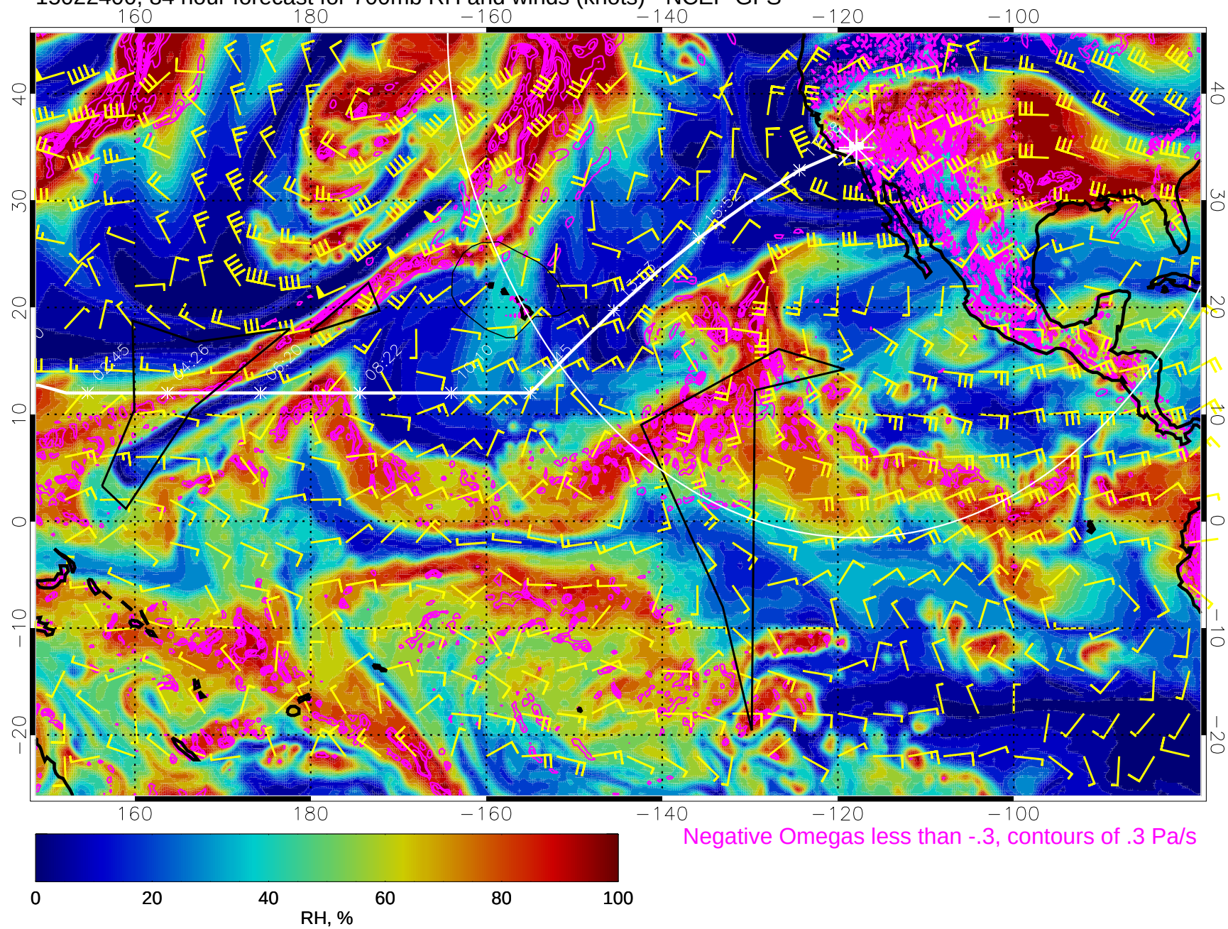
15022400, 84 hour forecast for 700mb RH and winds (knots) - NCEP GFS
