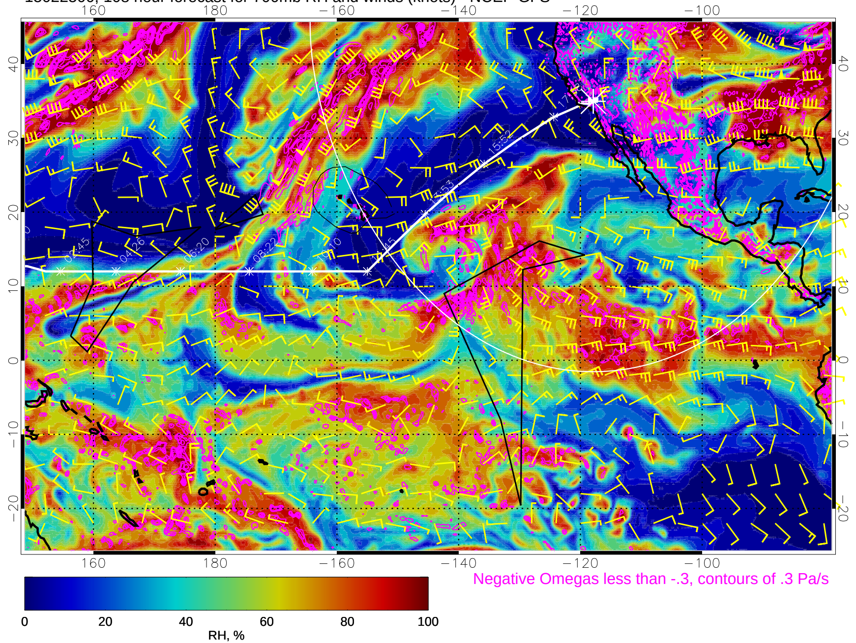
15022500, 108 hour forecast for 700mb RH and winds (knots) - NCEP GFS
