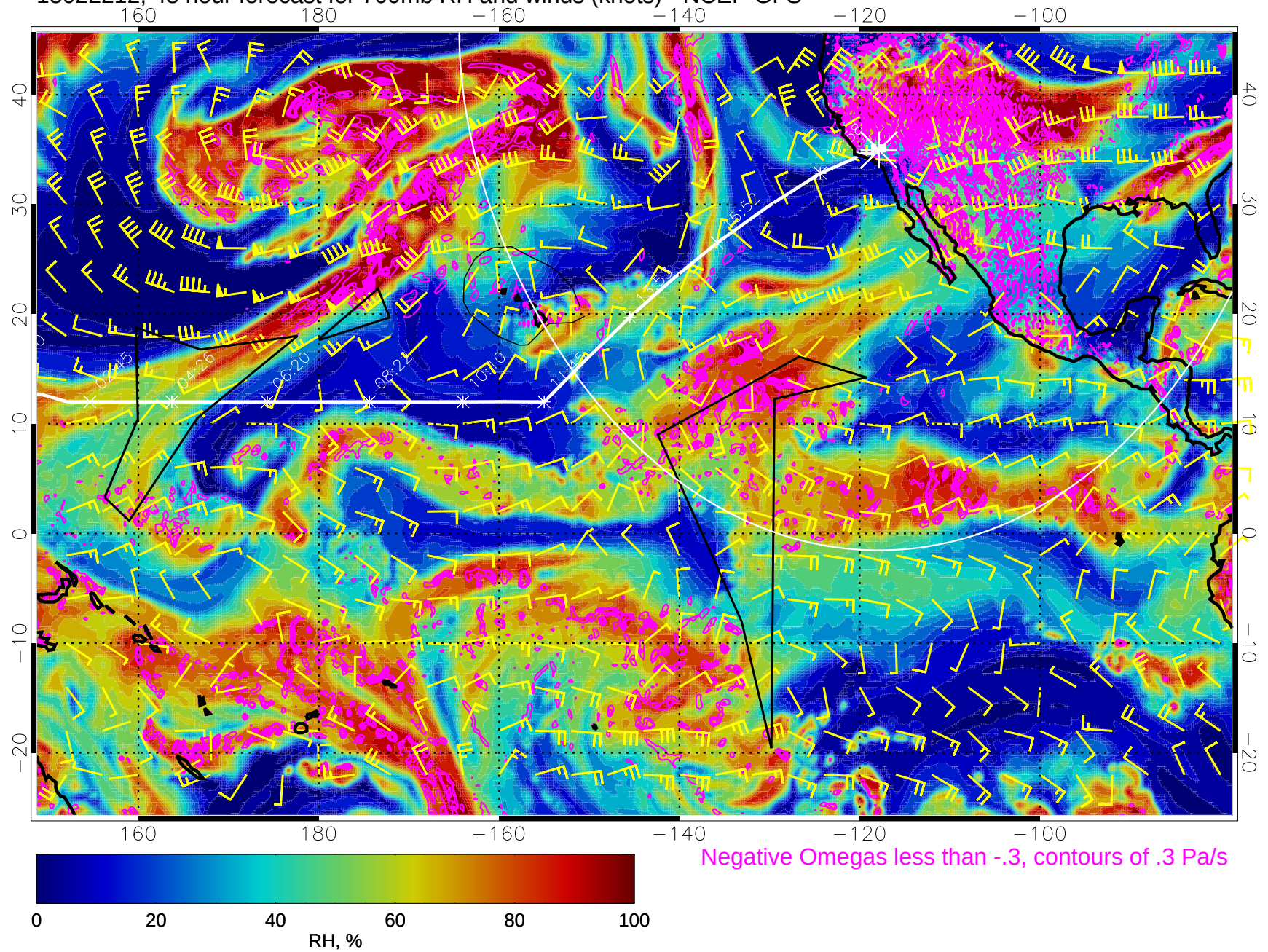
15022212, 48 hour forecast for 700mb RH and winds (knots) - NCEP GFS
