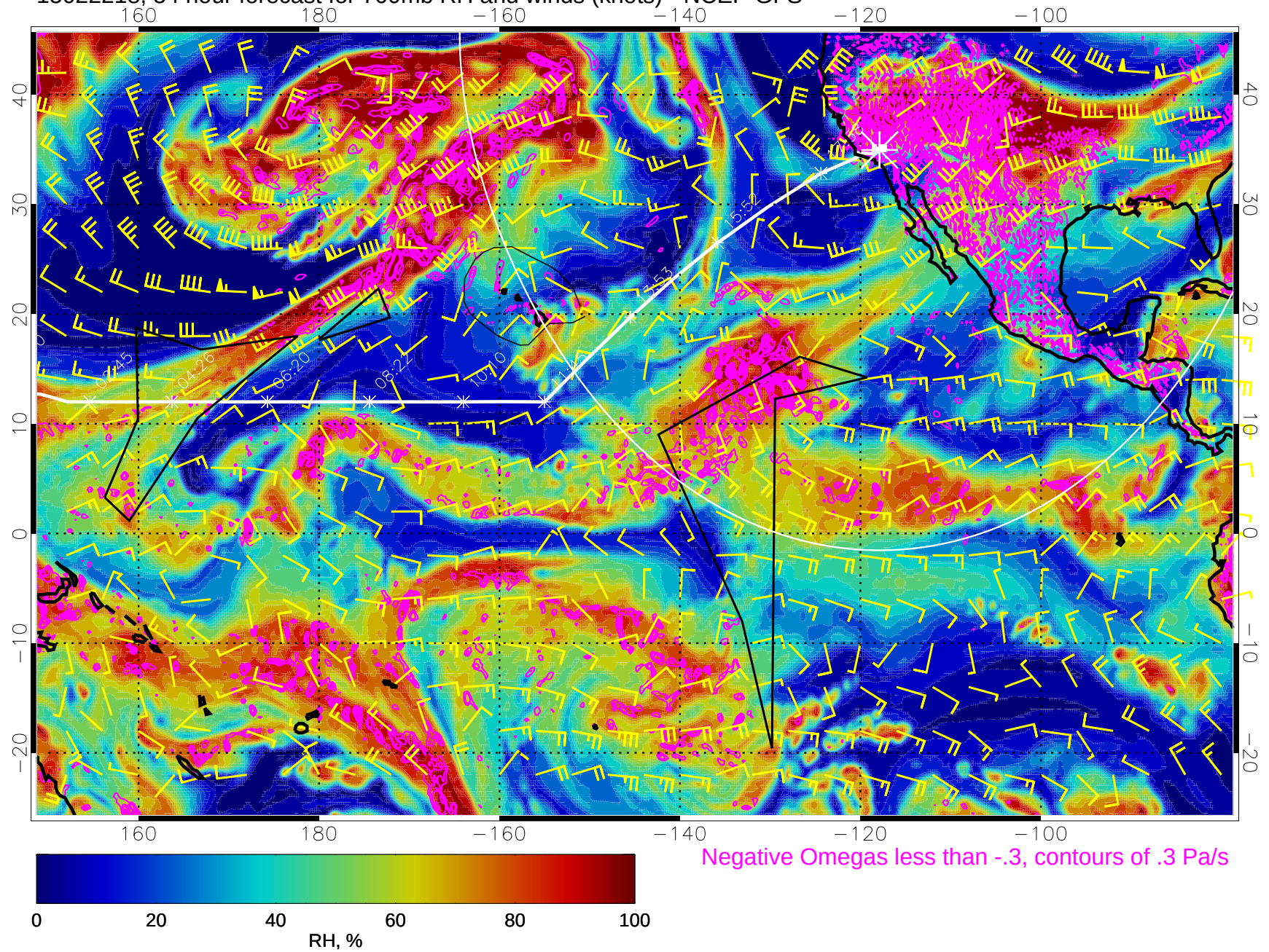
15022218, 54 hour forecast for 700mb RH and winds (knots) - NCEP GFS
