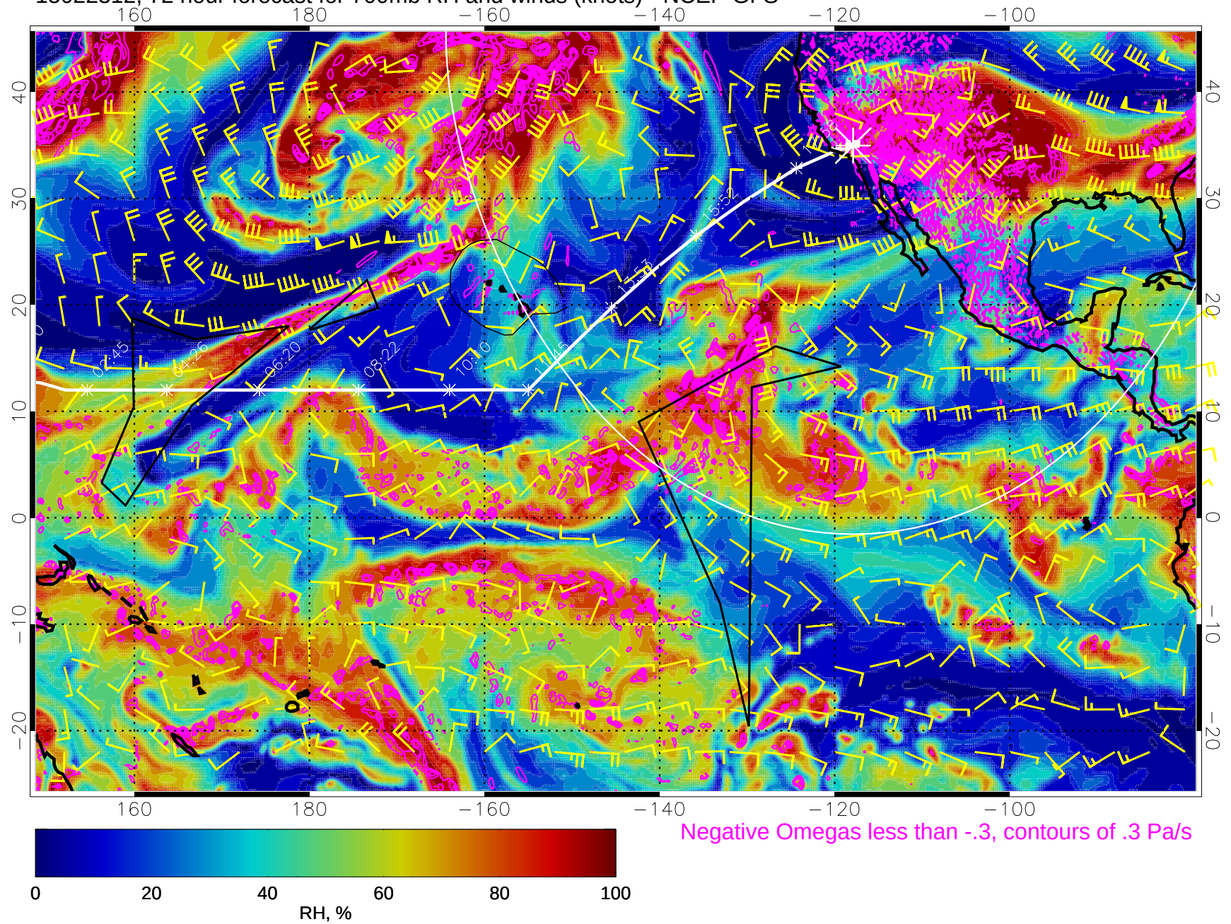
15022312, 72 hour forecast for 700mb RH and winds (knots) - NCEP GFS
