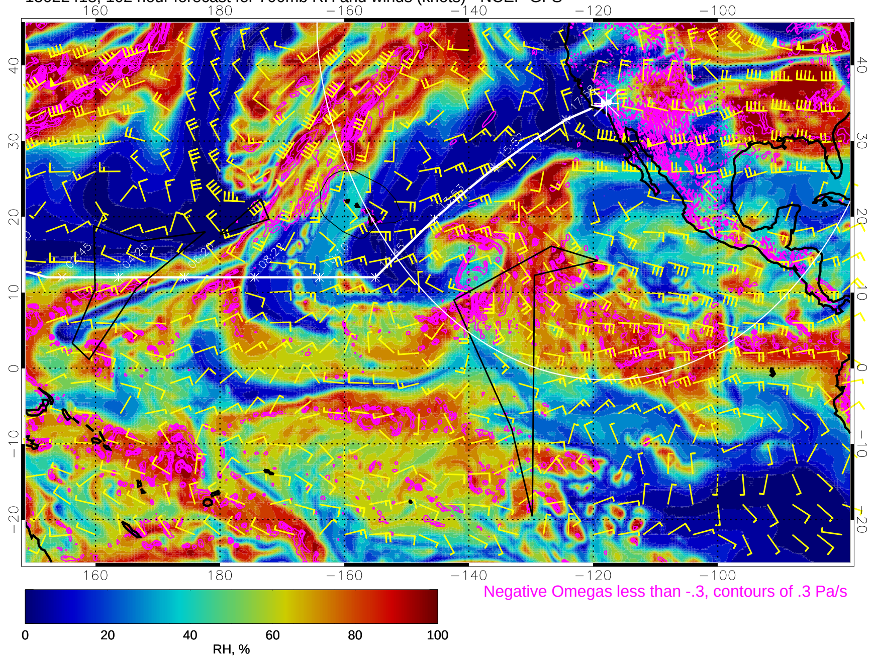
15022418, 102 hour forecast for 700mb RH and winds (knots) - NCEP GFS
