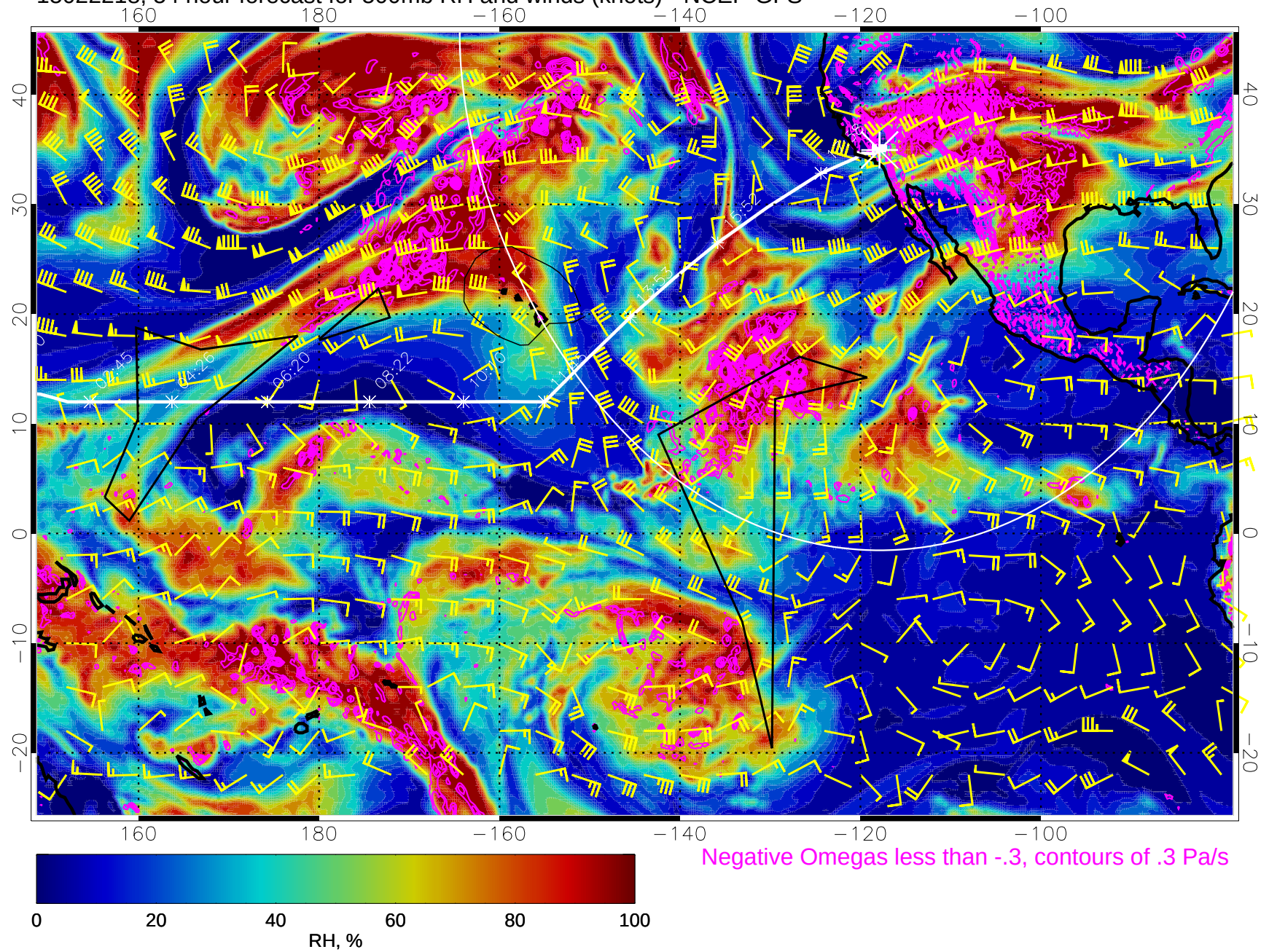
15022218, 54 hour forecast for 500mb RH and winds (knots) - NCEP GFS
