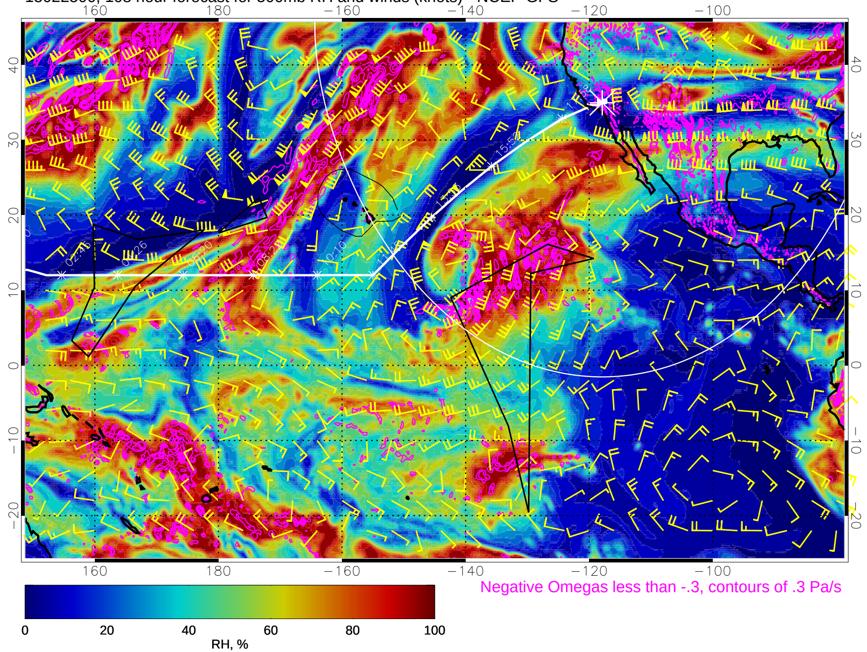
15022500, 108 hour forecast for 500mb RH and winds (knots) - NCEP GFS
