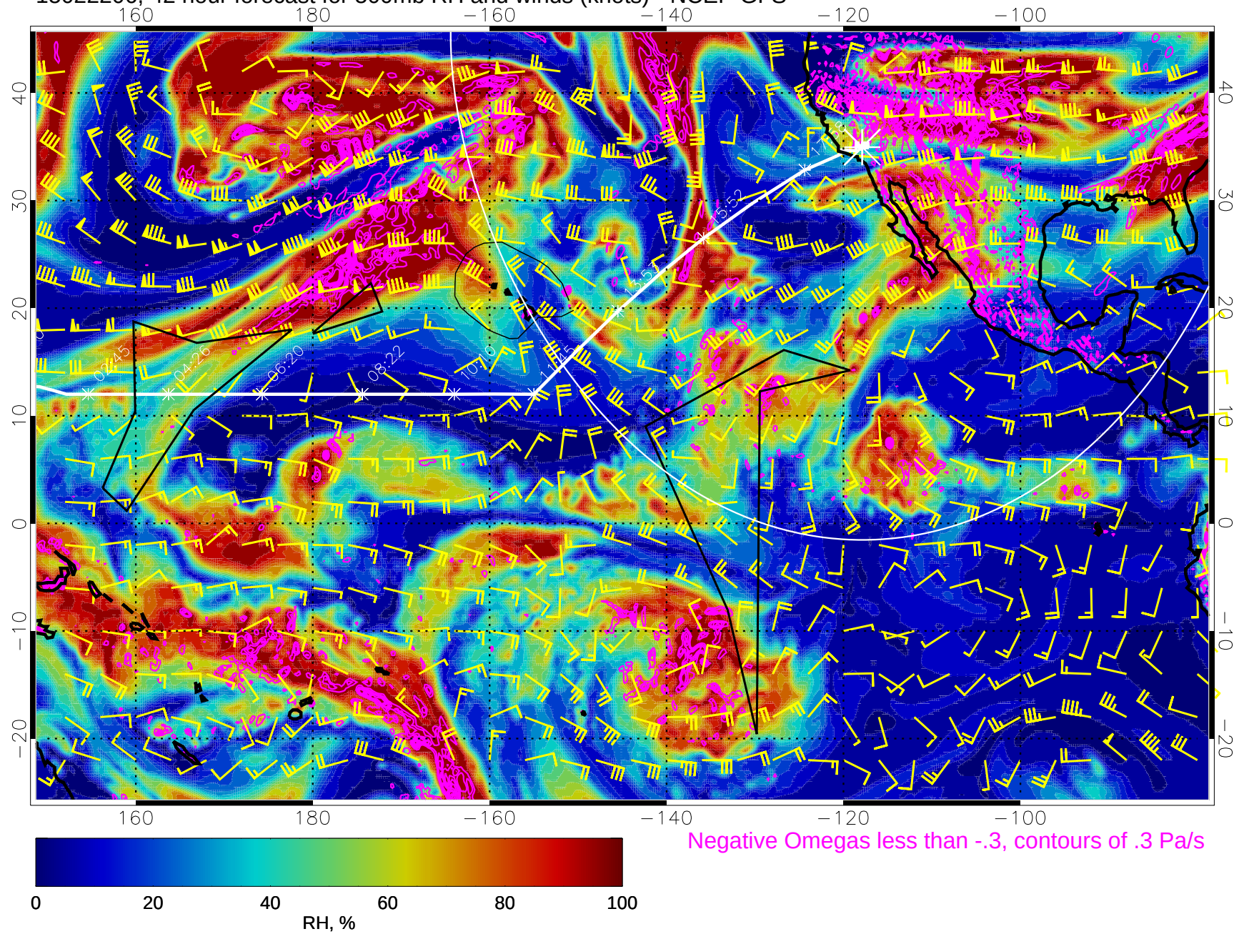
15022206, 42 hour forecast for 500mb RH and winds (knots) - NCEP GFS
