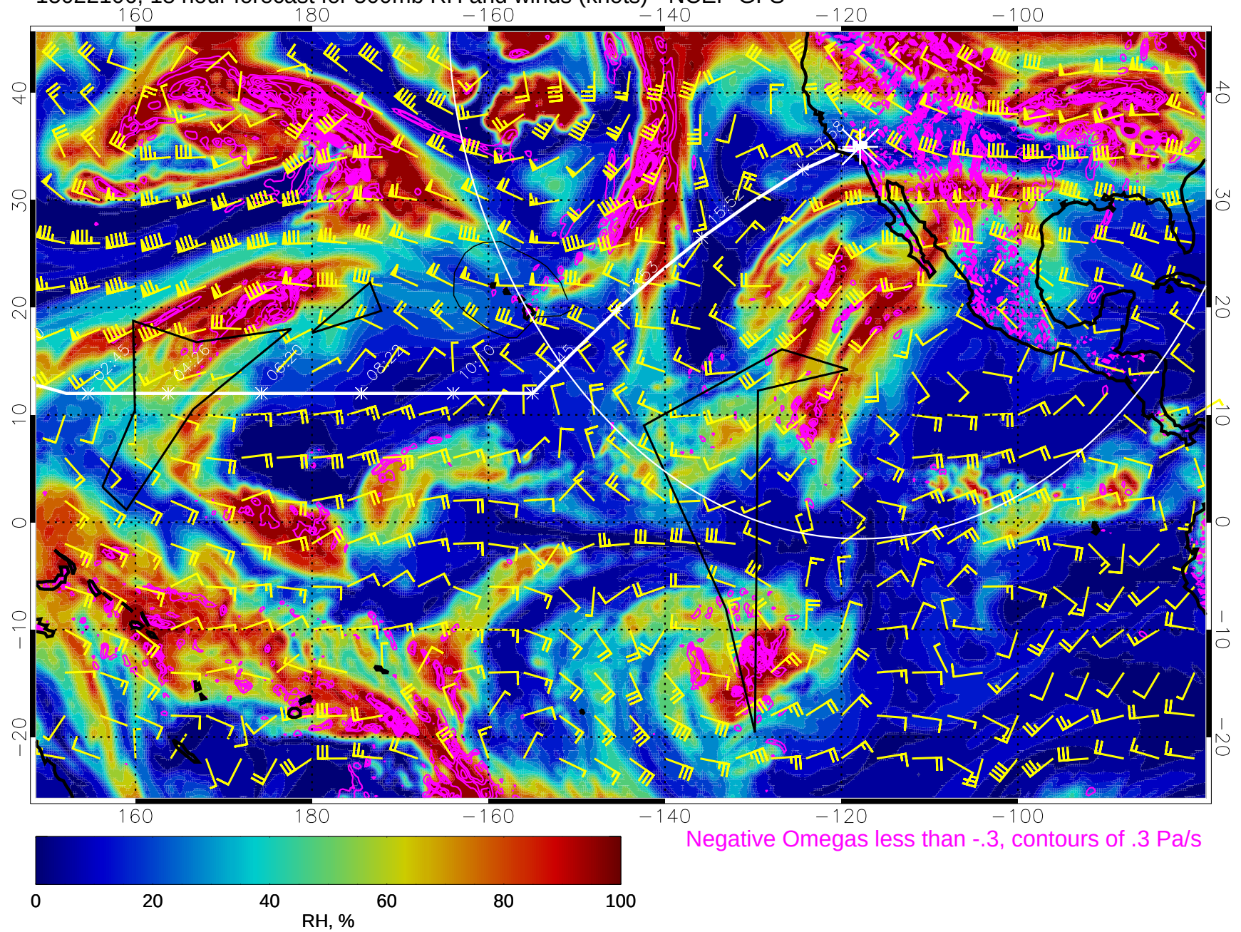
15022106, 18 hour forecast for 500mb RH and winds (knots) - NCEP GFS
