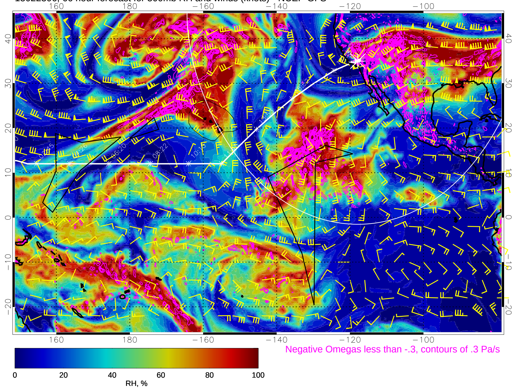
15022306, 66 hour forecast for 500mb RH and winds (knots) - NCEP GFS
