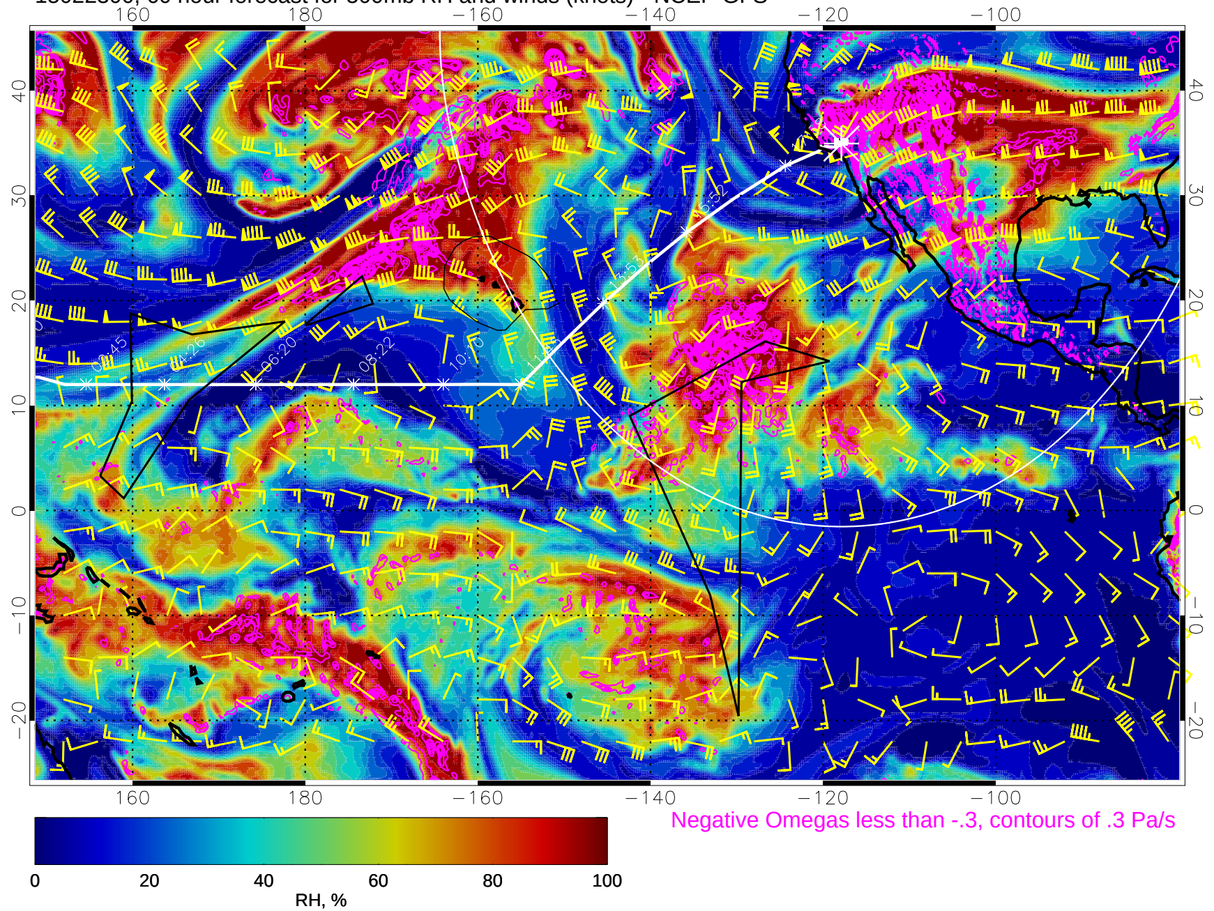
15022300, 60 hour forecast for 500mb RH and winds (knots) - NCEP GFS
