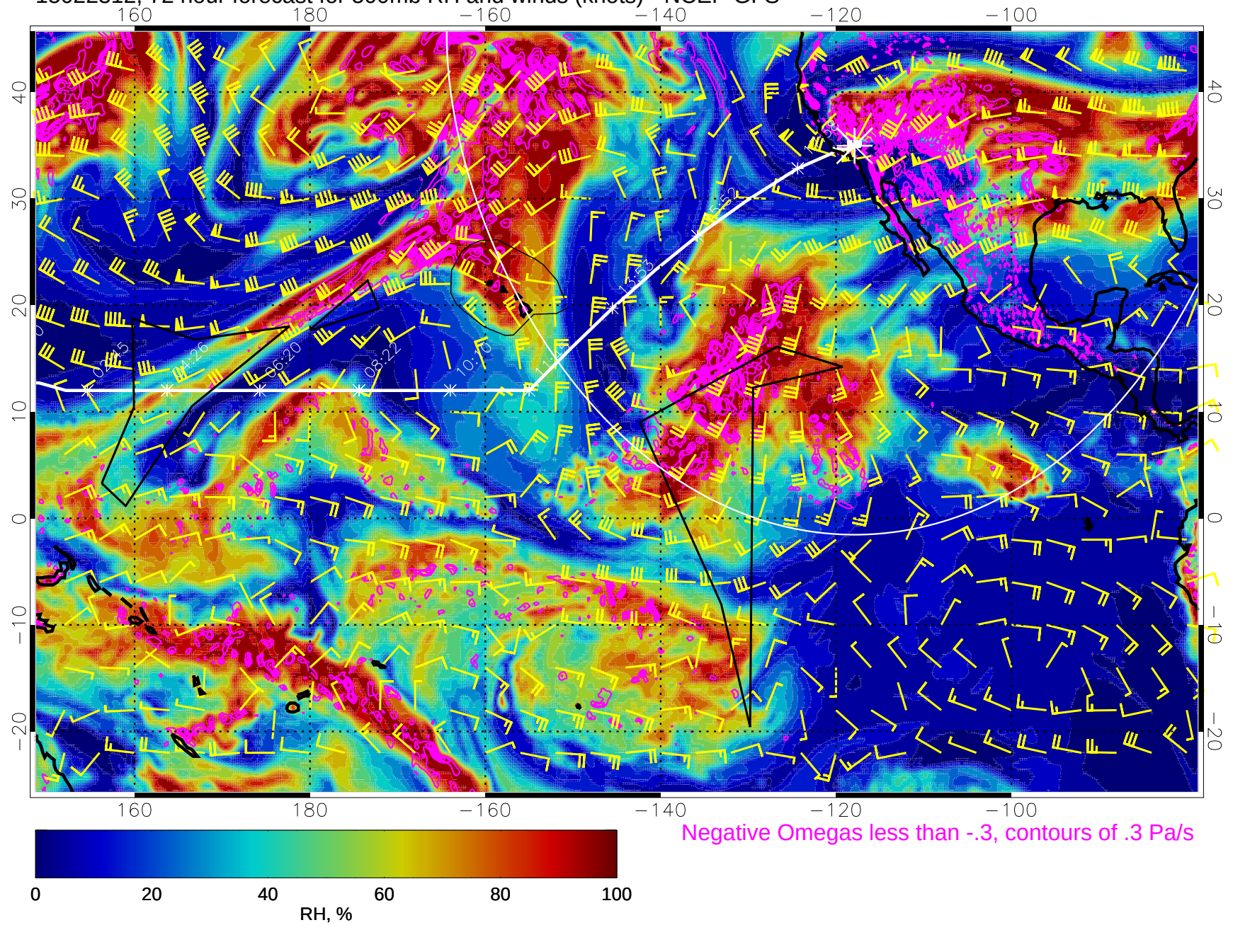
15022312, 72 hour forecast for 500mb RH and winds (knots) - NCEP GFS
