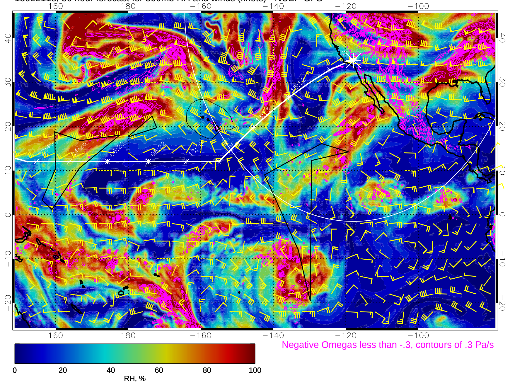
15022118, 30 hour forecast for 500mb RH and winds (knots) - NCEP GFS
