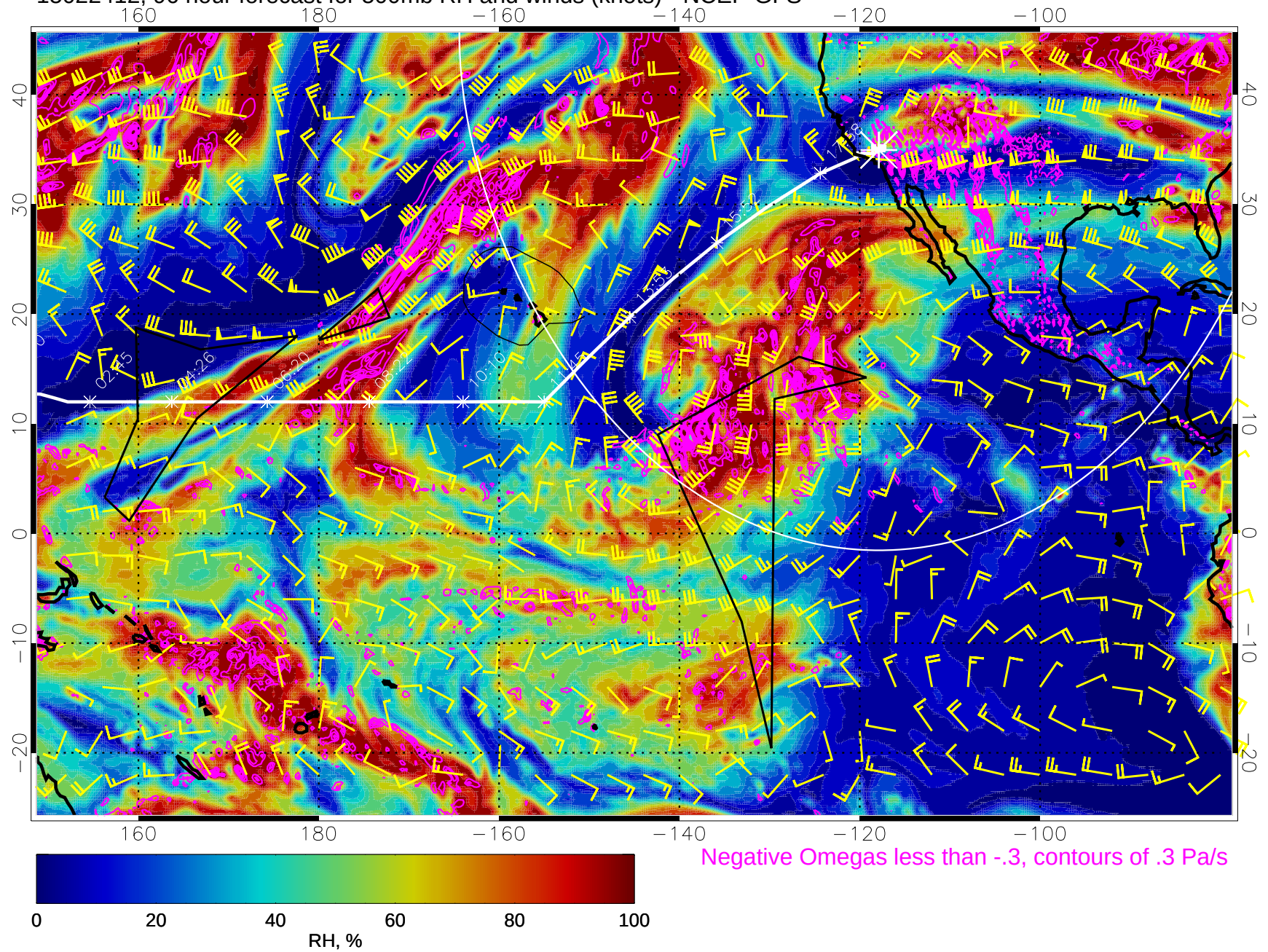
15022412, 96 hour forecast for 500mb RH and winds (knots) - NCEP GFS
