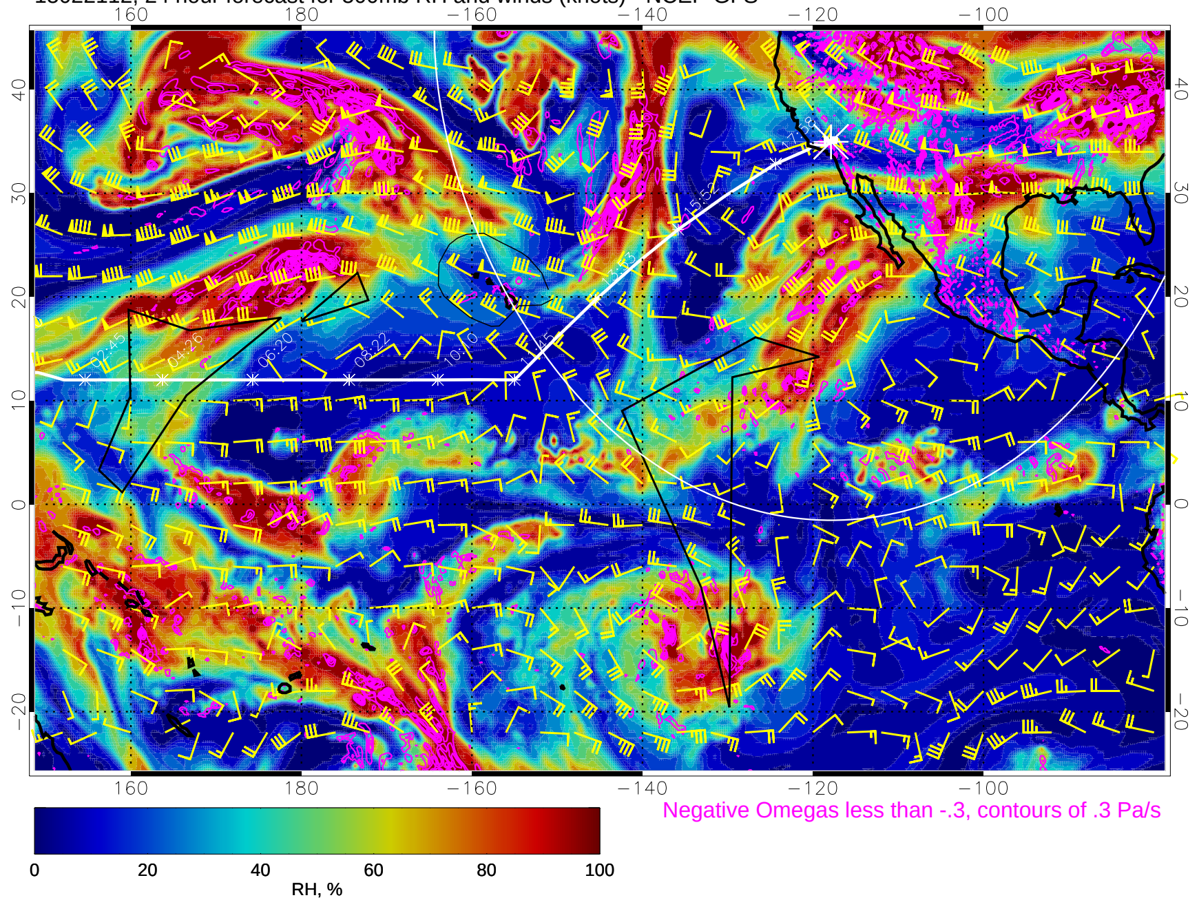
15022112, 24 hour forecast for 500mb RH and winds (knots) - NCEP GFS
