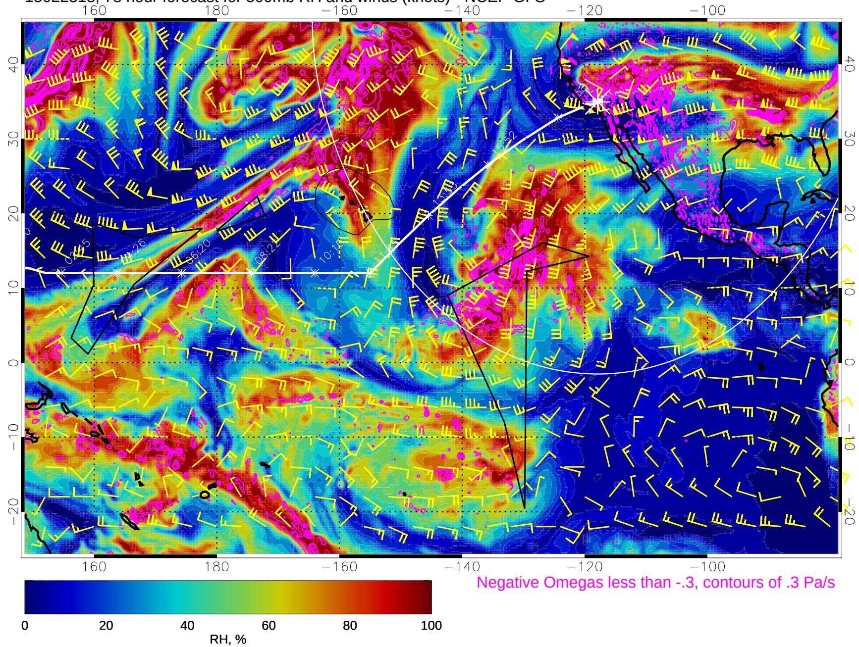
15022318, 78 hour forecast for 500mb RH and winds (knots) - NCEP GFS
