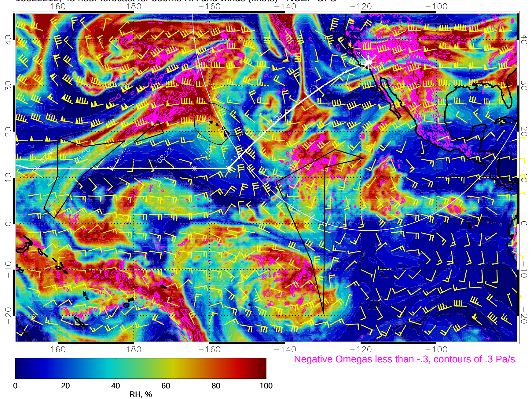
15022212, 48 hour forecast for 500mb RH and winds (knots) - NCEP GFS
