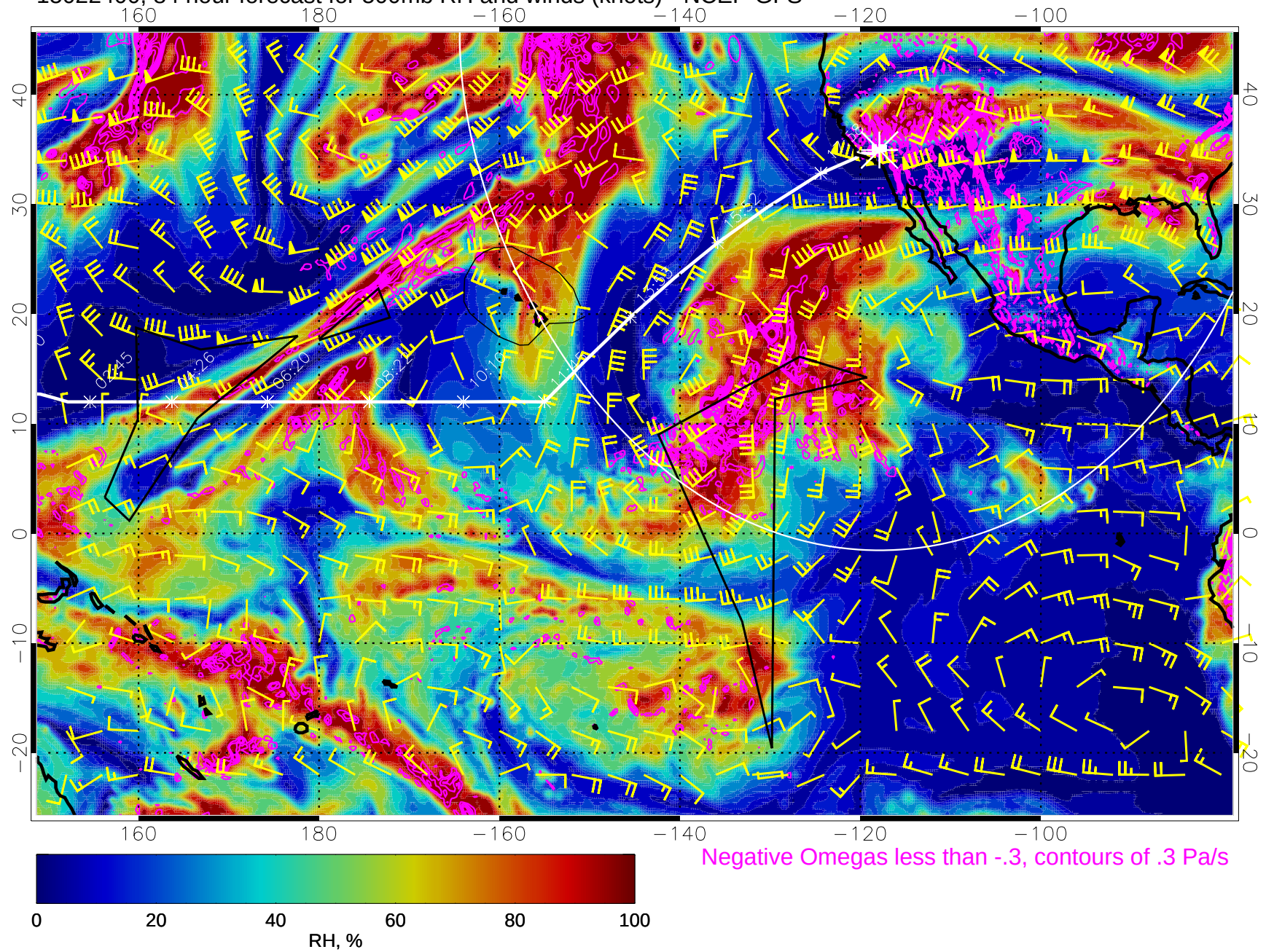
15022400, 84 hour forecast for 500mb RH and winds (knots) - NCEP GFS
