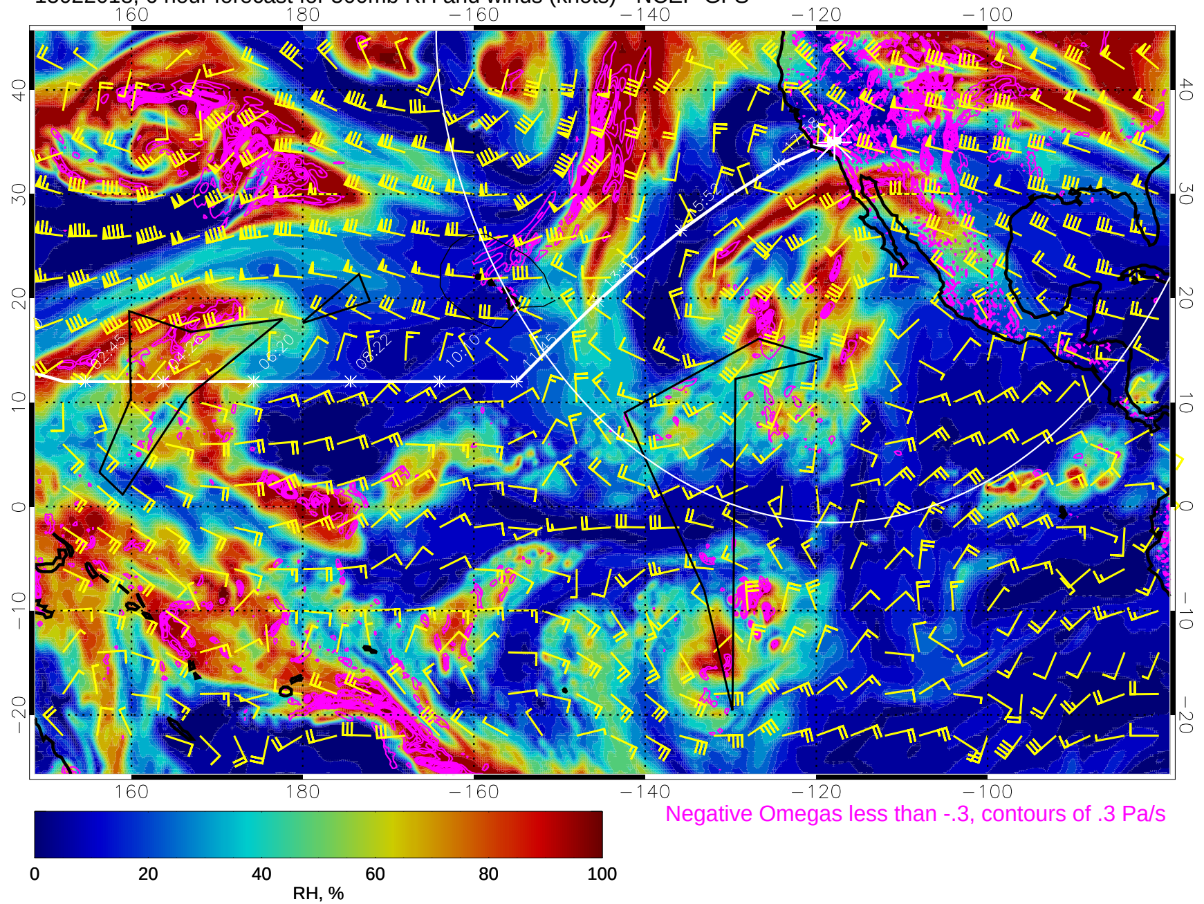
15022018, 6 hour forecast for 500mb RH and winds (knots) - NCEP GFS
