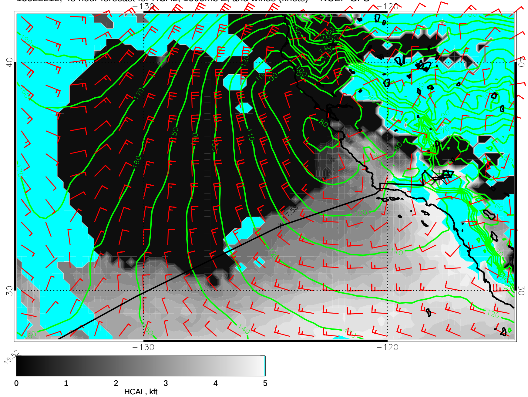
15022212, 48 hour forecast for HCAL, 1000mb Z, and winds (knots) -- NCEP GFS
