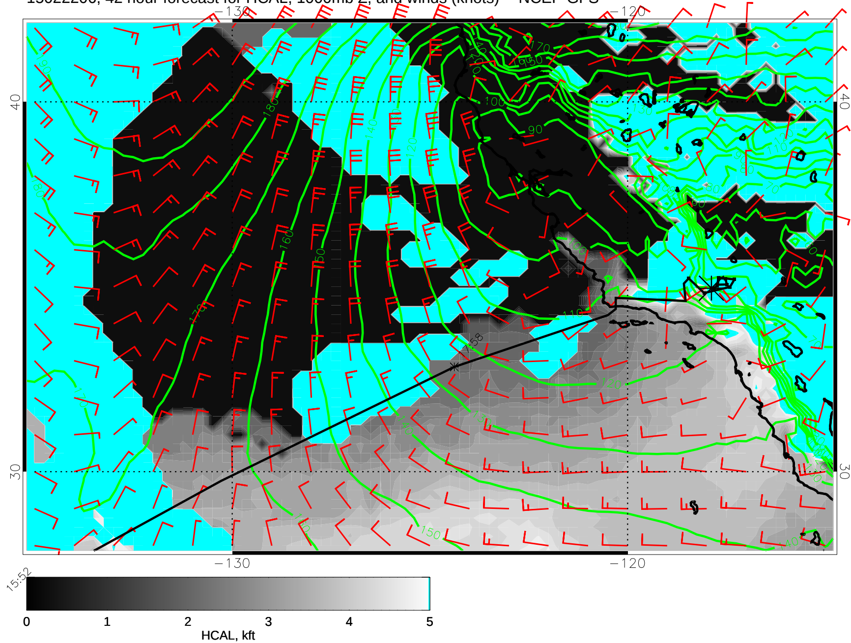
15022206, 42 hour forecast for HCAL, 1000mb Z, and winds (knots) -- NCEP GFS
