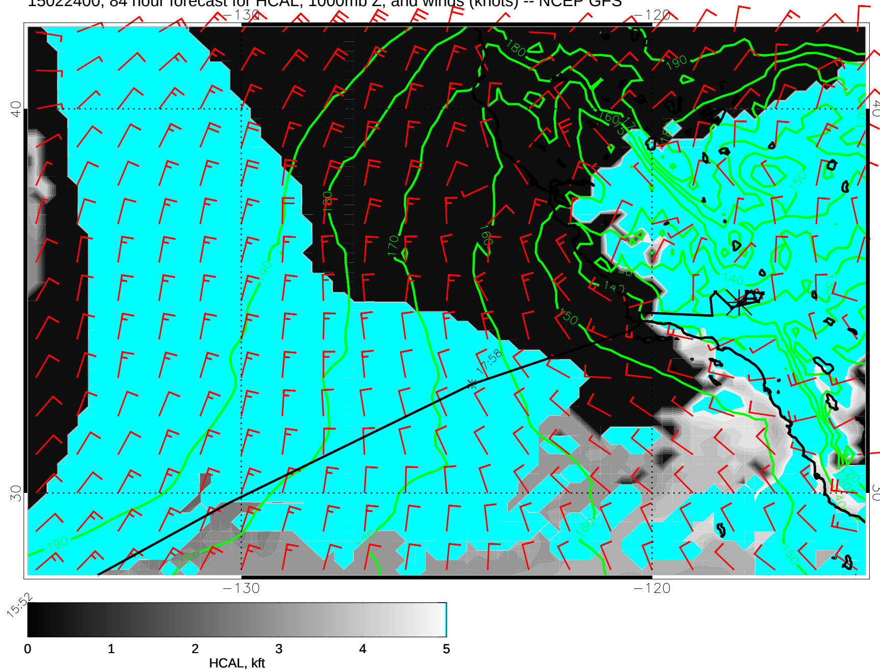
15022400, 84 hour forecast for HCAL, 1000mb Z, and winds (knots) -- NCEP GFS
