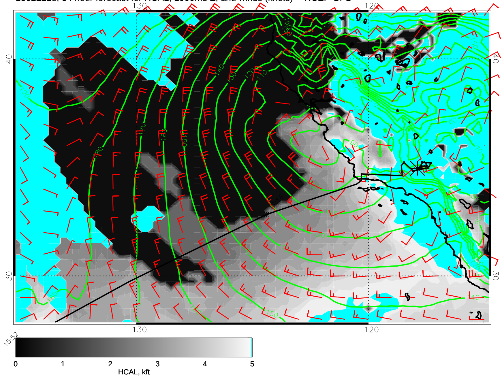
15022218, 54 hour forecast for HCAL, 1000mb Z, and winds (knots) -- NCEP GFS
