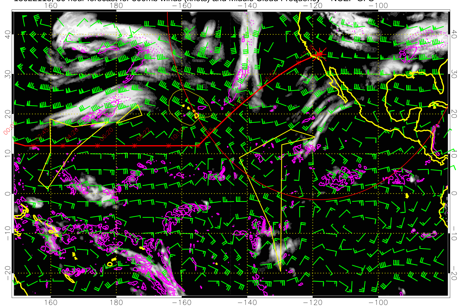
15022118, 30 hour forecast for 500mb winds (knots) and Middle Cloud Frequency -- NCEP GFS
