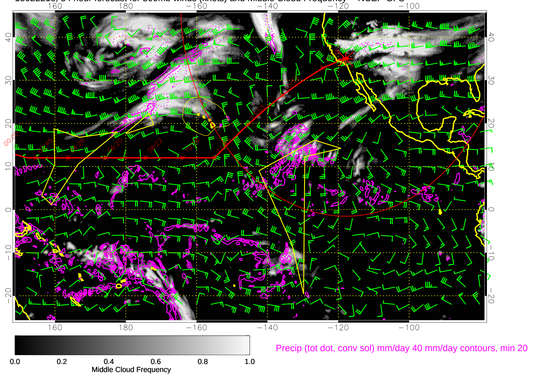
15022218, 54 hour forecast for 500mb winds (knots) and Middle Cloud Frequency -- NCEP GFS
