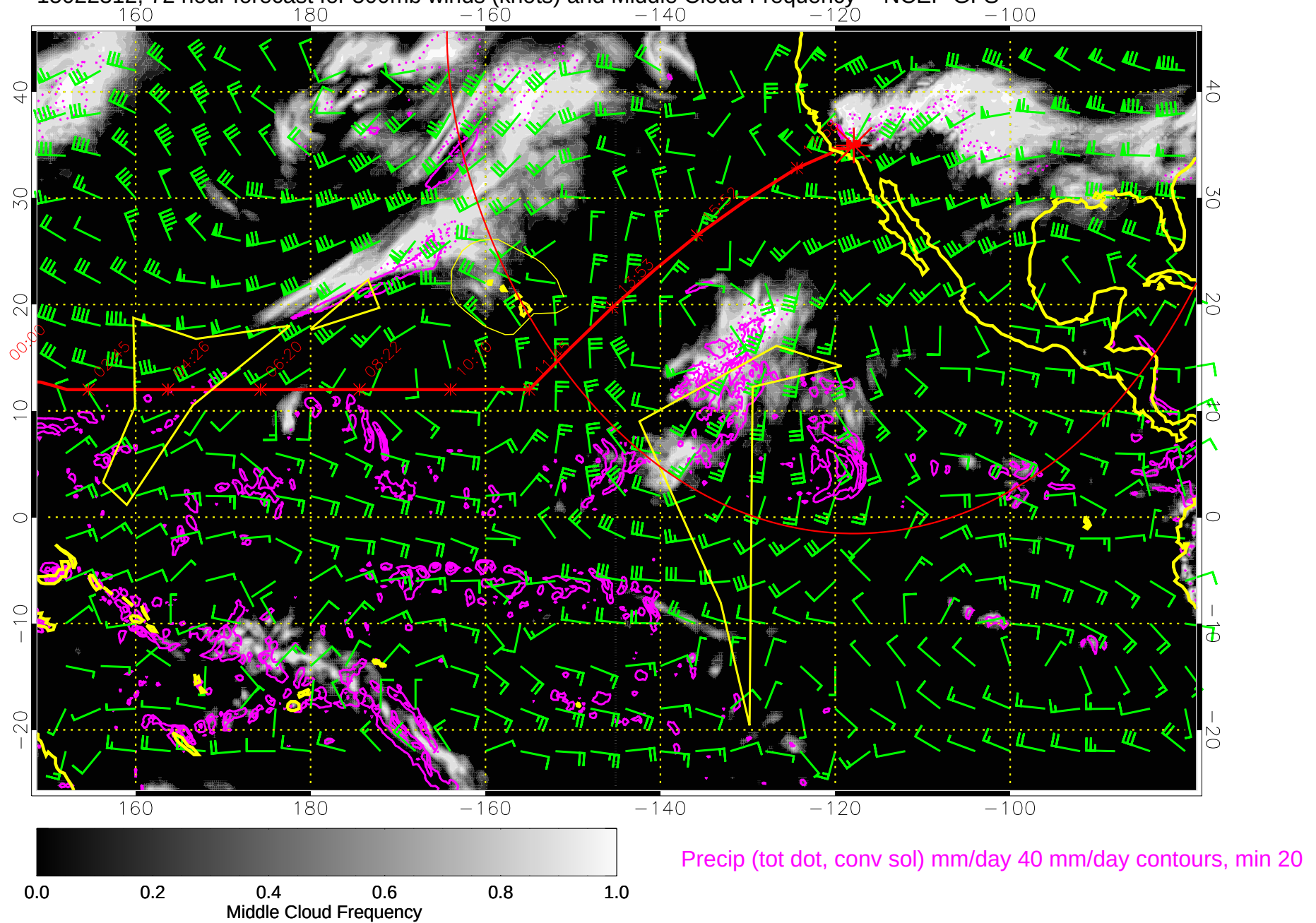
15022312, 72 hour forecast for 500mb winds (knots) and Middle Cloud Frequency -- NCEP GFS
