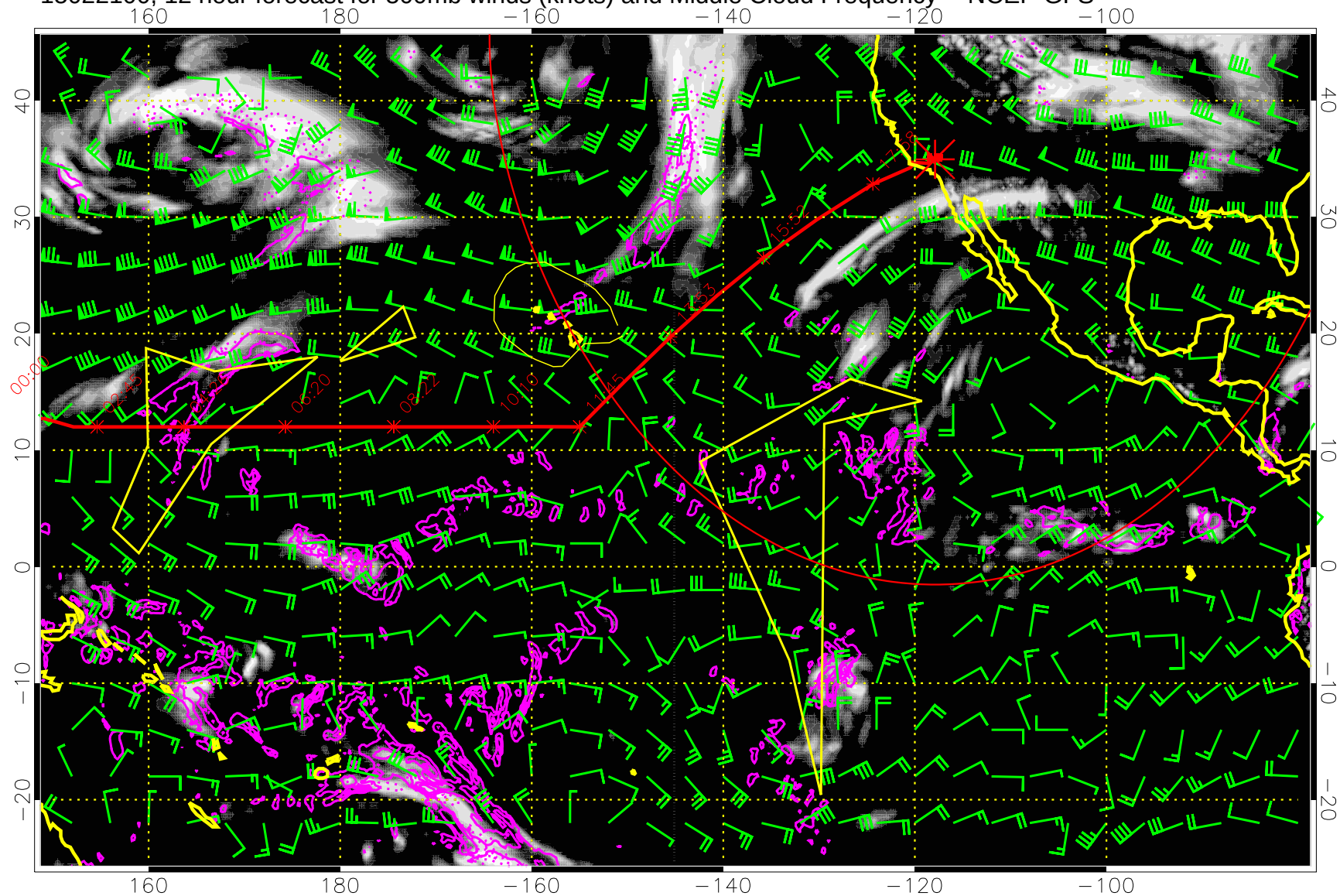
15022100, 12 hour forecast for 500mb winds (knots) and Middle Cloud Frequency -- NCEP GFS
