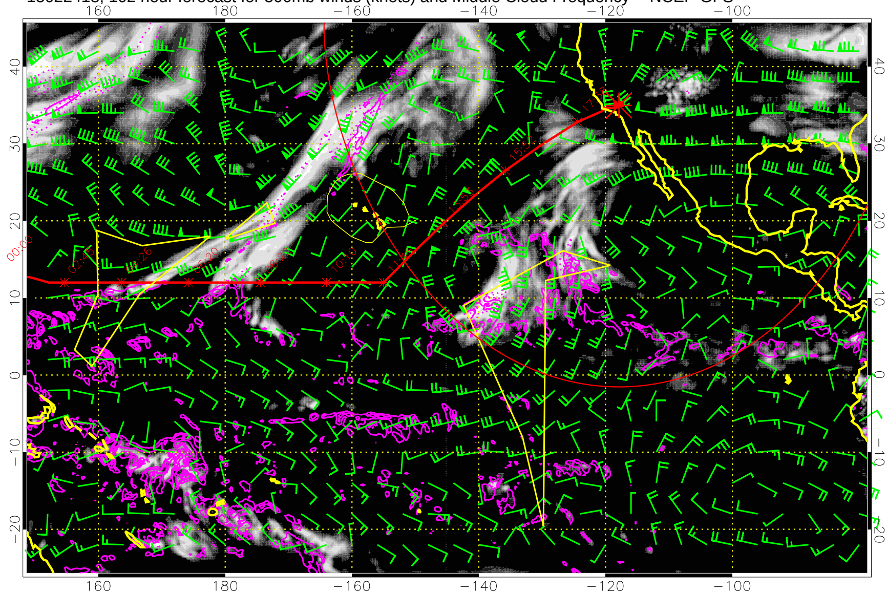
15022418, 102 hour forecast for 500mb winds (knots) and Middle Cloud Frequency -- NCEP GFS
