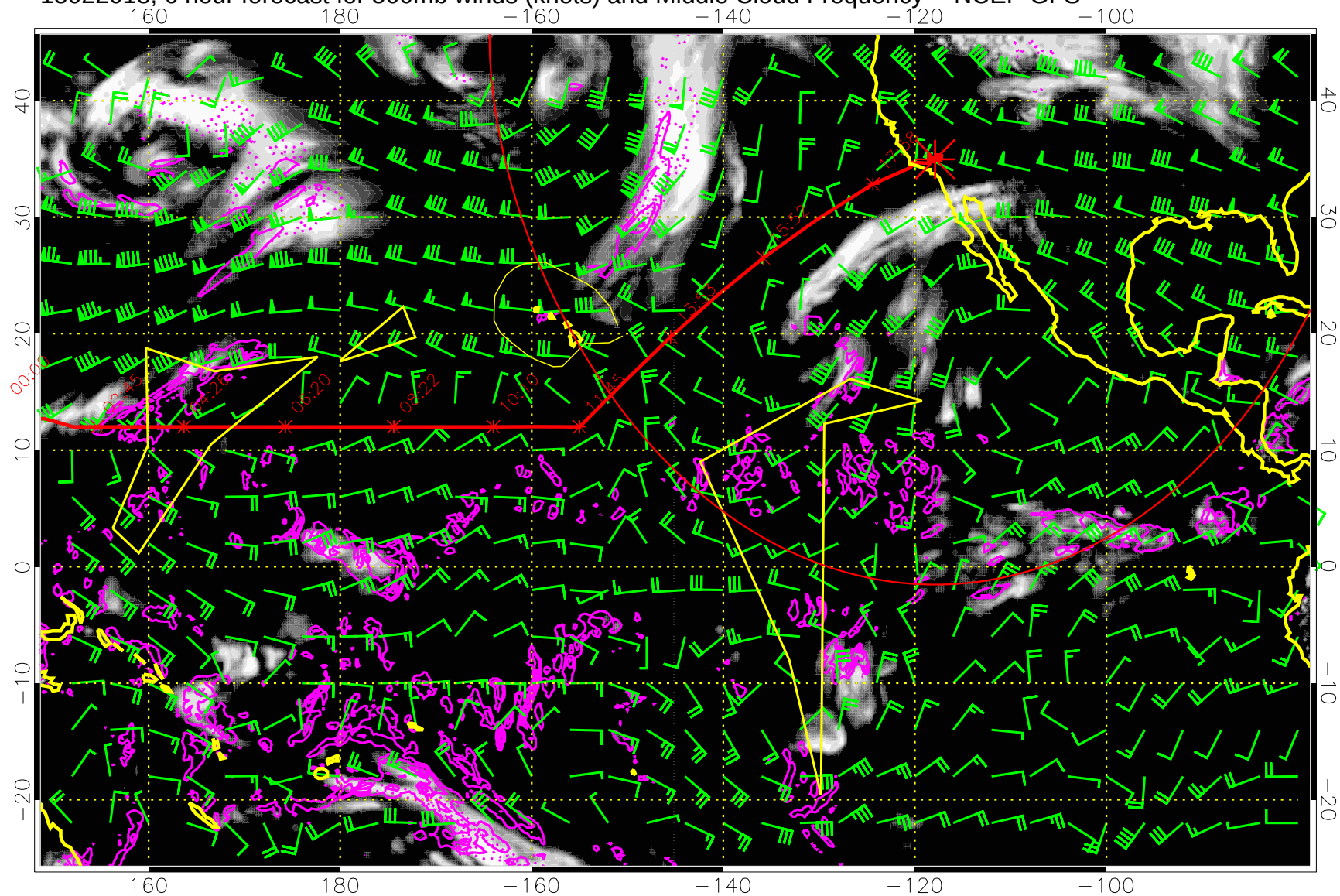
15022018, 6 hour forecast for 500mb winds (knots) and Middle Cloud Frequency -- NCEP GFS
