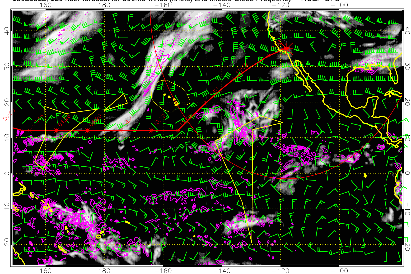
15022512, 120 hour forecast for 500mb winds (knots) and Middle Cloud Frequency -- NCEP GFS
