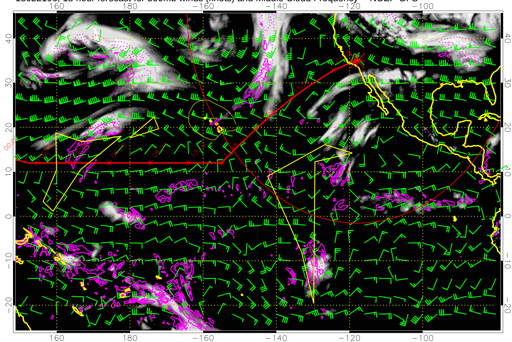
15022106, 18 hour forecast for 500mb winds (knots) and Middle Cloud Frequency -- NCEP GFS
