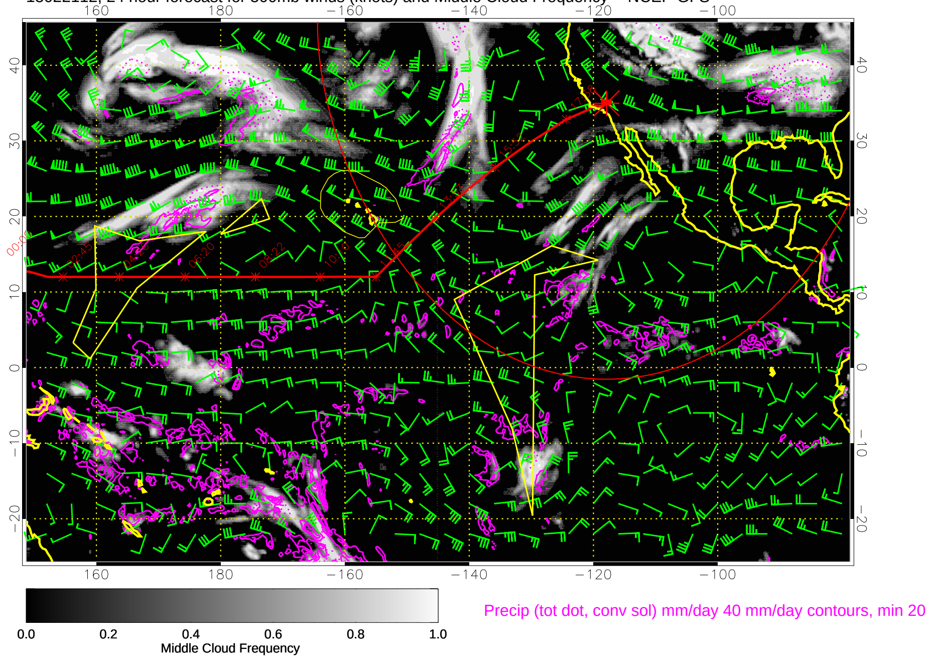
15022112, 24 hour forecast for 500mb winds (knots) and Middle Cloud Frequency -- NCEP GFS
