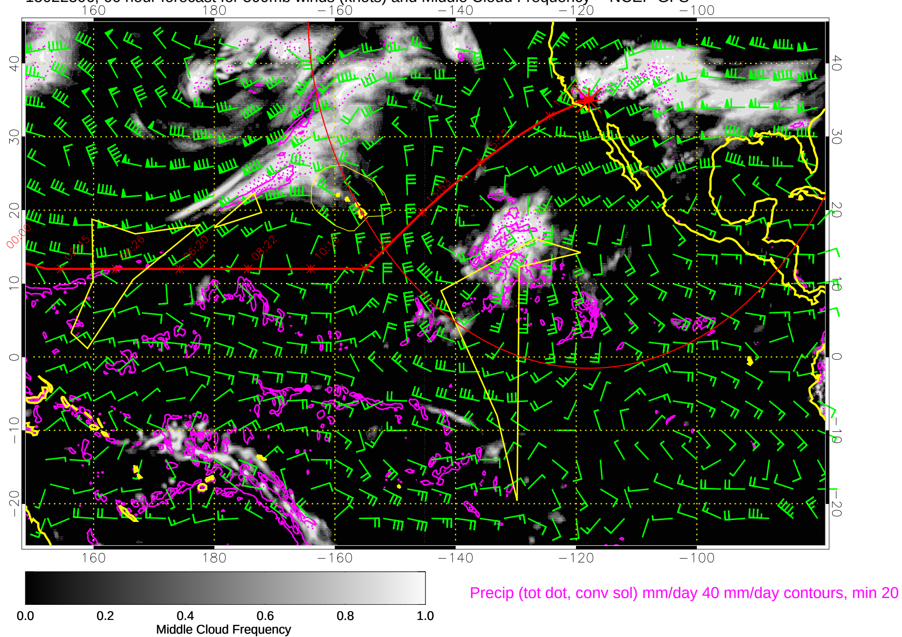
15022306, 66 hour forecast for 500mb winds (knots) and Middle Cloud Frequency -- NCEP GFS
