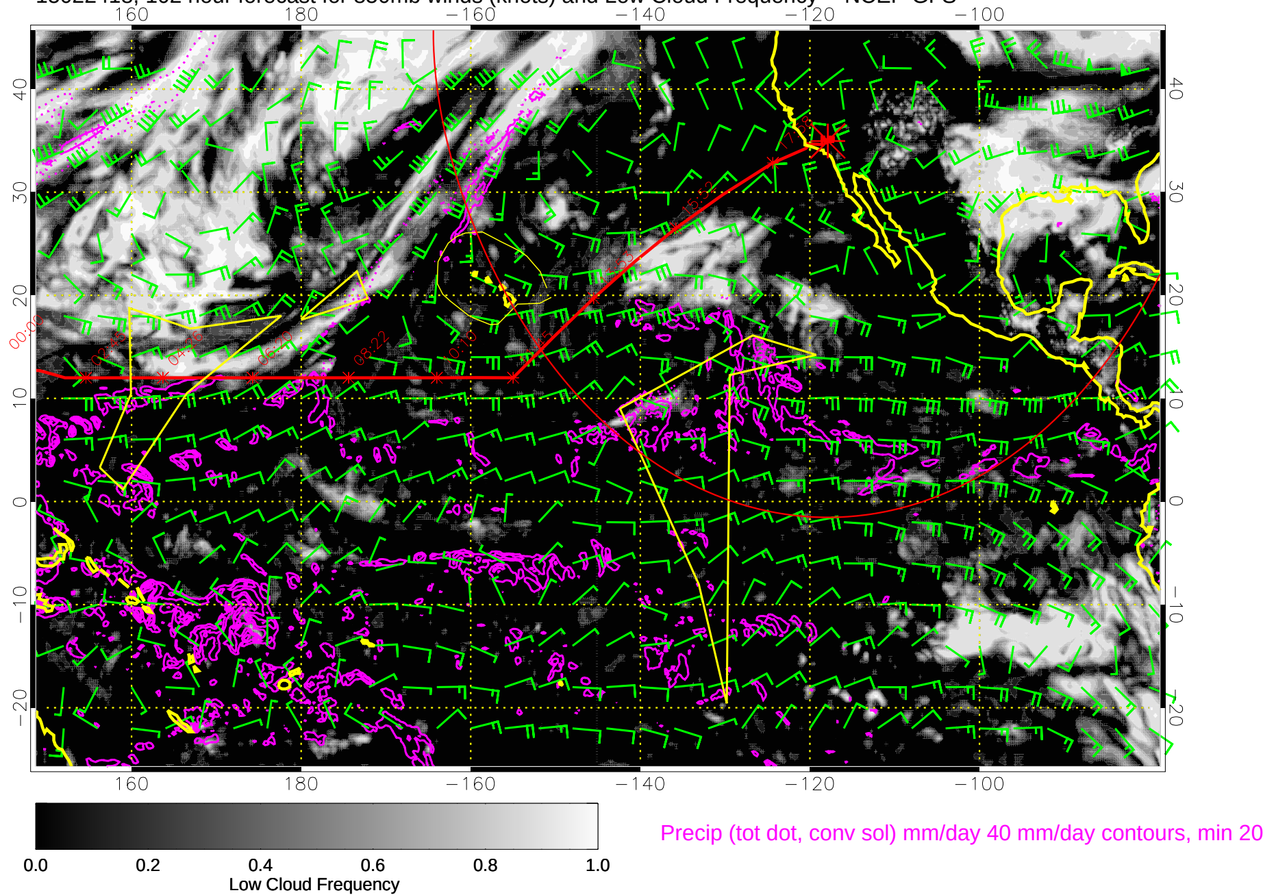
15022418, 102 hour forecast for 850mb winds (knots) and Low Cloud Frequency -- NCEP GFS
