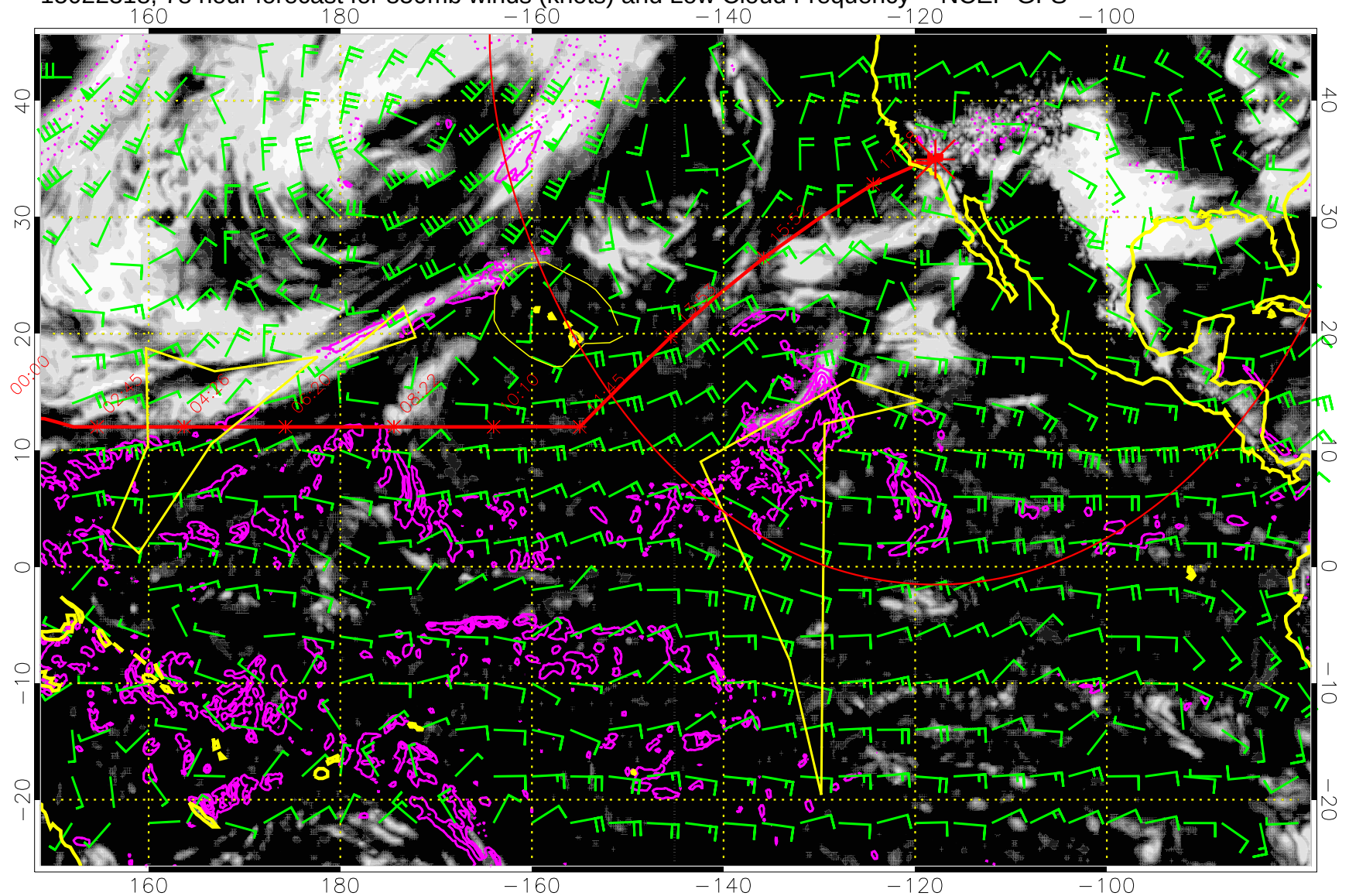
15022318, 78 hour forecast for 850mb winds (knots) and Low Cloud Frequency -- NCEP GFS
