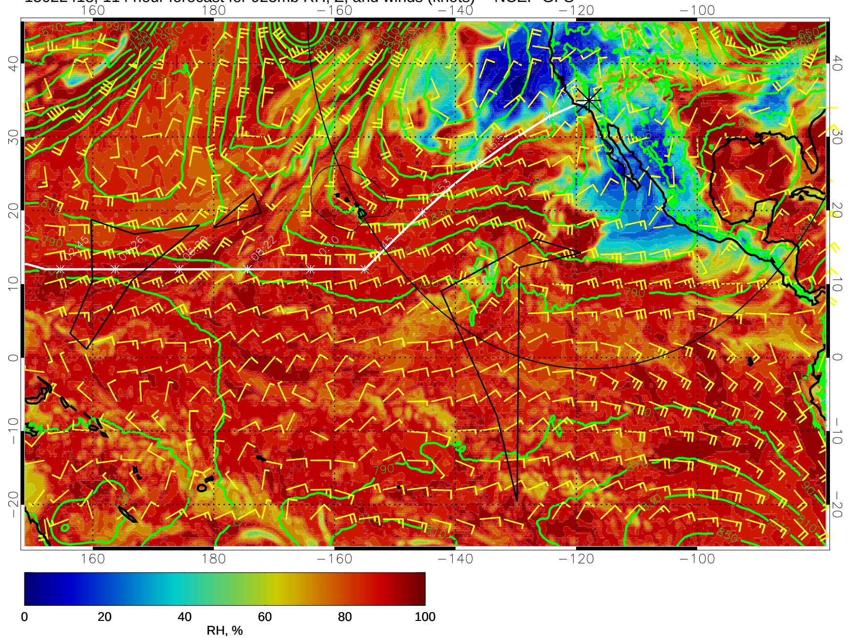
15022418, 114 hour forecast for 925mb RH, Z, and winds (knots) -- NCEP GFS
