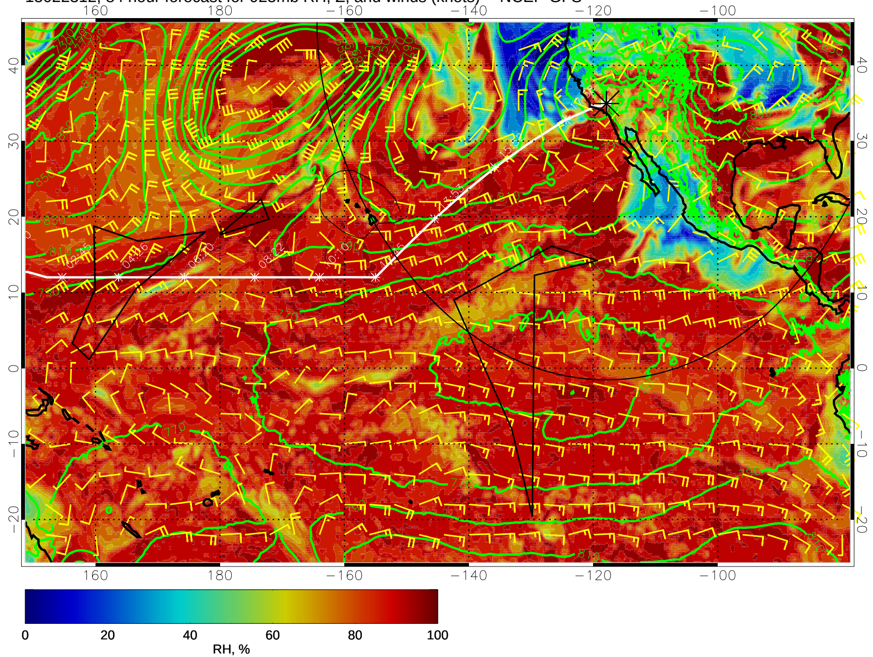
15022312, 84 hour forecast for 925mb RH, Z, and winds (knots) -- NCEP GFS
