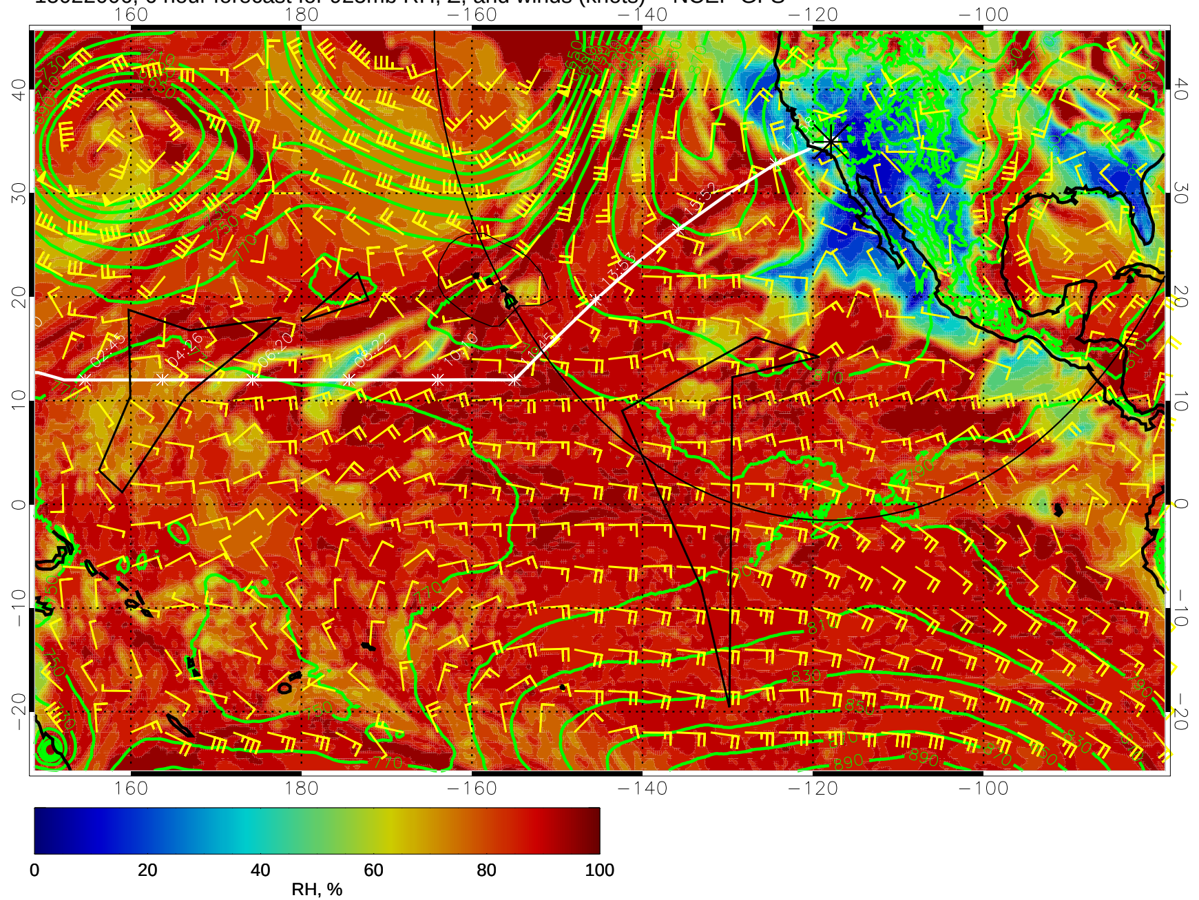
15022006, 6 hour forecast for 925mb RH, Z, and winds (knots) -- NCEP GFS
