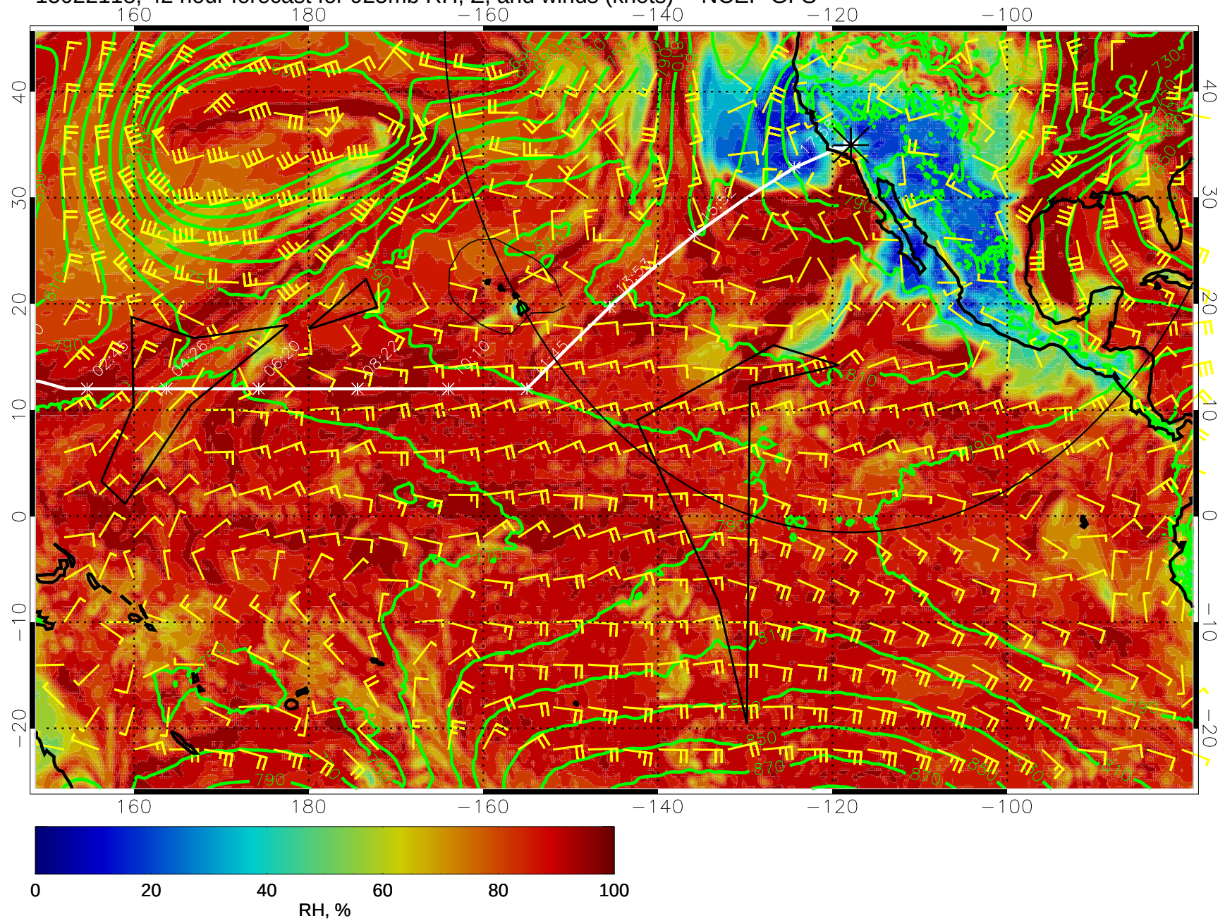
15022118, 42 hour forecast for 925mb RH, Z, and winds (knots) -- NCEP GFS
