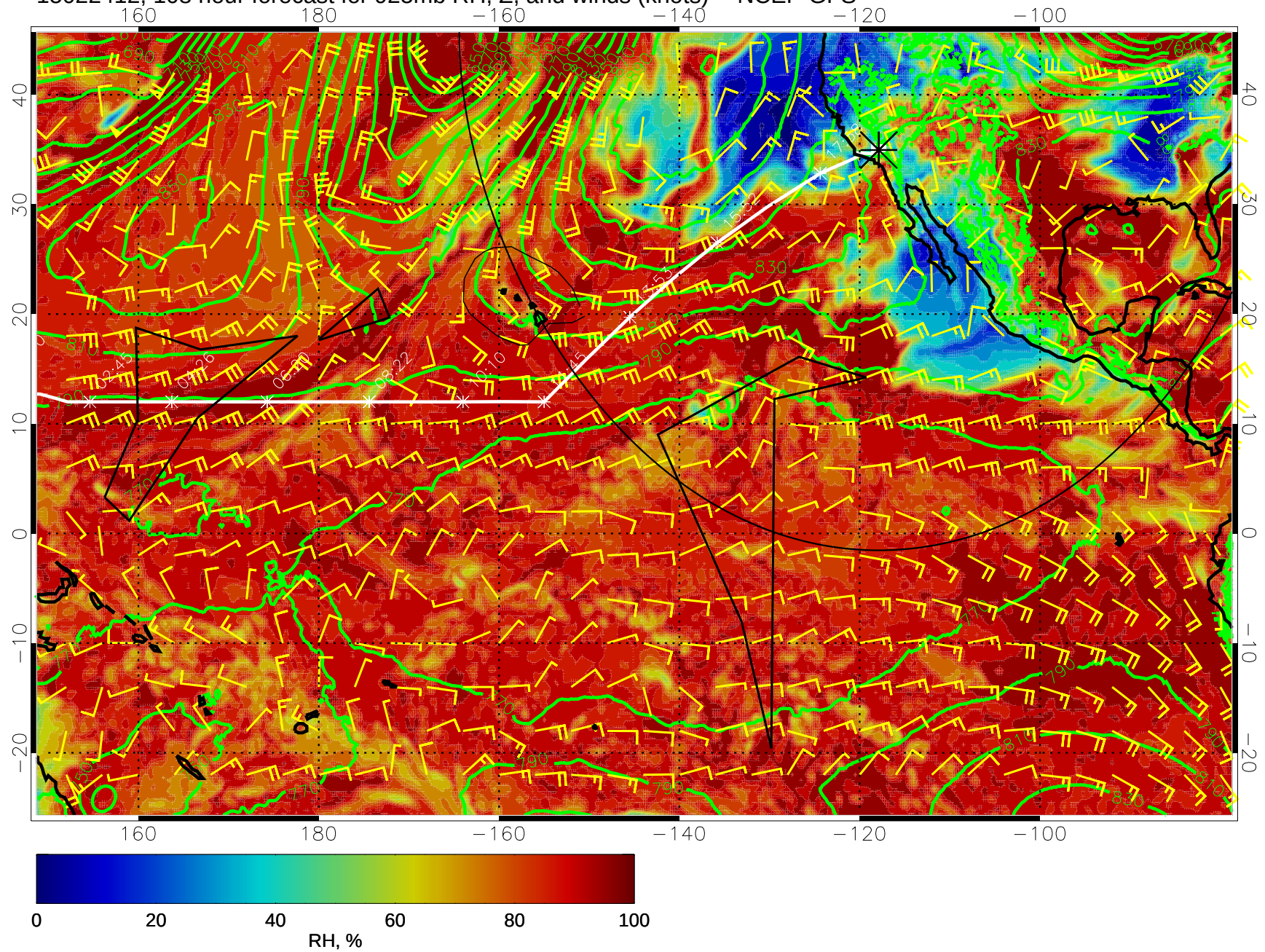
15022412, 108 hour forecast for 925mb RH, Z, and winds (knots) -- NCEP GFS
