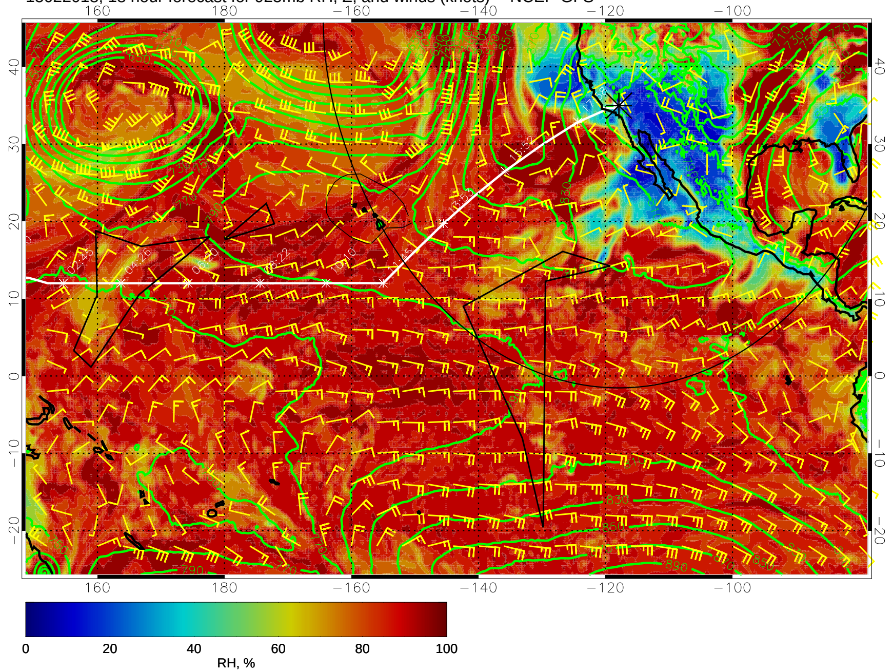
15022018, 18 hour forecast for 925mb RH, Z, and winds (knots) -- NCEP GFS
