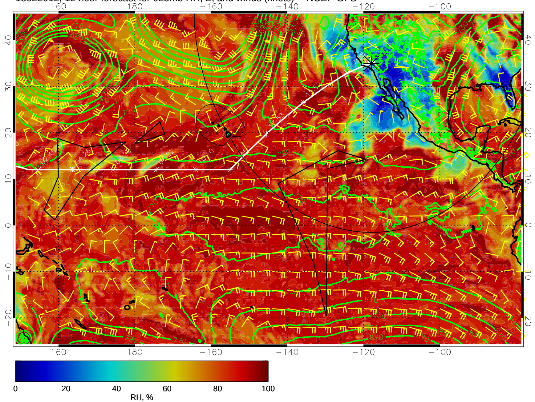
15022012, 12 hour forecast for 925mb RH, Z, and winds (knots) -- NCEP GFS
