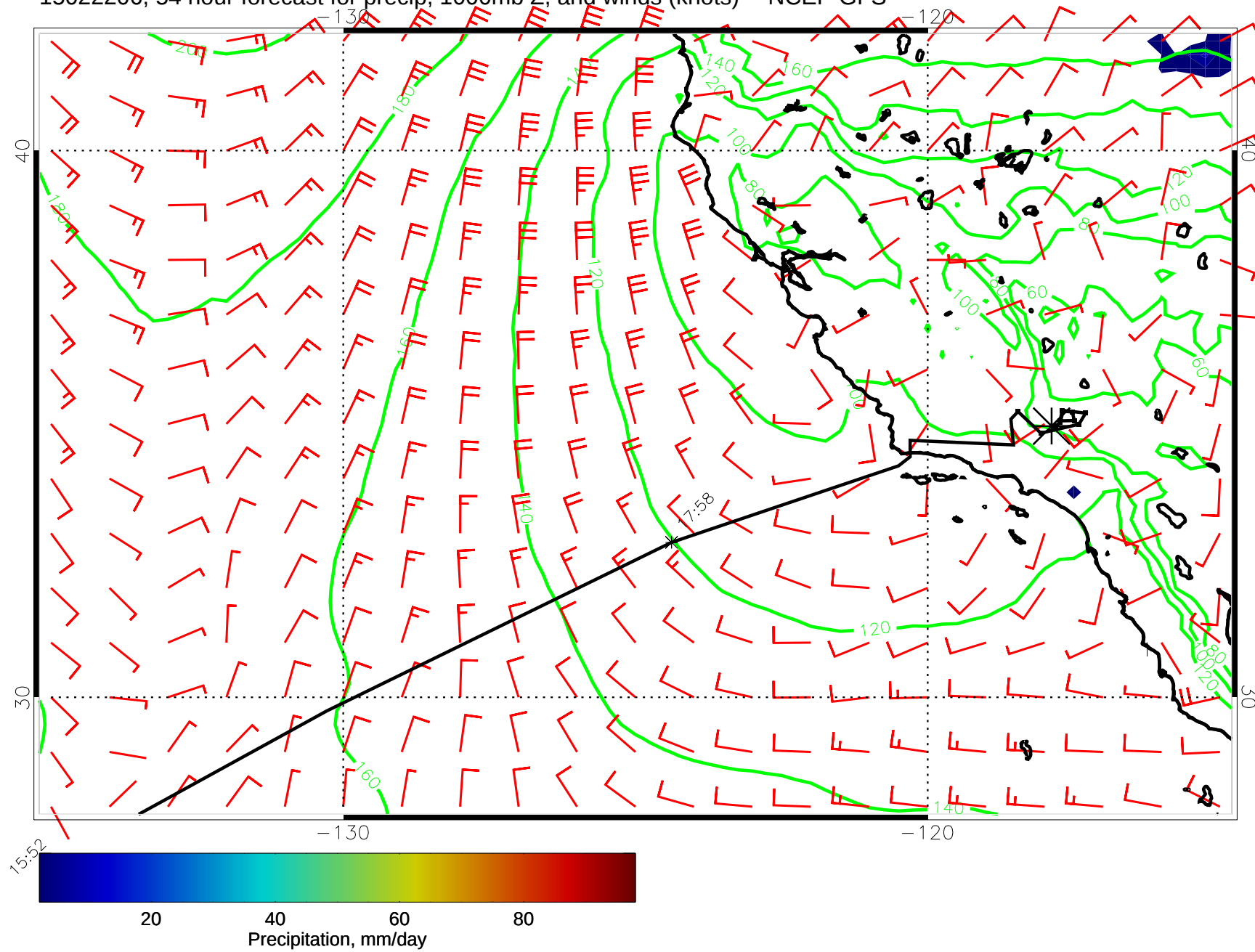
15022206, 54 hour forecast for precip, 1000mb Z, and winds (knots) -- NCEP GFS
