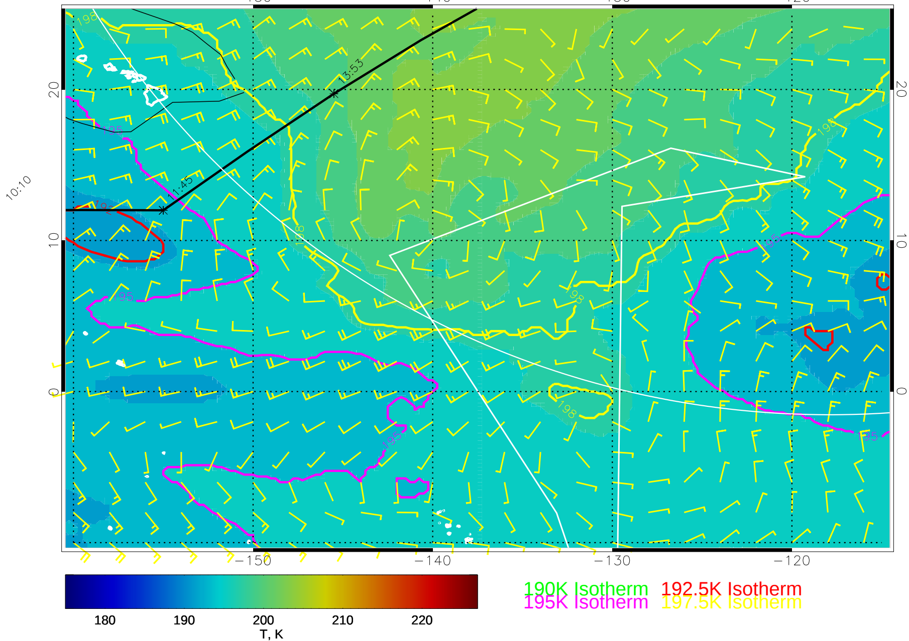
15022406, 102 hour forecast for 70mb T and winds (knots) -- NCEP GFS
