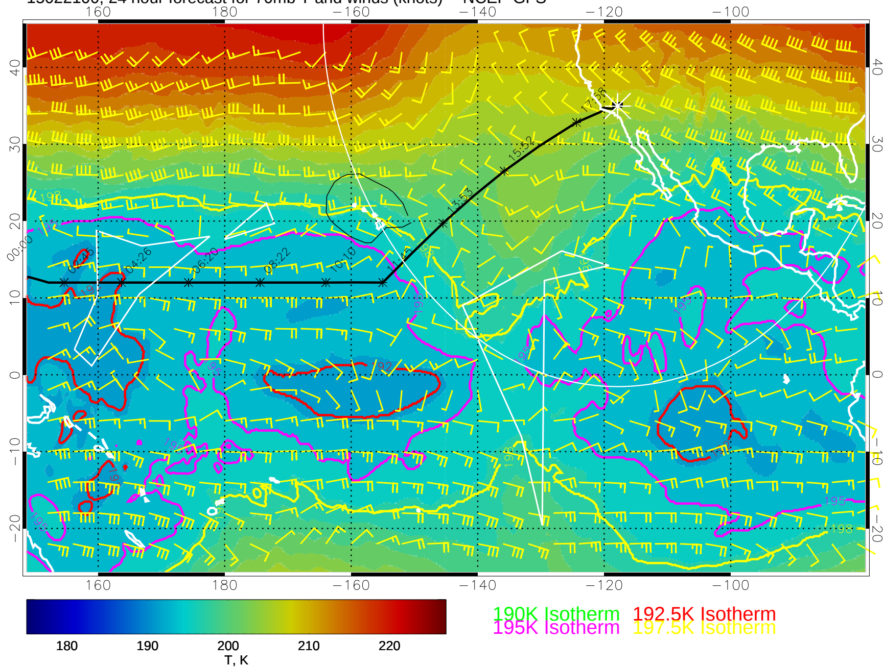
15022100, 24 hour forecast for 70mb T and winds (knots) -- NCEP GFS
