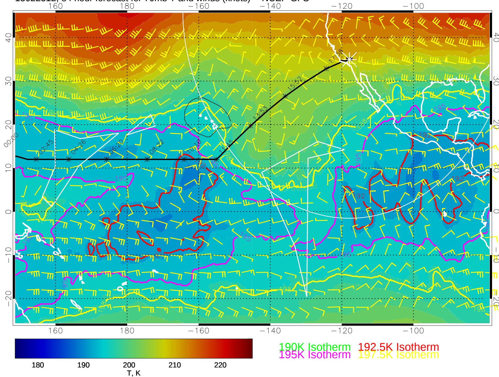
15022312, 84 hour forecast for 70mb T and winds (knots) -- NCEP GFS
