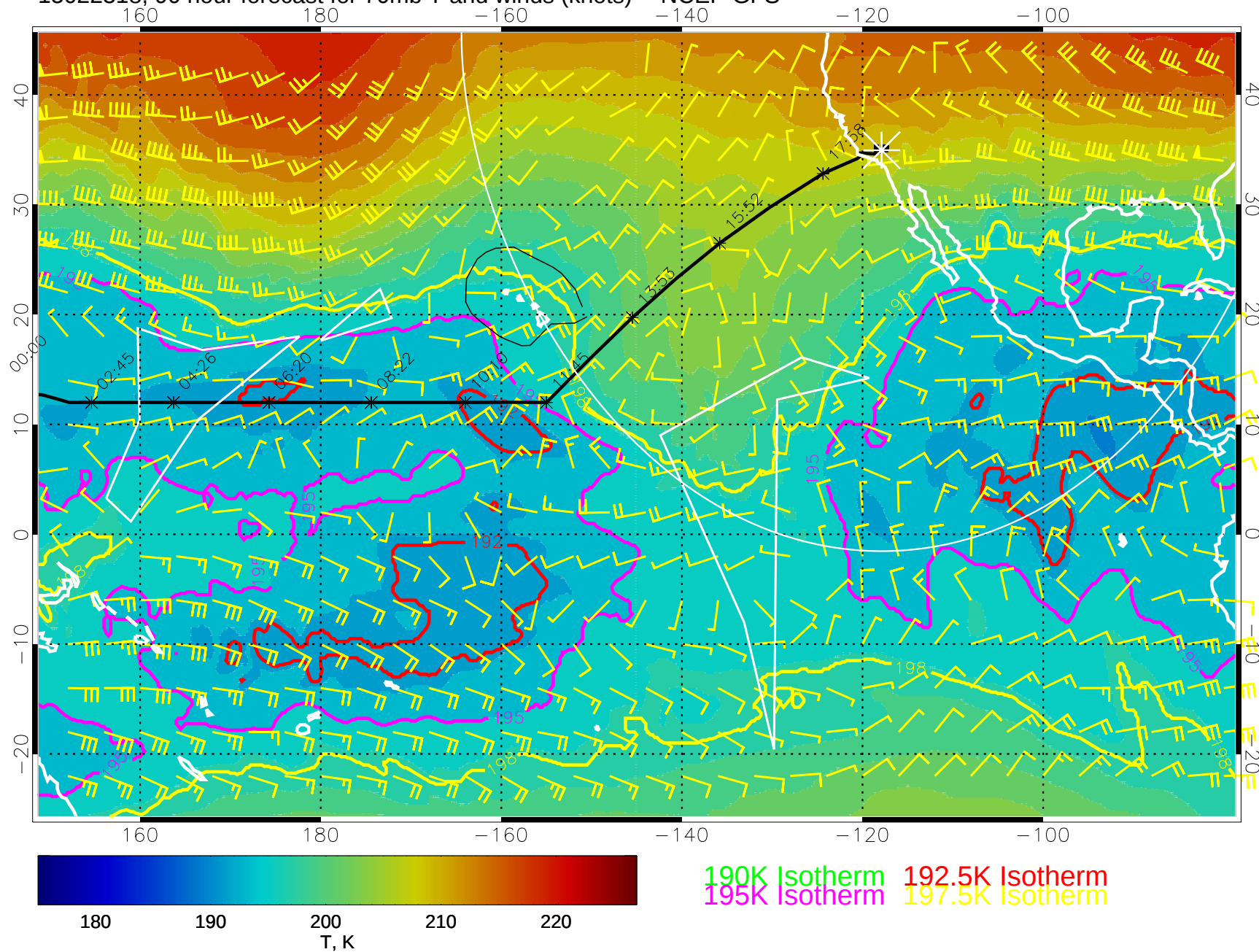
15022318, 90 hour forecast for 70mb T and winds (knots) -- NCEP GFS
