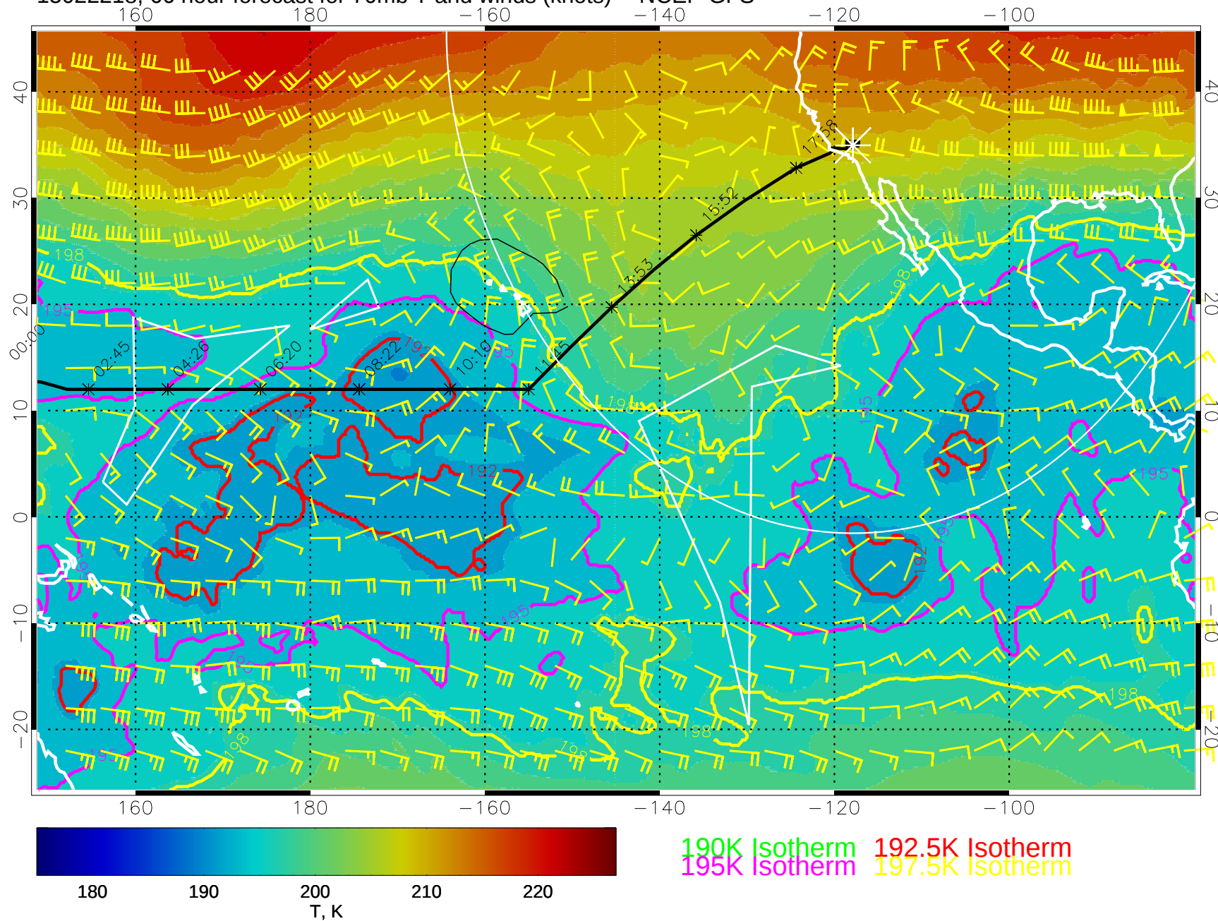
15022218, 66 hour forecast for 70mb T and winds (knots) -- NCEP GFS
