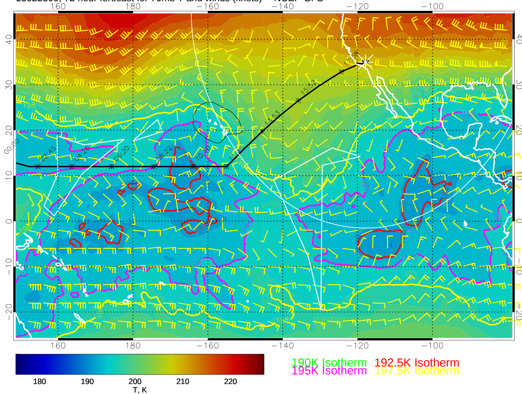
15022300, 72 hour forecast for 70mb T and winds (knots) -- NCEP GFS
