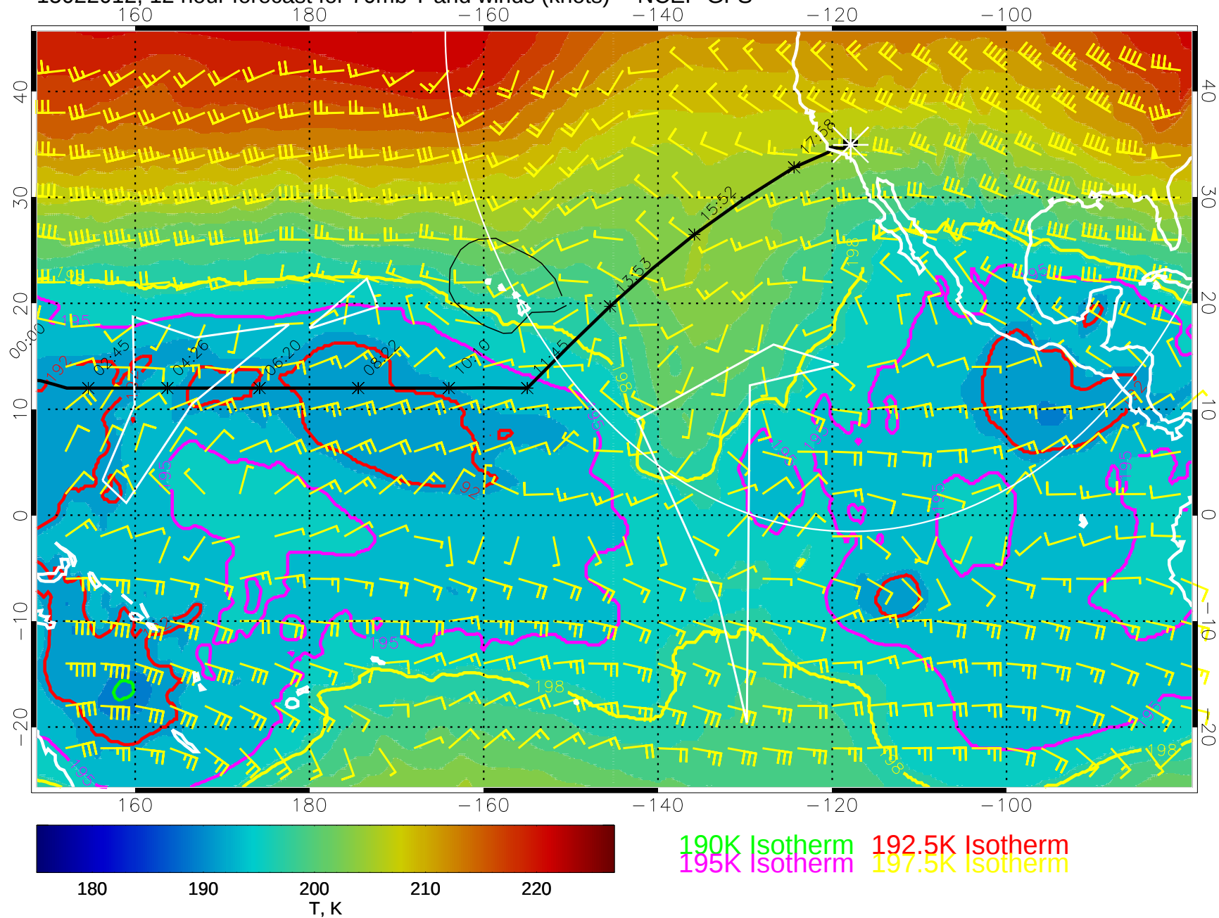
15022012, 12 hour forecast for 70mb T and winds (knots) -- NCEP GFS
