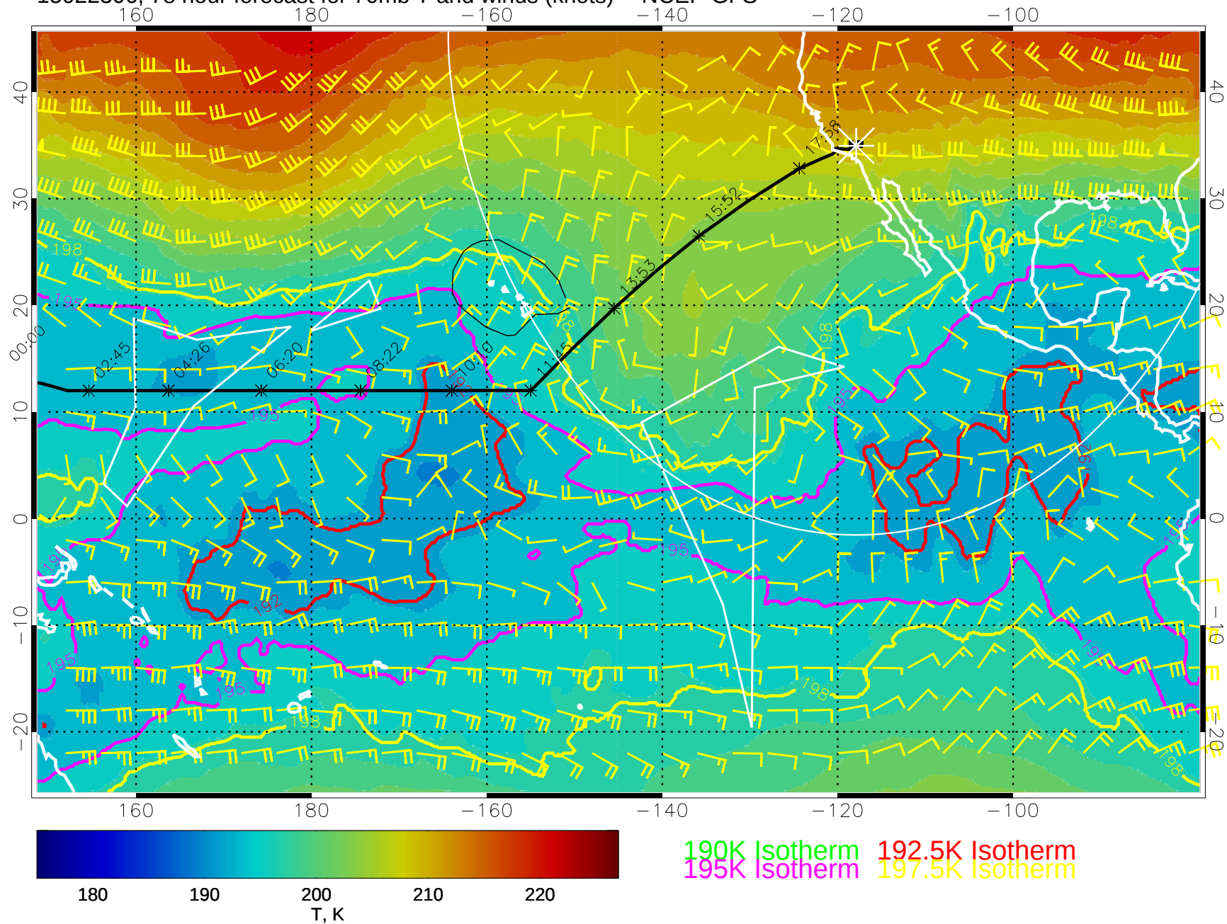
15022306, 78 hour forecast for 70mb T and winds (knots) -- NCEP GFS
