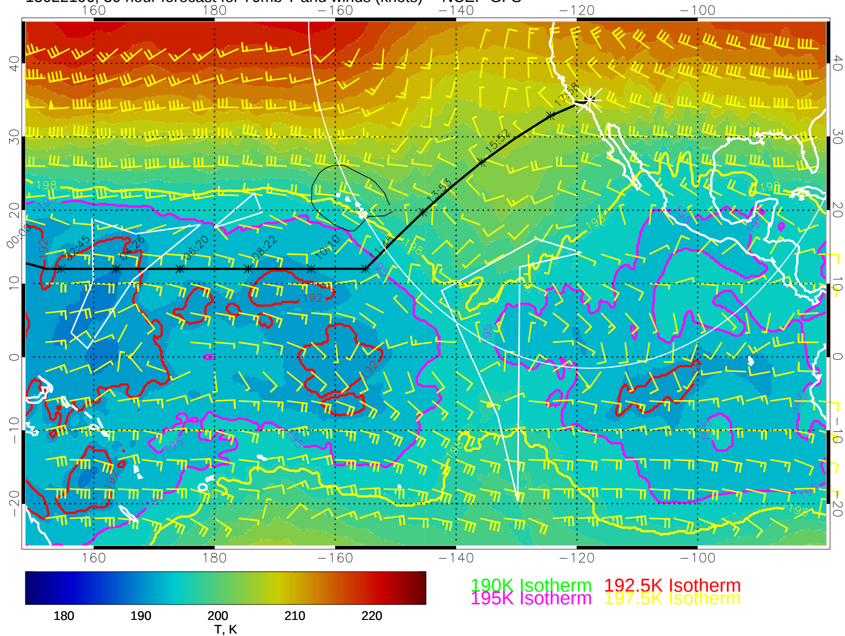
15022106, 30 hour forecast for 70mb T and winds (knots) -- NCEP GFS
