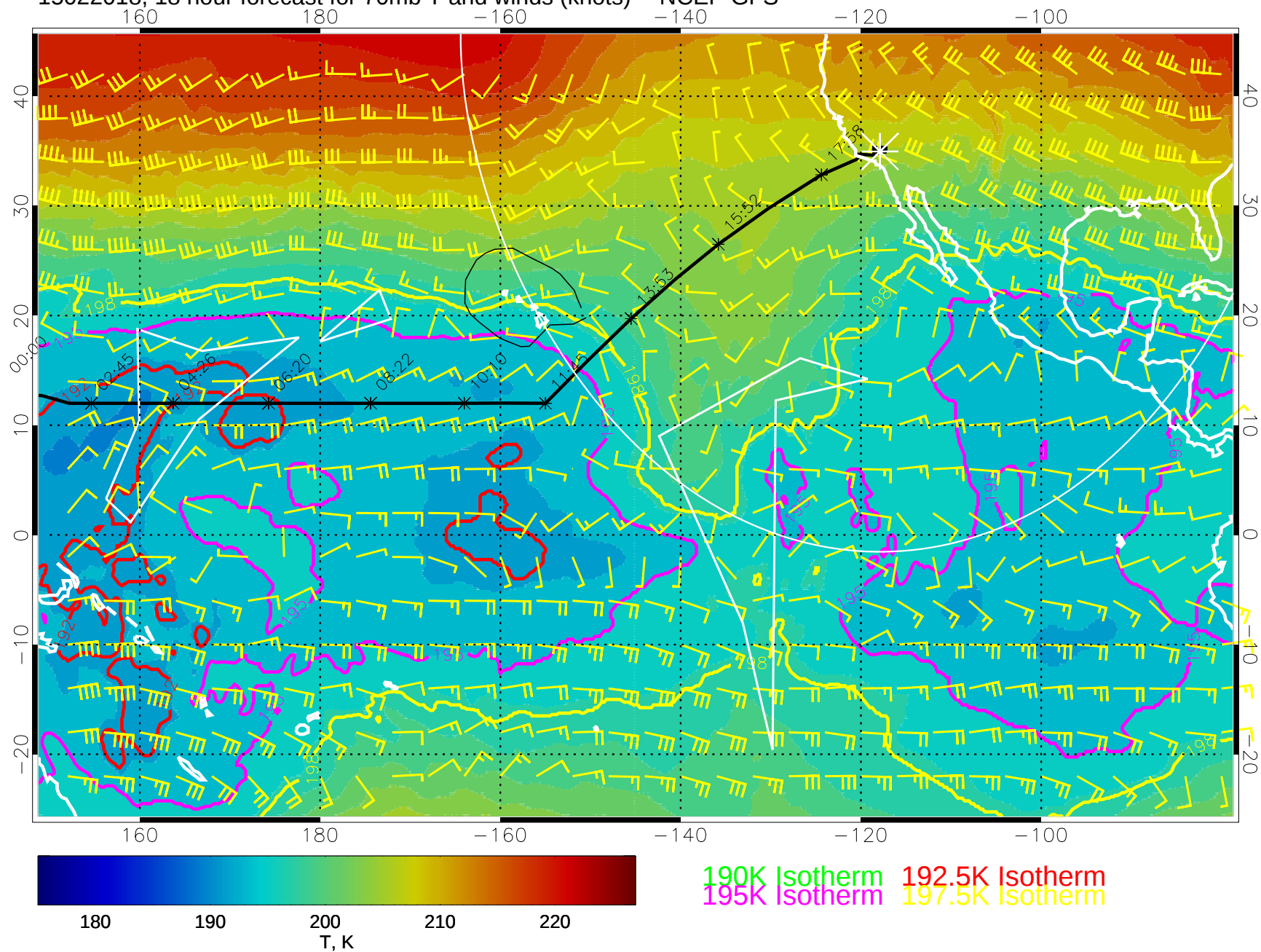
15022018, 18 hour forecast for 70mb T and winds (knots) -- NCEP GFS
