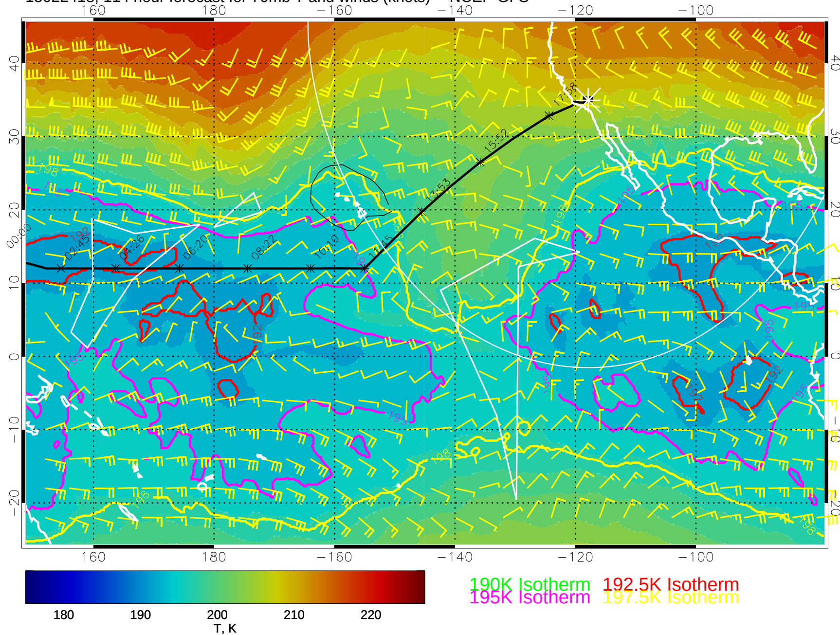
15022418, 114 hour forecast for 70mb T and winds (knots) -- NCEP GFS
