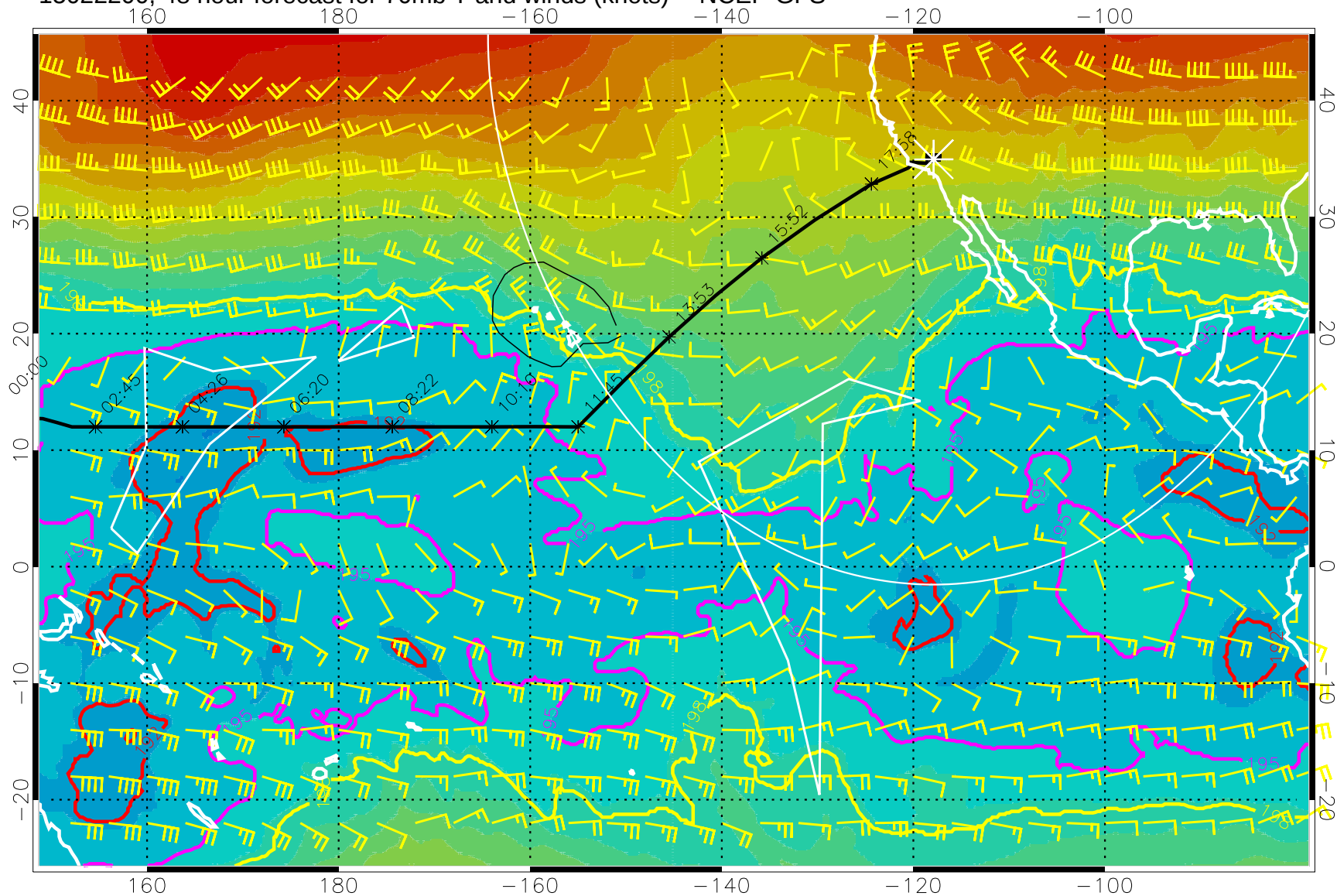
15022200, 48 hour forecast for 70mb T and winds (knots) -- NCEP GFS
