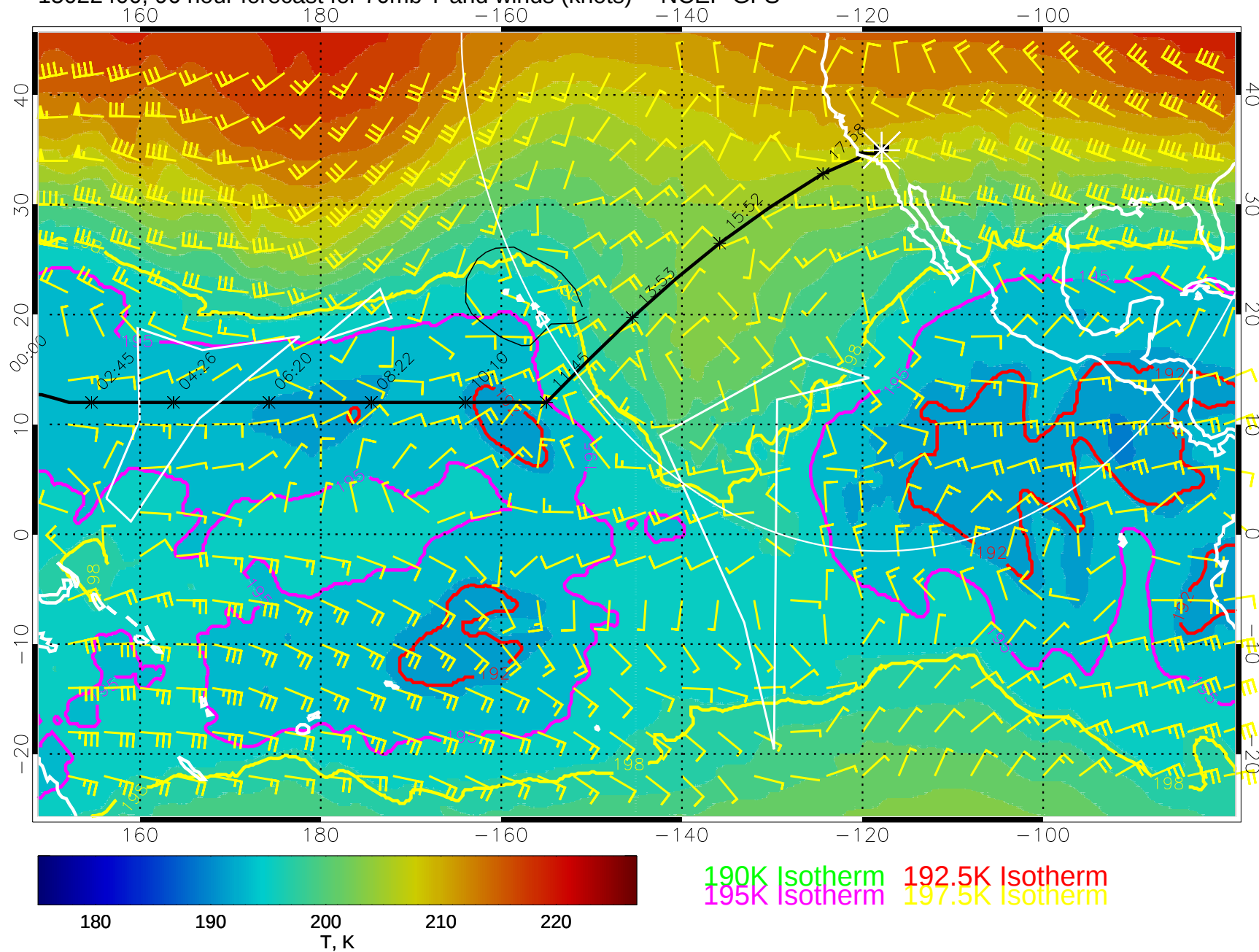
15022400, 96 hour forecast for 70mb T and winds (knots) -- NCEP GFS
