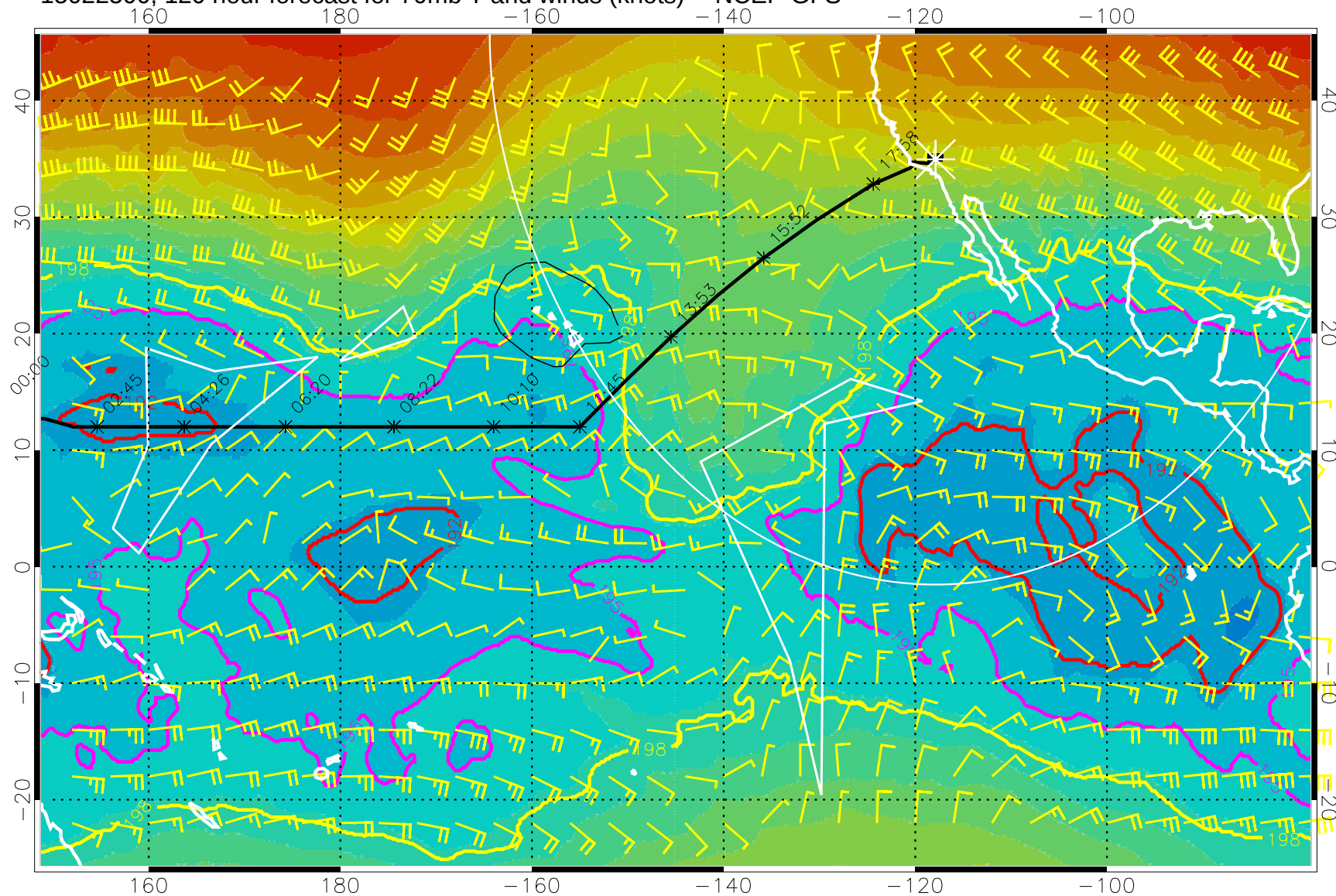
15022500, 120 hour forecast for 70mb T and winds (knots) -- NCEP GFS
