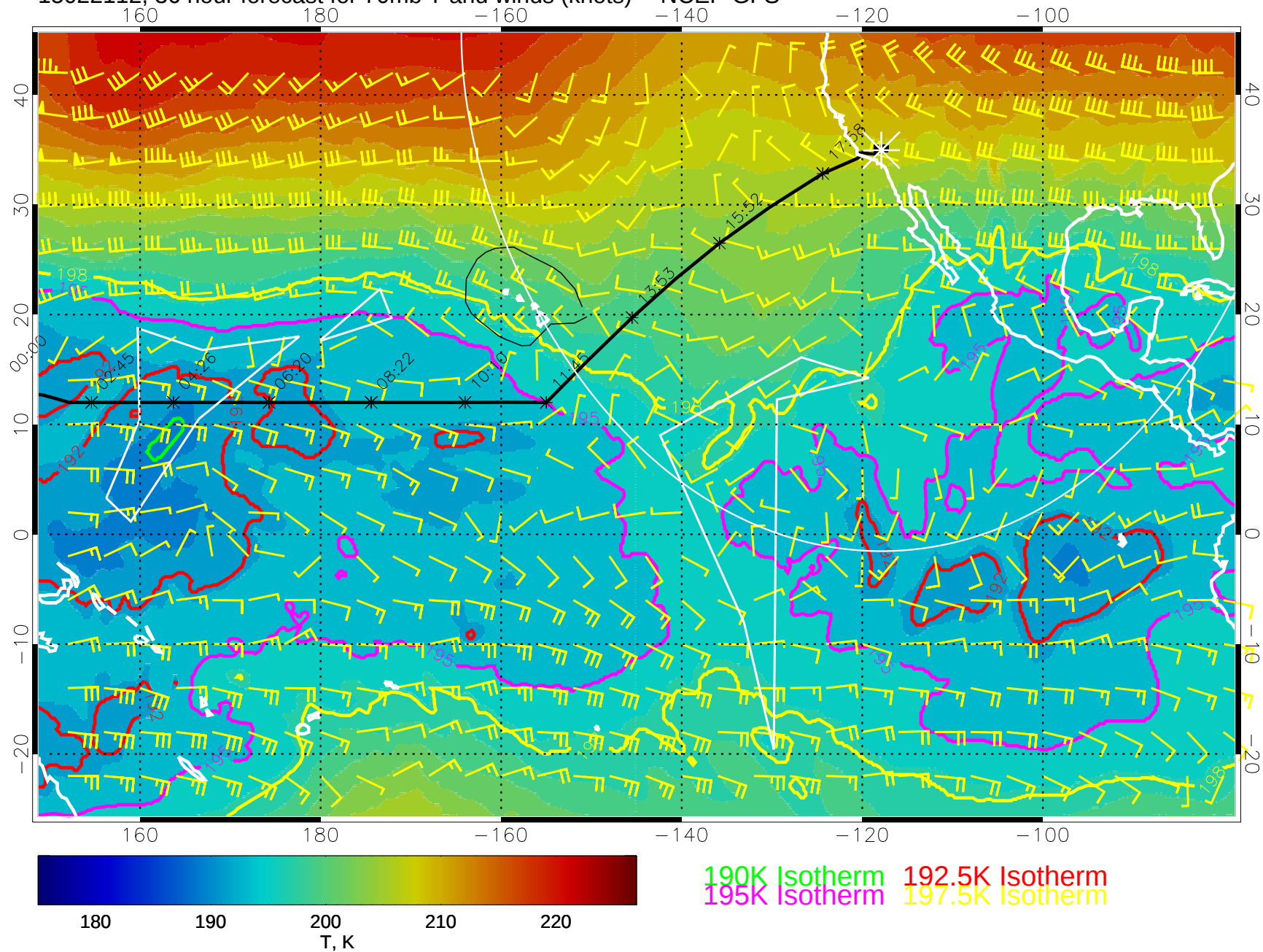
15022112, 36 hour forecast for 70mb T and winds (knots) -- NCEP GFS
