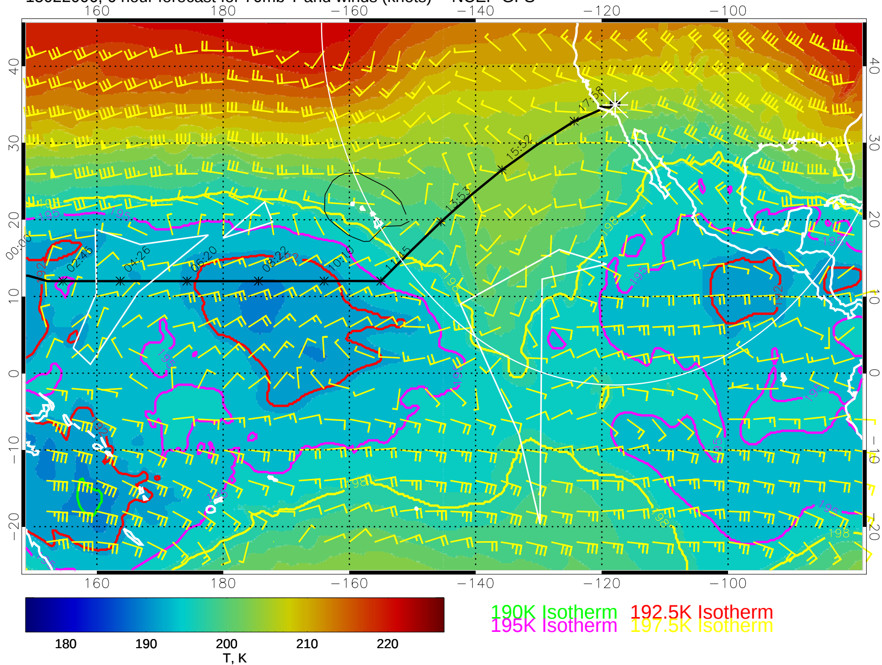
15022006, 6 hour forecast for 70mb T and winds (knots) -- NCEP GFS
