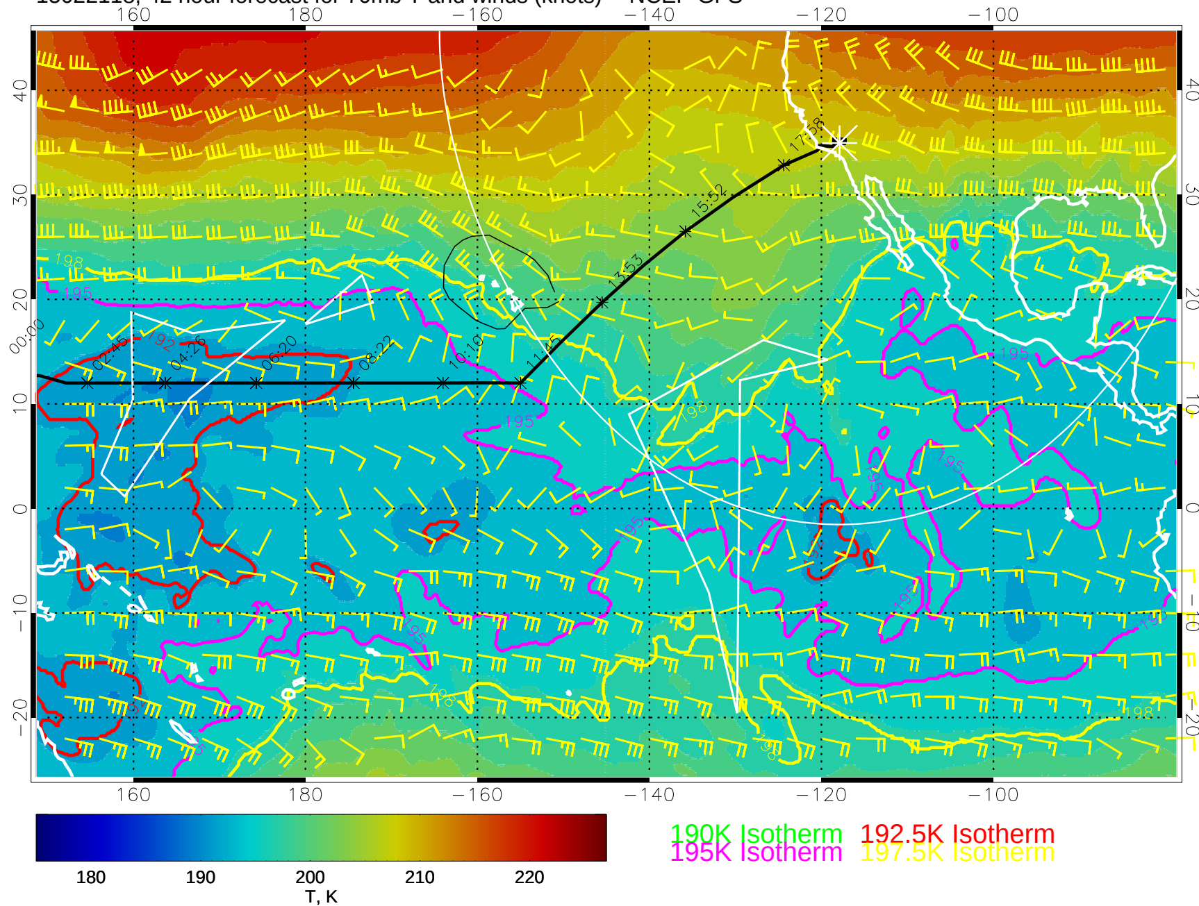
15022118, 42 hour forecast for 70mb T and winds (knots) -- NCEP GFS
