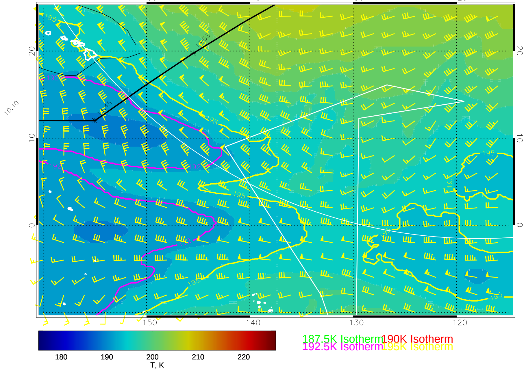
15022212, 60 hour forecast for 100mb T and winds (knots) -- NCEP GFS
