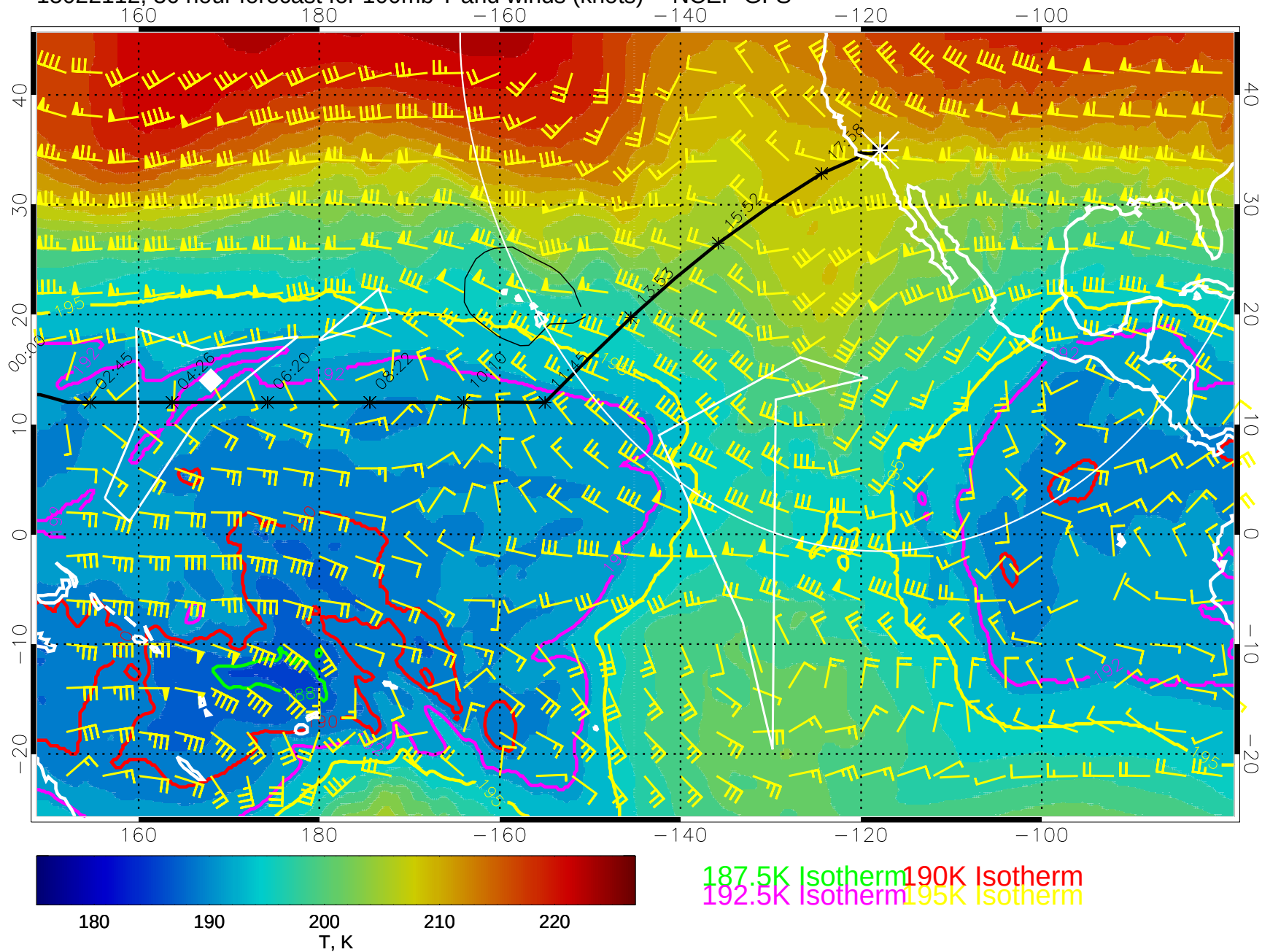
15022112, 36 hour forecast for 100mb T and winds (knots) -- NCEP GFS
