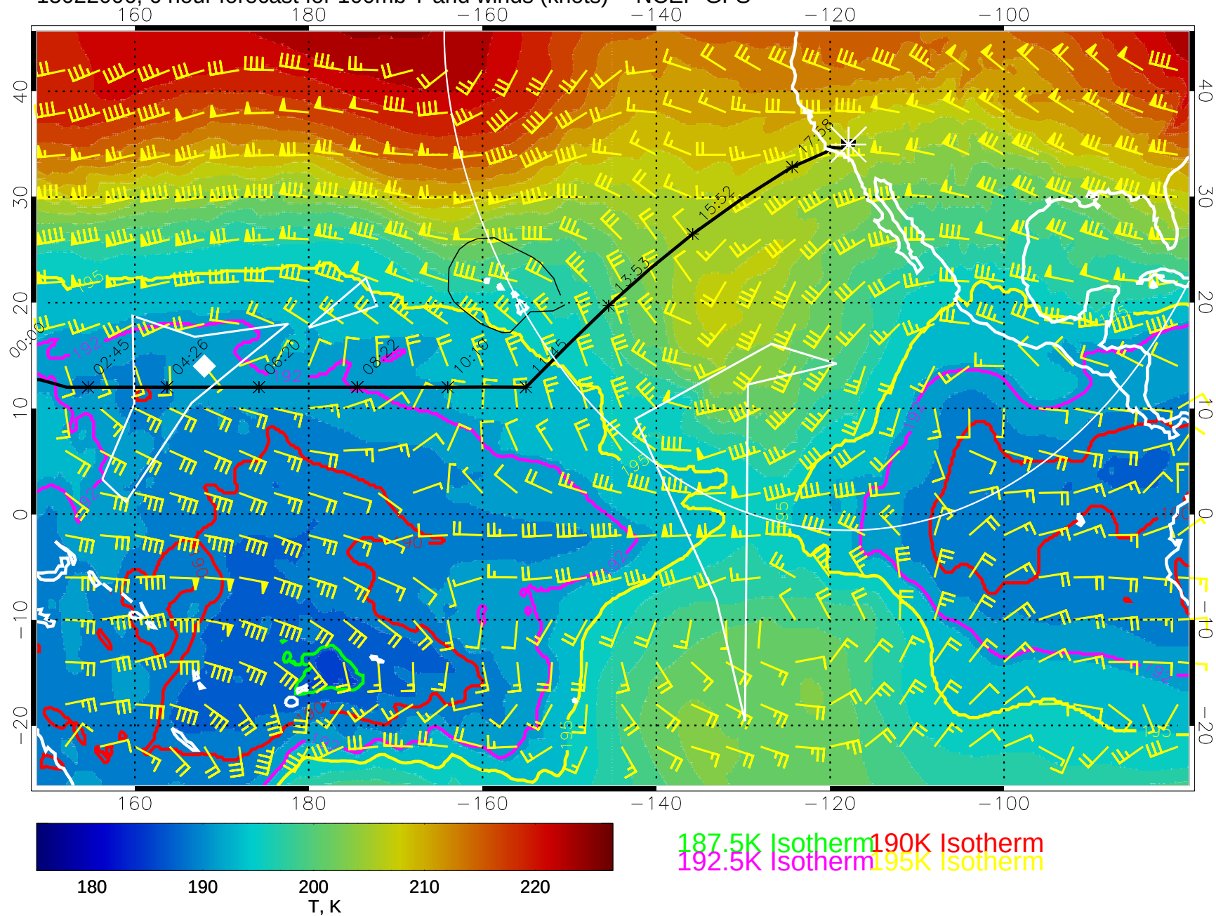
15022006, 6 hour forecast for 100mb T and winds (knots) -- NCEP GFS
