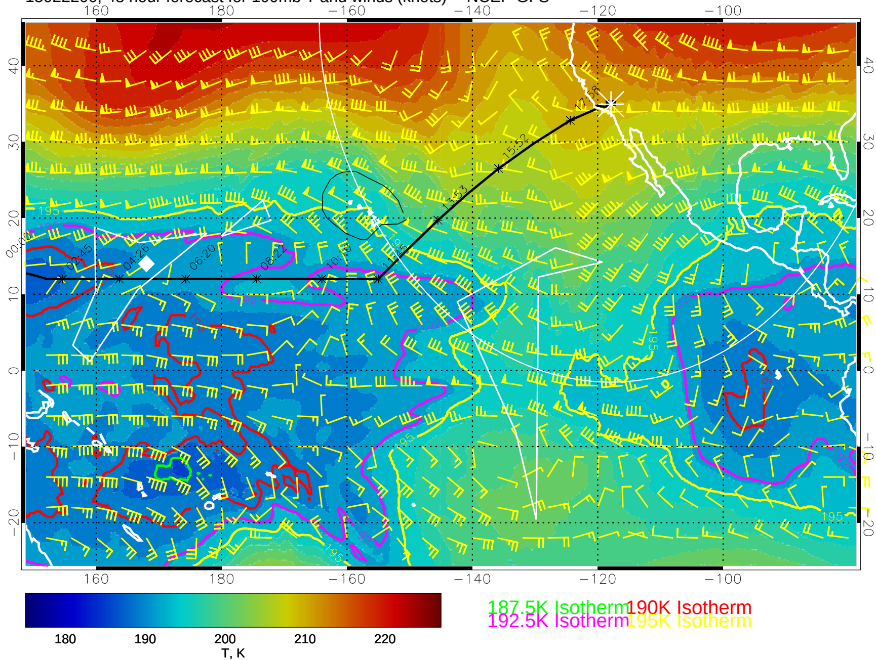
15022200, 48 hour forecast for 100mb T and winds (knots) -- NCEP GFS
