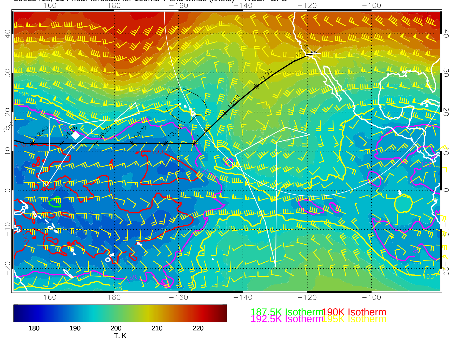
15022418, 114 hour forecast for 100mb T and winds (knots) -- NCEP GFS
