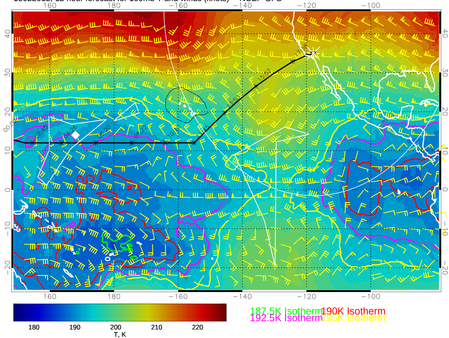
15022012, 12 hour forecast for 100mb T and winds (knots) -- NCEP GFS
