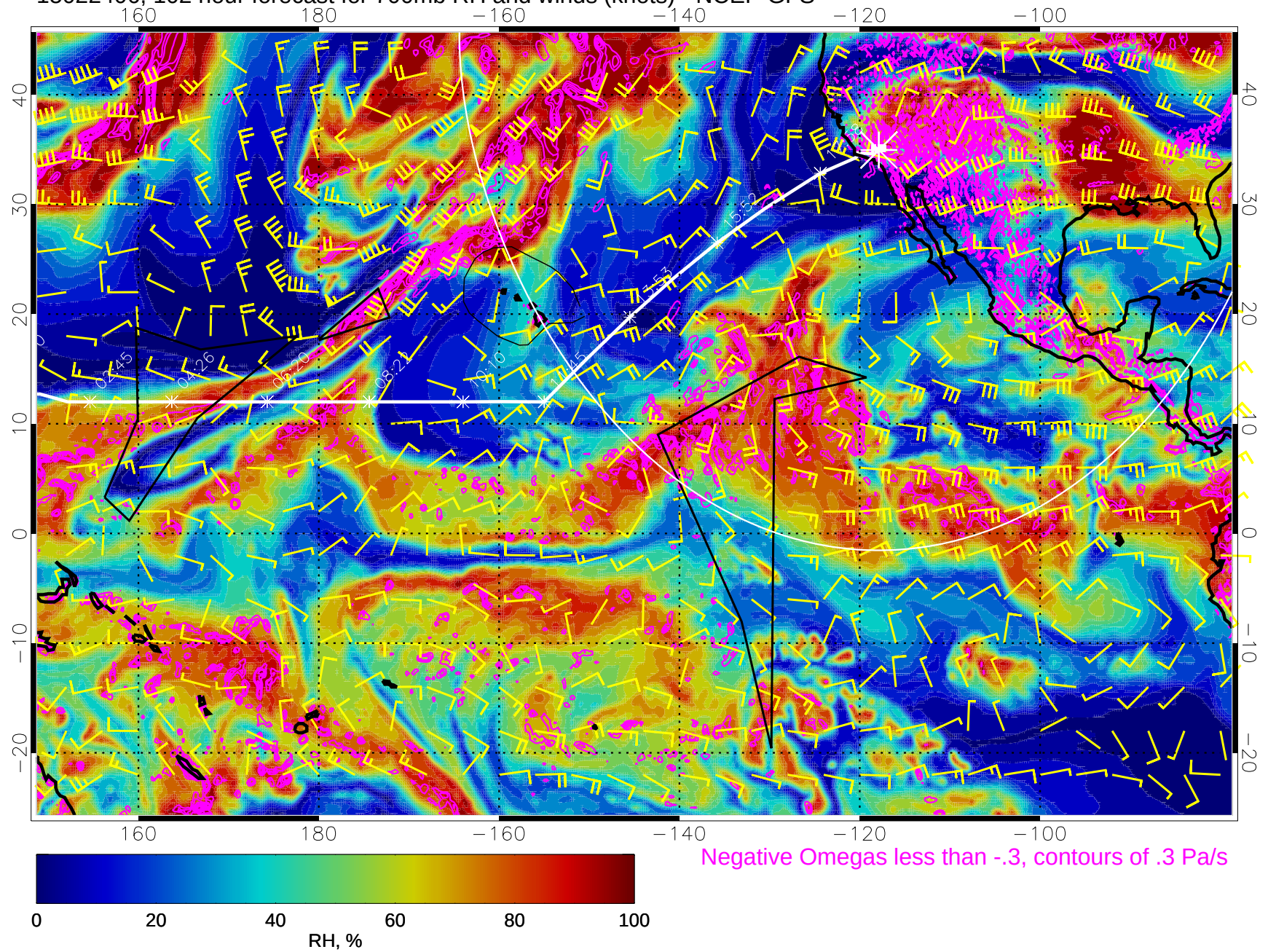
15022406, 102 hour forecast for 700mb RH and winds (knots) - NCEP GFS
