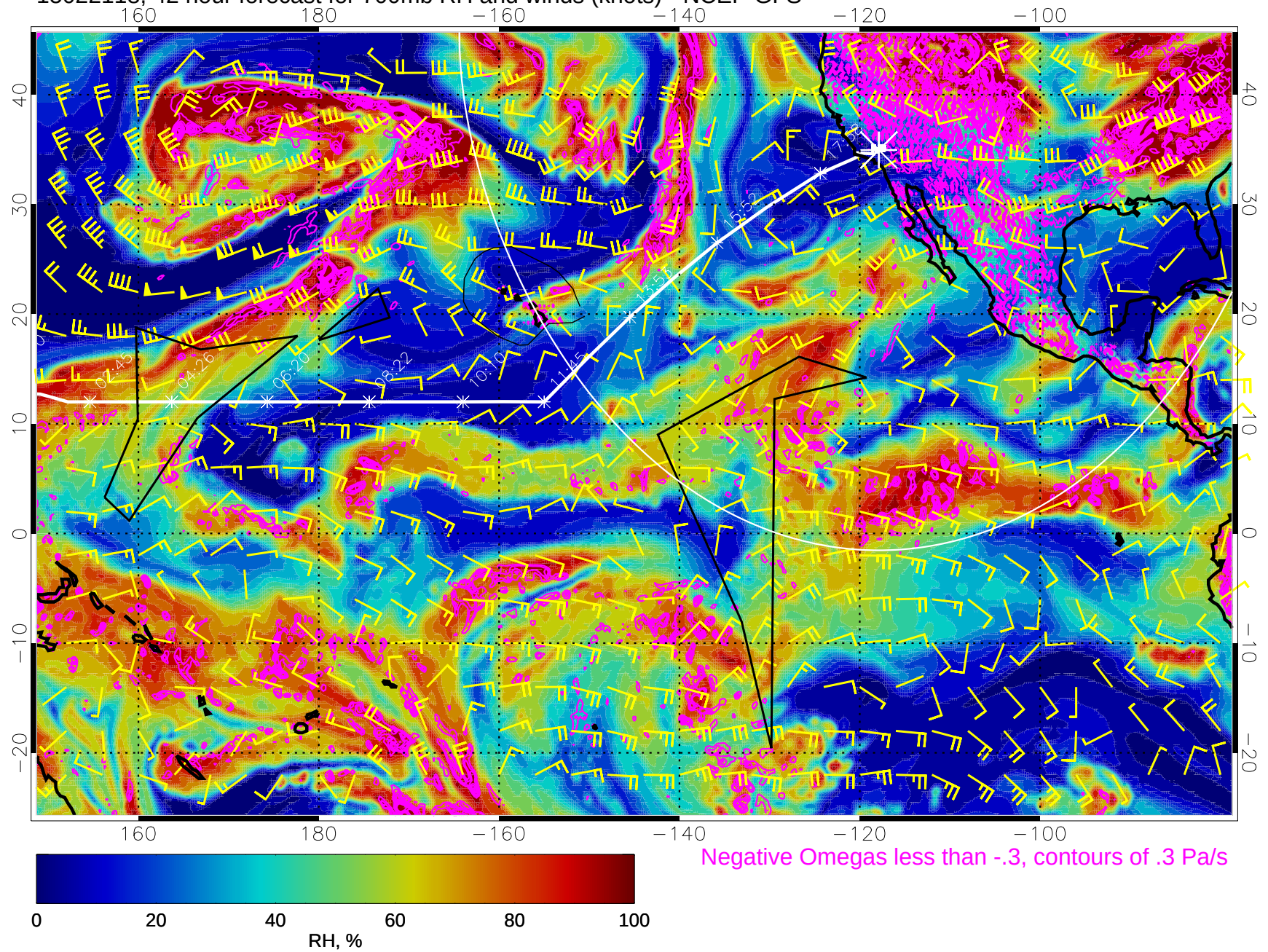
15022118, 42 hour forecast for 700mb RH and winds (knots) - NCEP GFS
