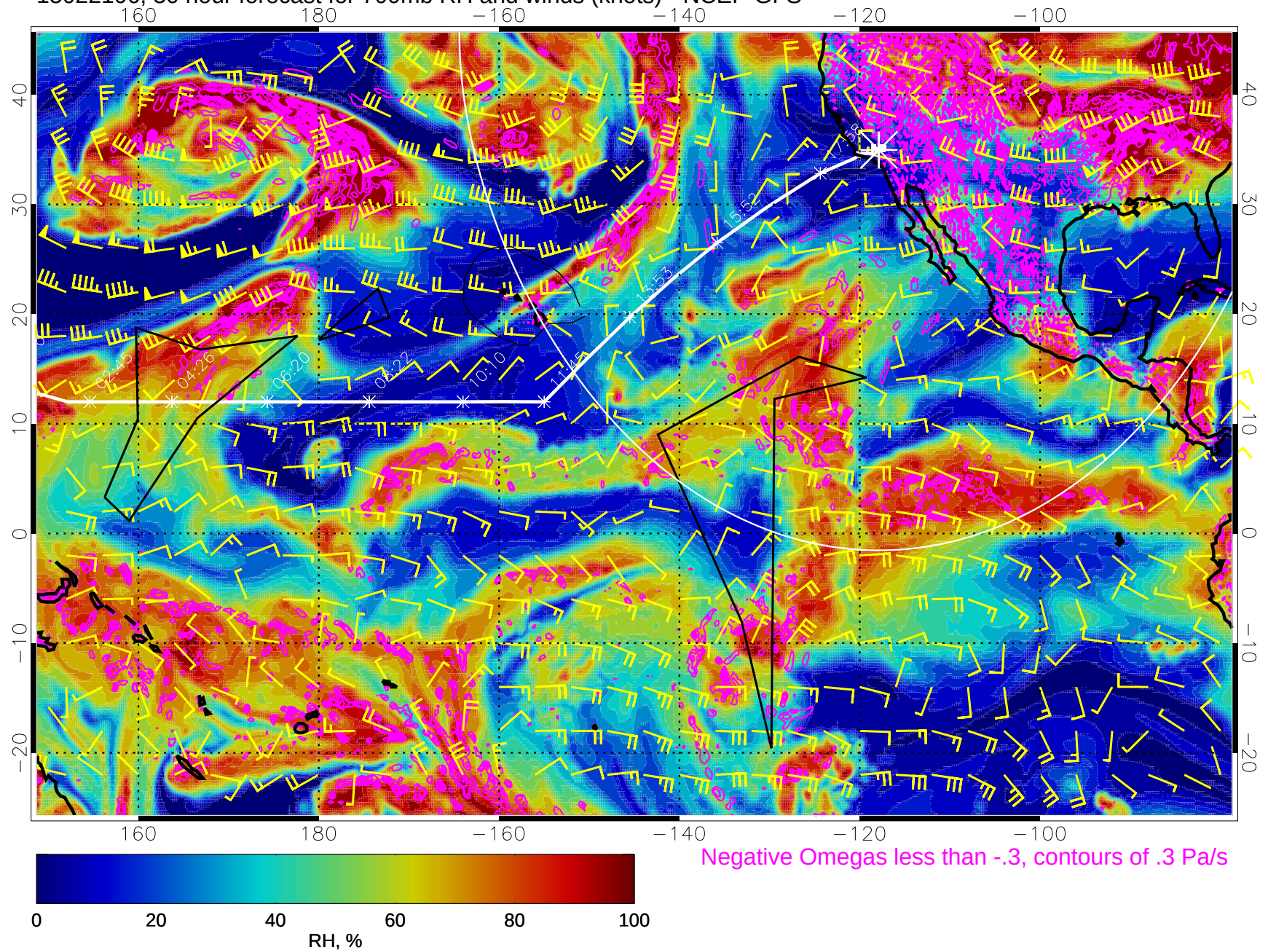
15022106, 30 hour forecast for 700mb RH and winds (knots) - NCEP GFS
