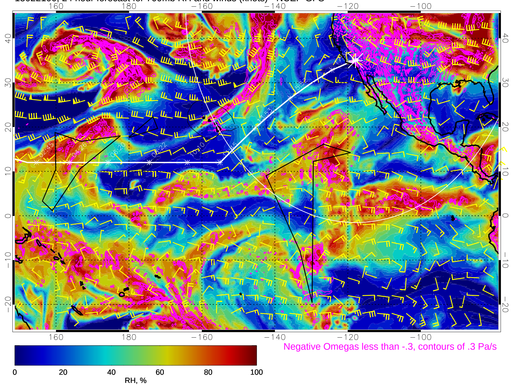
15022100, 24 hour forecast for 700mb RH and winds (knots) - NCEP GFS
