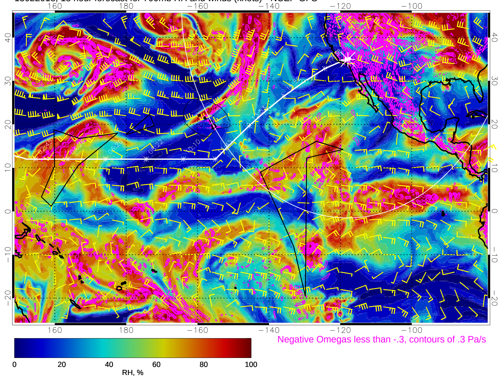
15022018, 18 hour forecast for 700mb RH and winds (knots) - NCEP GFS
