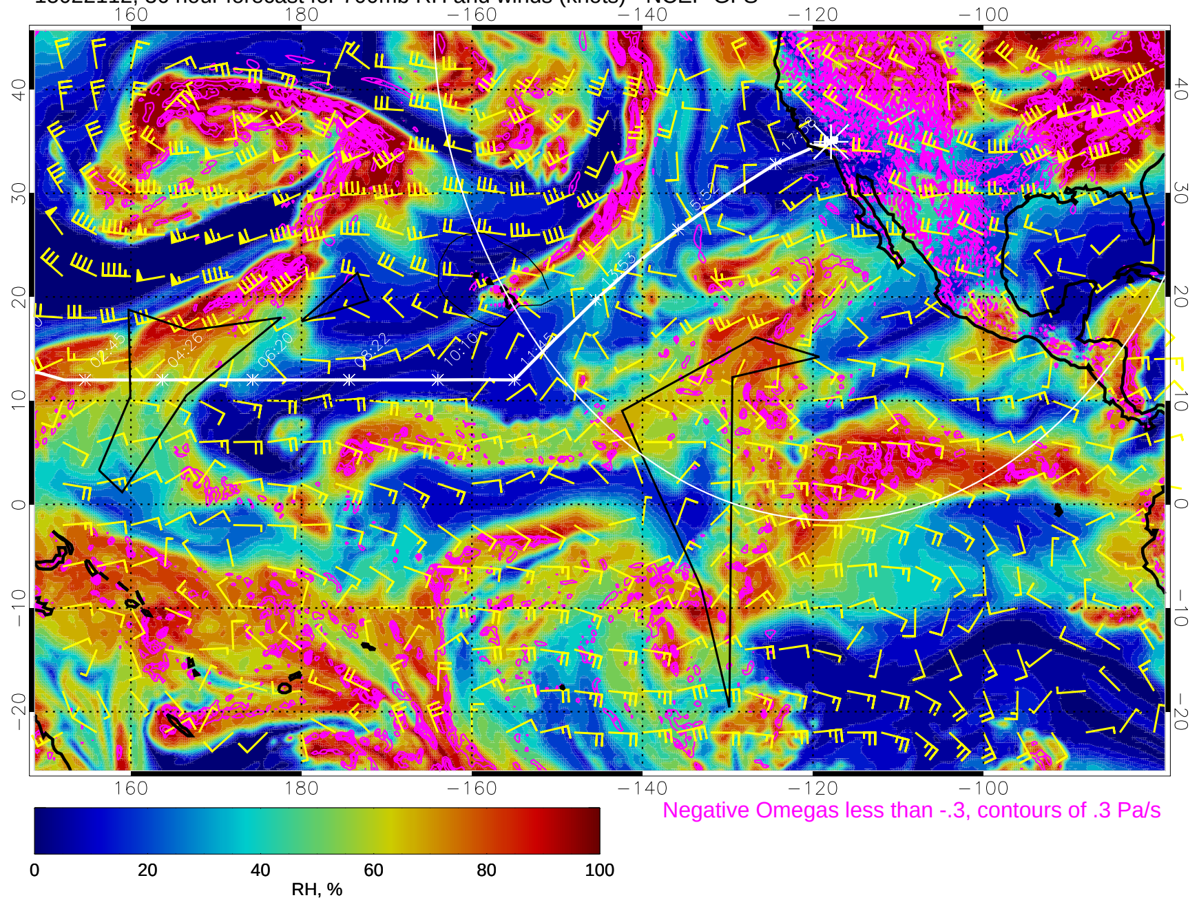
15022112, 36 hour forecast for 700mb RH and winds (knots) - NCEP GFS
