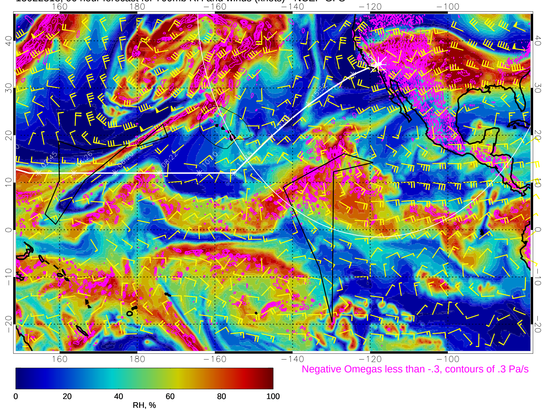
15022318, 90 hour forecast for 700mb RH and winds (knots) - NCEP GFS
