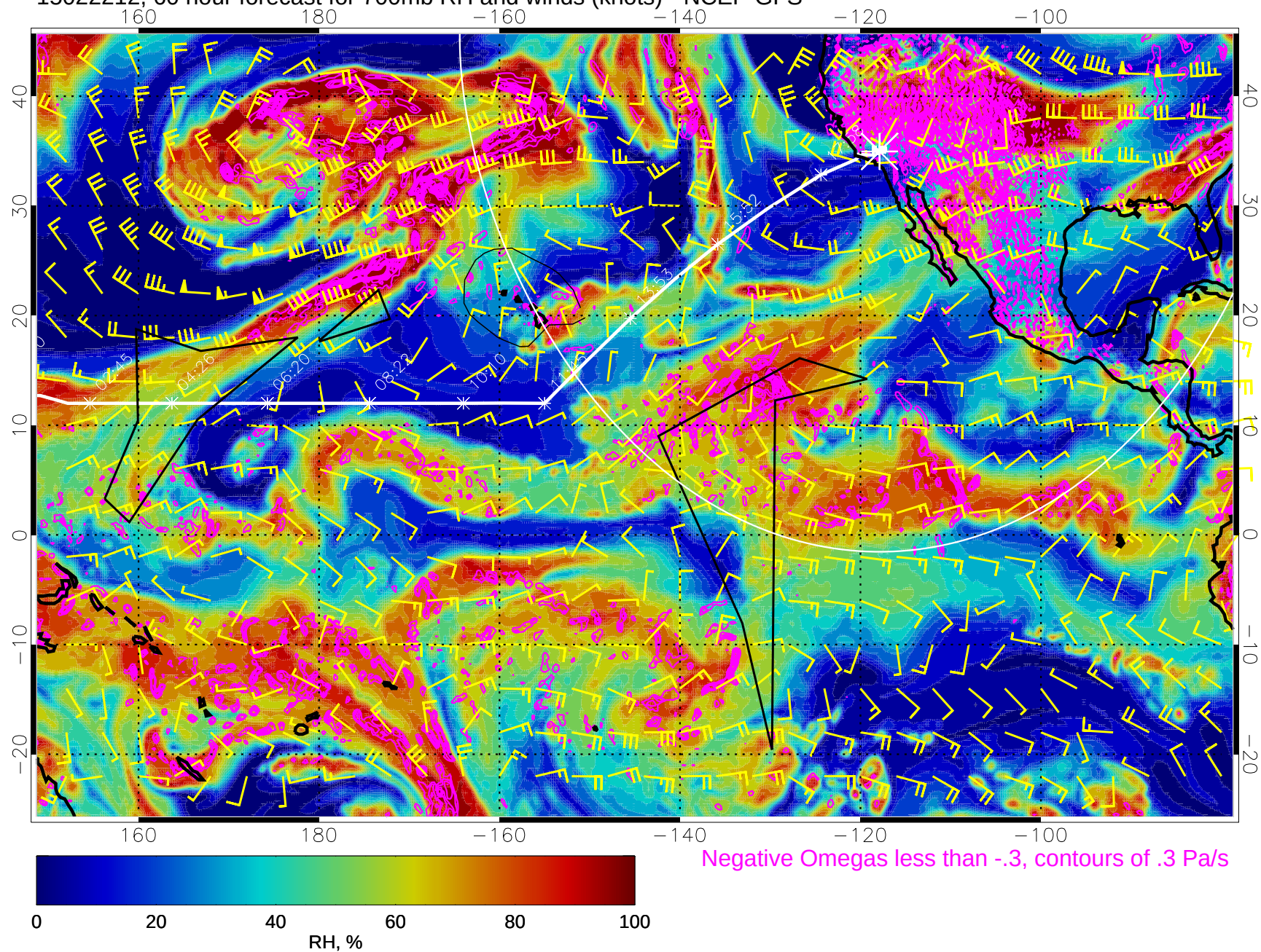
15022212, 60 hour forecast for 700mb RH and winds (knots) - NCEP GFS
