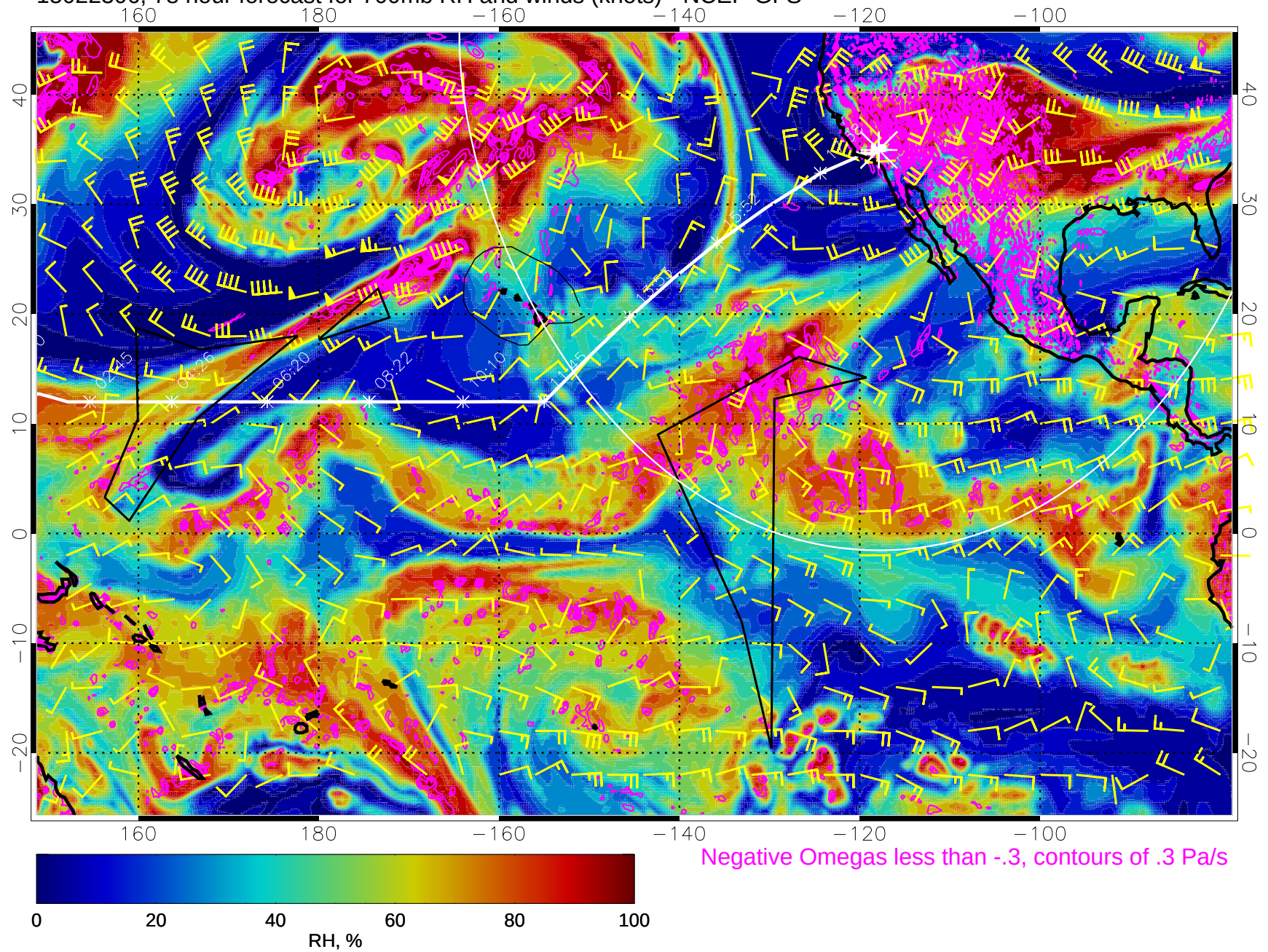
15022306, 78 hour forecast for 700mb RH and winds (knots) - NCEP GFS
