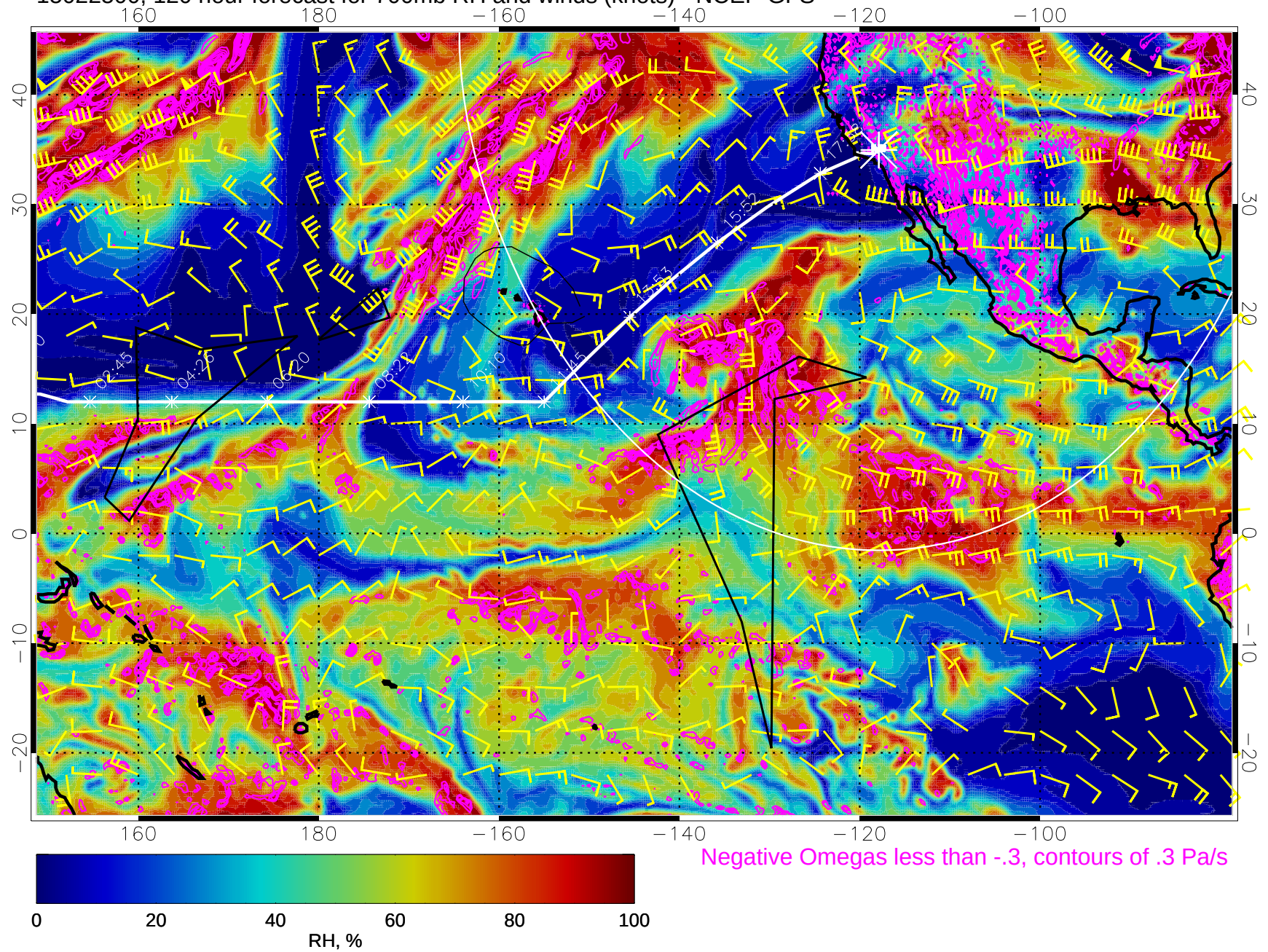
15022500, 120 hour forecast for 700mb RH and winds (knots) - NCEP GFS
