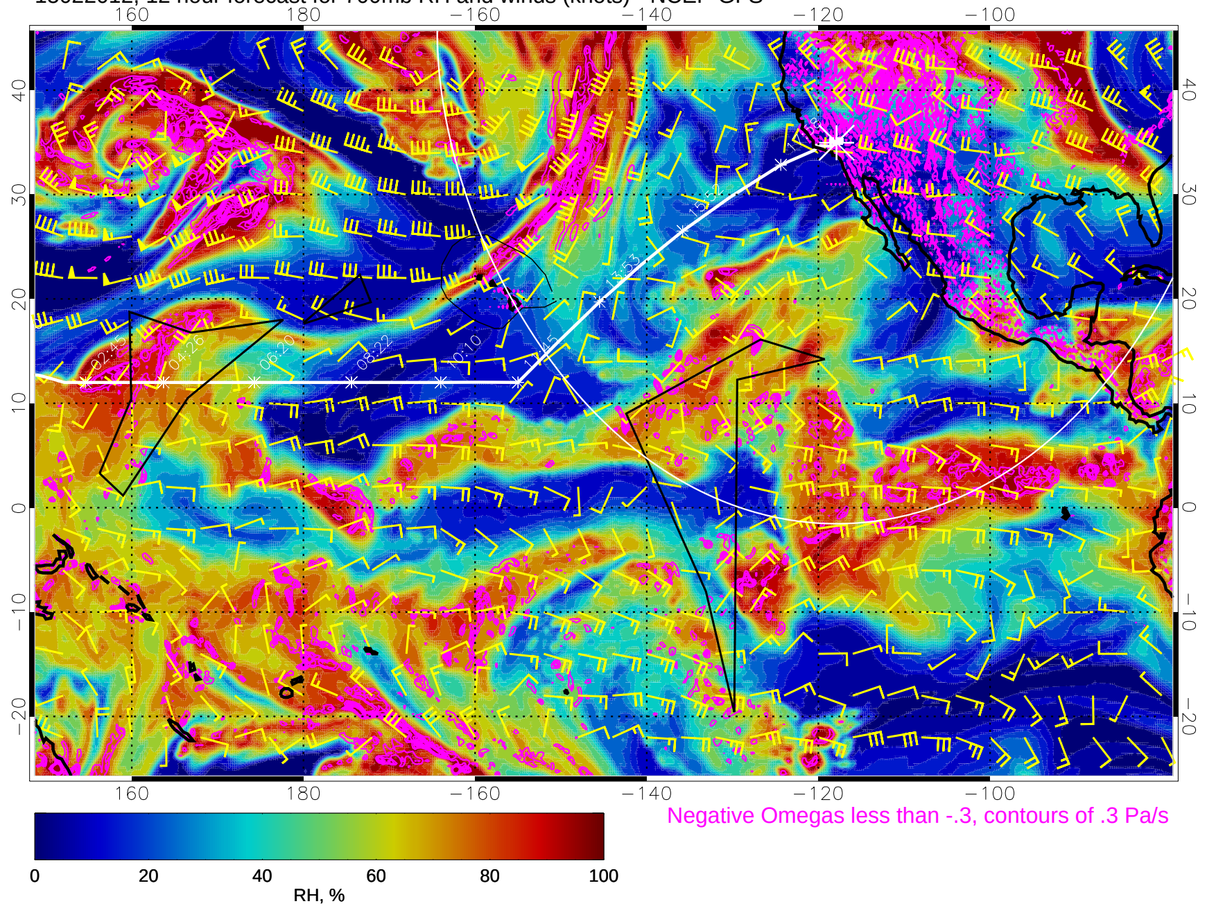
15022012, 12 hour forecast for 700mb RH and winds (knots) - NCEP GFS
