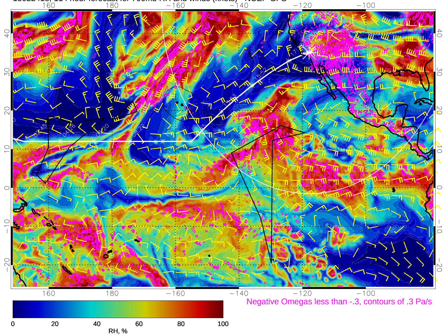
15022418, 114 hour forecast for 700mb RH and winds (knots) - NCEP GFS
