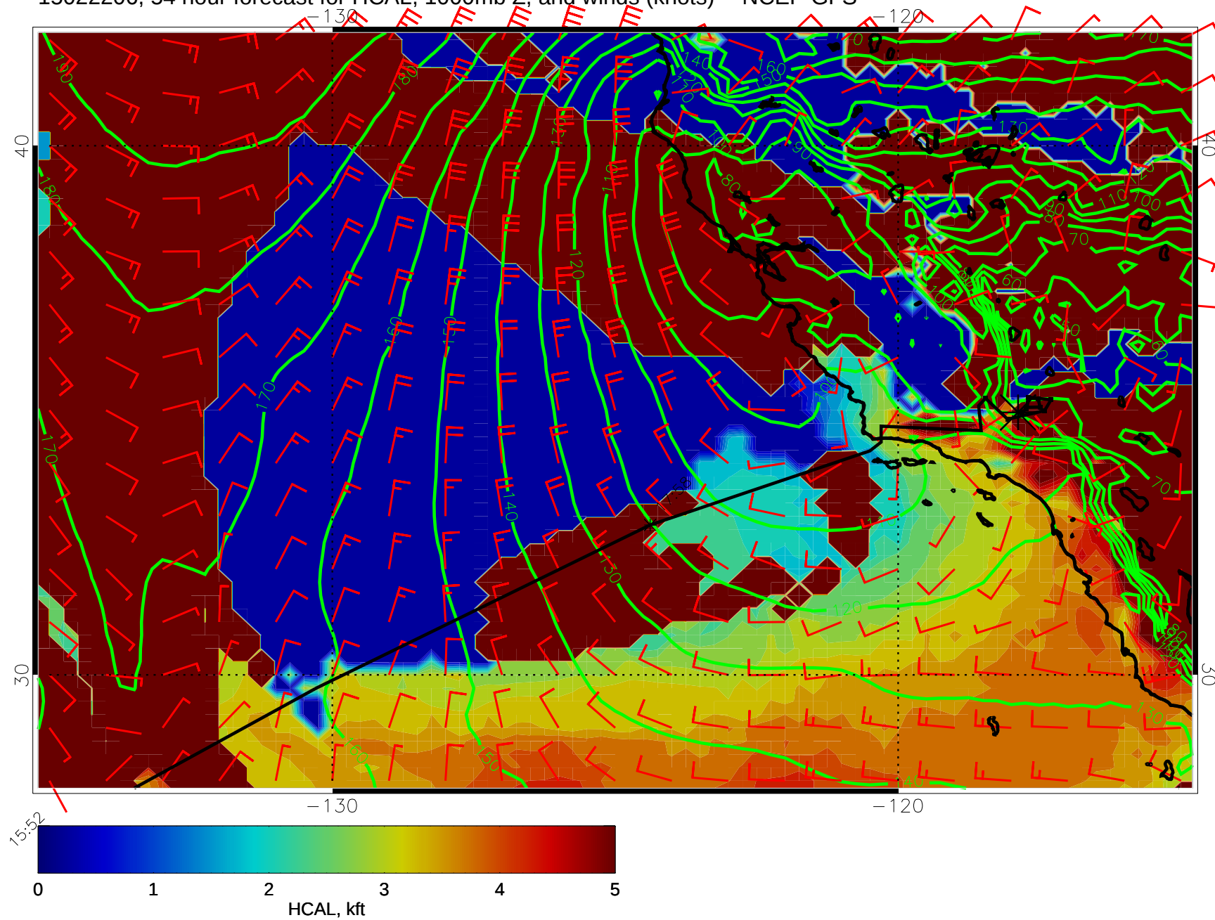
15022206, 54 hour forecast for HCAL, 1000mb Z, and winds (knots) -- NCEP GFS
