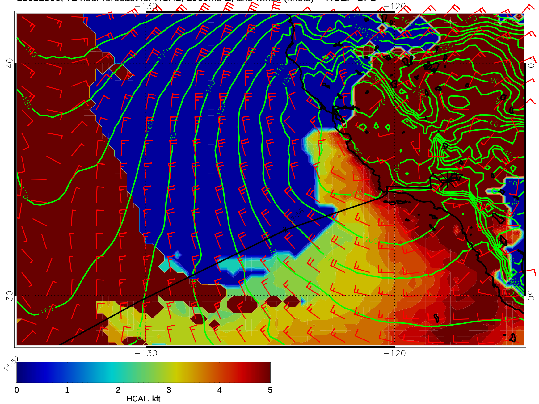
15022300, 72 hour forecast for HCAL, 1000mb Z, and winds (knots) -- NCEP GFS
