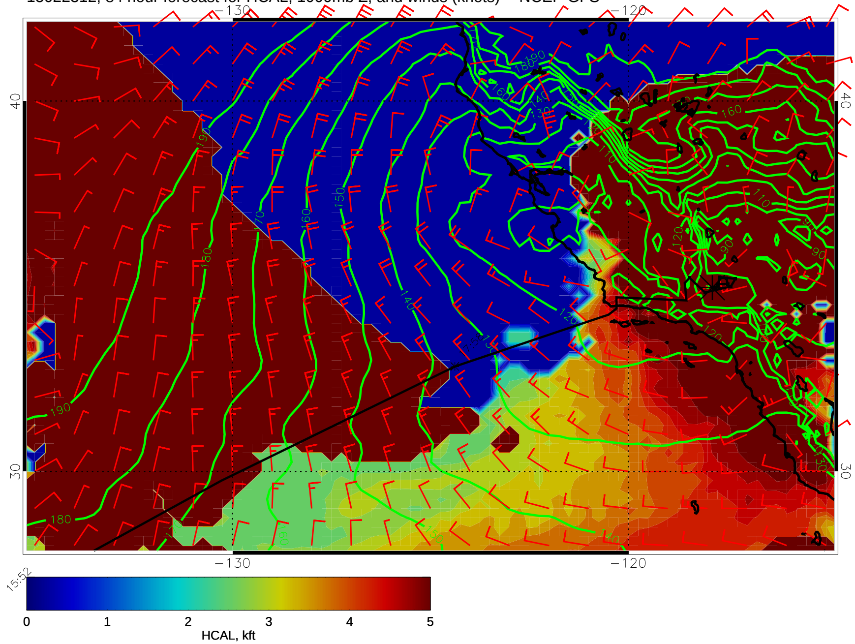
15022312, 84 hour forecast for HCAL, 1000mb Z, and winds (knots) -- NCEP GFS
