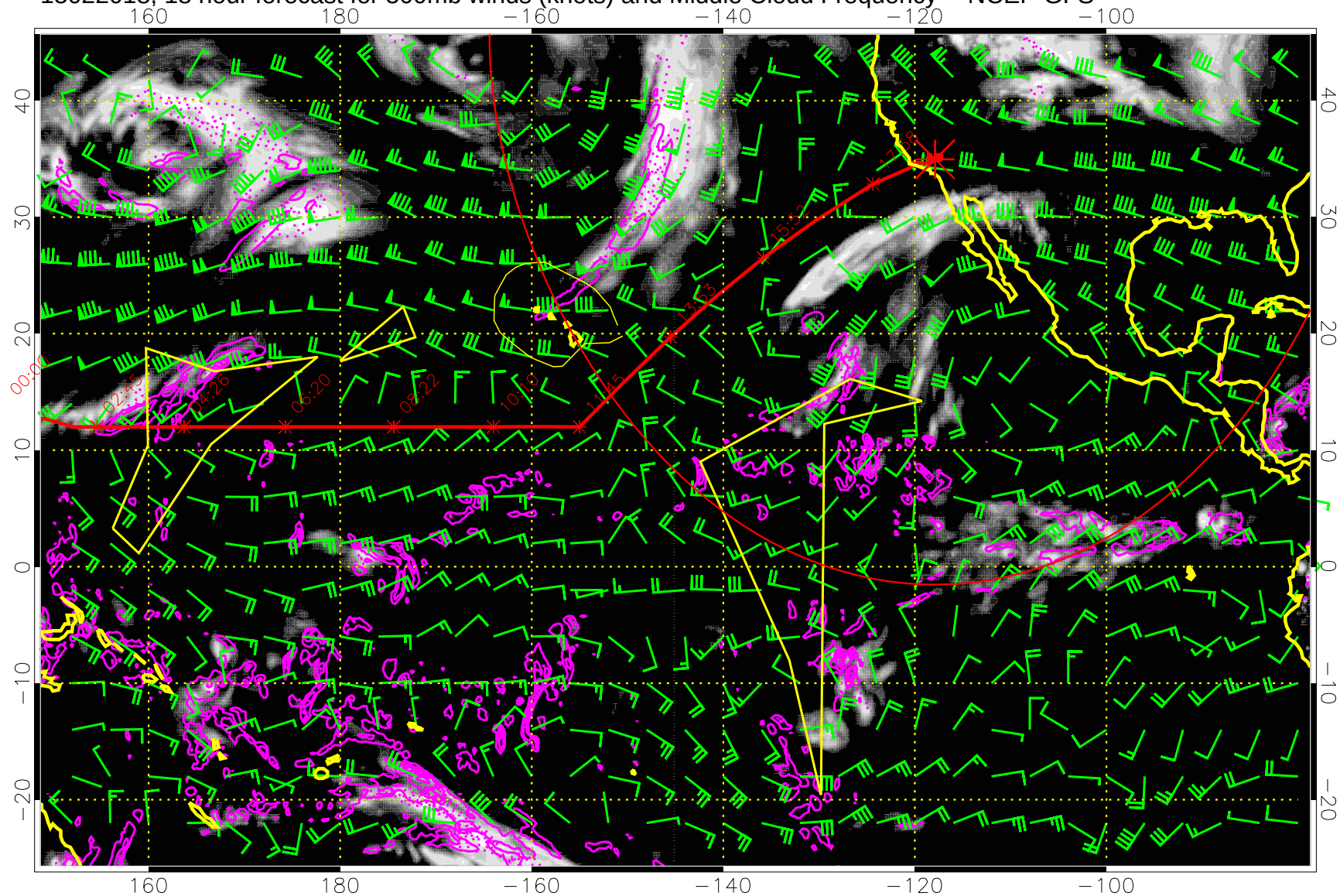
15022018, 18 hour forecast for 500mb winds (knots) and Middle Cloud Frequency -- NCEP GFS
