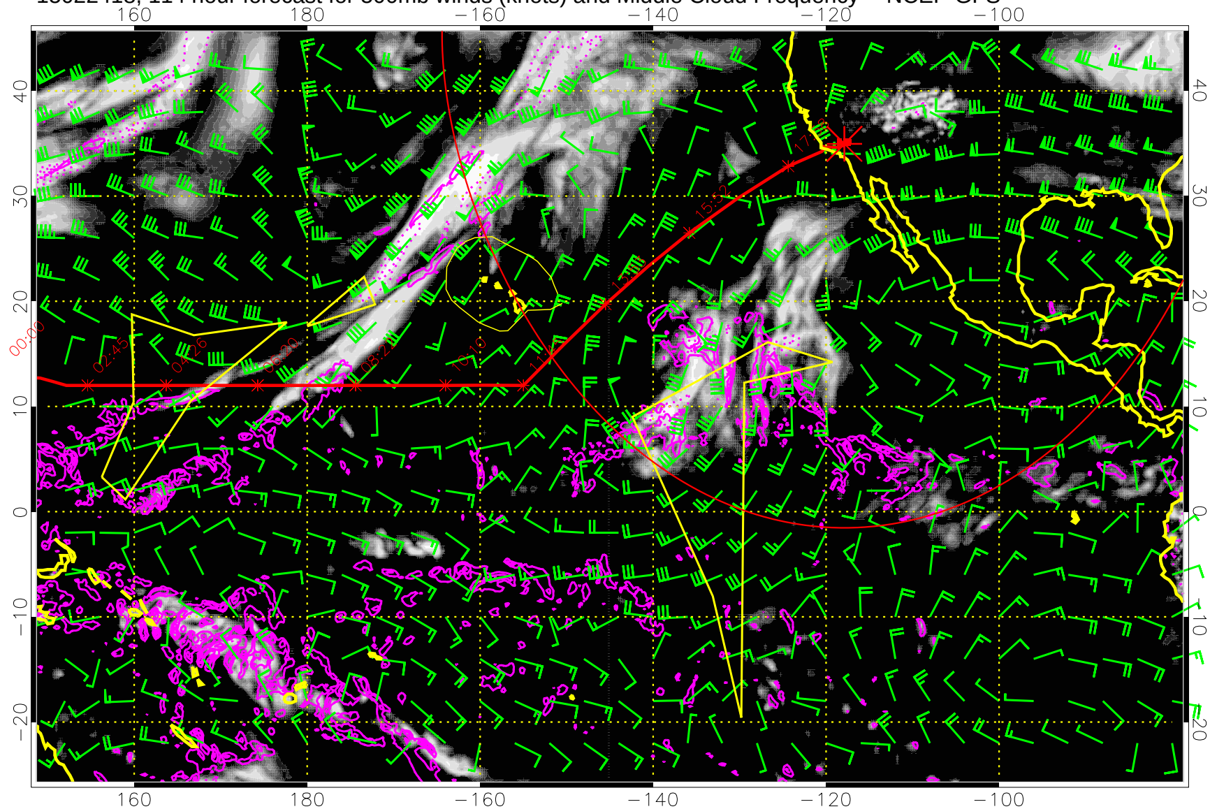
15022418, 114 hour forecast for 500mb winds (knots) and Middle Cloud Frequency -- NCEP GFS
