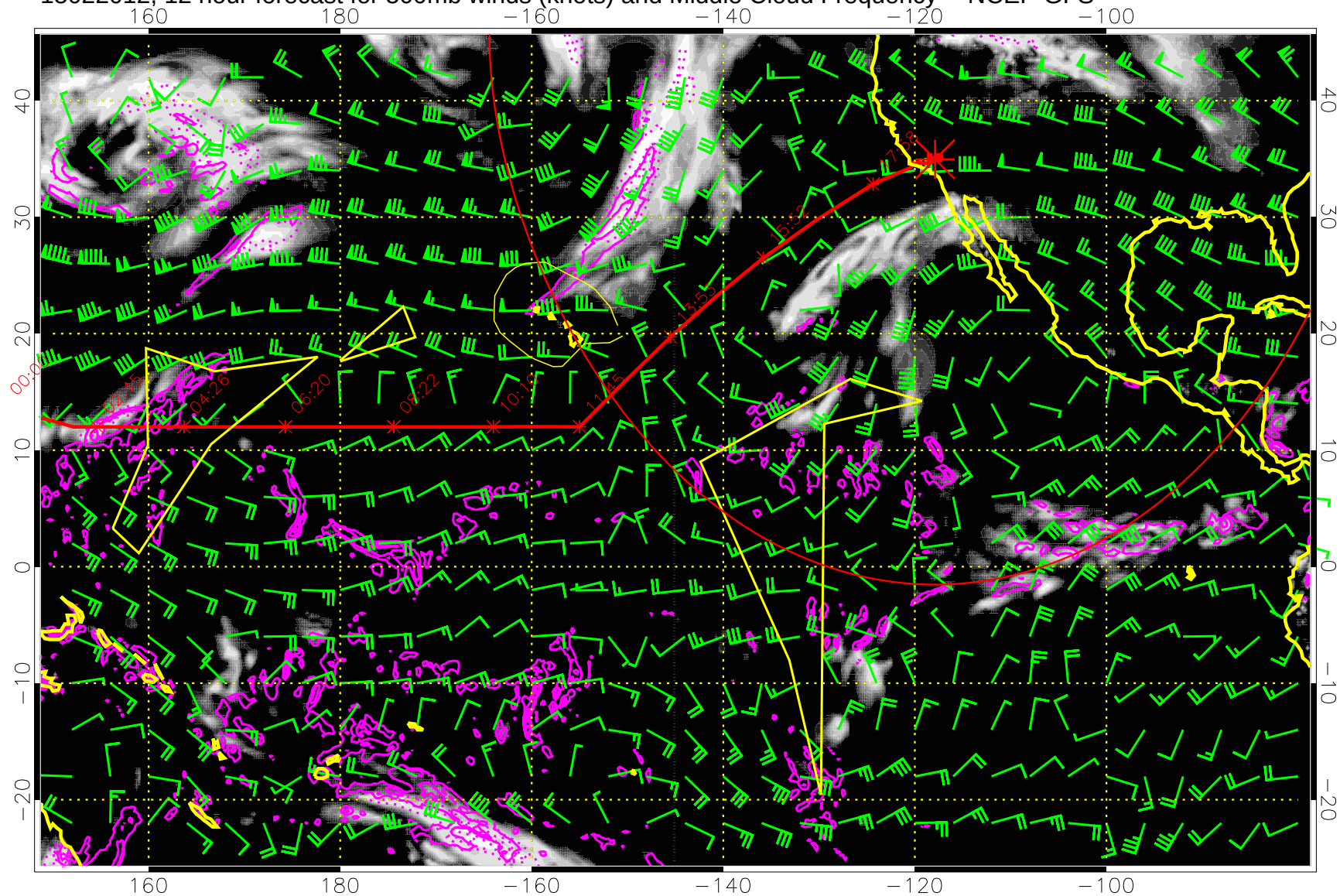
15022012, 12 hour forecast for 500mb winds (knots) and Middle Cloud Frequency -- NCEP GFS
