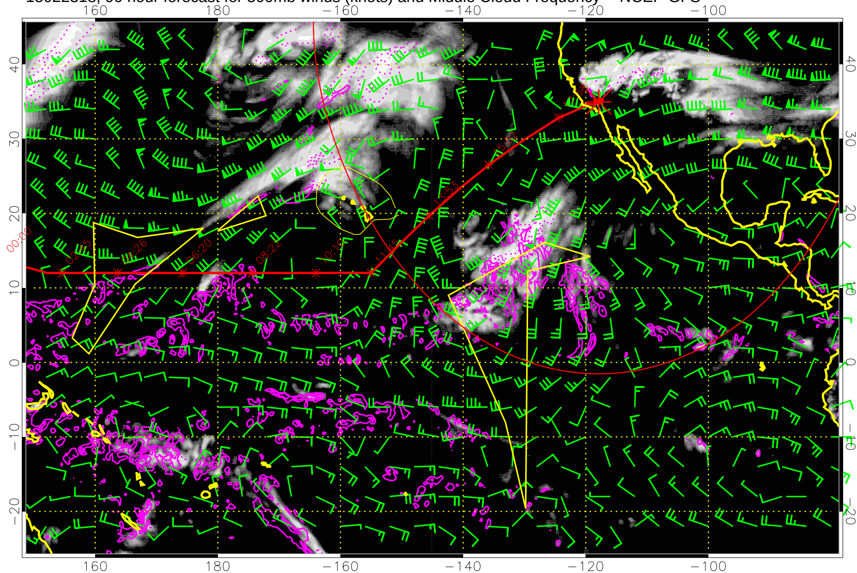
15022318, 90 hour forecast for 500mb winds (knots) and Middle Cloud Frequency -- NCEP GFS
