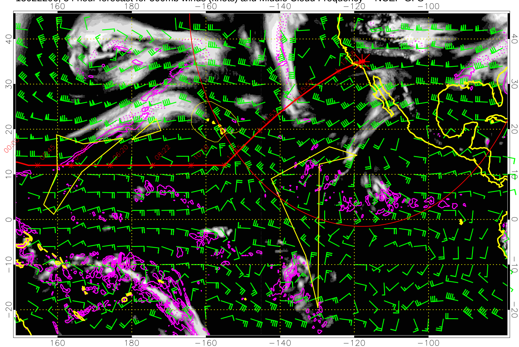
15022206, 54 hour forecast for 500mb winds (knots) and Middle Cloud Frequency -- NCEP GFS
