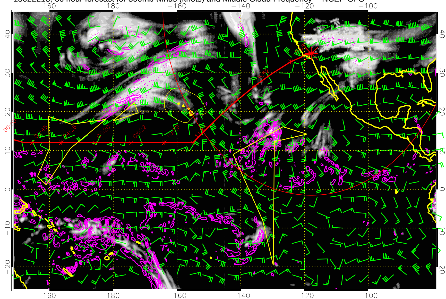
15022218, 66 hour forecast for 500mb winds (knots) and Middle Cloud Frequency -- NCEP GFS
