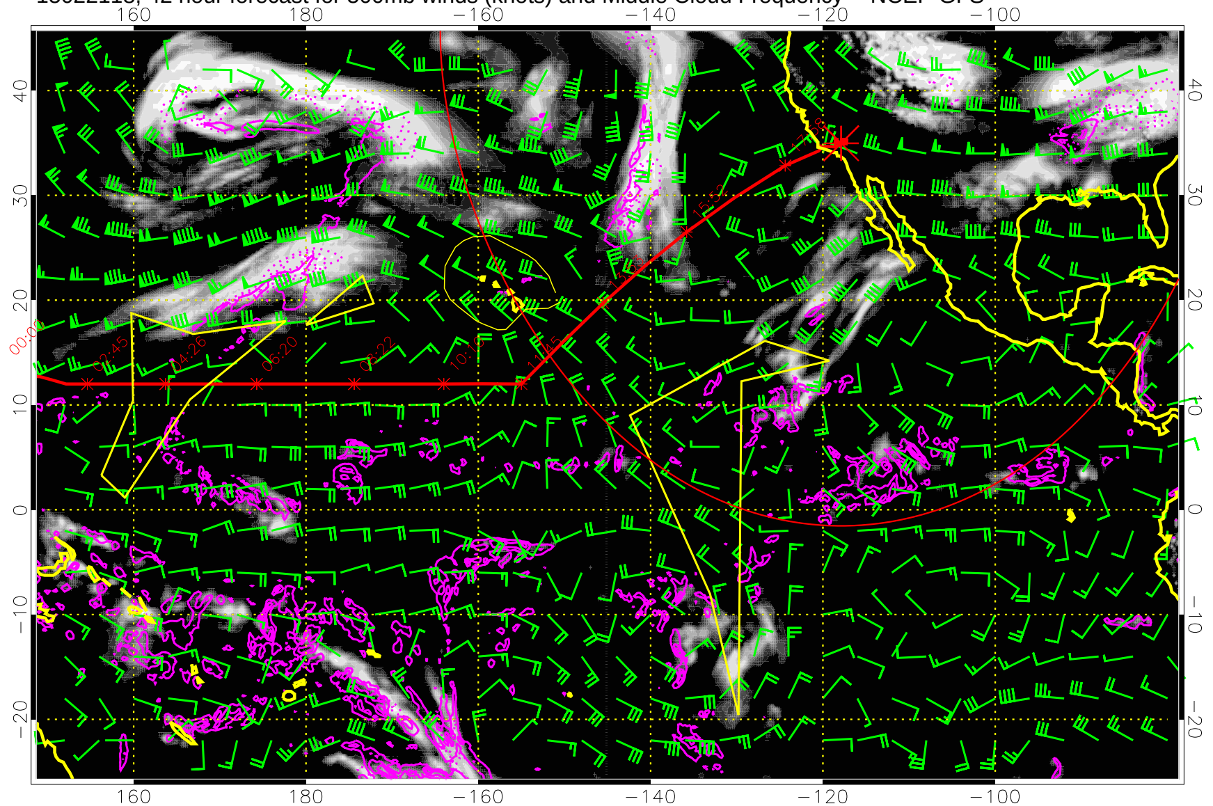
15022118, 42 hour forecast for 500mb winds (knots) and Middle Cloud Frequency -- NCEP GFS
