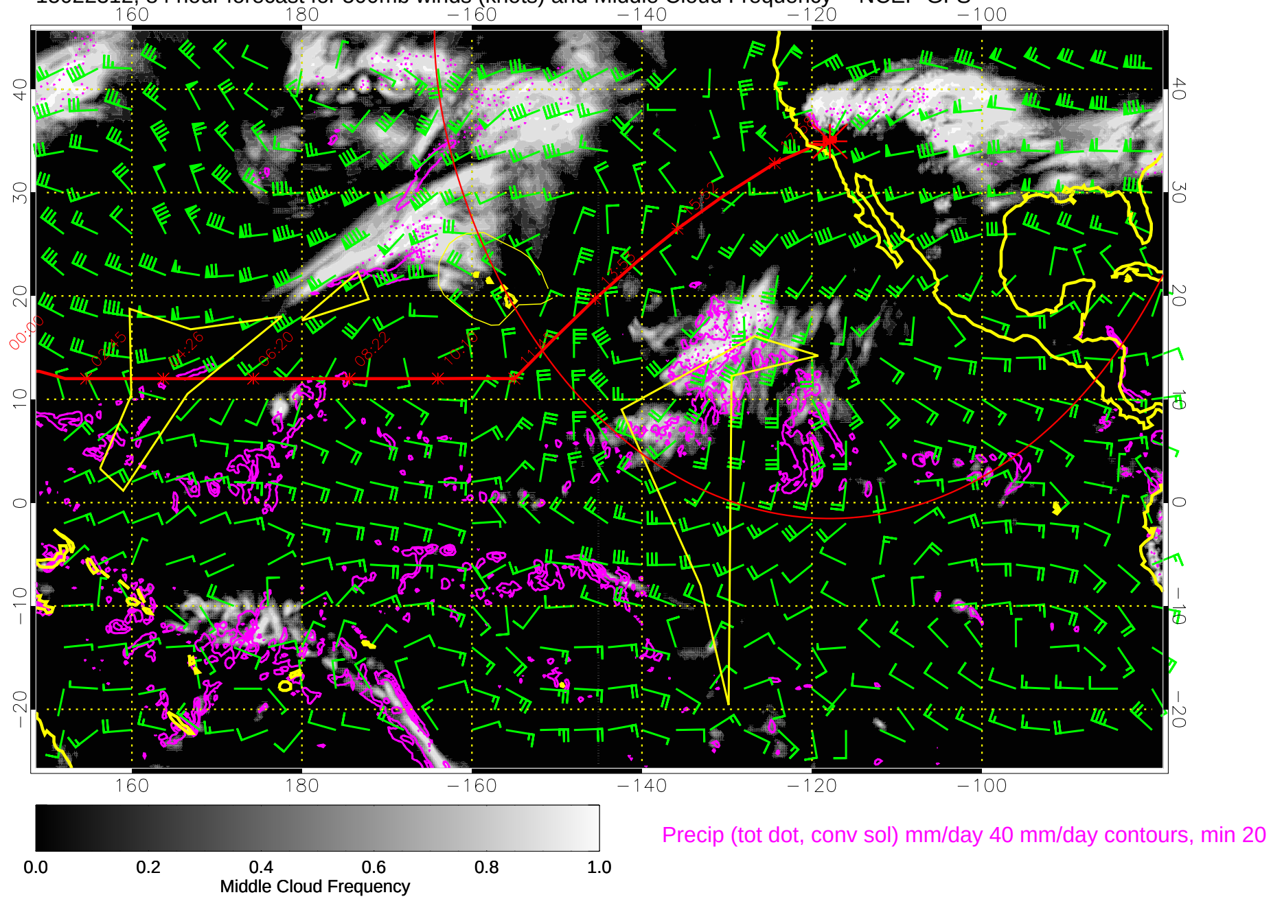
15022312, 84 hour forecast for 500mb winds (knots) and Middle Cloud Frequency -- NCEP GFS
