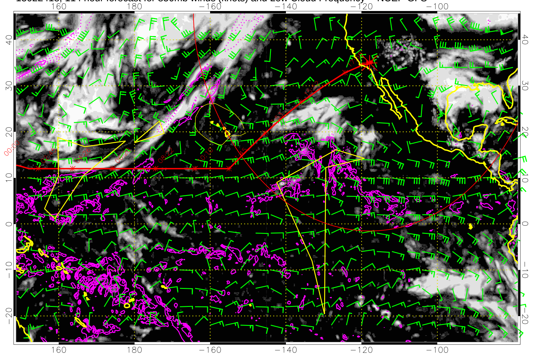
15022418, 114 hour forecast for 850mb winds (knots) and Low Cloud Frequency -- NCEP GFS
