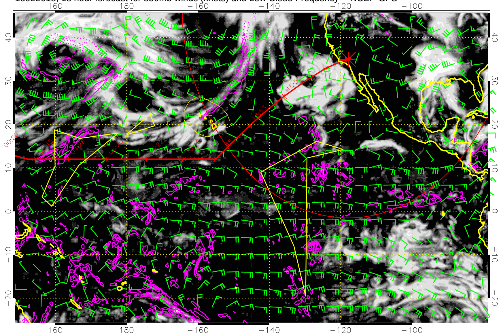
15022018, 18 hour forecast for 850mb winds (knots) and Low Cloud Frequency -- NCEP GFS
