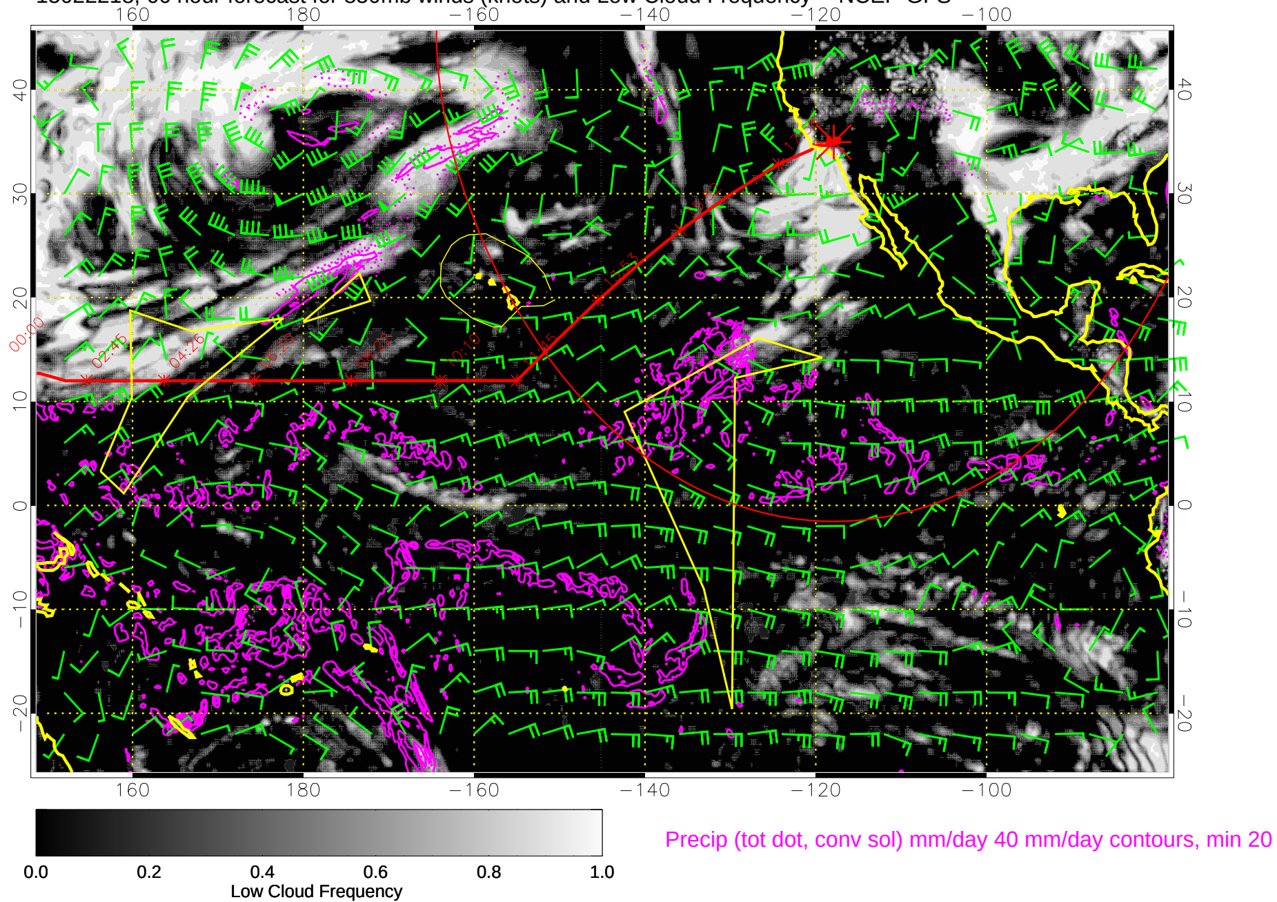
15022218, 66 hour forecast for 850mb winds (knots) and Low Cloud Frequency -- NCEP GFS
