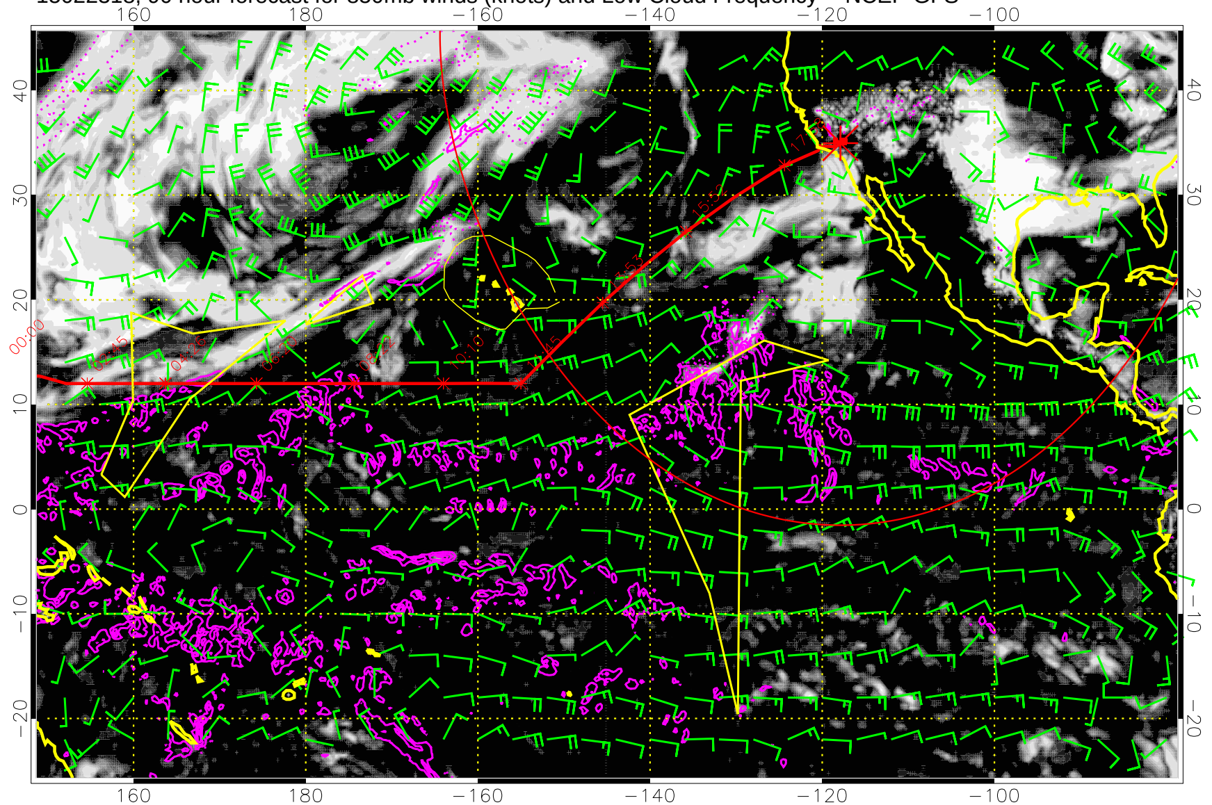
15022318, 90 hour forecast for 850mb winds (knots) and Low Cloud Frequency -- NCEP GFS
