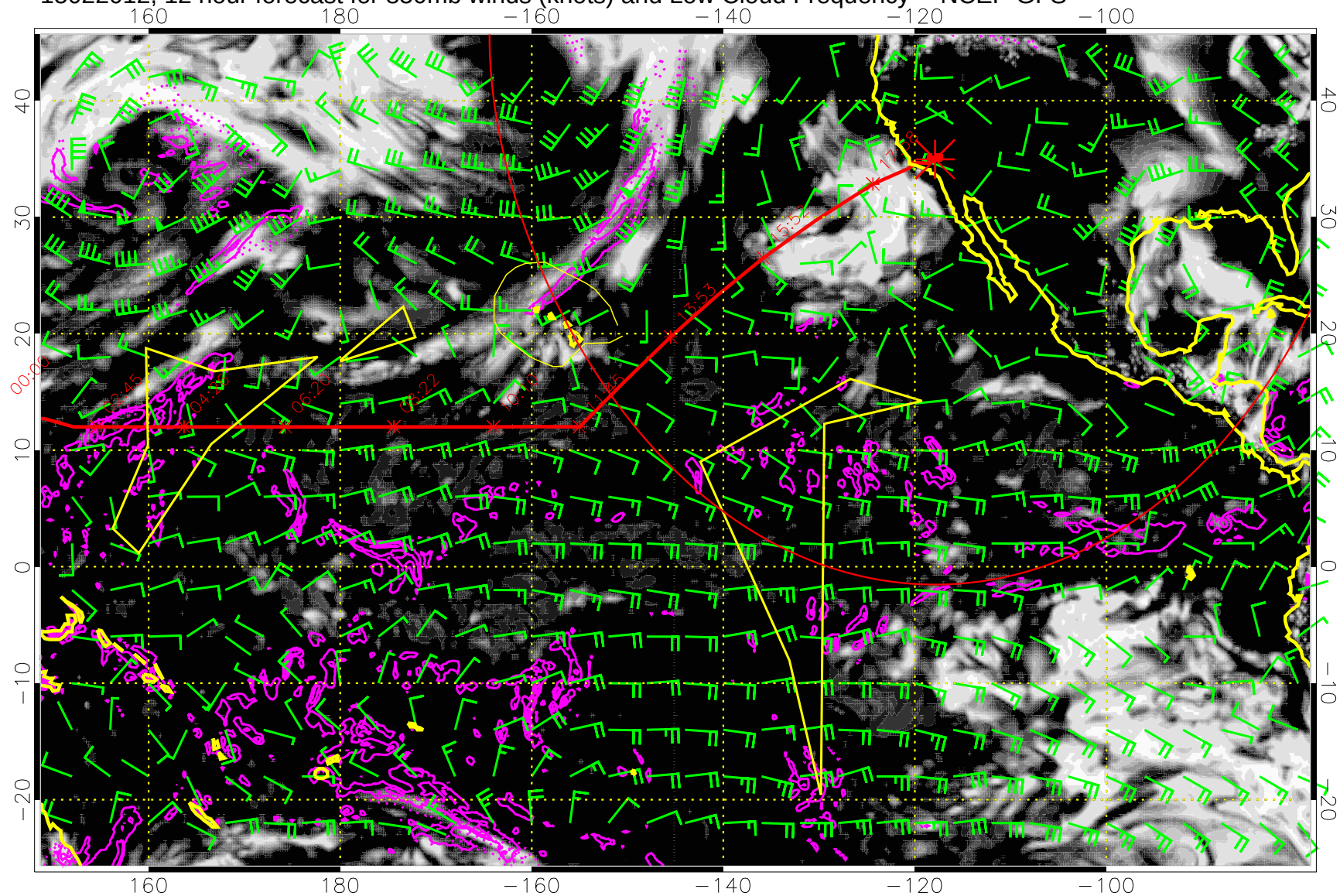
15022012, 12 hour forecast for 850mb winds (knots) and Low Cloud Frequency -- NCEP GFS
