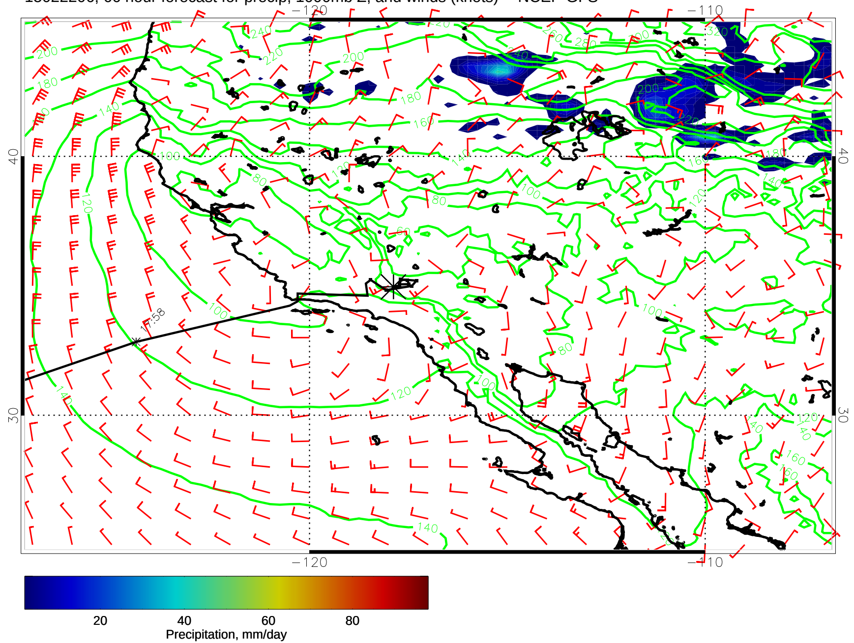
15022206, 66 hour forecast for precip, 1000mb Z, and winds (knots) -- NCEP GFS
