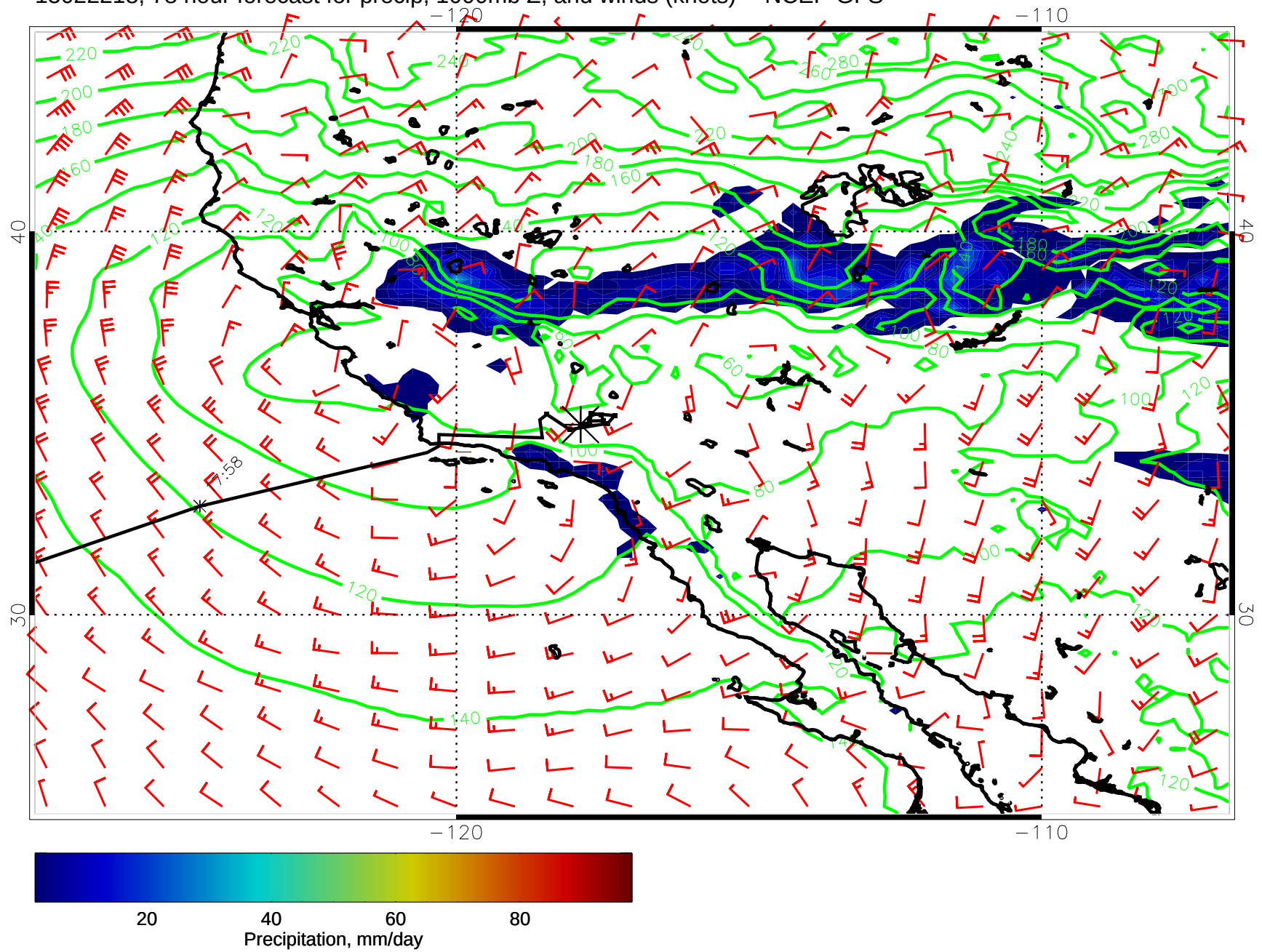
15022218, 78 hour forecast for precip, 1000mb Z, and winds (knots) -- NCEP GFS
