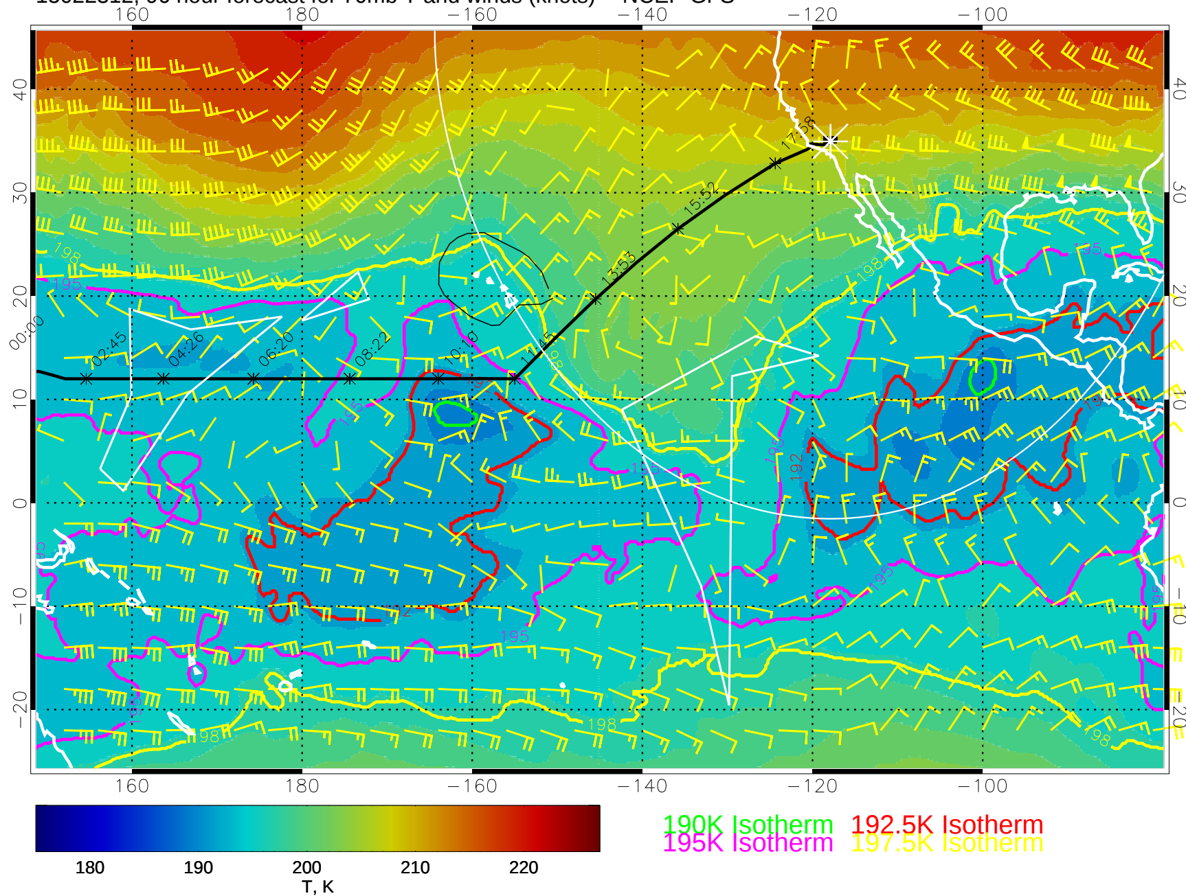
15022312, 96 hour forecast for 70mb T and winds (knots) -- NCEP GFS
