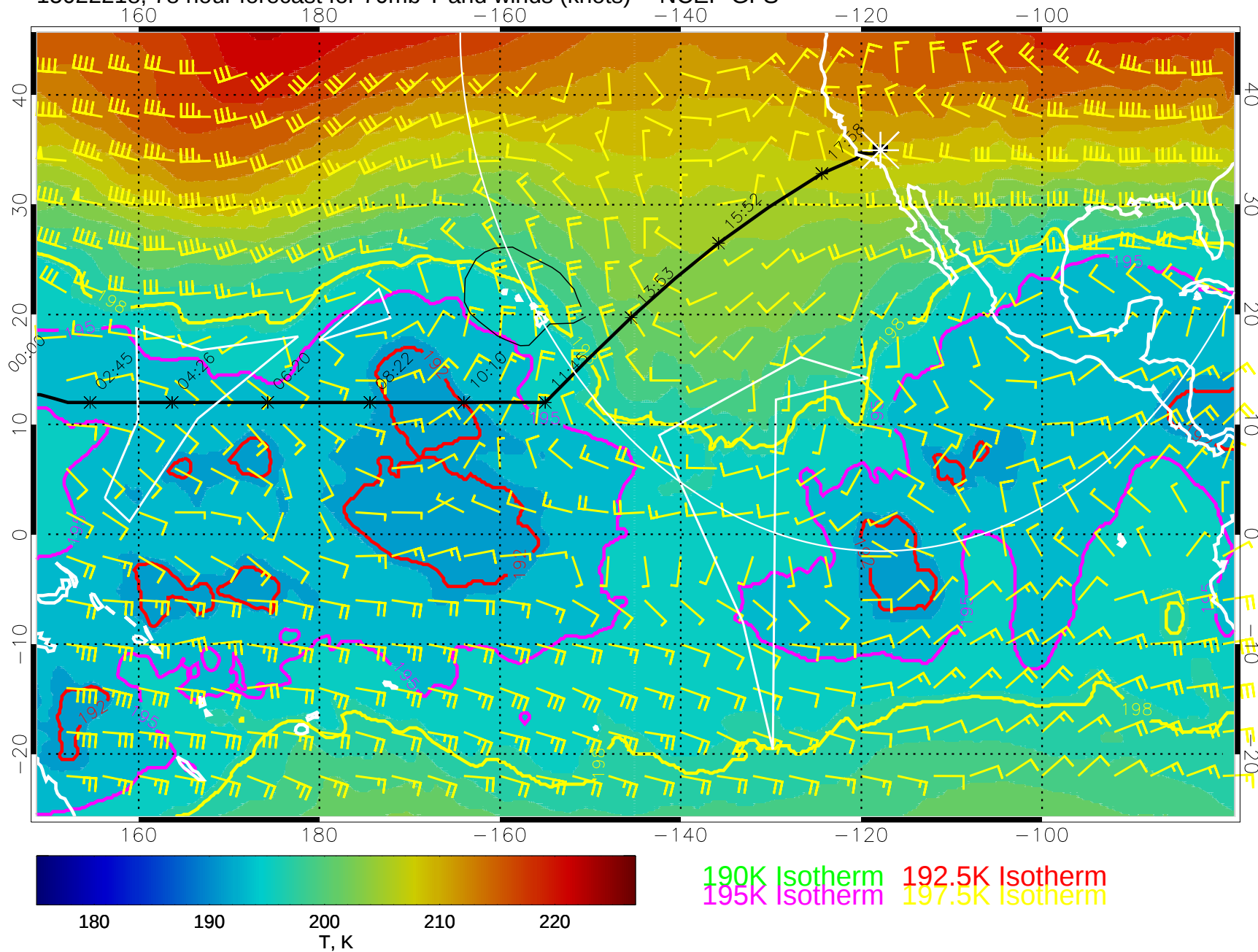
15022218, 78 hour forecast for 70mb T and winds (knots) -- NCEP GFS
