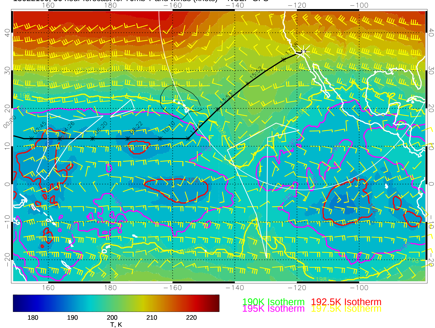
15022100, 36 hour forecast for 70mb T and winds (knots) -- NCEP GFS
