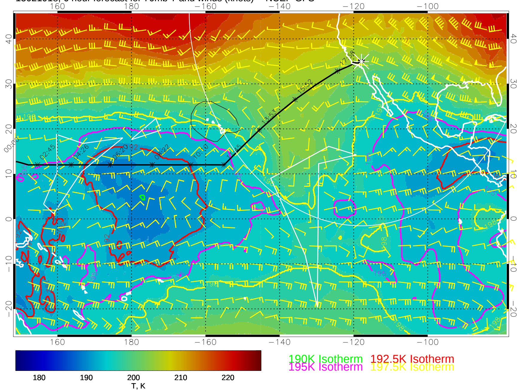
15021918, 6 hour forecast for 70mb T and winds (knots) -- NCEP GFS
