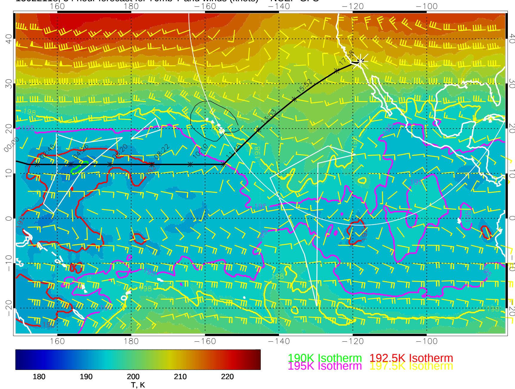
15022118, 54 hour forecast for 70mb T and winds (knots) -- NCEP GFS
