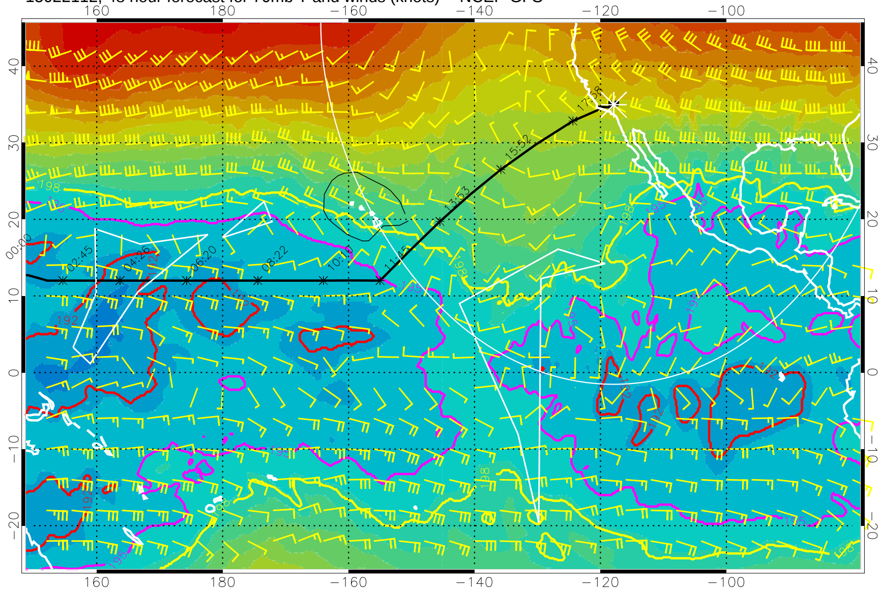
15022112, 48 hour forecast for 70mb T and winds (knots) -- NCEP GFS
