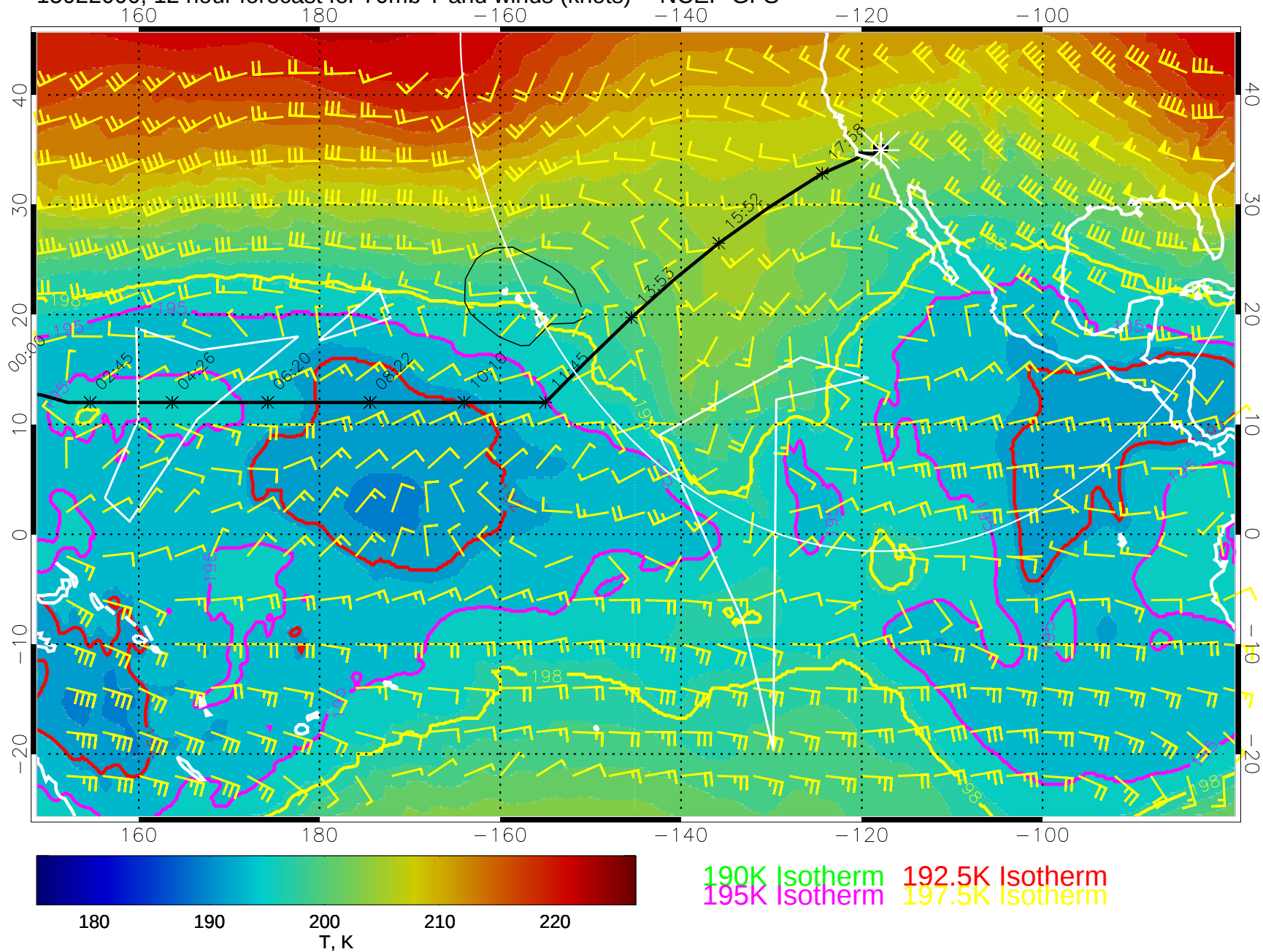
15022000, 12 hour forecast for 70mb T and winds (knots) -- NCEP GFS
