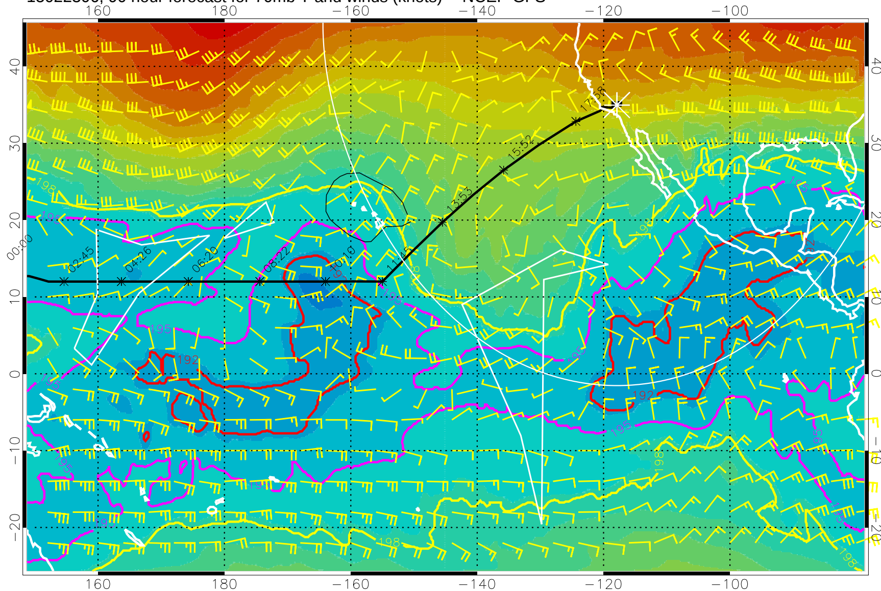
15022306, 90 hour forecast for 70mb T and winds (knots) -- NCEP GFS
