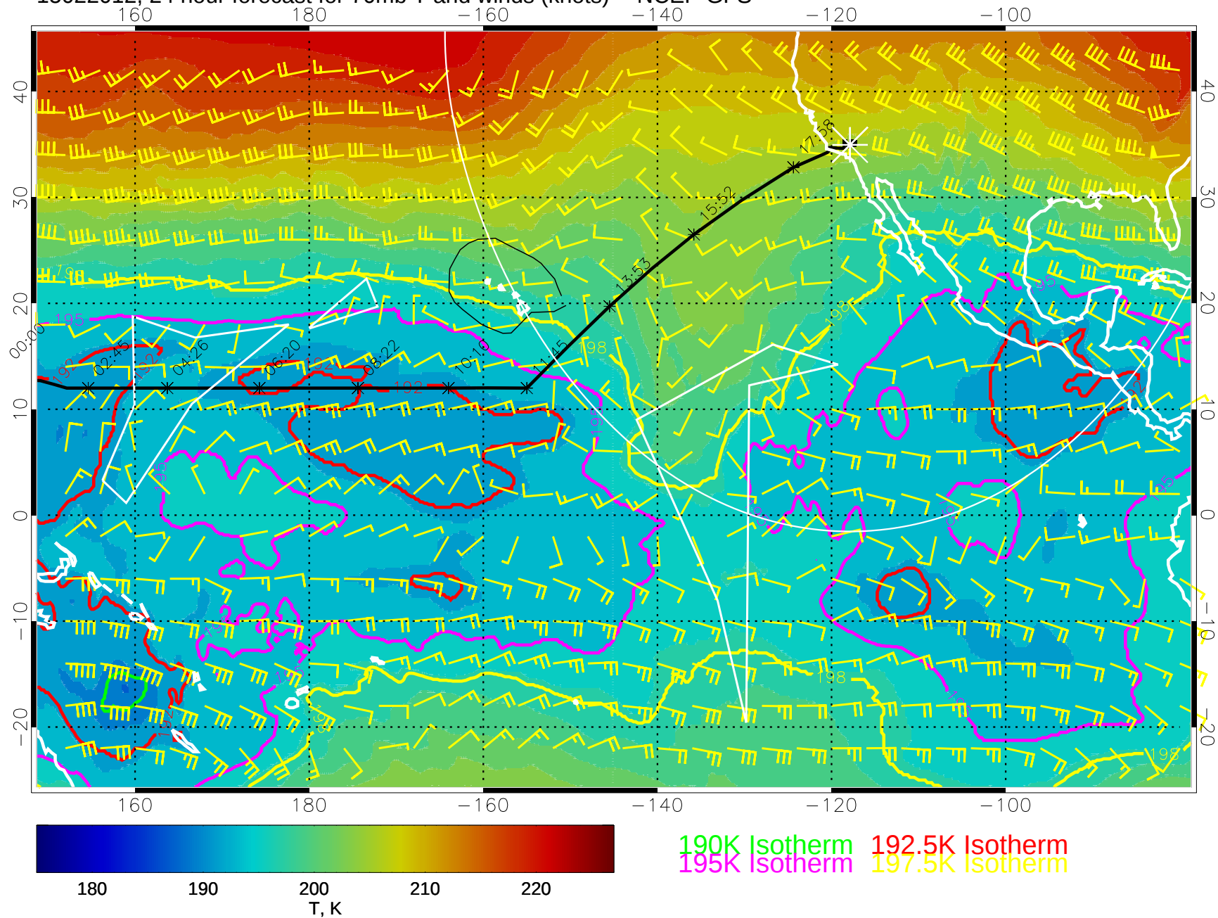
15022012, 24 hour forecast for 70mb T and winds (knots) -- NCEP GFS
