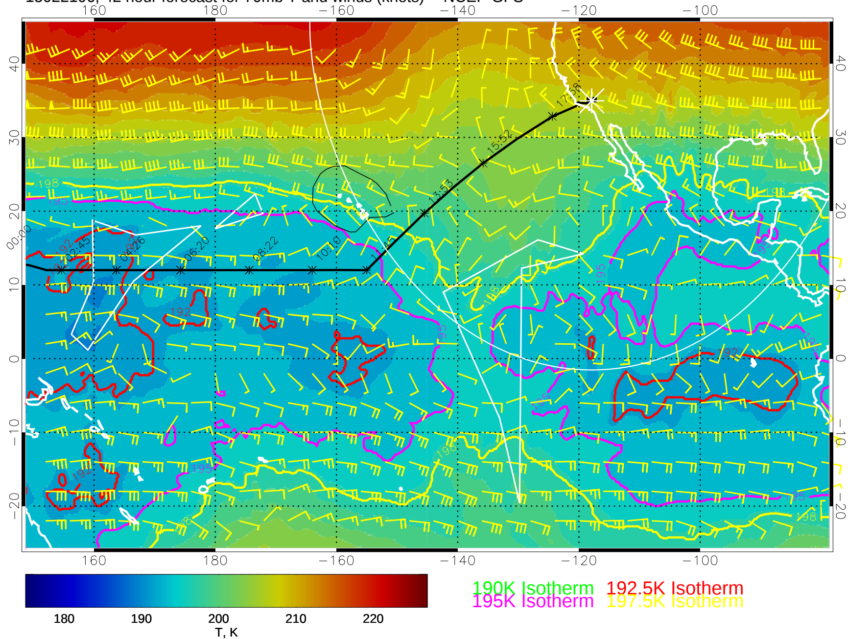
15022106, 42 hour forecast for 70mb T and winds (knots) -- NCEP GFS
