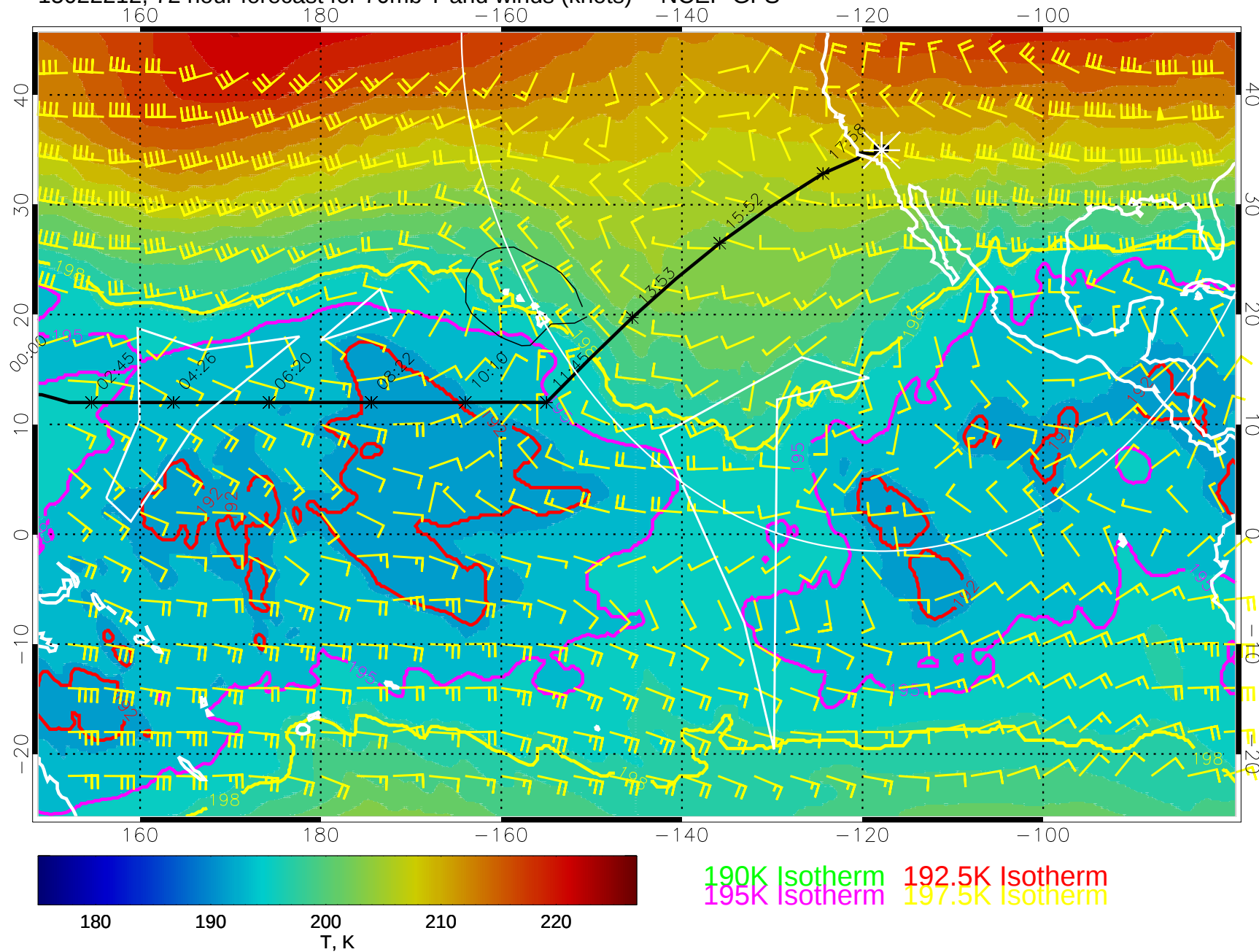
15022212, 72 hour forecast for 70mb T and winds (knots) -- NCEP GFS
