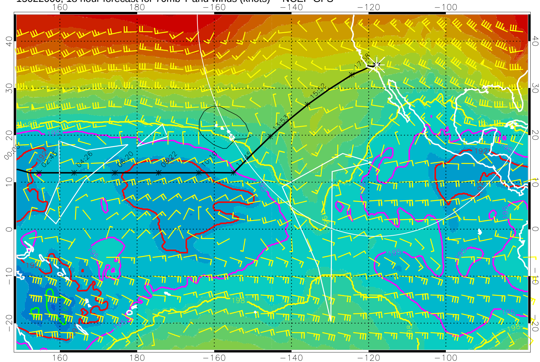
15022006, 18 hour forecast for 70mb T and winds (knots) -- NCEP GFS
