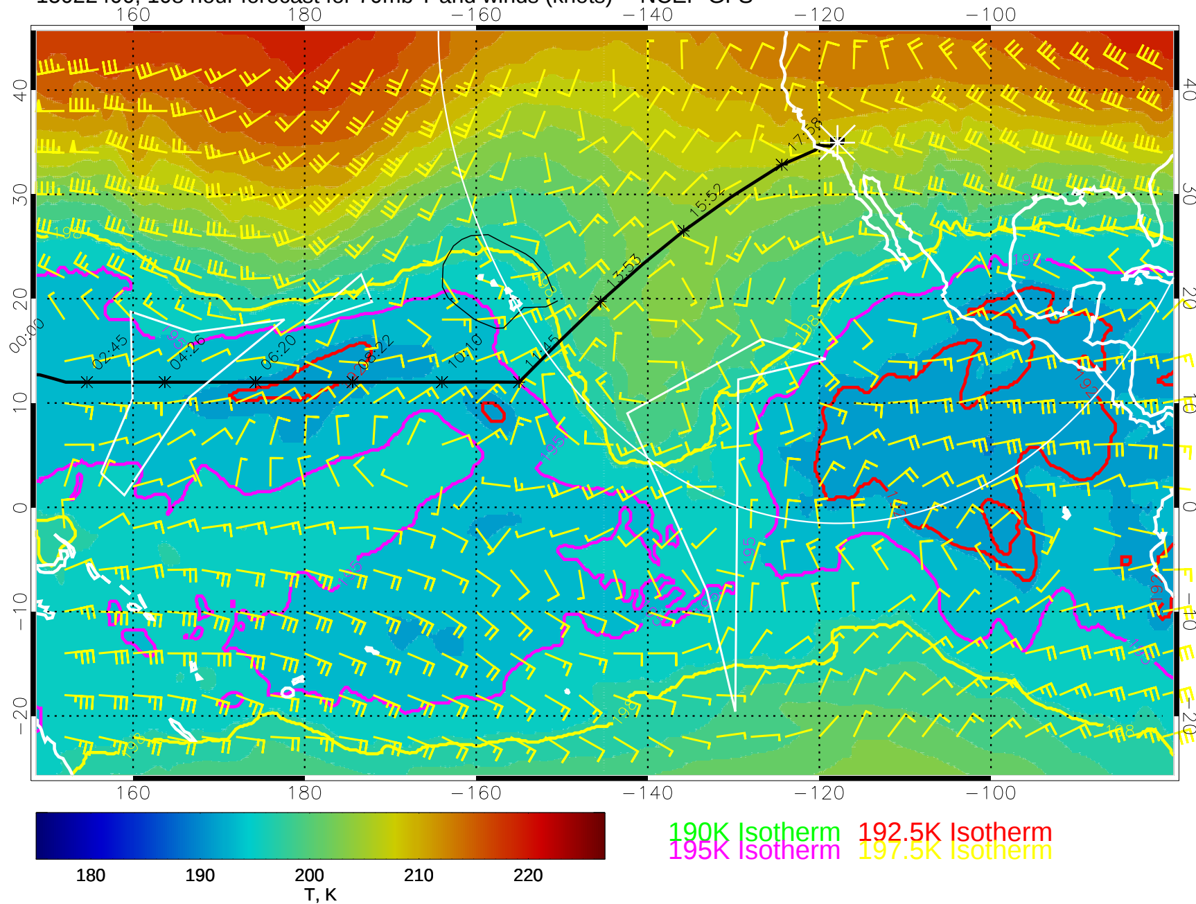
15022400, 108 hour forecast for 70mb T and winds (knots) -- NCEP GFS
