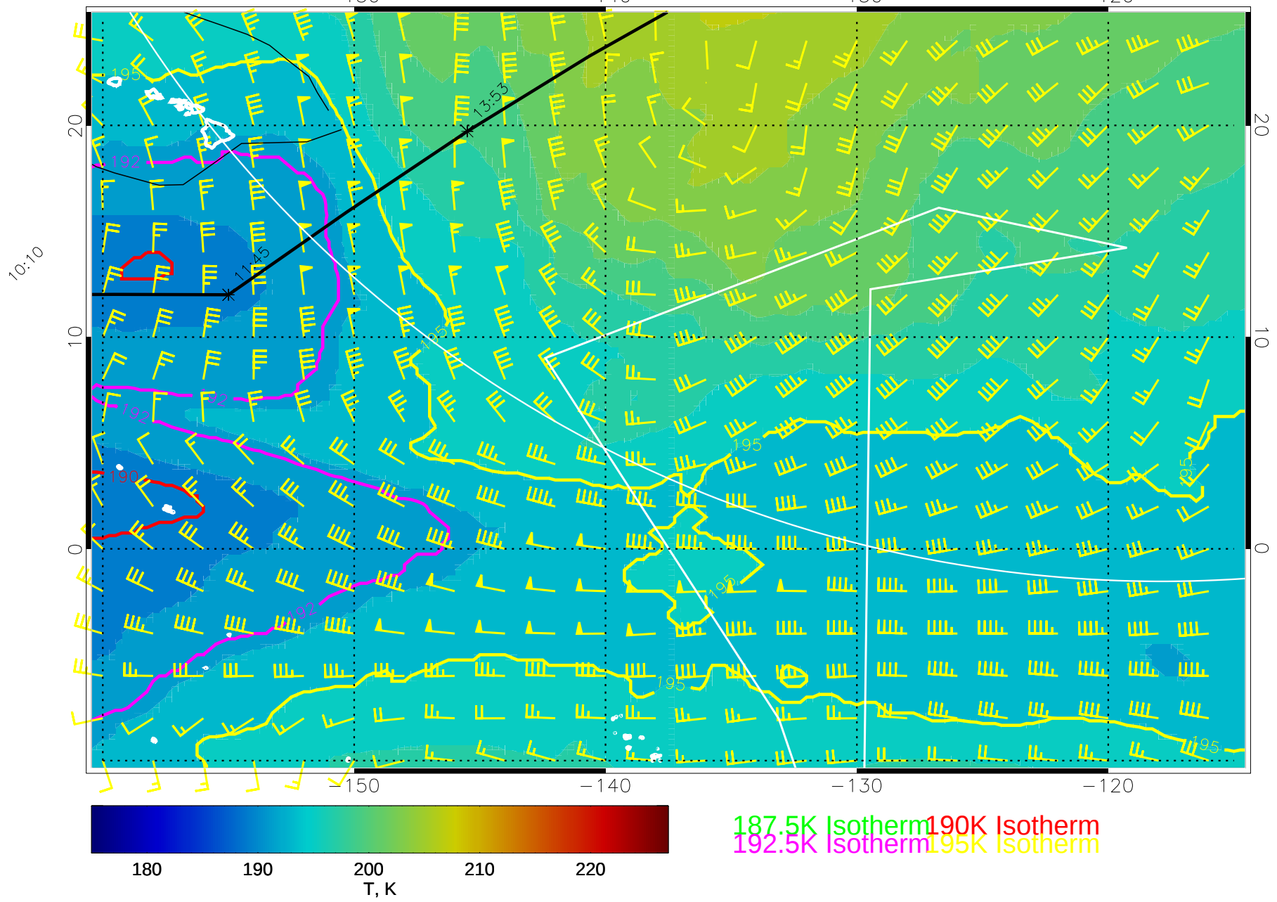
15022312, 96 hour forecast for 100mb T and winds (knots) -- NCEP GFS
