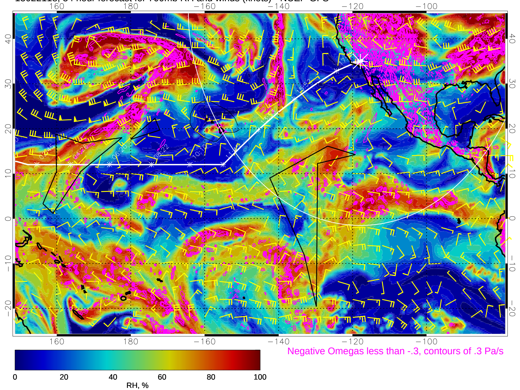
15022118, 54 hour forecast for 700mb RH and winds (knots) - NCEP GFS
