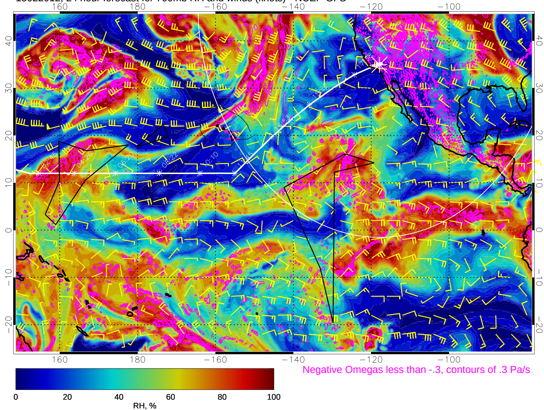
15022012, 24 hour forecast for 700mb RH and winds (knots) - NCEP GFS
