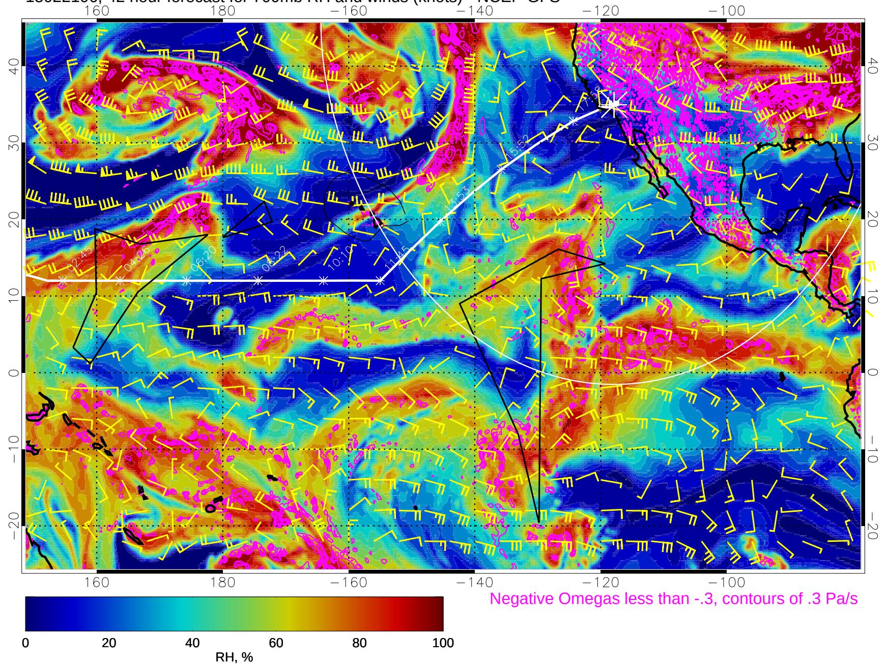
15022106, 42 hour forecast for 700mb RH and winds (knots) - NCEP GFS
