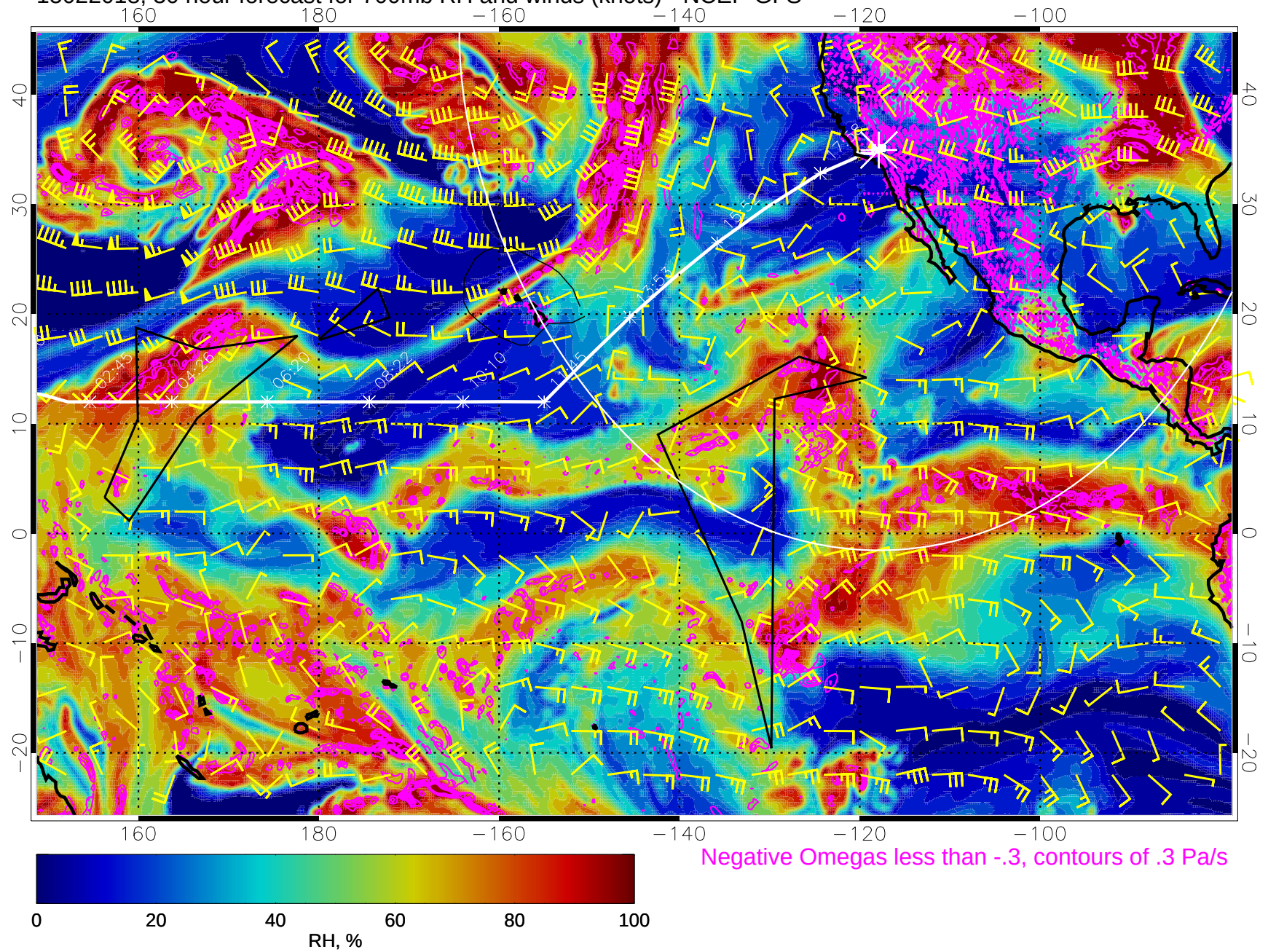
15022018, 30 hour forecast for 700mb RH and winds (knots) - NCEP GFS
