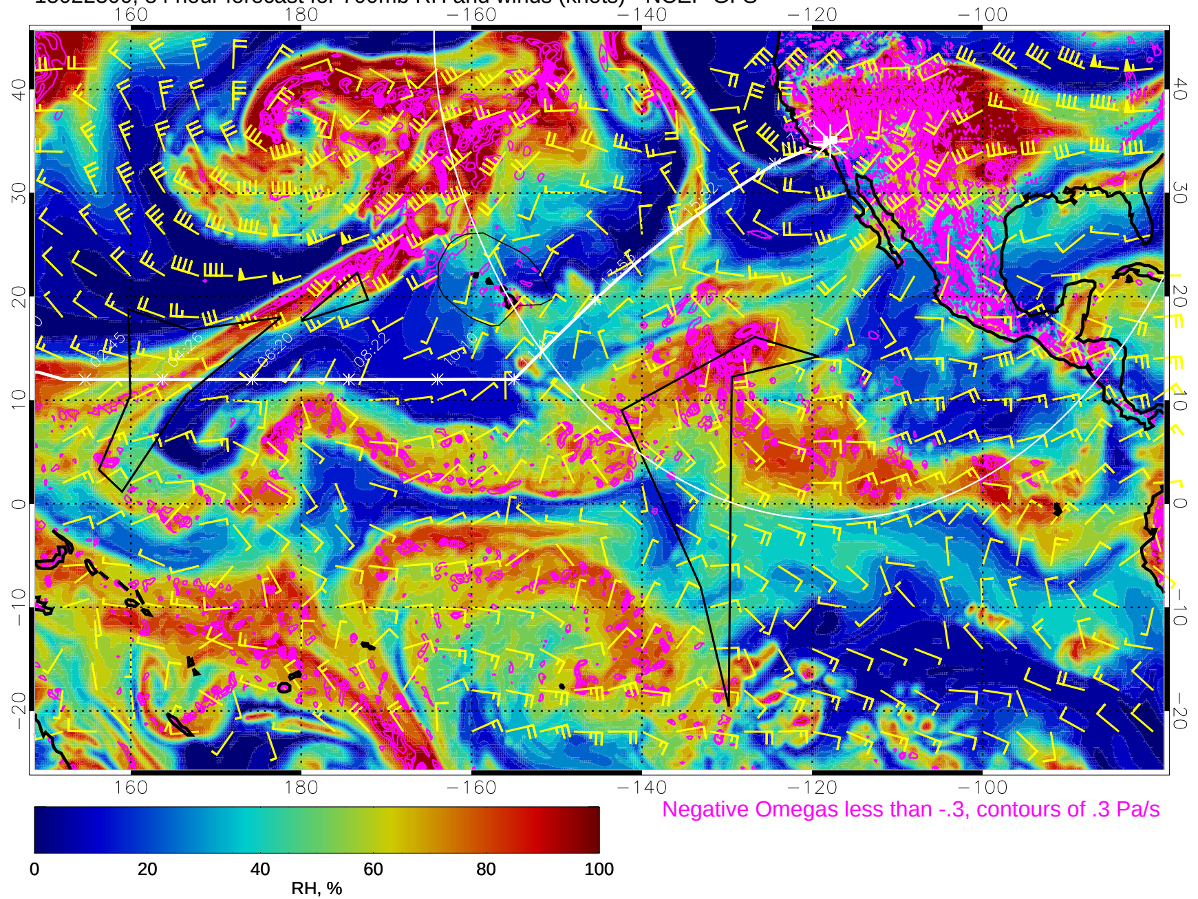
15022300, 84 hour forecast for 700mb RH and winds (knots) - NCEP GFS
