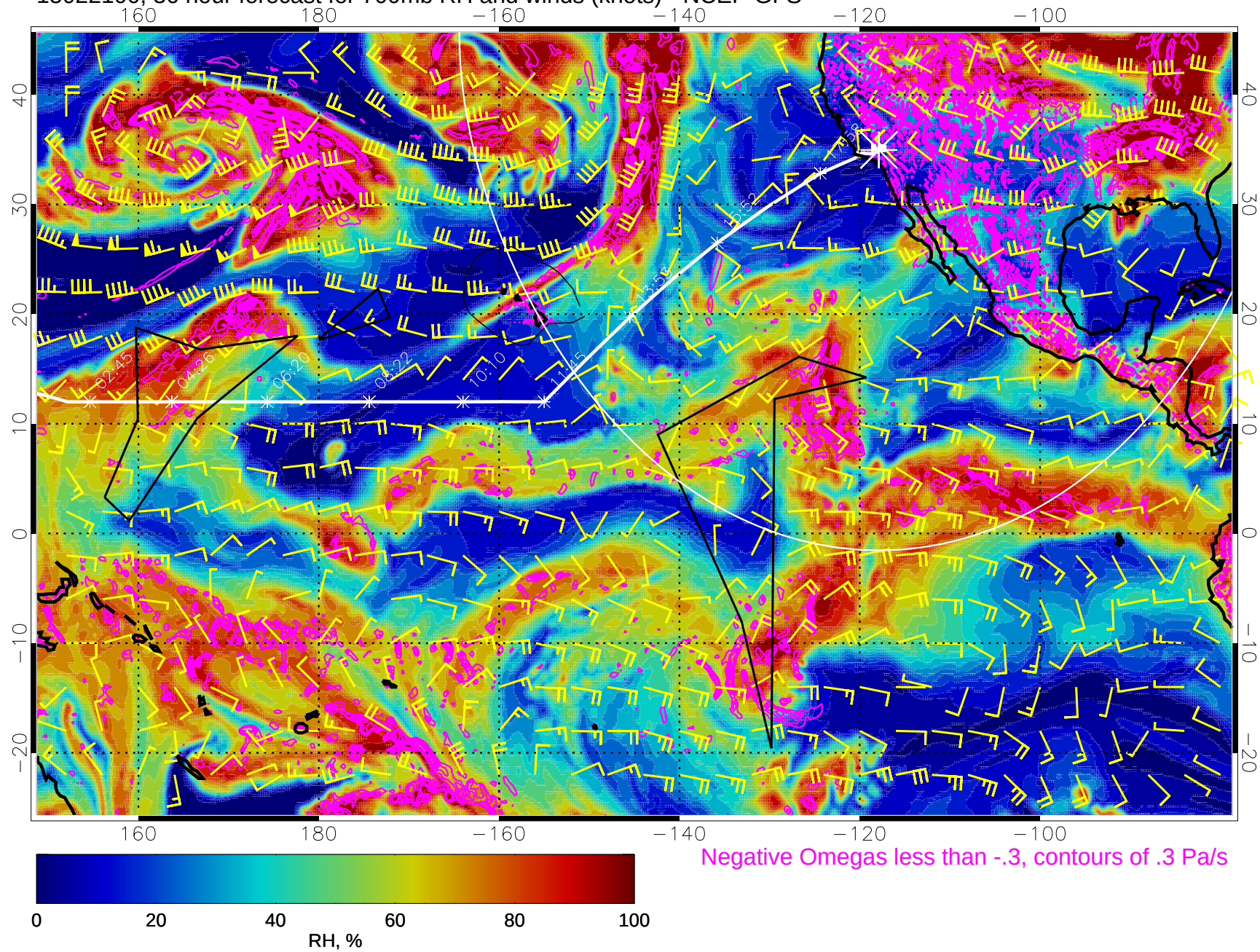
15022100, 36 hour forecast for 700mb RH and winds (knots) - NCEP GFS
