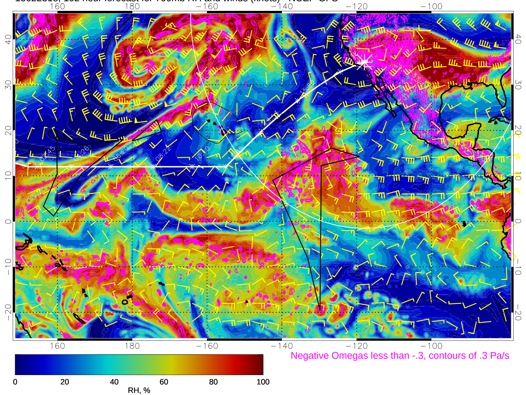
15022318, 102 hour forecast for 700mb RH and winds (knots) - NCEP GFS
