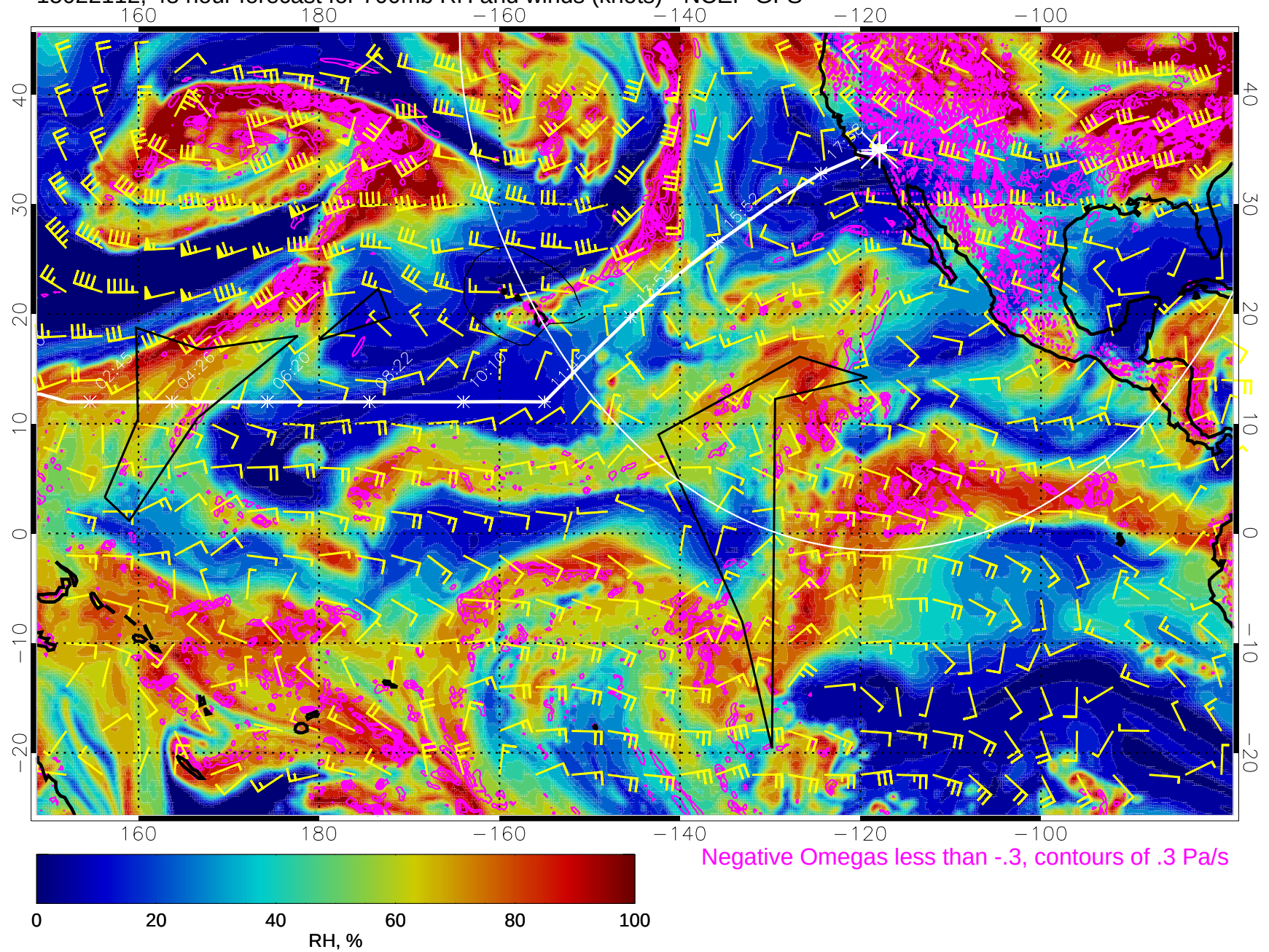
15022112, 48 hour forecast for 700mb RH and winds (knots) - NCEP GFS
