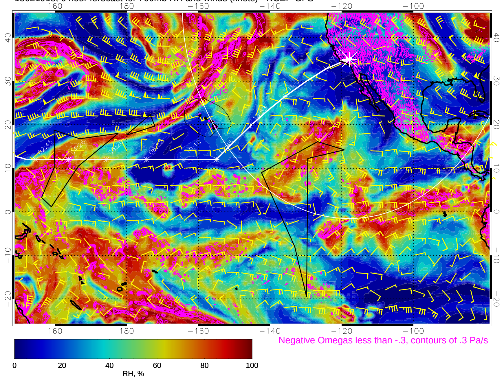
15021918, 6 hour forecast for 700mb RH and winds (knots) - NCEP GFS
