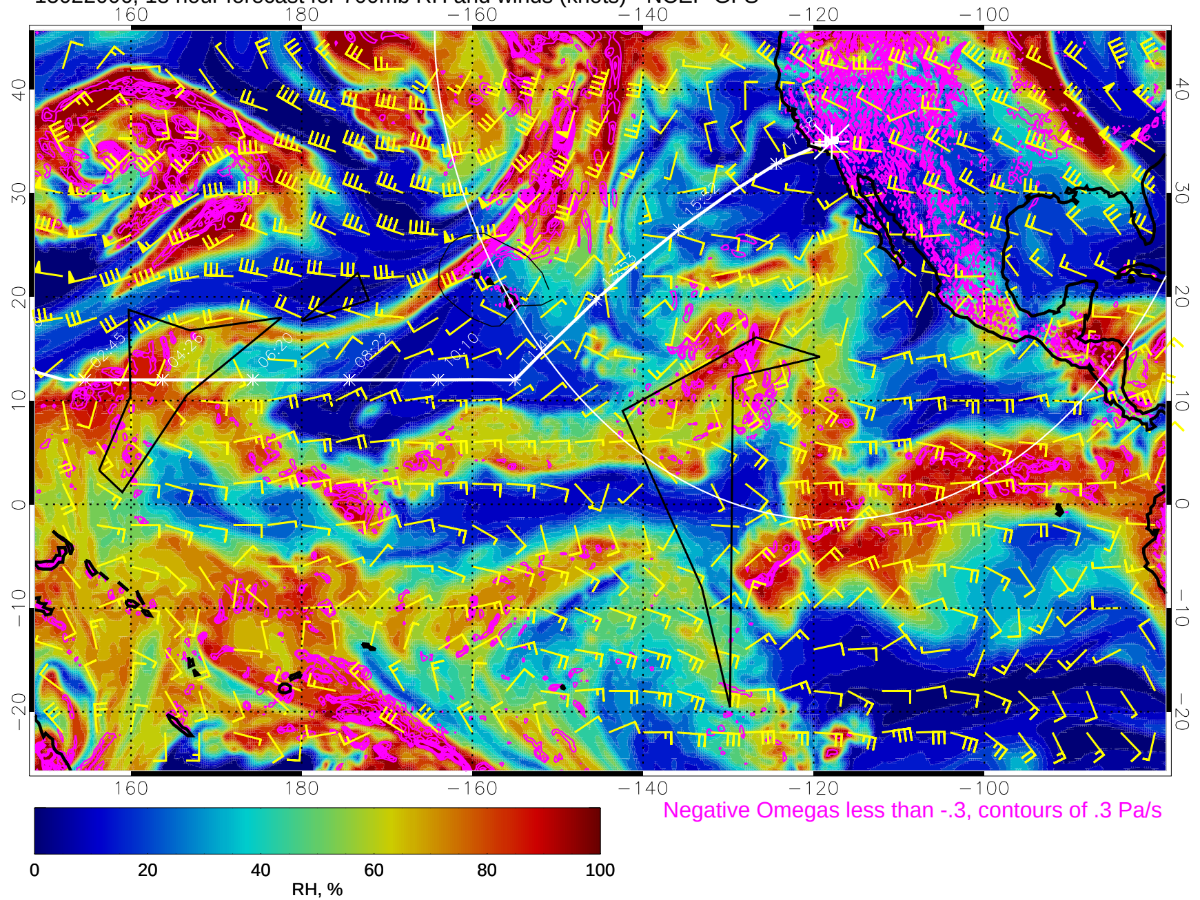
15022006, 18 hour forecast for 700mb RH and winds (knots) - NCEP GFS
