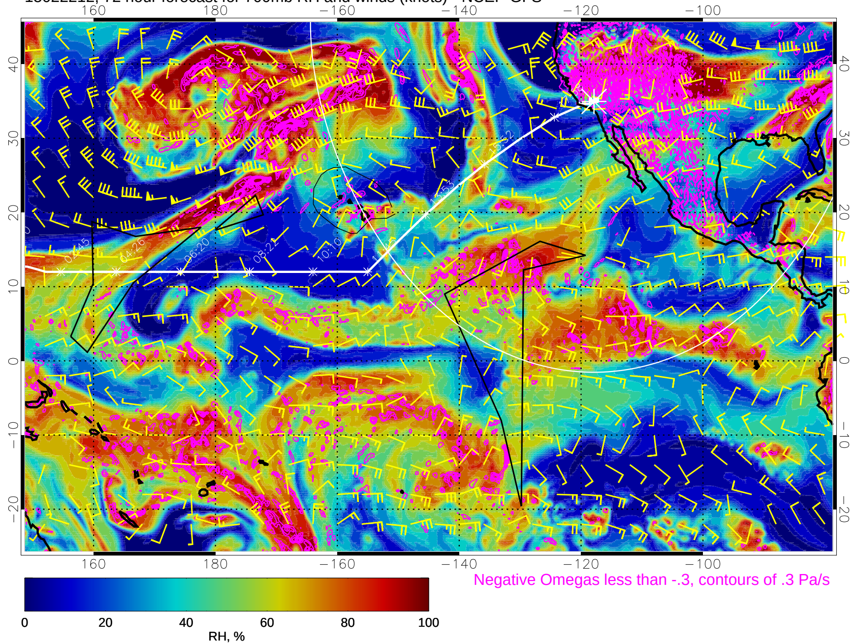
15022212, 72 hour forecast for 700mb RH and winds (knots) - NCEP GFS
