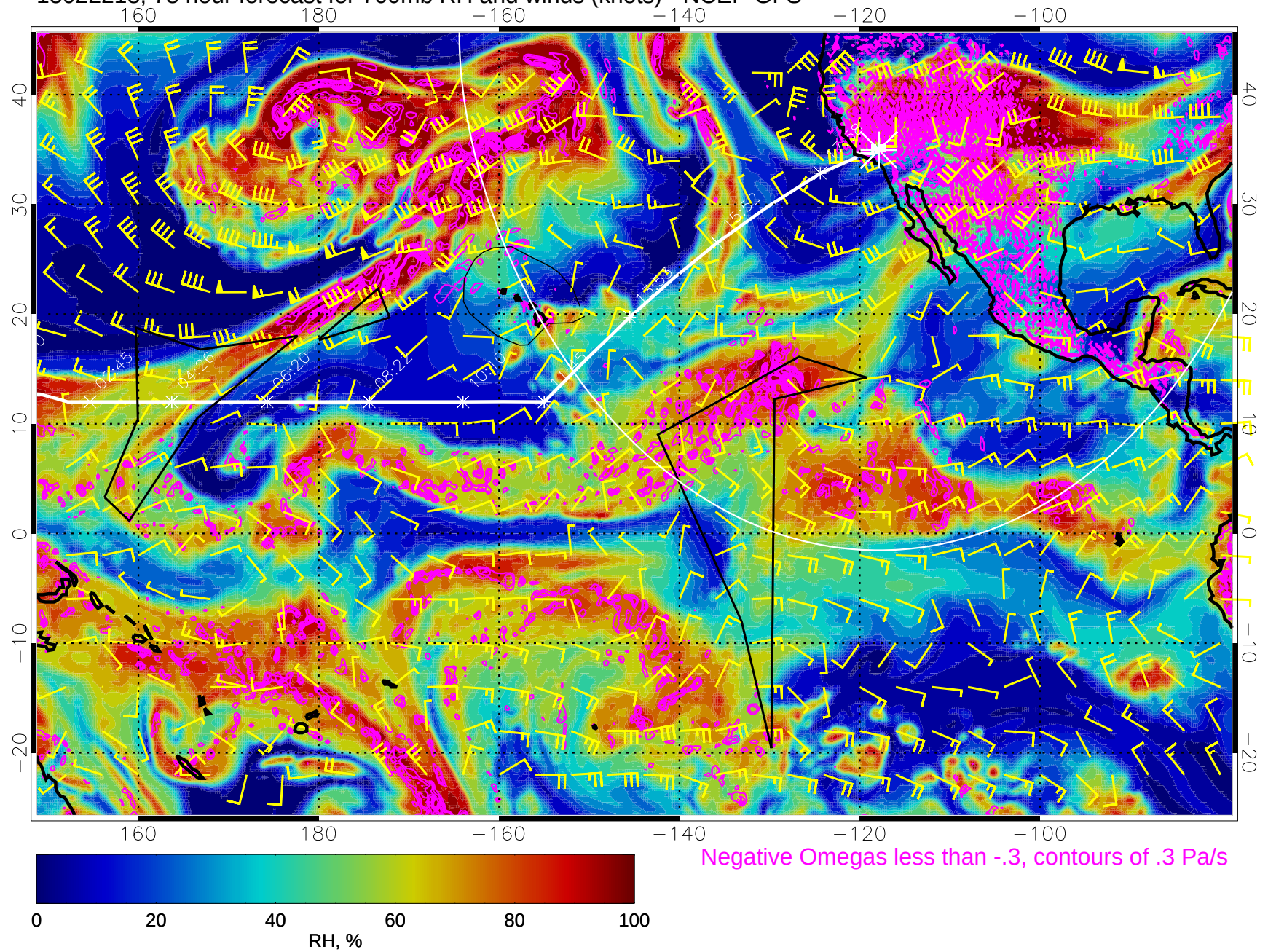
15022218, 78 hour forecast for 700mb RH and winds (knots) - NCEP GFS
