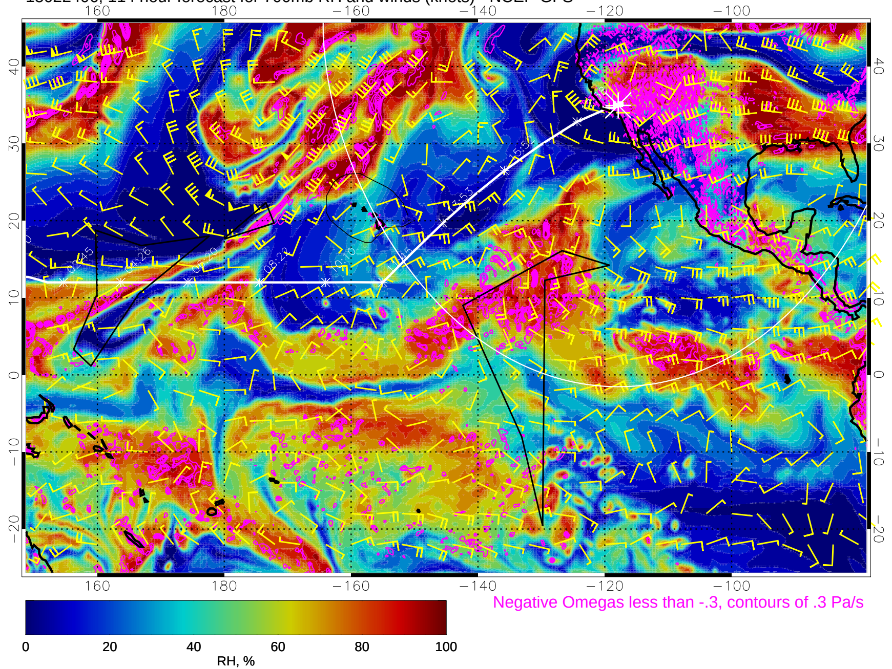
15022406, 114 hour forecast for 700mb RH and winds (knots) - NCEP GFS
