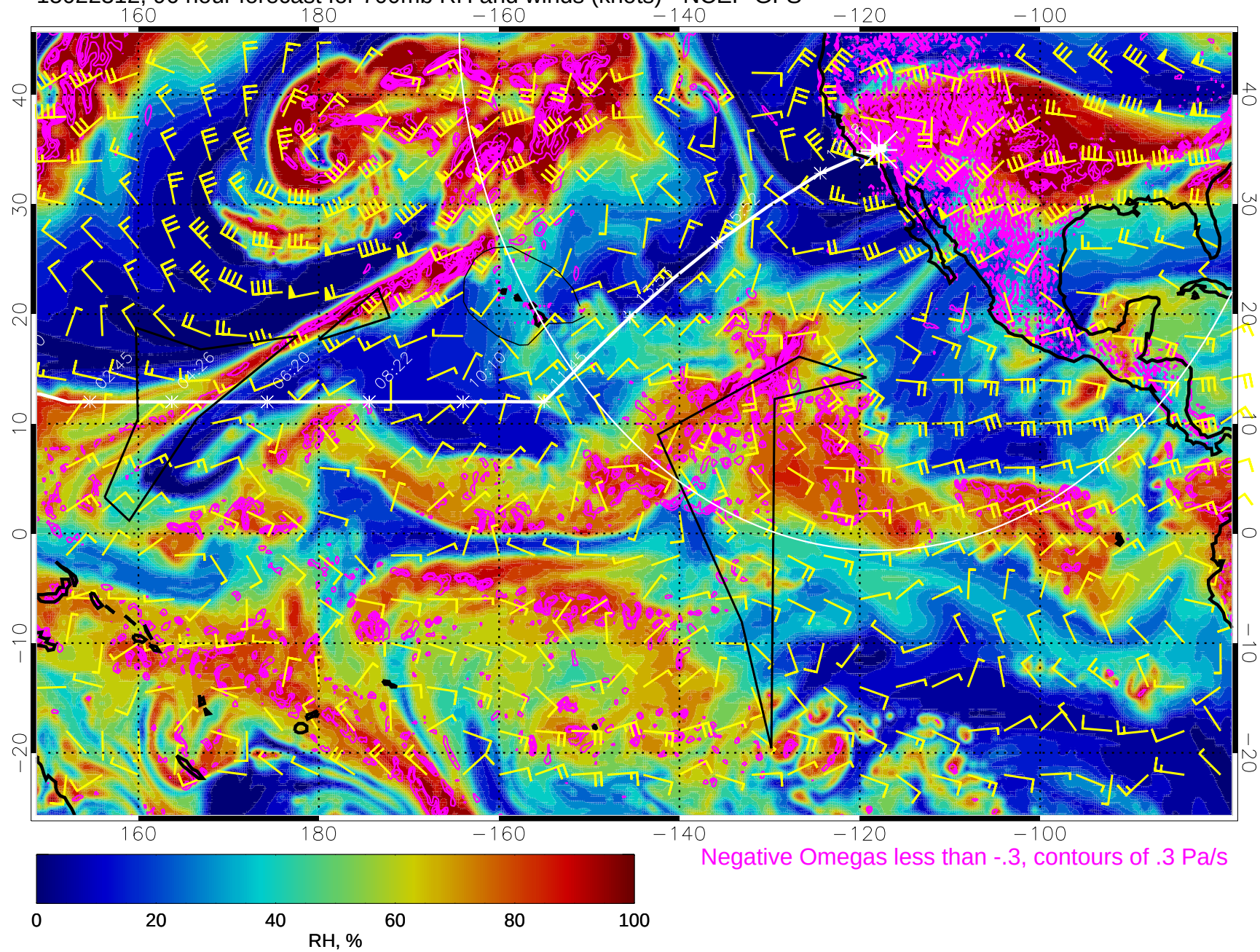
15022312, 96 hour forecast for 700mb RH and winds (knots) - NCEP GFS
