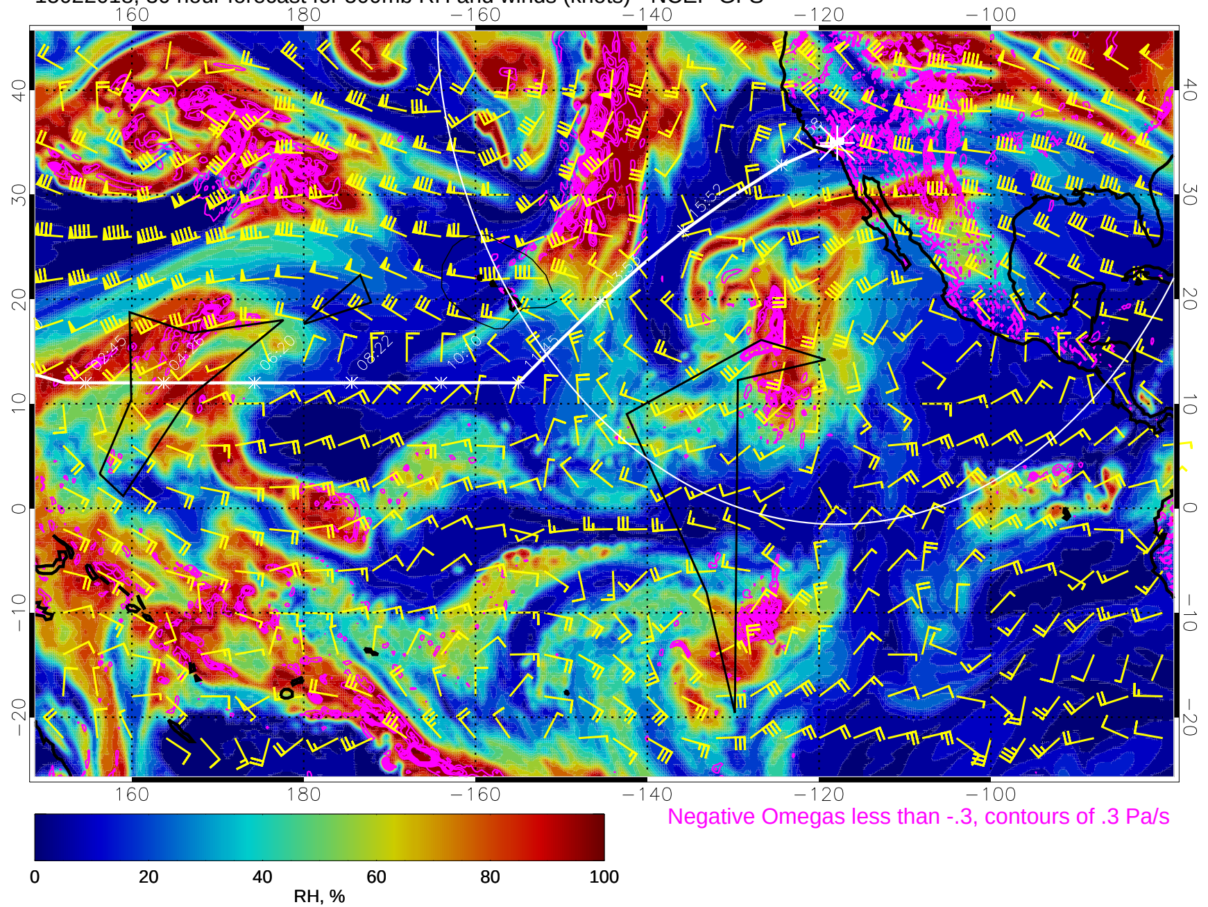
15022018, 30 hour forecast for 500mb RH and winds (knots) - NCEP GFS
