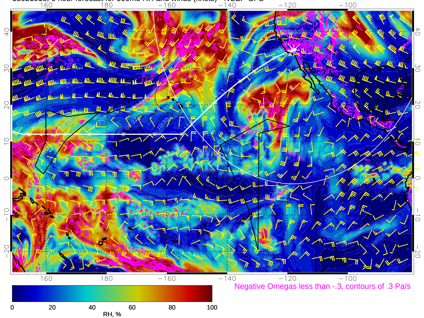
15021918, 6 hour forecast for 500mb RH and winds (knots) - NCEP GFS
