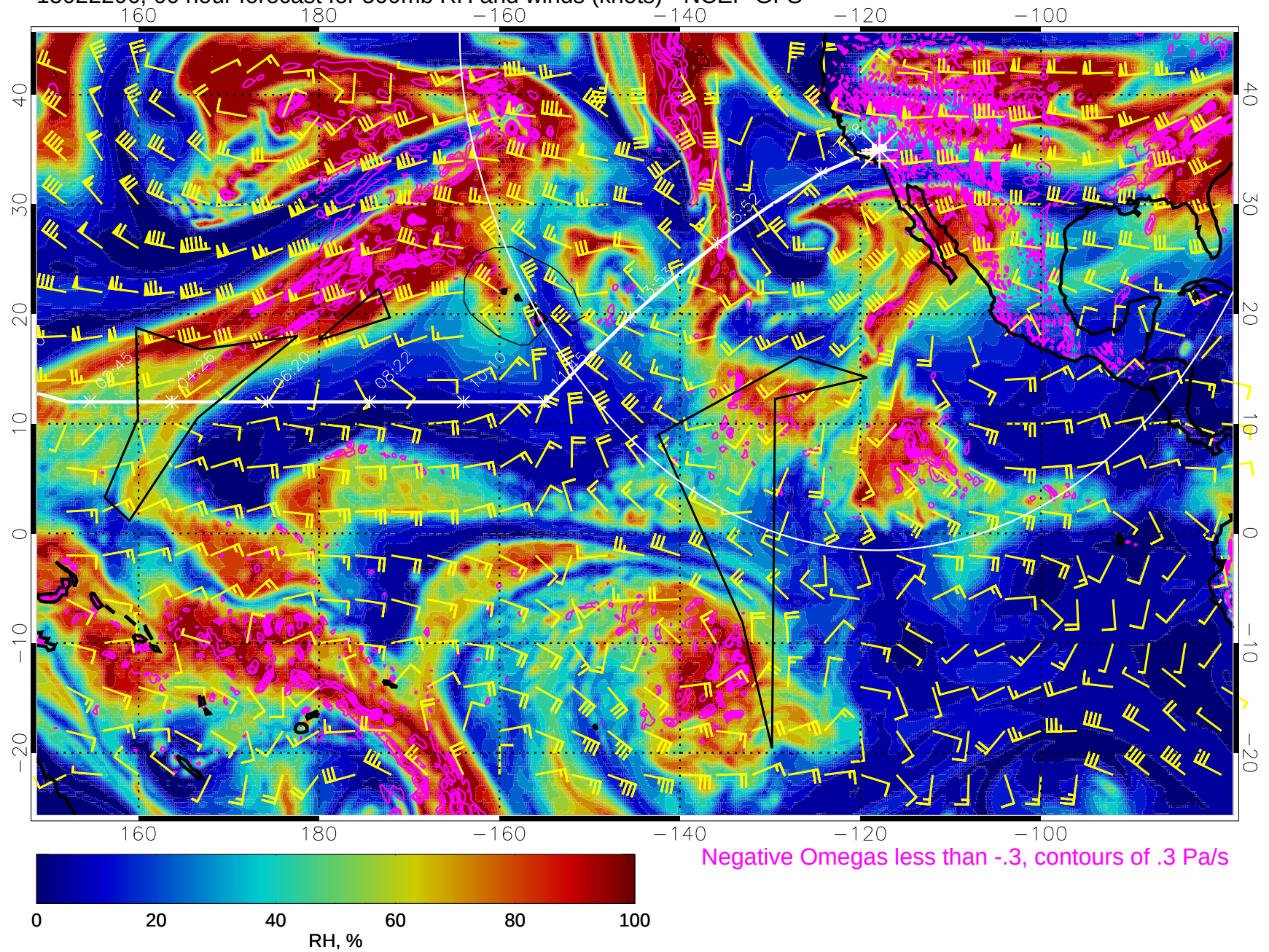
15022206, 66 hour forecast for 500mb RH and winds (knots) - NCEP GFS
