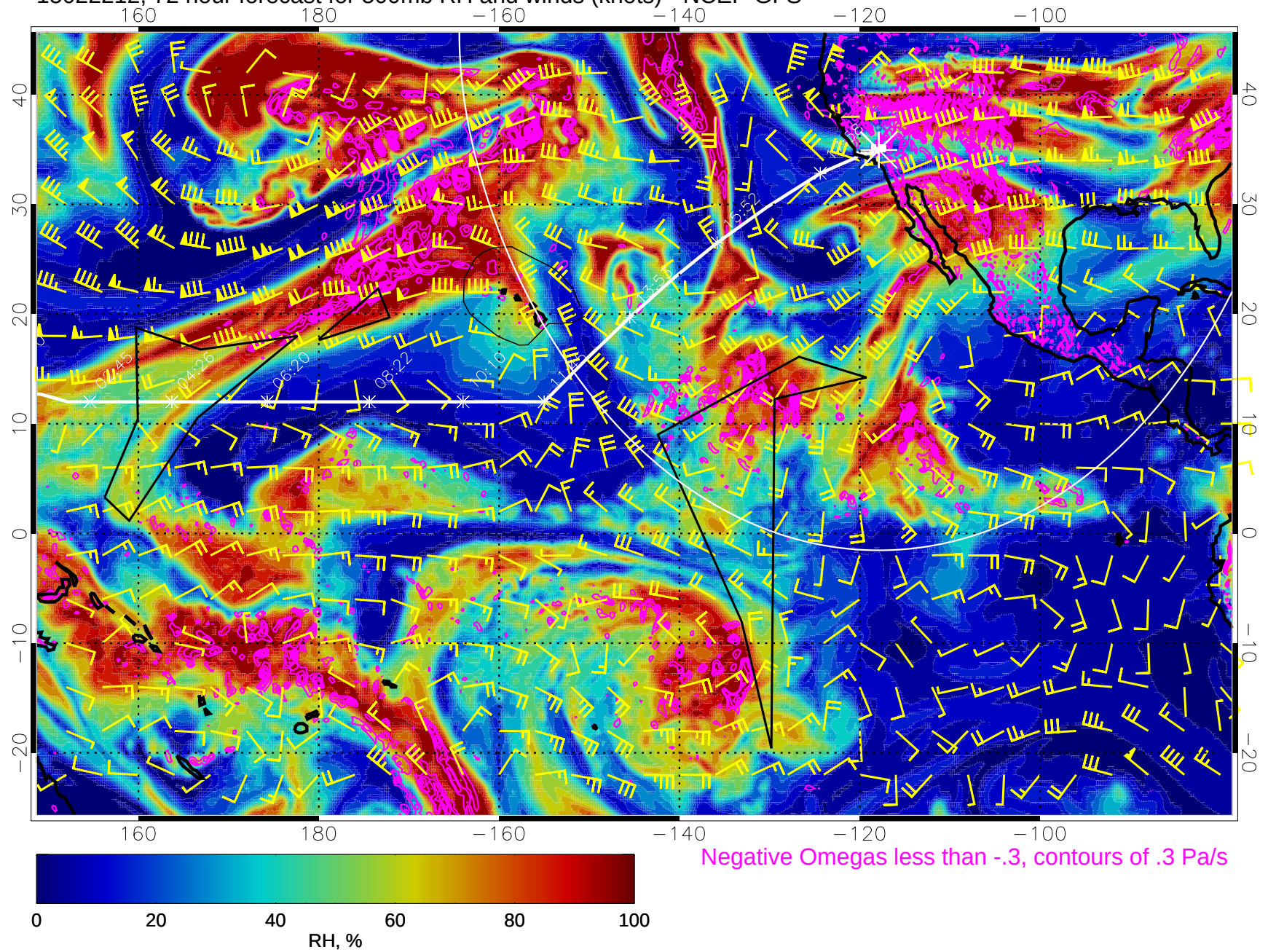
15022212, 72 hour forecast for 500mb RH and winds (knots) - NCEP GFS
