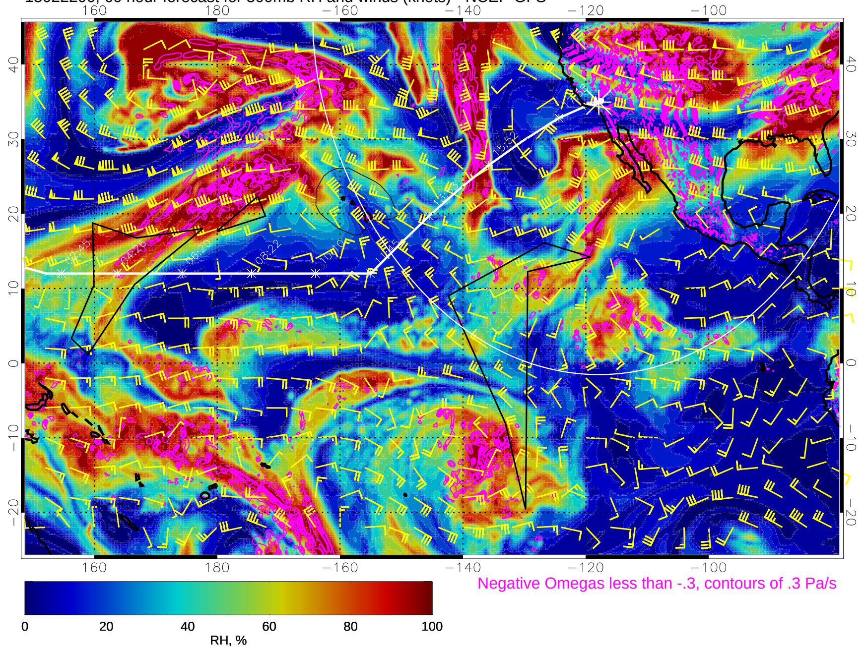
15022200, 60 hour forecast for 500mb RH and winds (knots) - NCEP GFS
