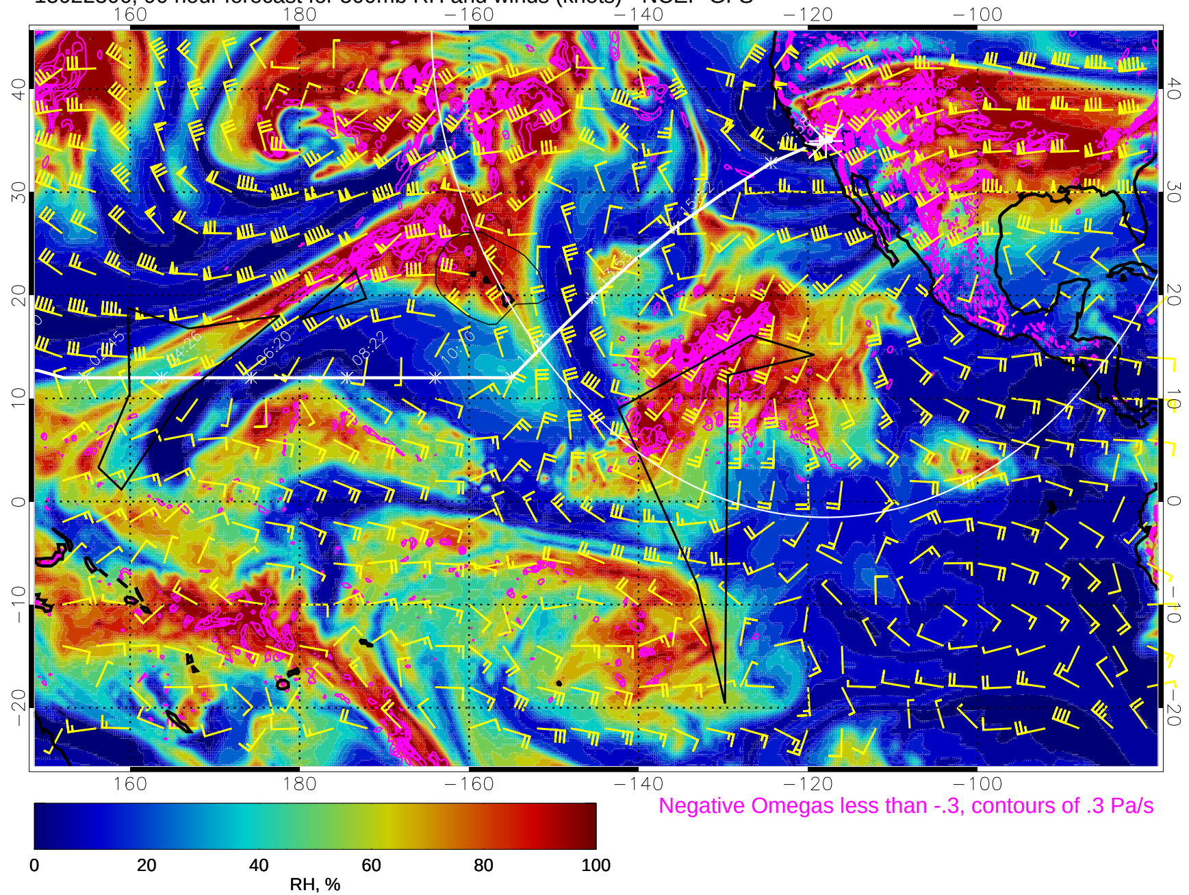
15022306, 90 hour forecast for 500mb RH and winds (knots) - NCEP GFS
