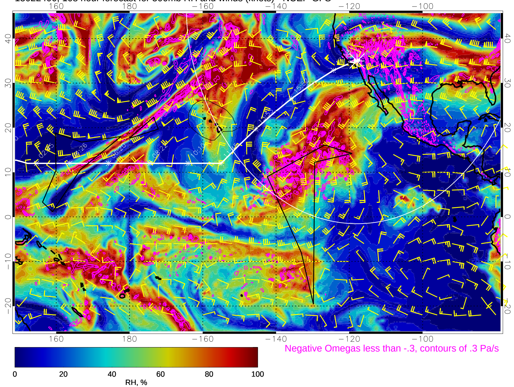
15022400, 108 hour forecast for 500mb RH and winds (knots) - NCEP GFS
