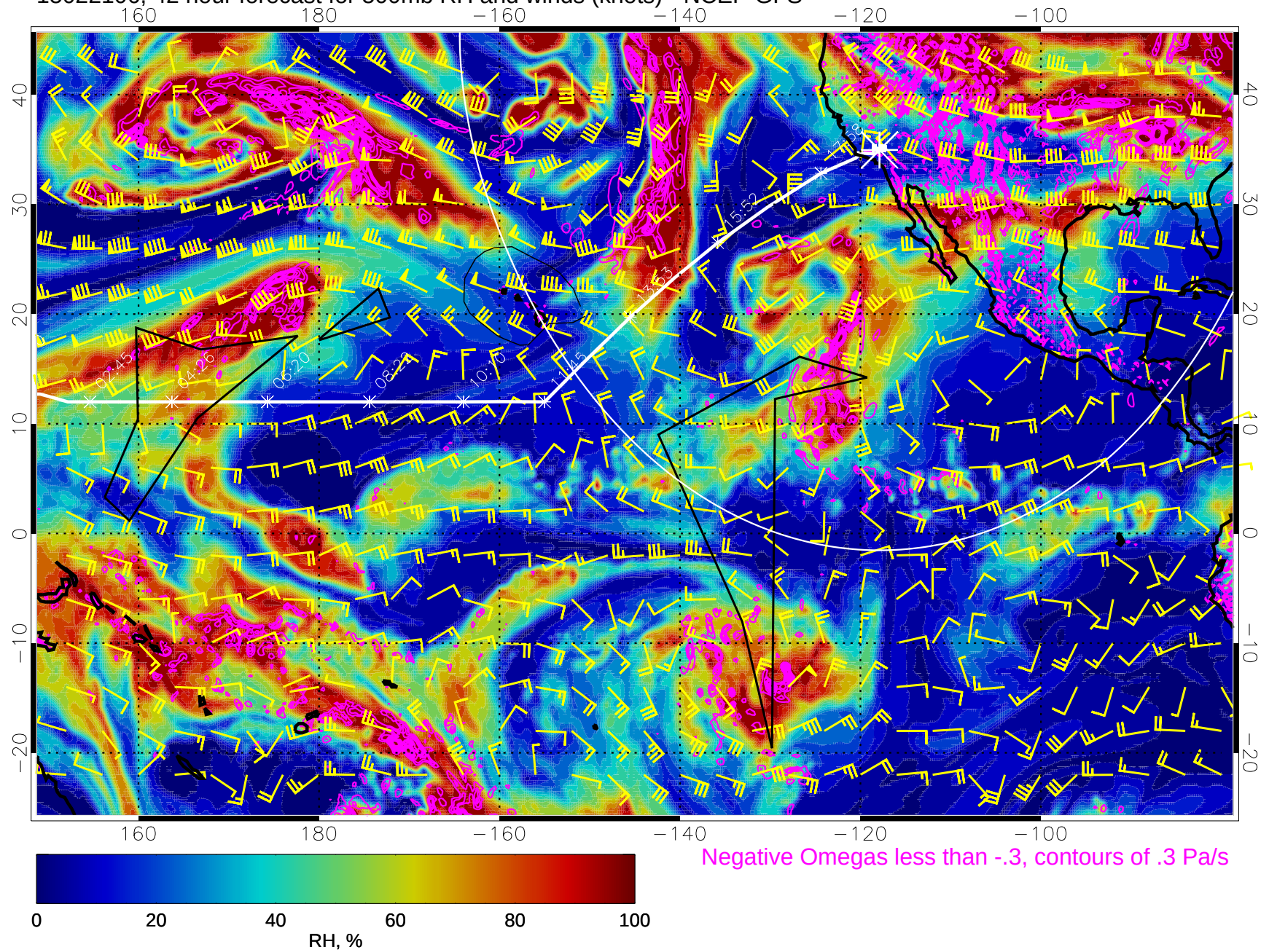
15022106, 42 hour forecast for 500mb RH and winds (knots) - NCEP GFS
