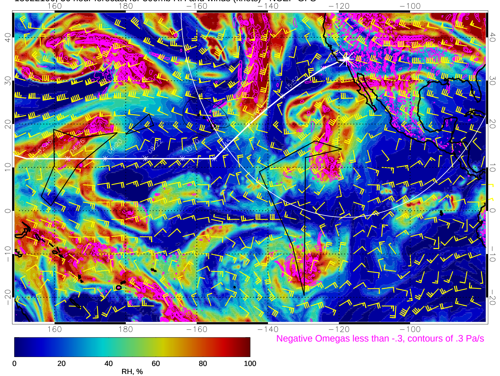
15022100, 36 hour forecast for 500mb RH and winds (knots) - NCEP GFS
