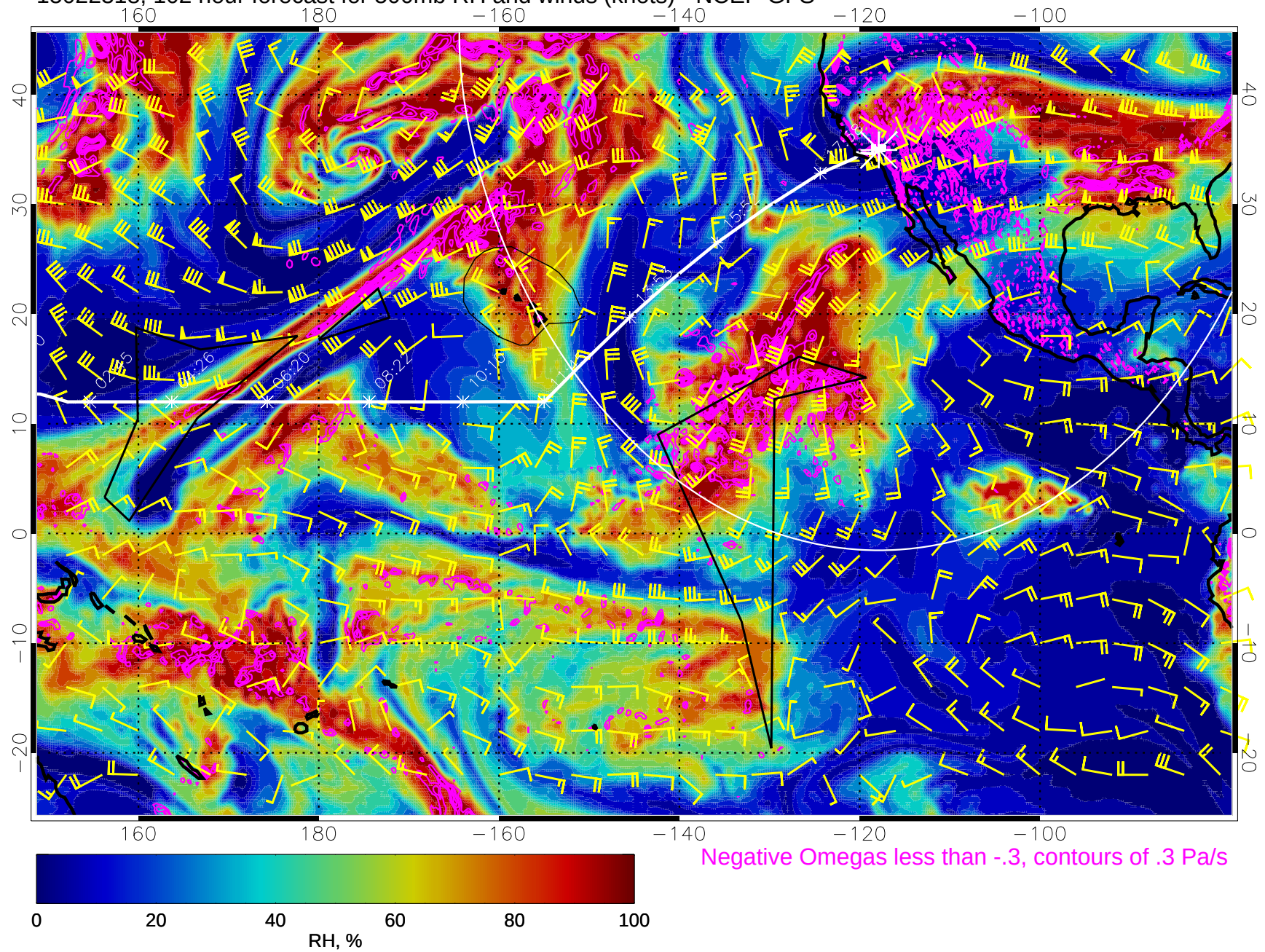
15022318, 102 hour forecast for 500mb RH and winds (knots) - NCEP GFS
