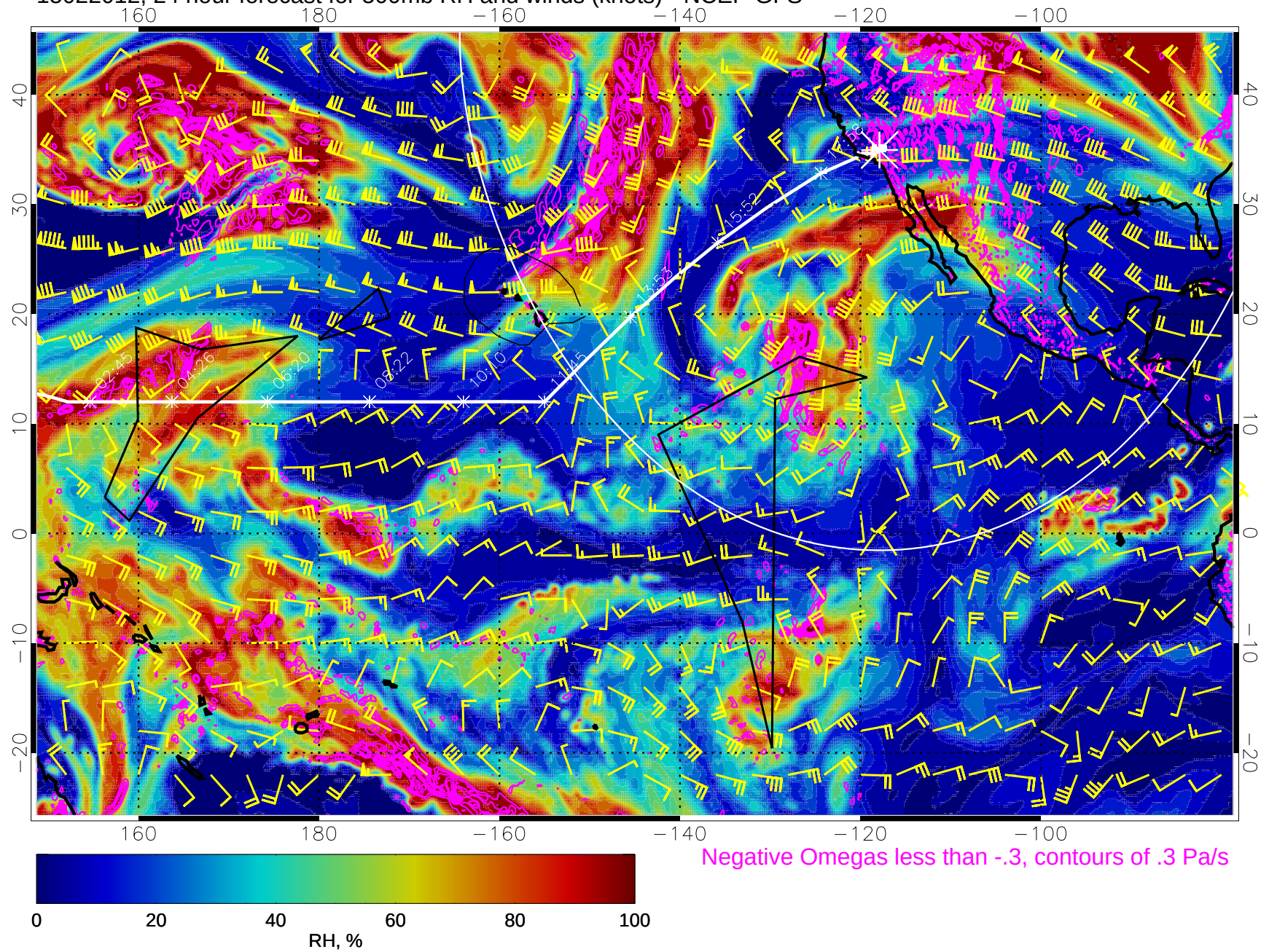
15022012, 24 hour forecast for 500mb RH and winds (knots) - NCEP GFS
