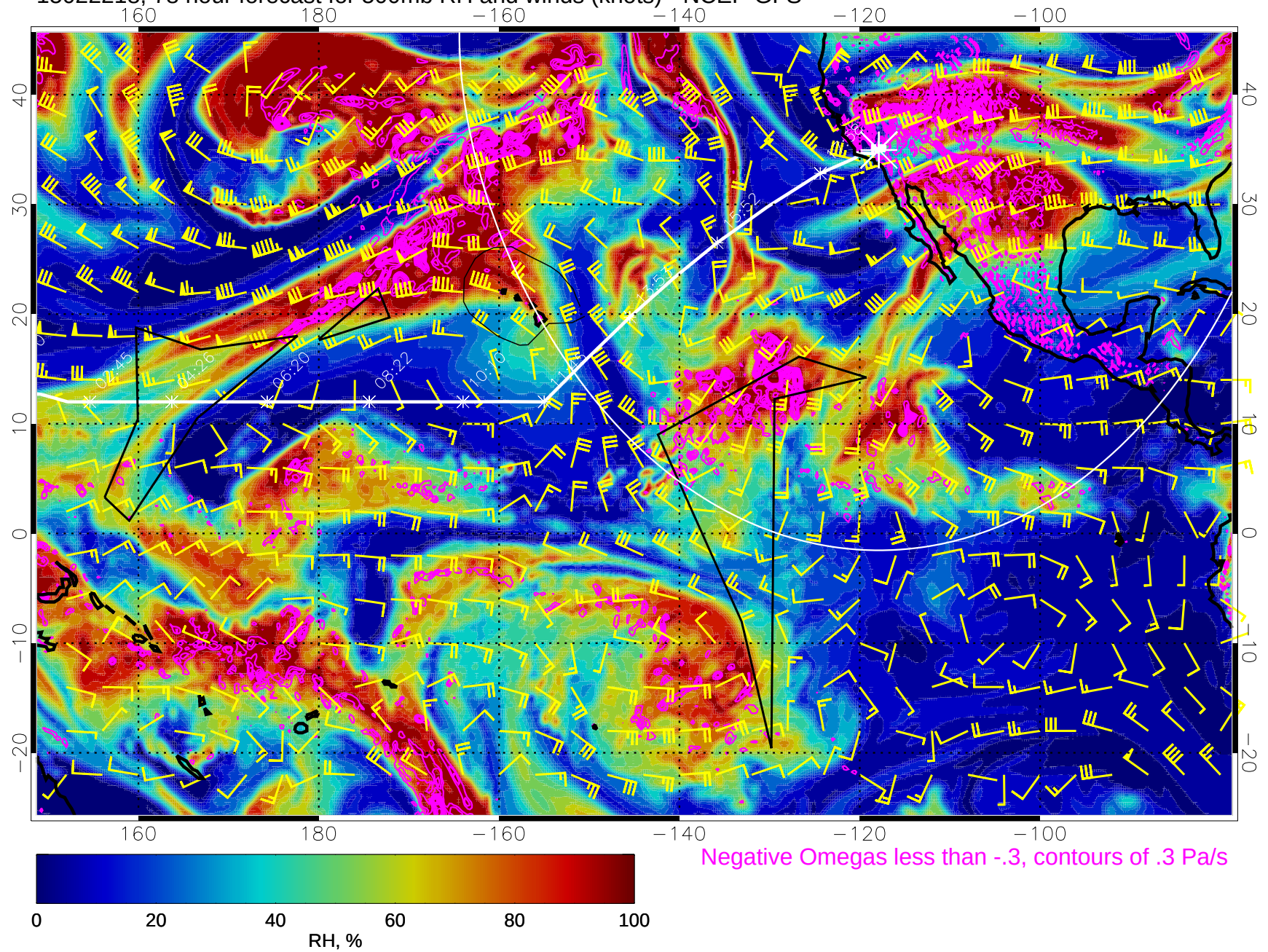
15022218, 78 hour forecast for 500mb RH and winds (knots) - NCEP GFS
