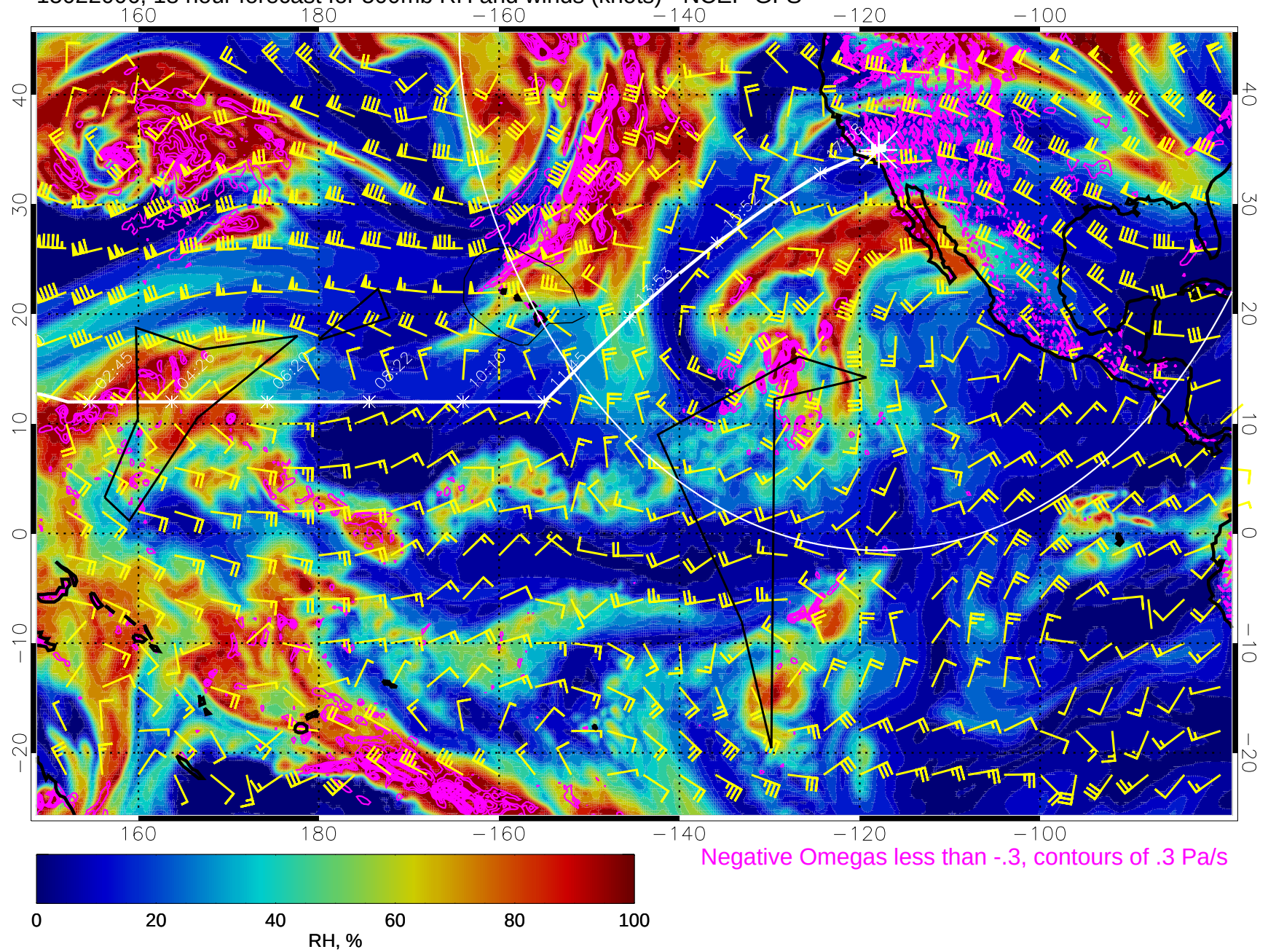
15022006, 18 hour forecast for 500mb RH and winds (knots) - NCEP GFS
