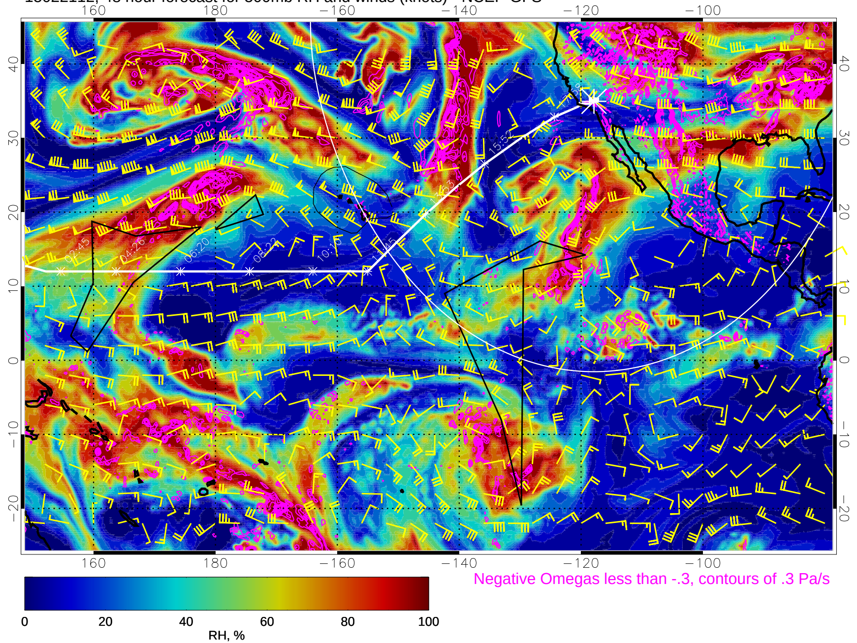
15022112, 48 hour forecast for 500mb RH and winds (knots) - NCEP GFS
