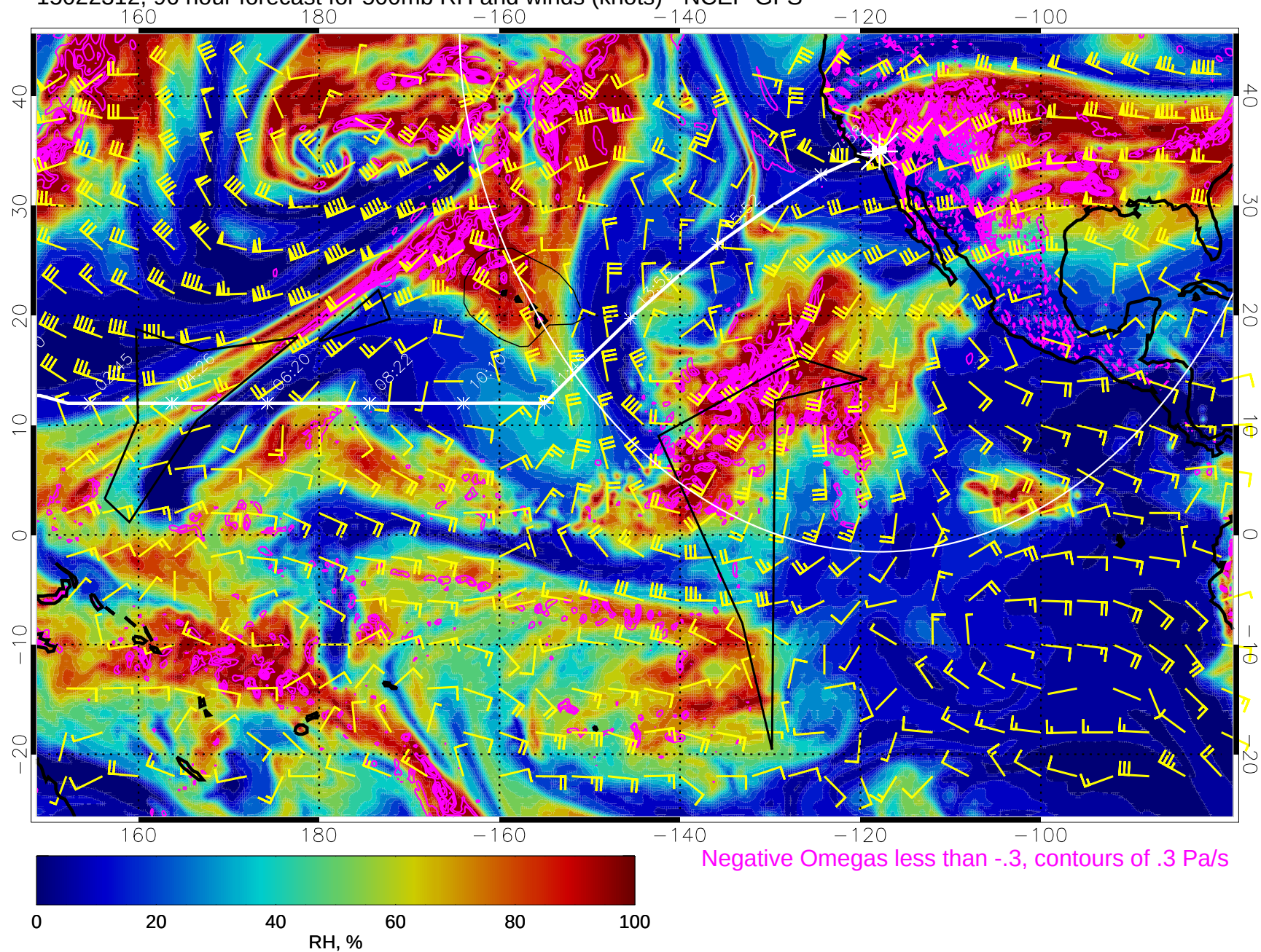
15022312, 96 hour forecast for 500mb RH and winds (knots) - NCEP GFS
