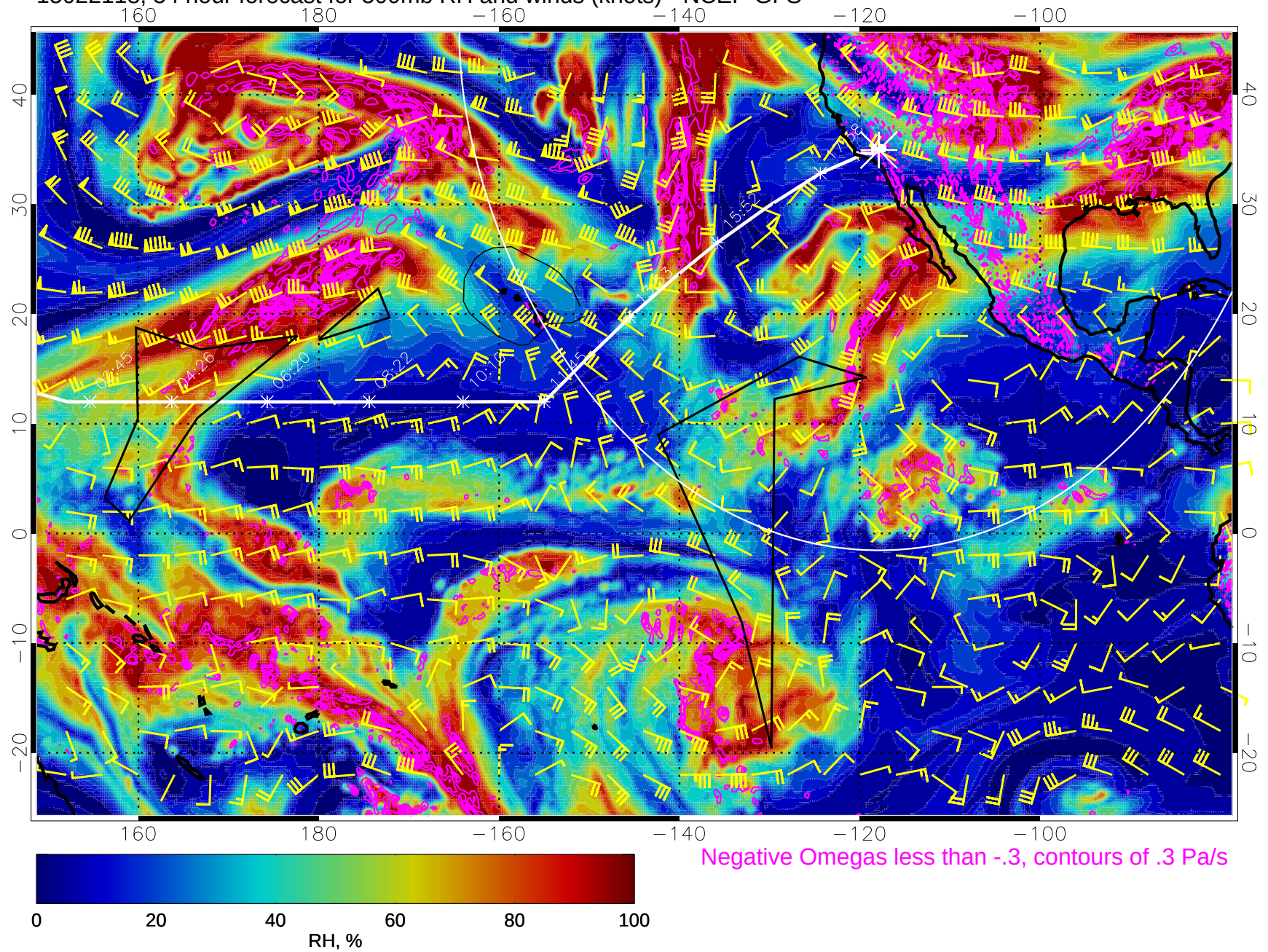
15022118, 54 hour forecast for 500mb RH and winds (knots) - NCEP GFS
