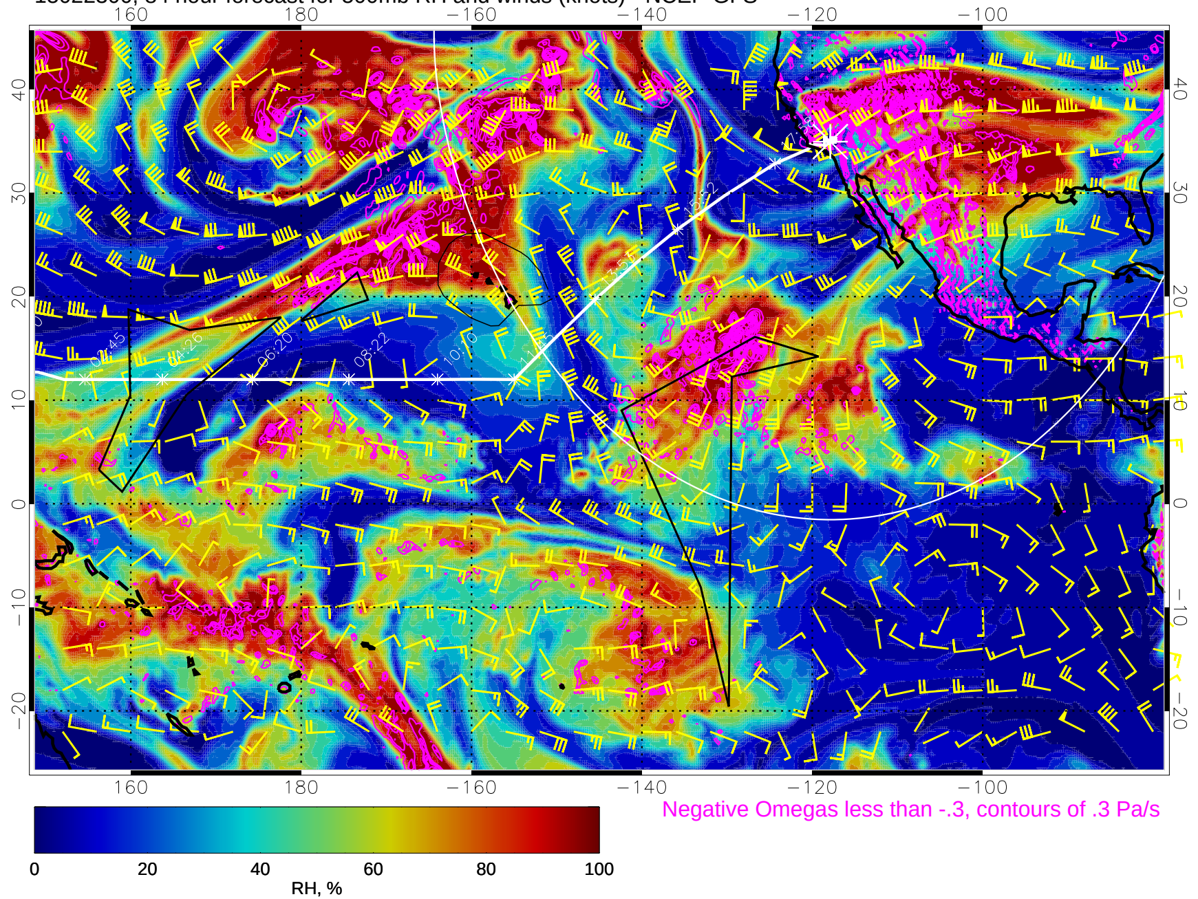
15022300, 84 hour forecast for 500mb RH and winds (knots) - NCEP GFS
