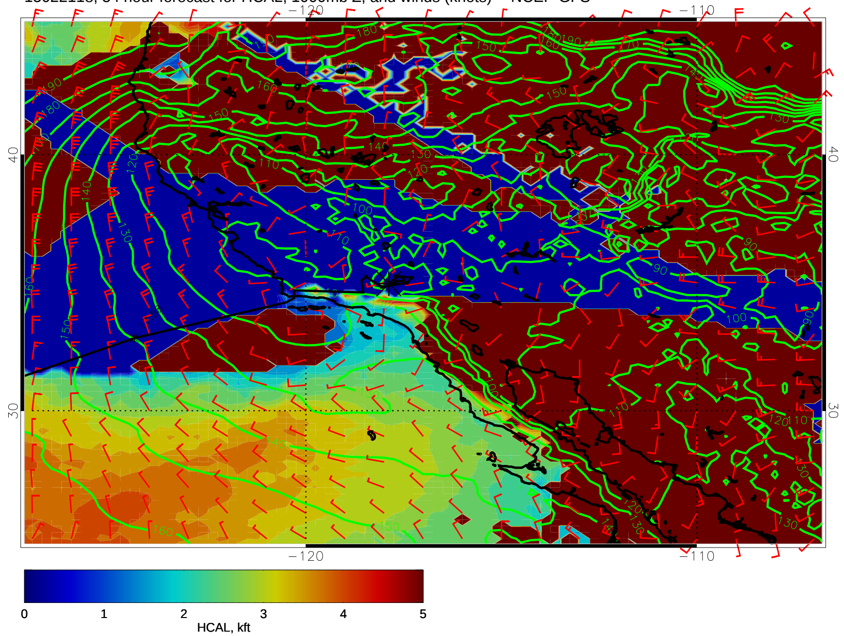
15022118, 54 hour forecast for HCAL, 1000mb Z, and winds (knots) -- NCEP GFS
