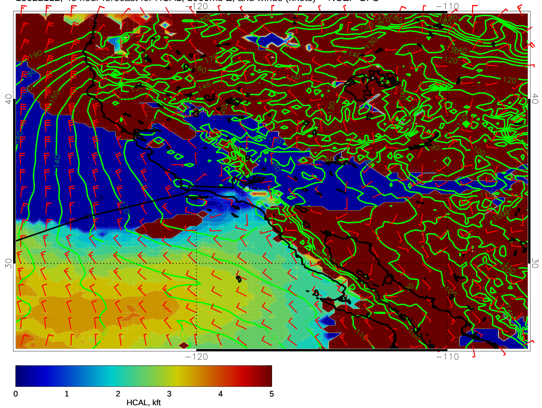
15022112, 48 hour forecast for HCAL, 1000mb Z, and winds (knots) -- NCEP GFS
