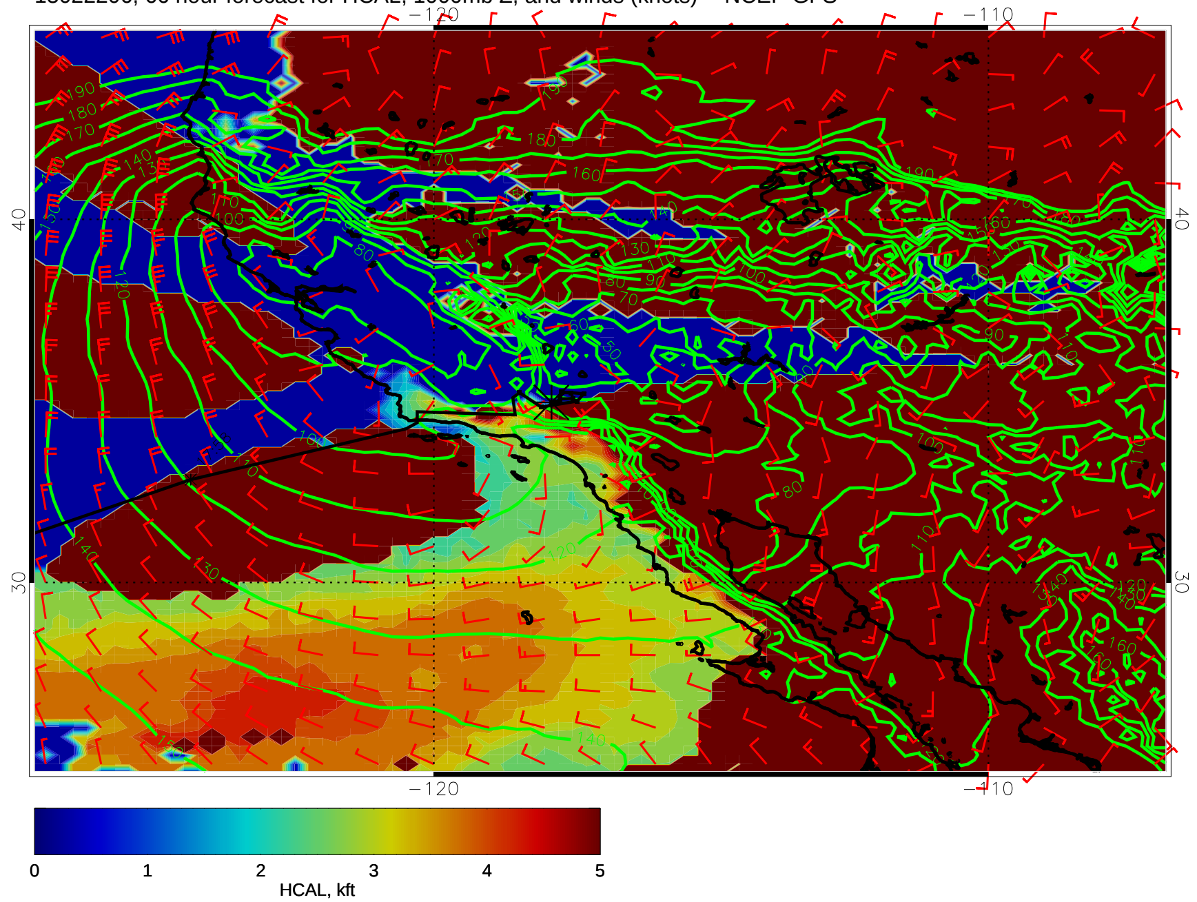
15022206, 66 hour forecast for HCAL, 1000mb Z, and winds (knots) -- NCEP GFS
