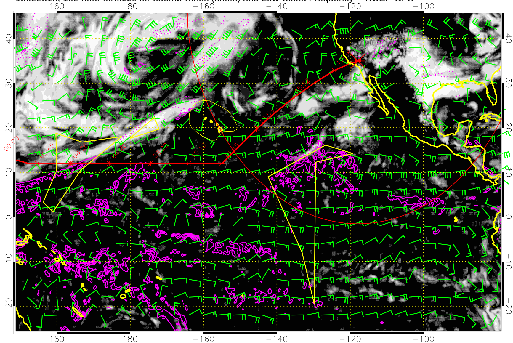
15022318, 102 hour forecast for 850mb winds (knots) and Low Cloud Frequency -- NCEP GFS
