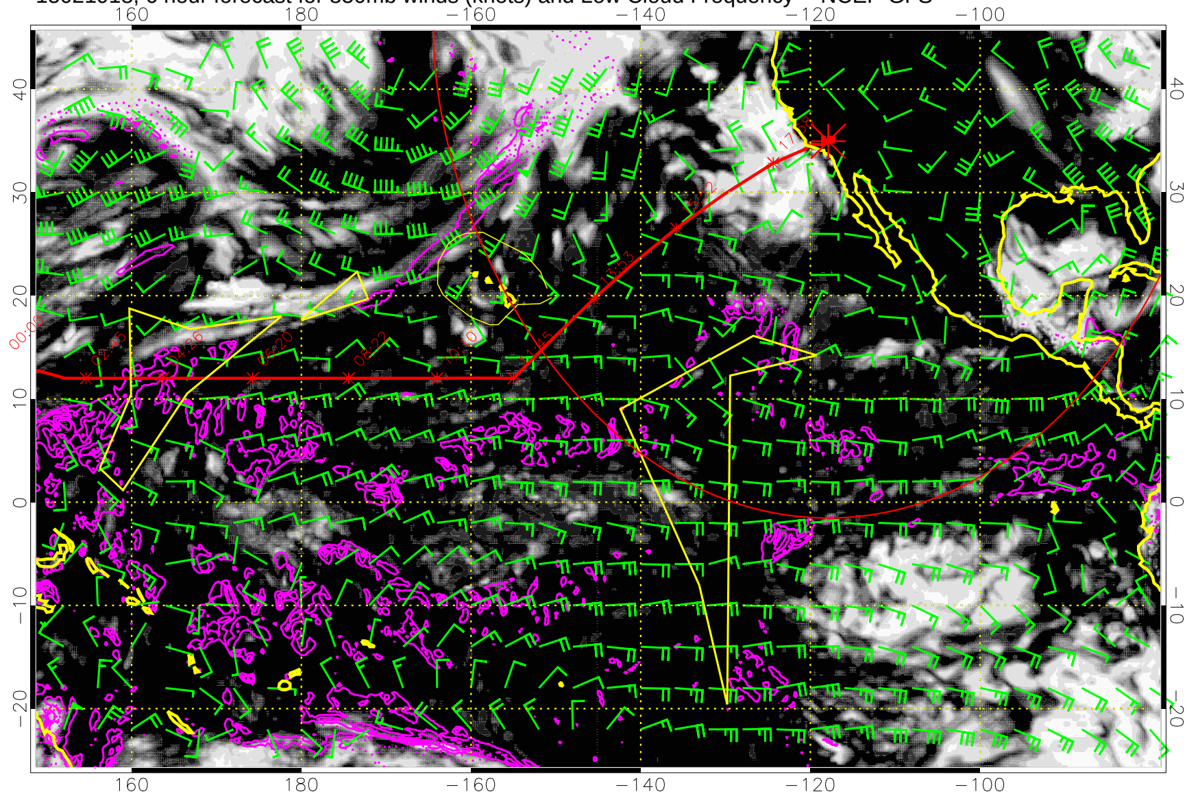
15021918, 6 hour forecast for 850mb winds (knots) and Low Cloud Frequency -- NCEP GFS
