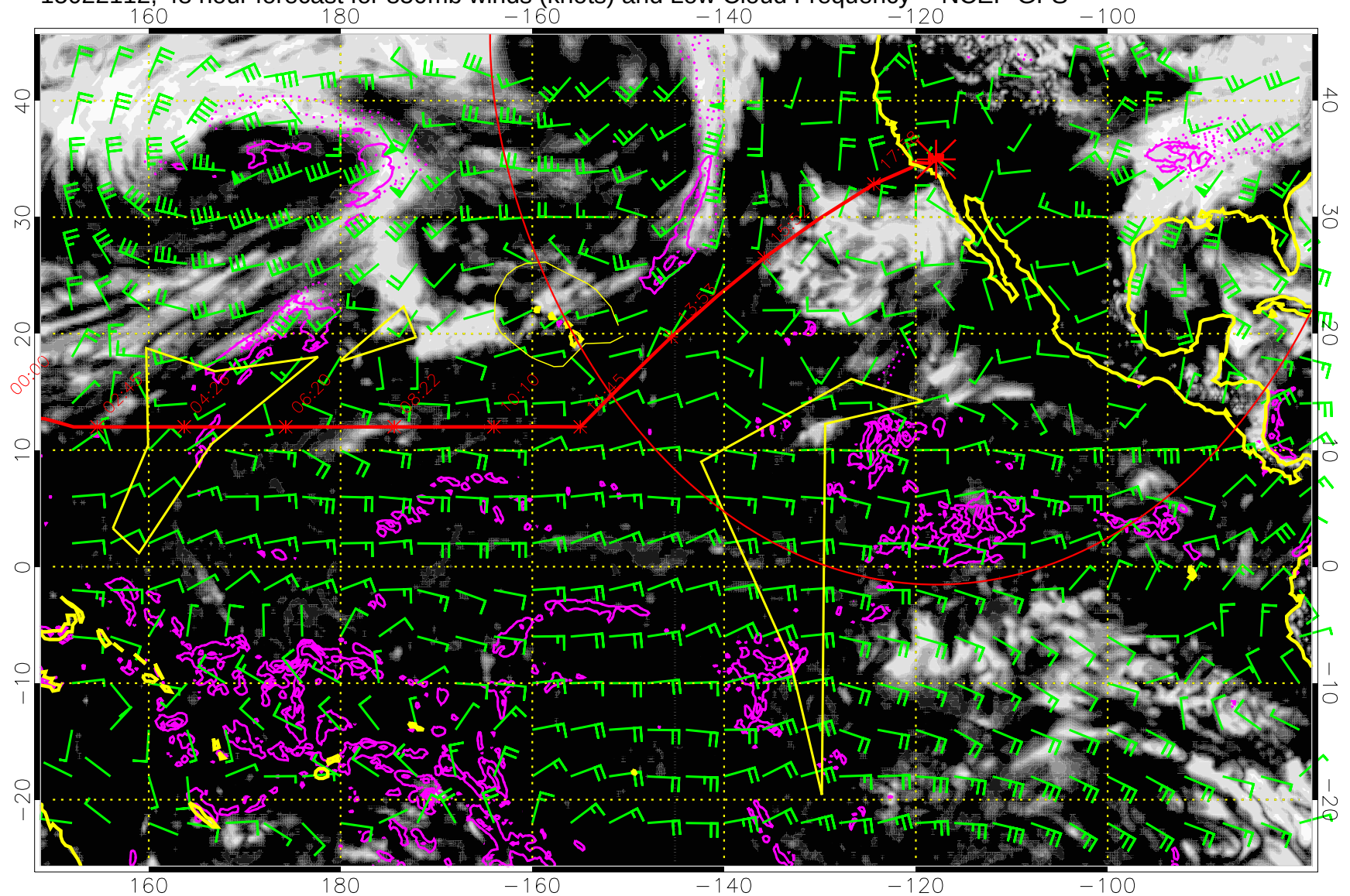
15022112, 48 hour forecast for 850mb winds (knots) and Low Cloud Frequency -- NCEP GFS
