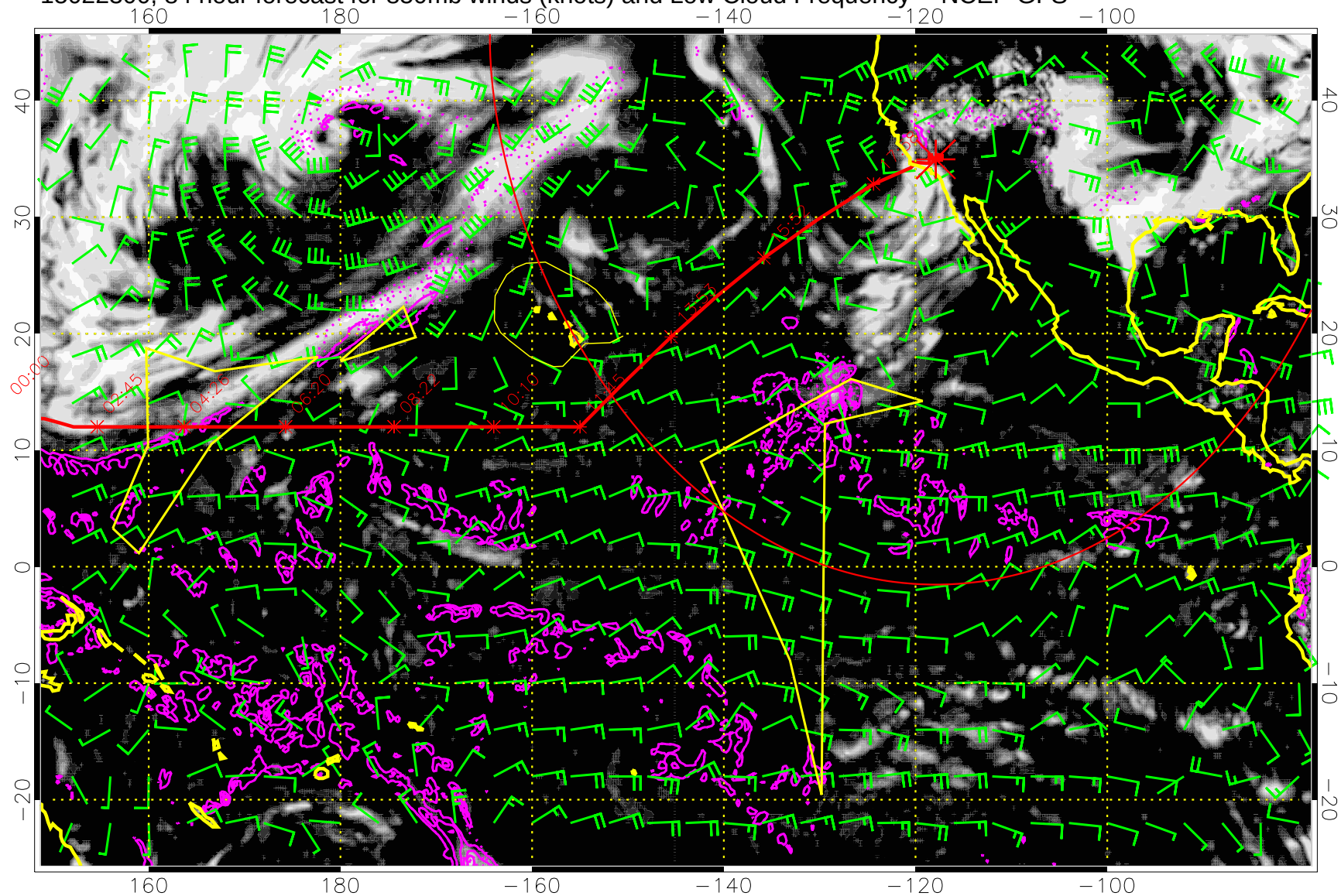
15022300, 84 hour forecast for 850mb winds (knots) and Low Cloud Frequency -- NCEP GFS
