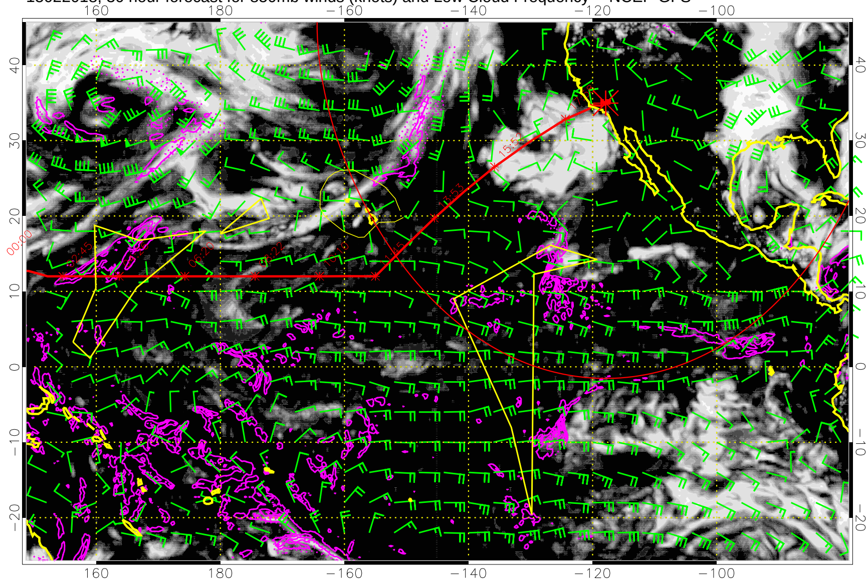
15022018, 30 hour forecast for 850mb winds (knots) and Low Cloud Frequency -- NCEP GFS
