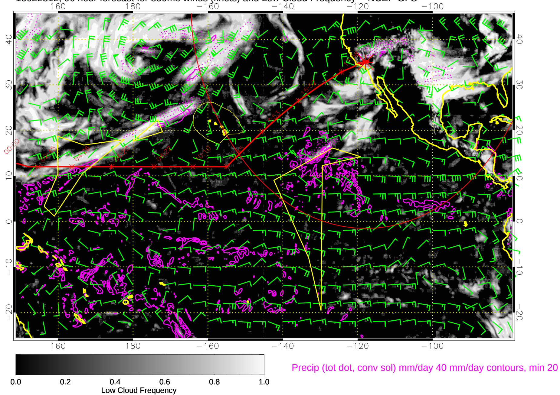
15022312, 96 hour forecast for 850mb winds (knots) and Low Cloud Frequency -- NCEP GFS
