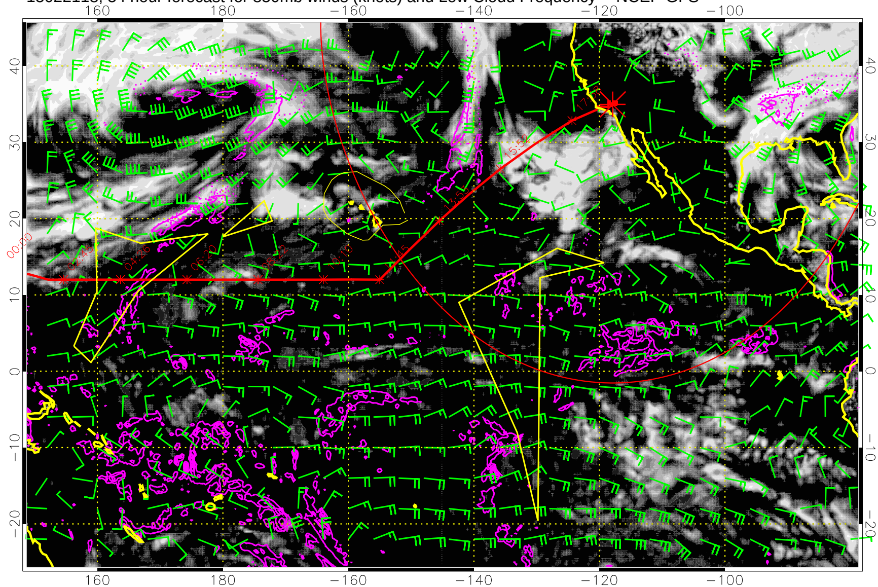
15022118, 54 hour forecast for 850mb winds (knots) and Low Cloud Frequency -- NCEP GFS
