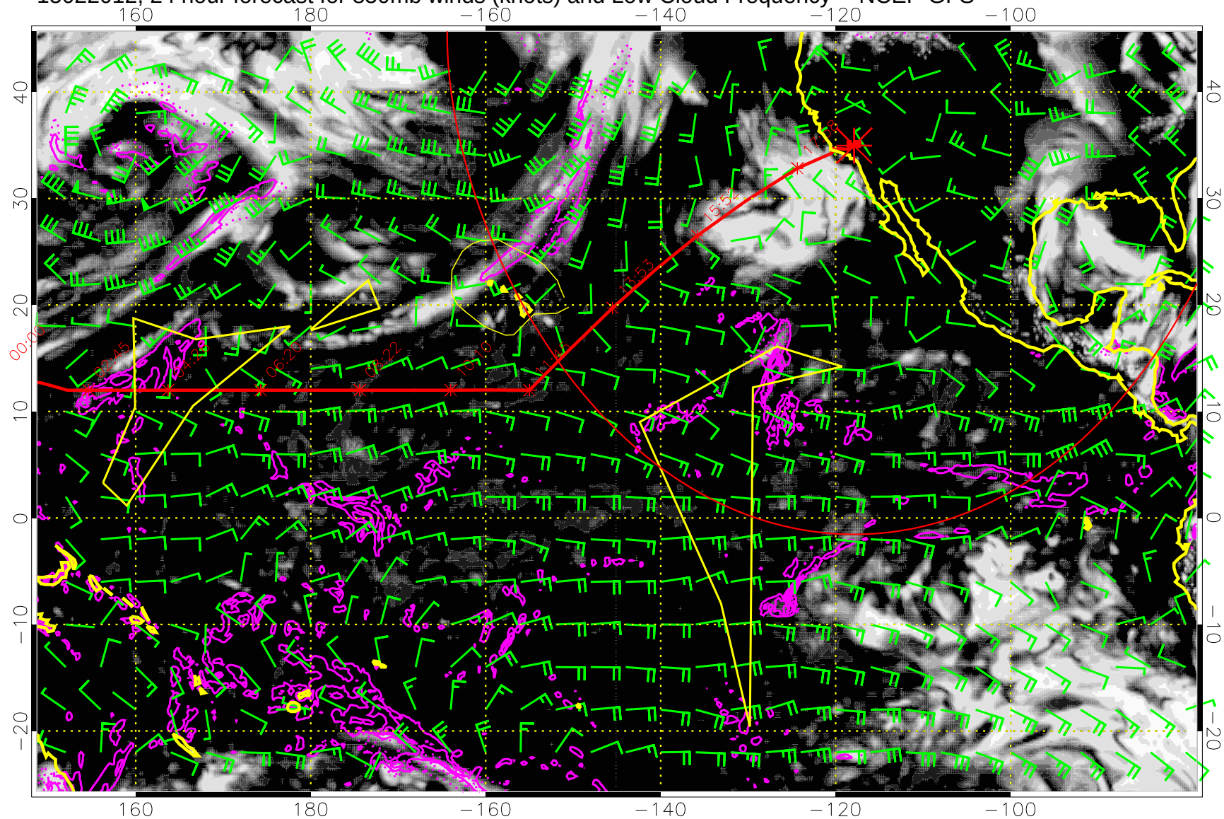
15022012, 24 hour forecast for 850mb winds (knots) and Low Cloud Frequency -- NCEP GFS
