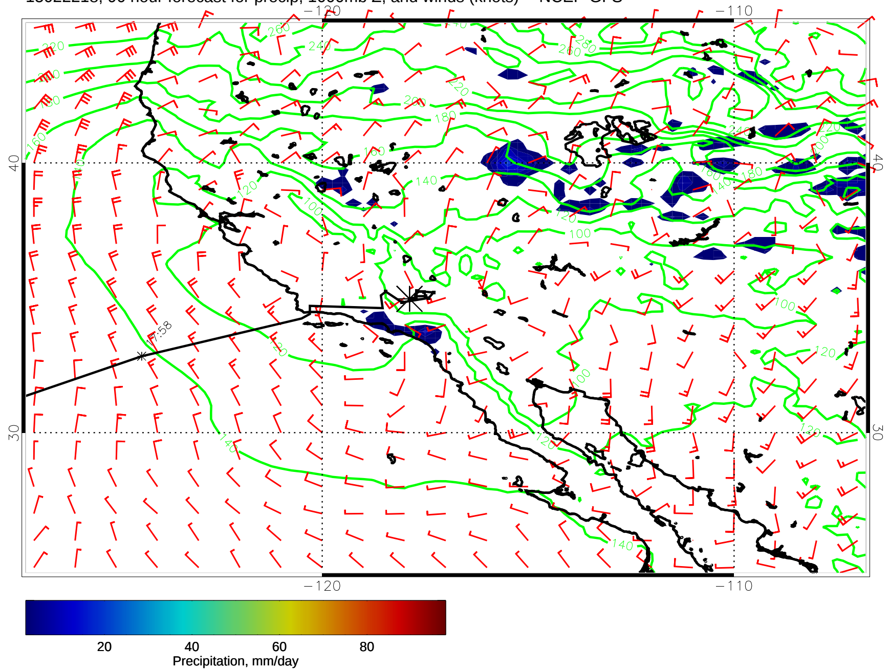
15022218, 90 hour forecast for precip, 1000mb Z, and winds (knots) -- NCEP GFS
