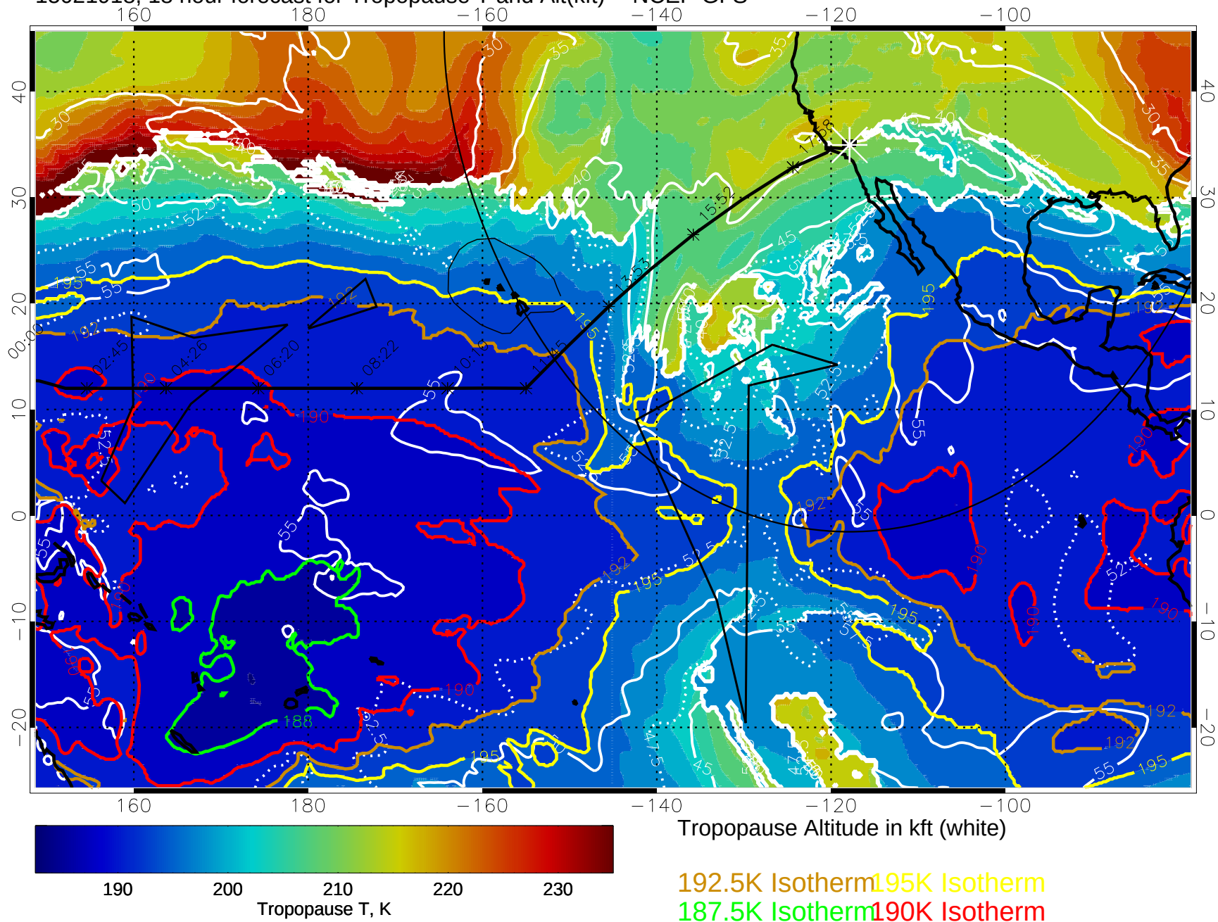
15021918, 18 hour forecast for Tropopause T and Alt(kft) -- NCEP GFS
