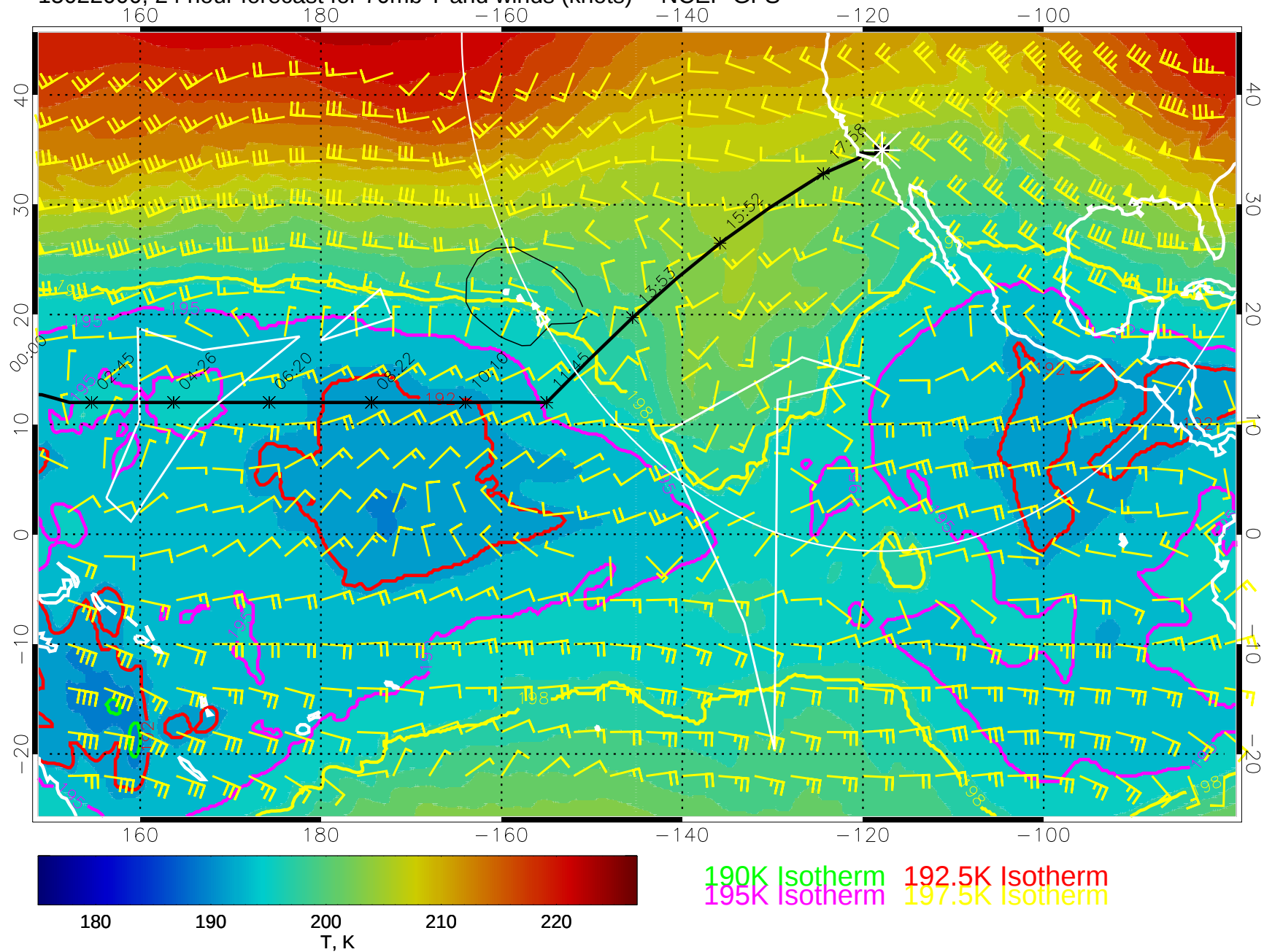
15022000, 24 hour forecast for 70mb T and winds (knots) -- NCEP GFS
