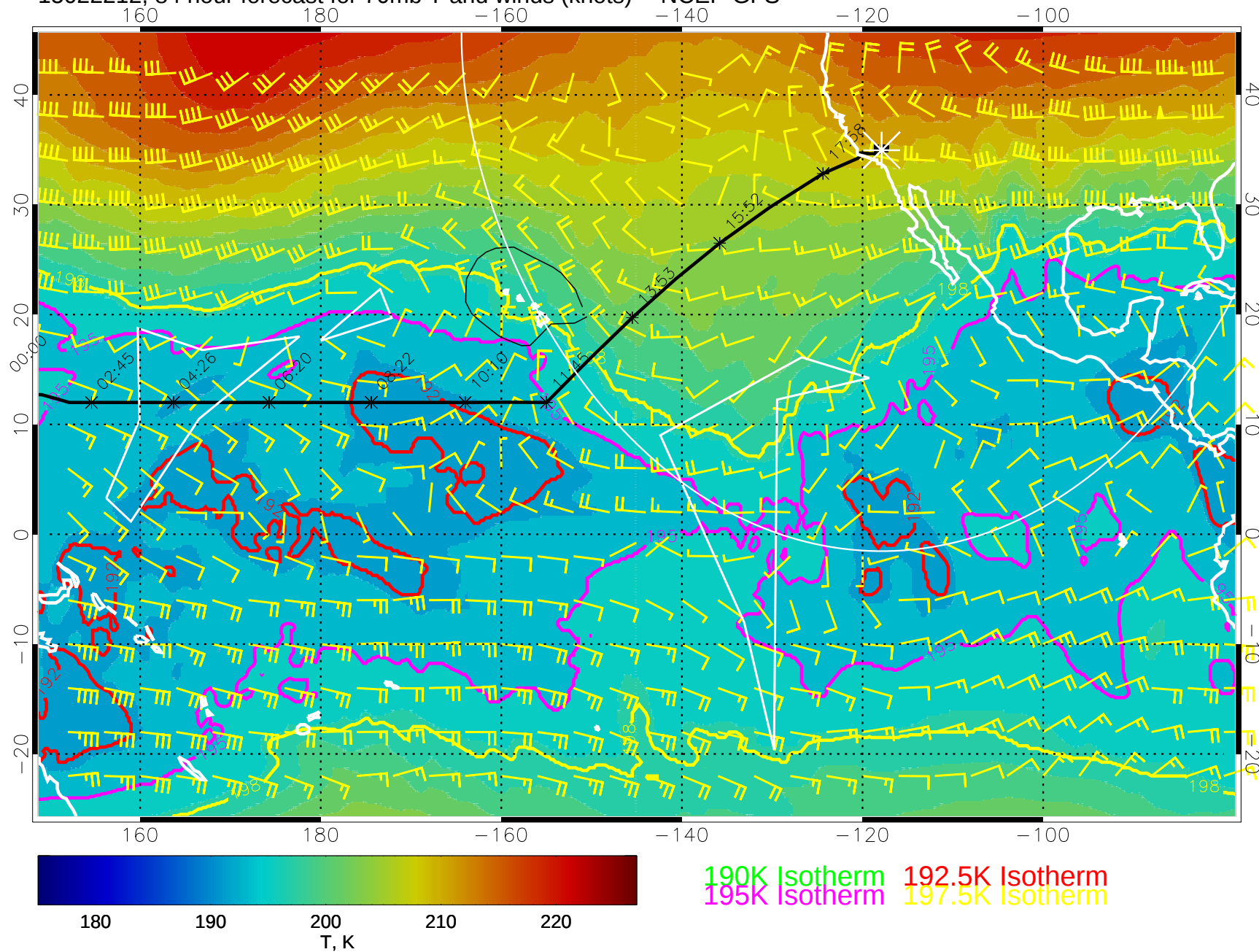
15022212, 84 hour forecast for 70mb T and winds (knots) -- NCEP GFS
