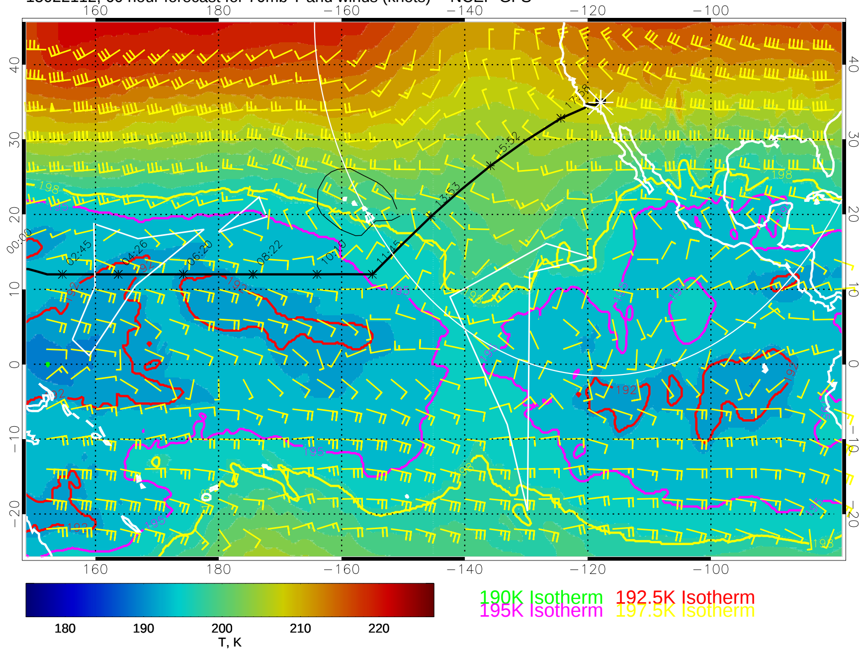
15022112, 60 hour forecast for 70mb T and winds (knots) -- NCEP GFS
