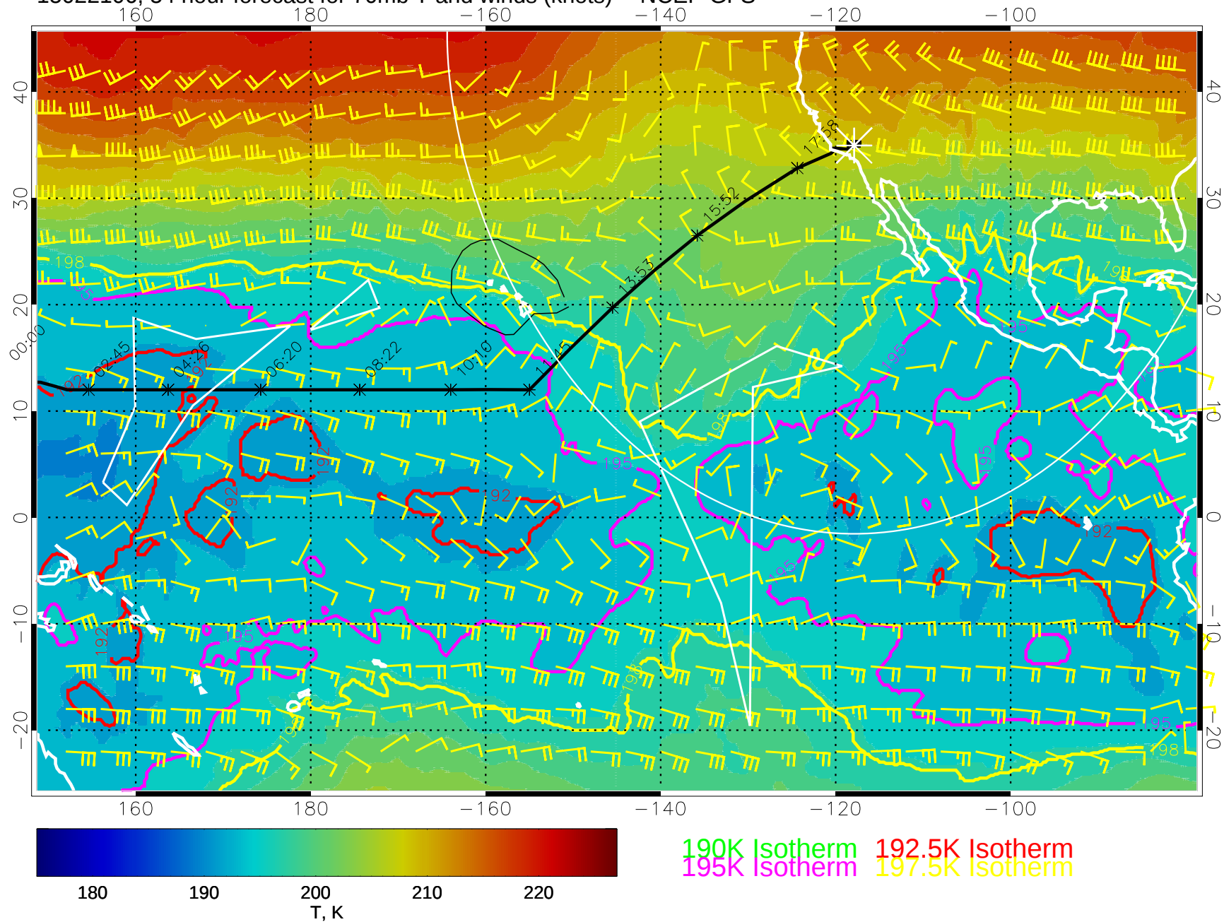
15022106, 54 hour forecast for 70mb T and winds (knots) -- NCEP GFS
