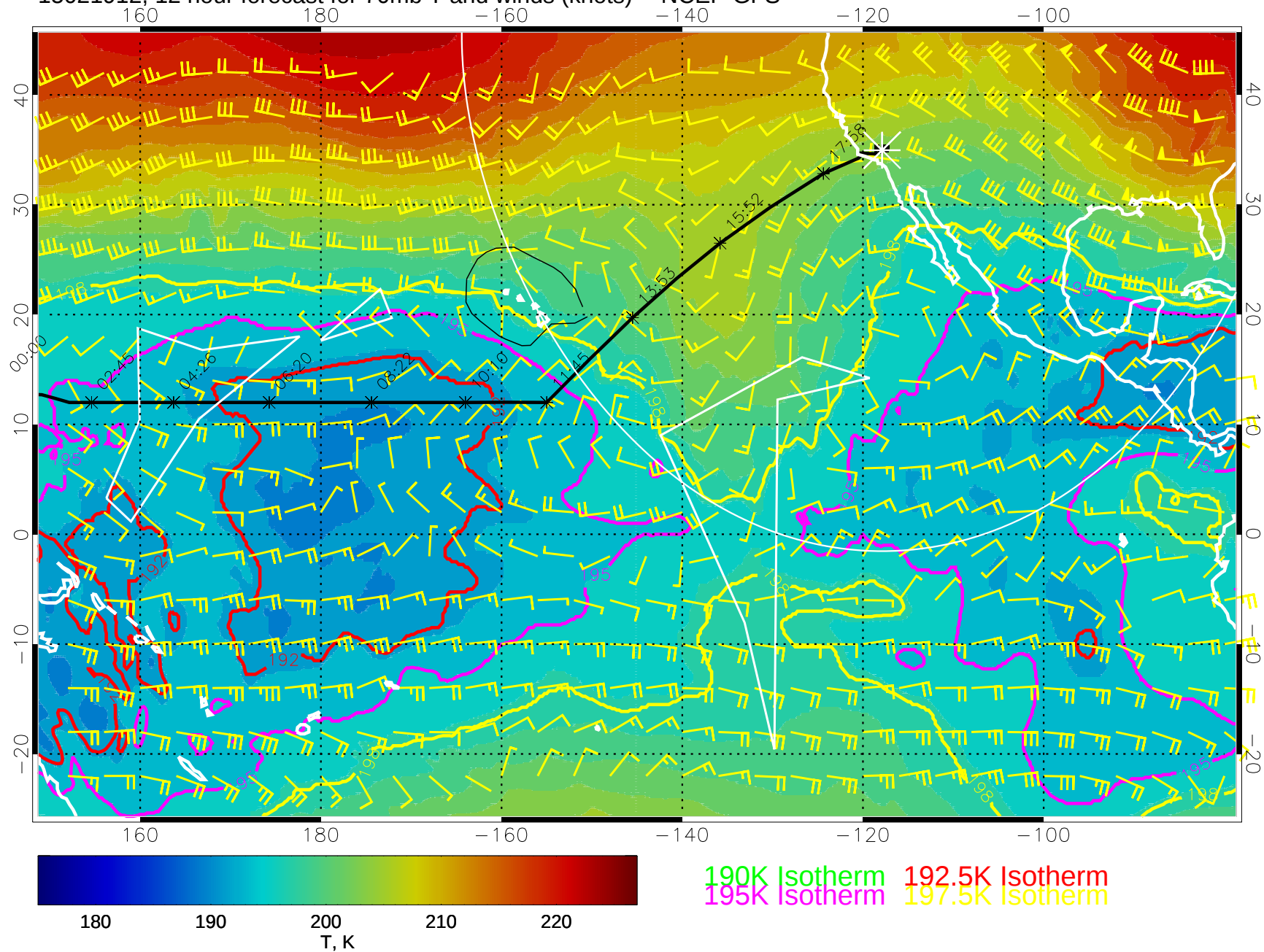
15021912, 12 hour forecast for 70mb T and winds (knots) -- NCEP GFS
