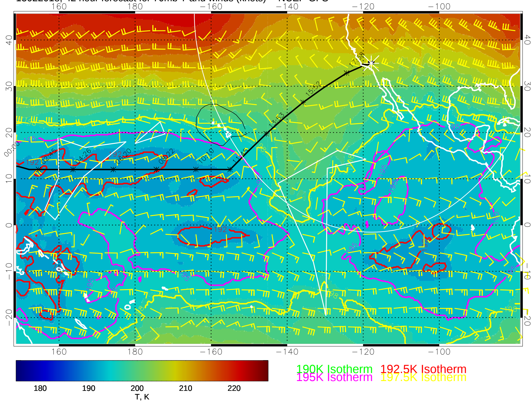
15022018, 42 hour forecast for 70mb T and winds (knots) -- NCEP GFS
