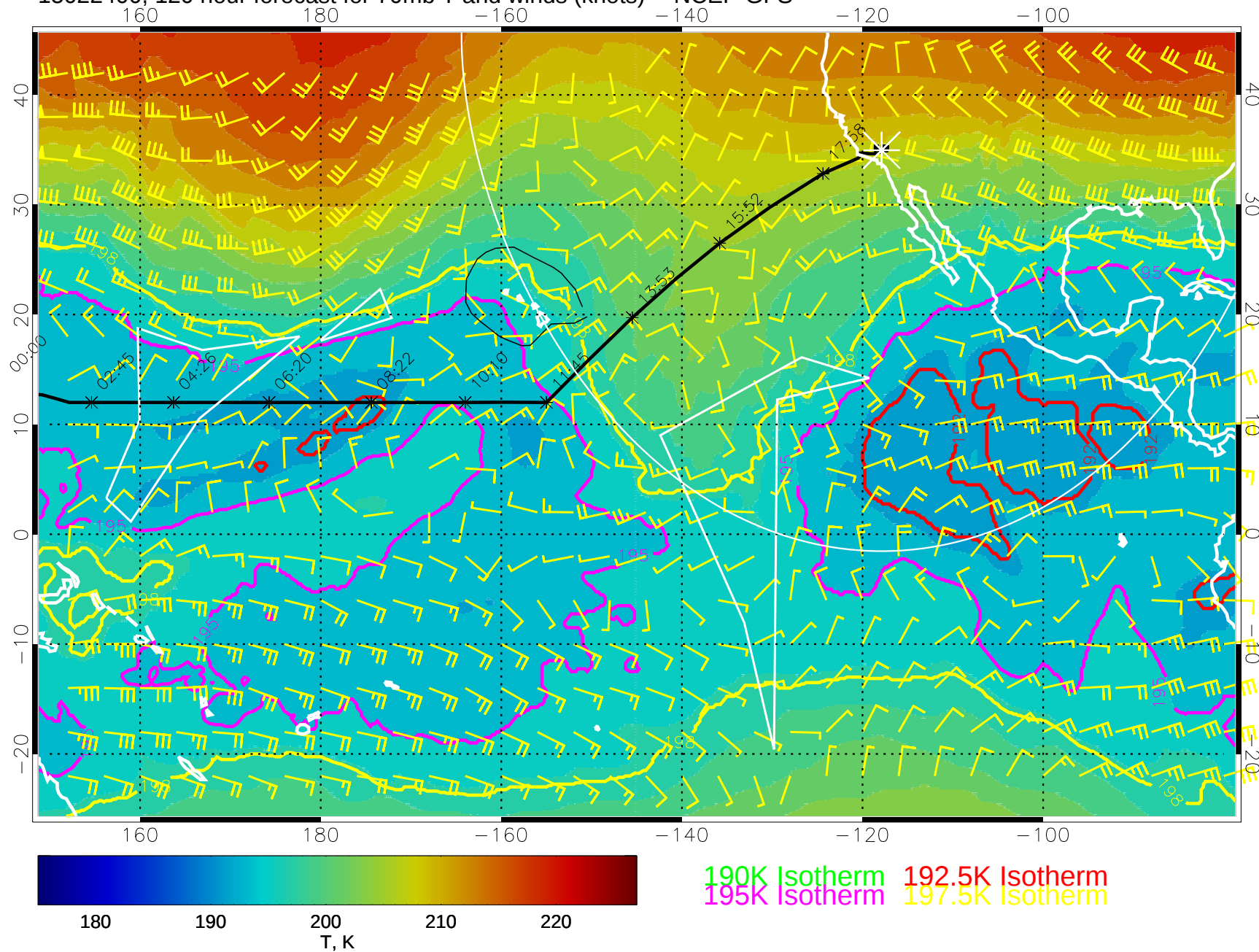
15022400, 120 hour forecast for 70mb T and winds (knots) -- NCEP GFS
