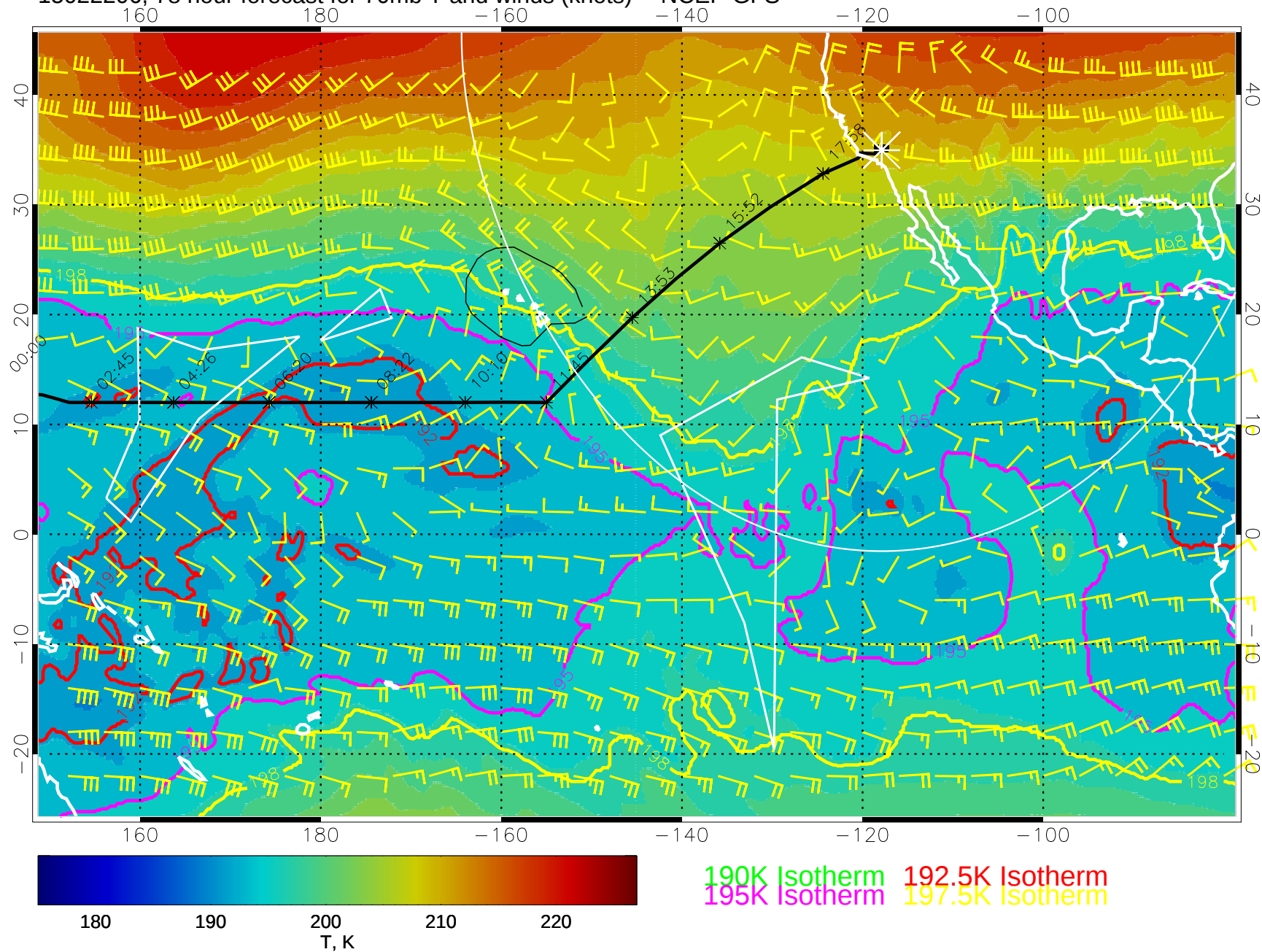
15022206, 78 hour forecast for 70mb T and winds (knots) -- NCEP GFS
