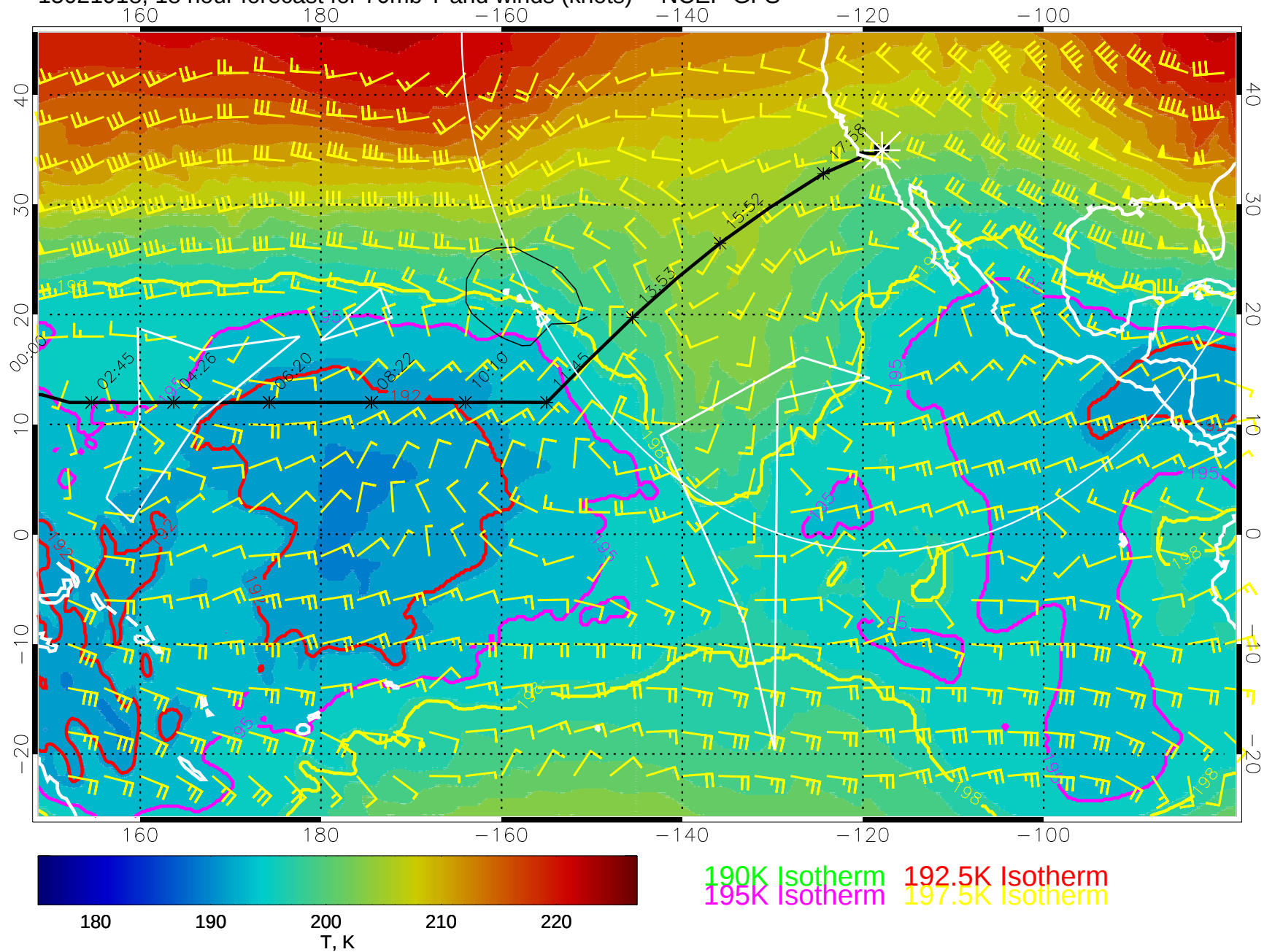
15021918, 18 hour forecast for 70mb T and winds (knots) -- NCEP GFS
