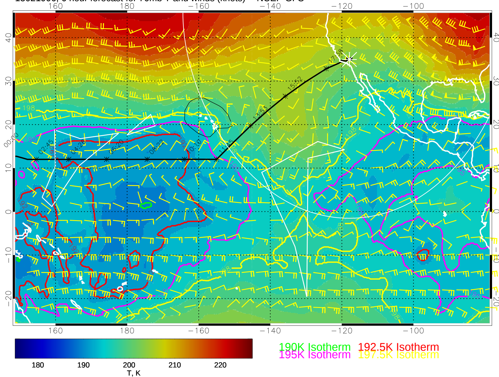
15021906, 6 hour forecast for 70mb T and winds (knots) -- NCEP GFS
