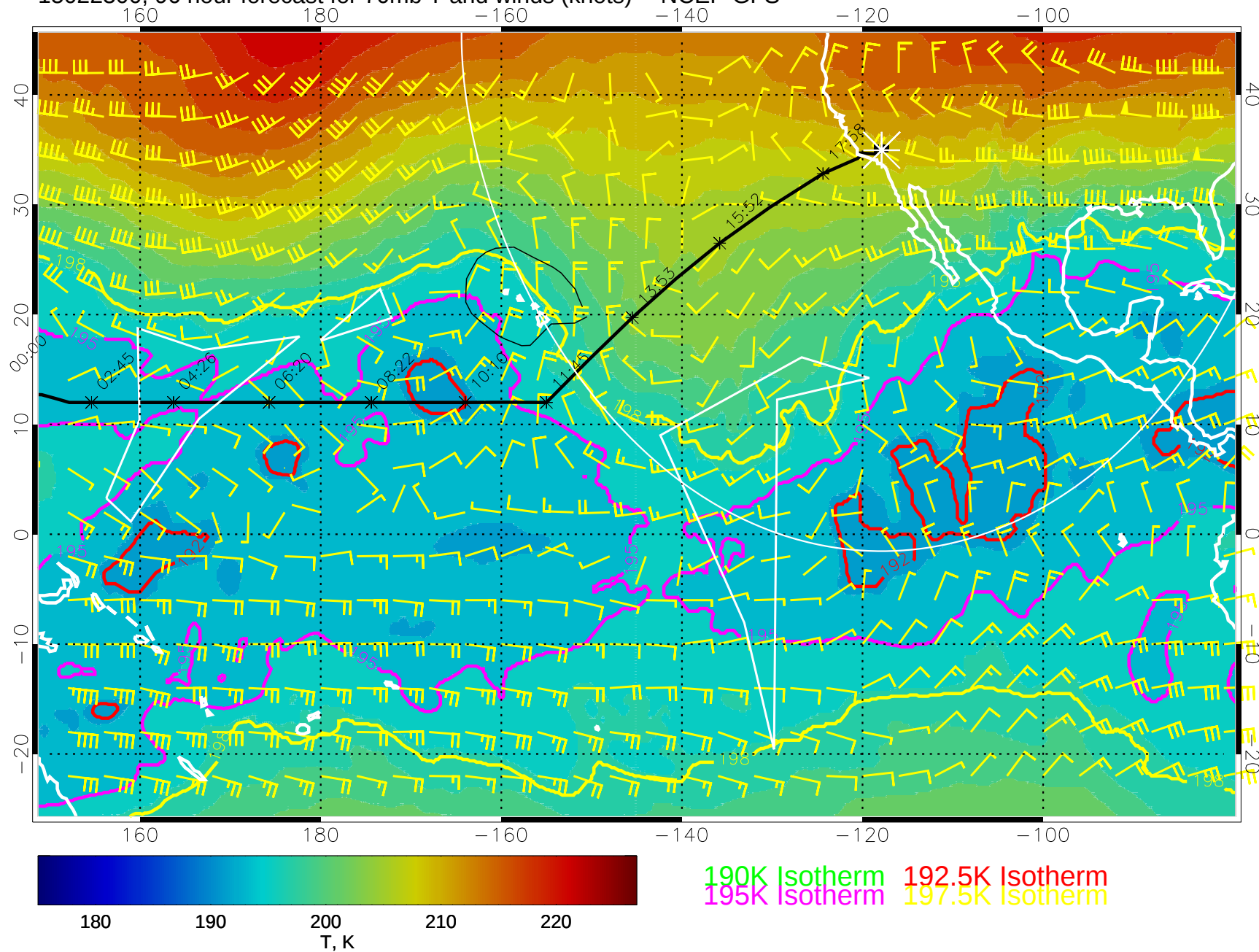
15022300, 96 hour forecast for 70mb T and winds (knots) -- NCEP GFS
