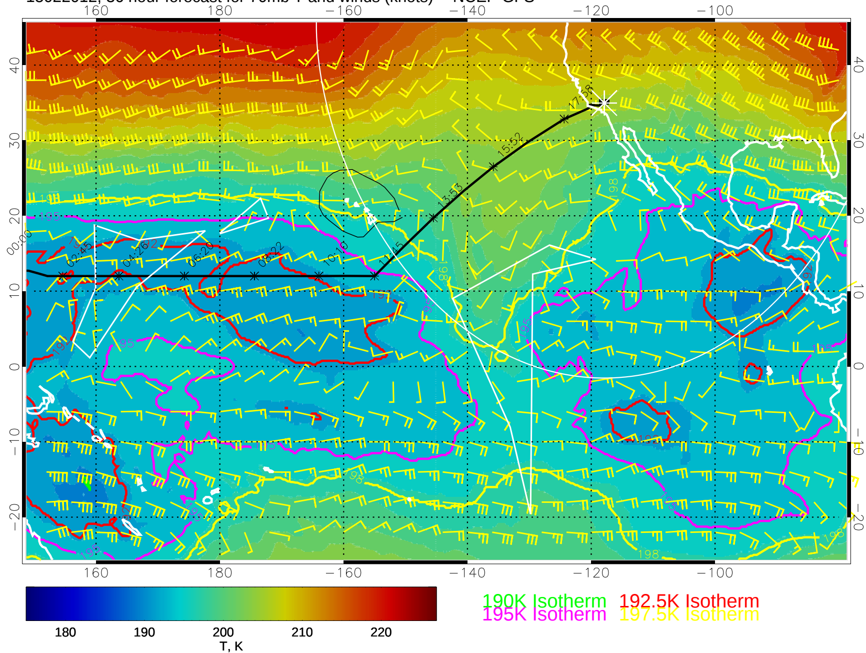
15022012, 36 hour forecast for 70mb T and winds (knots) -- NCEP GFS
