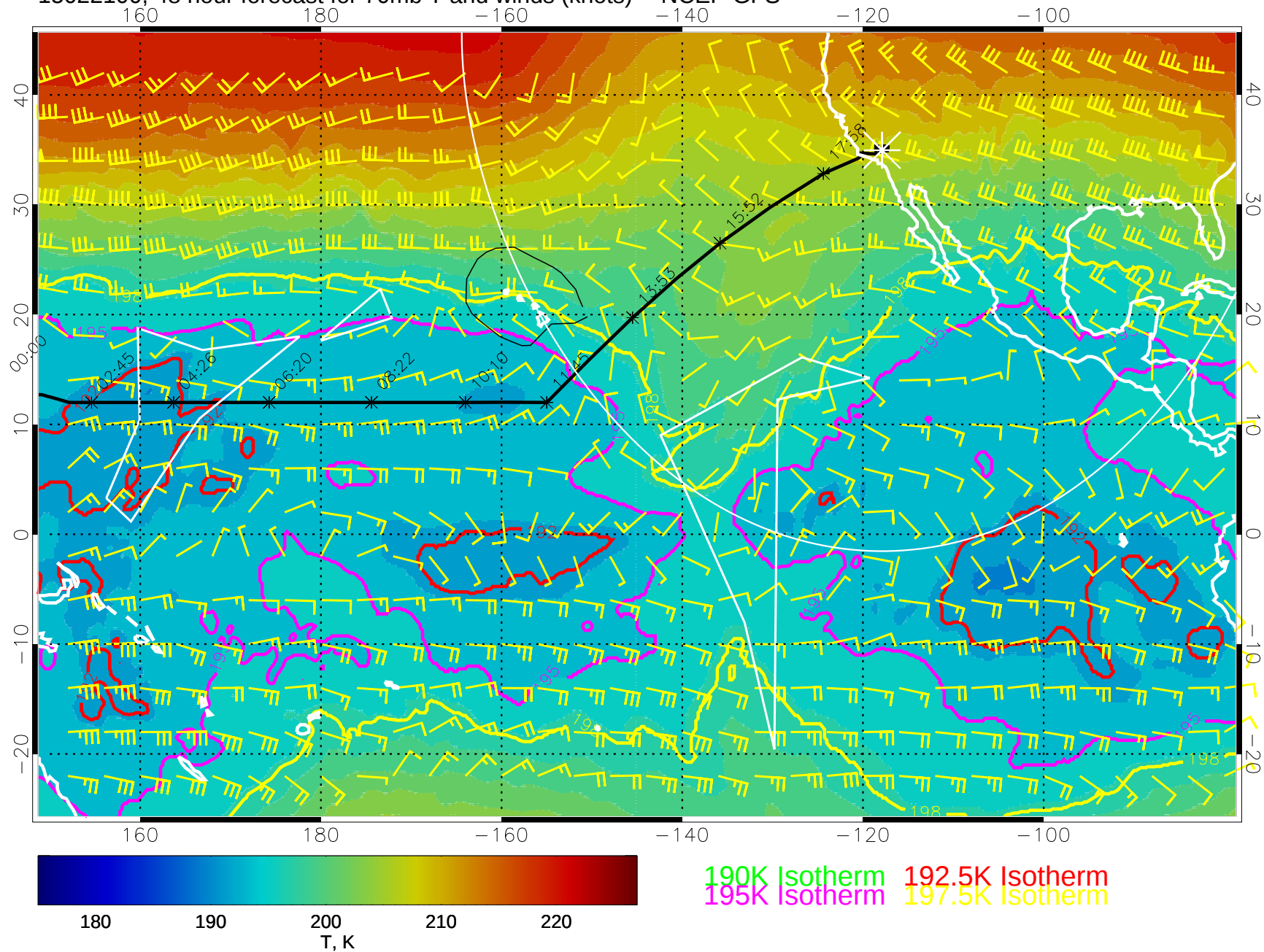
15022100, 48 hour forecast for 70mb T and winds (knots) -- NCEP GFS
