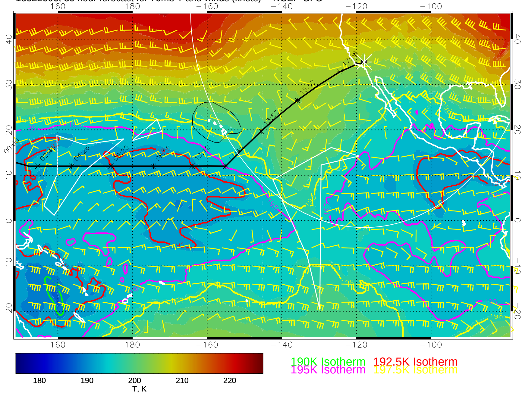
15022006, 30 hour forecast for 70mb T and winds (knots) -- NCEP GFS
