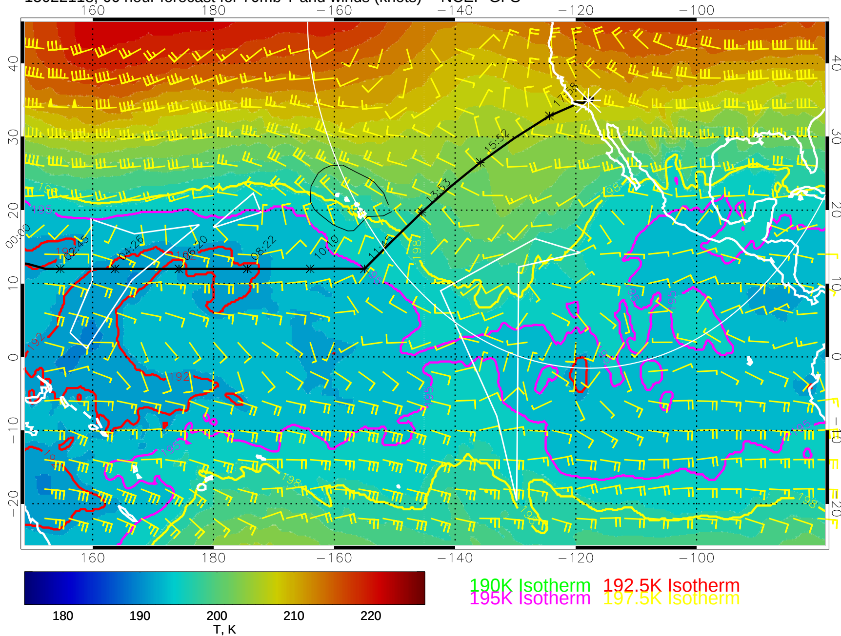
15022118, 66 hour forecast for 70mb T and winds (knots) -- NCEP GFS
