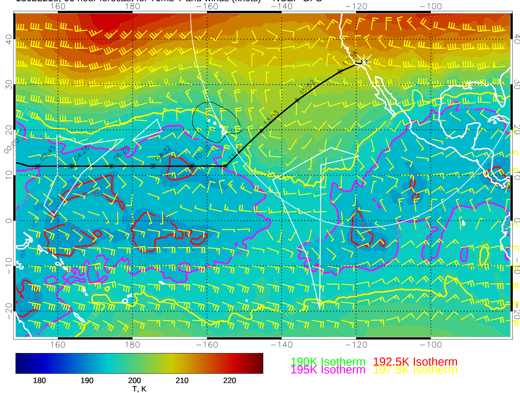
15022218, 90 hour forecast for 70mb T and winds (knots) -- NCEP GFS
