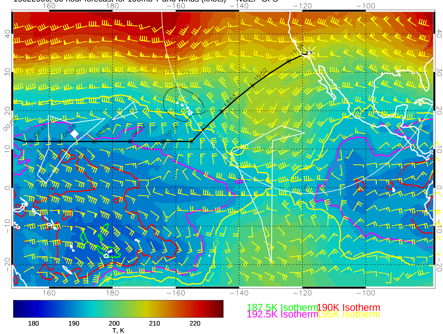
15022006, 30 hour forecast for 100mb T and winds (knots) -- NCEP GFS
