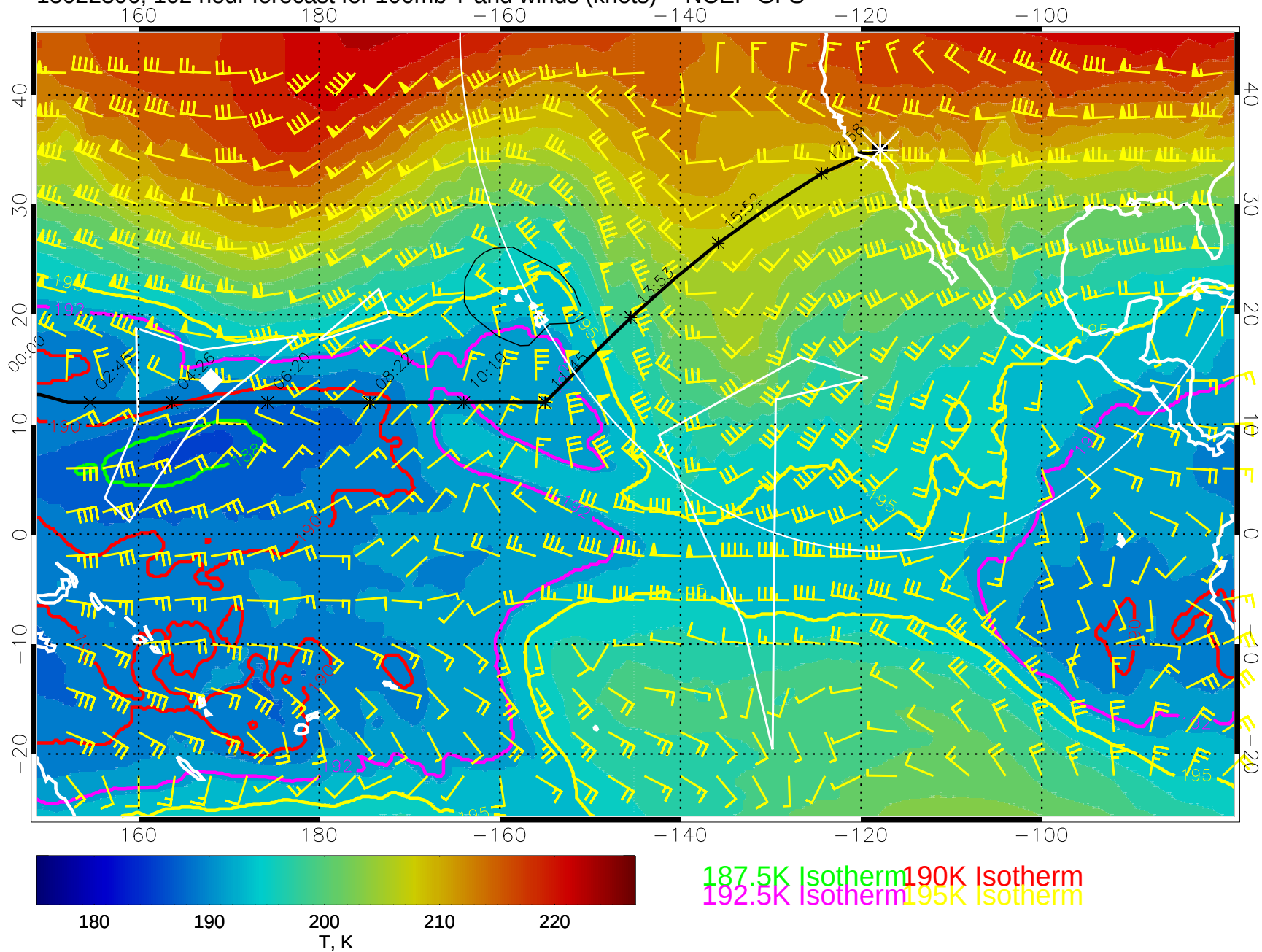
15022306, 102 hour forecast for 100mb T and winds (knots) -- NCEP GFS
