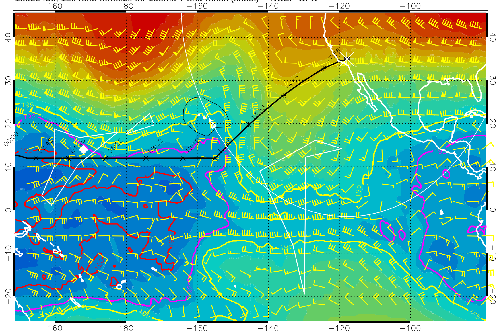
15022400, 120 hour forecast for 100mb T and winds (knots) -- NCEP GFS
