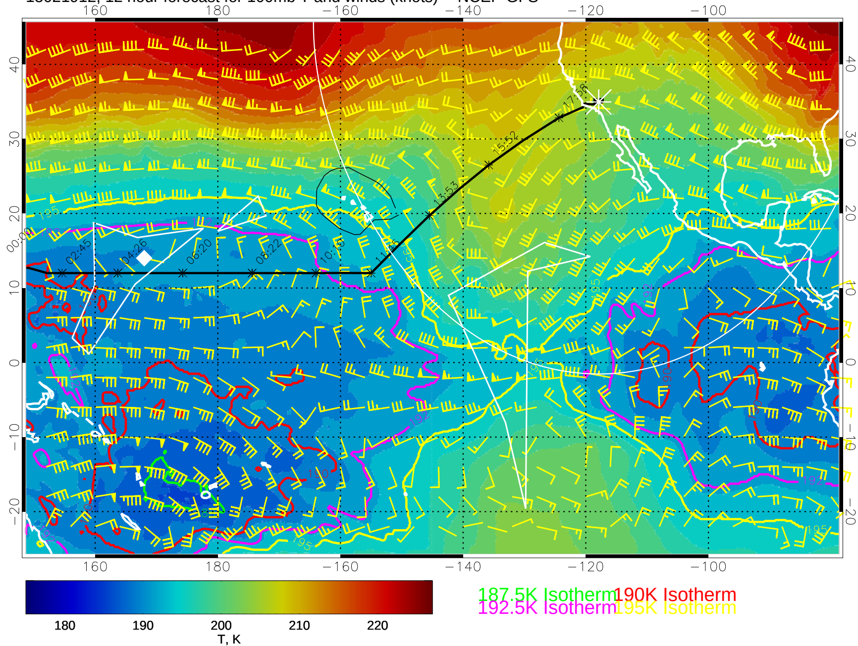
15021912, 12 hour forecast for 100mb T and winds (knots) -- NCEP GFS
