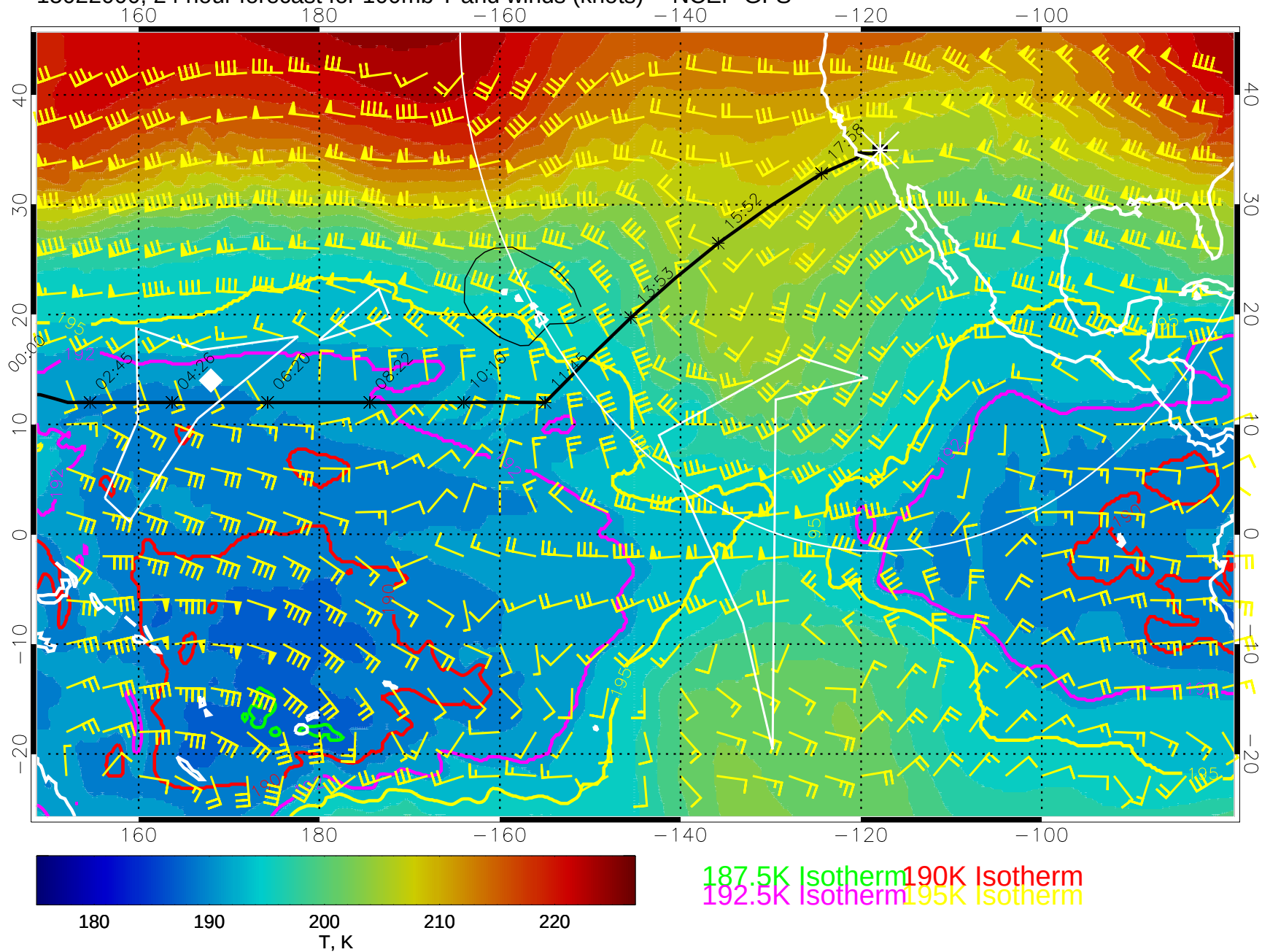
15022000, 24 hour forecast for 100mb T and winds (knots) -- NCEP GFS
