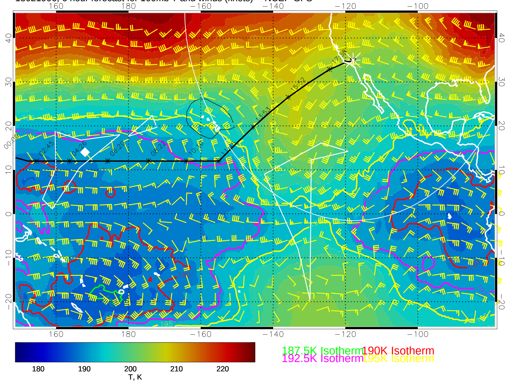
15021906, 6 hour forecast for 100mb T and winds (knots) -- NCEP GFS
