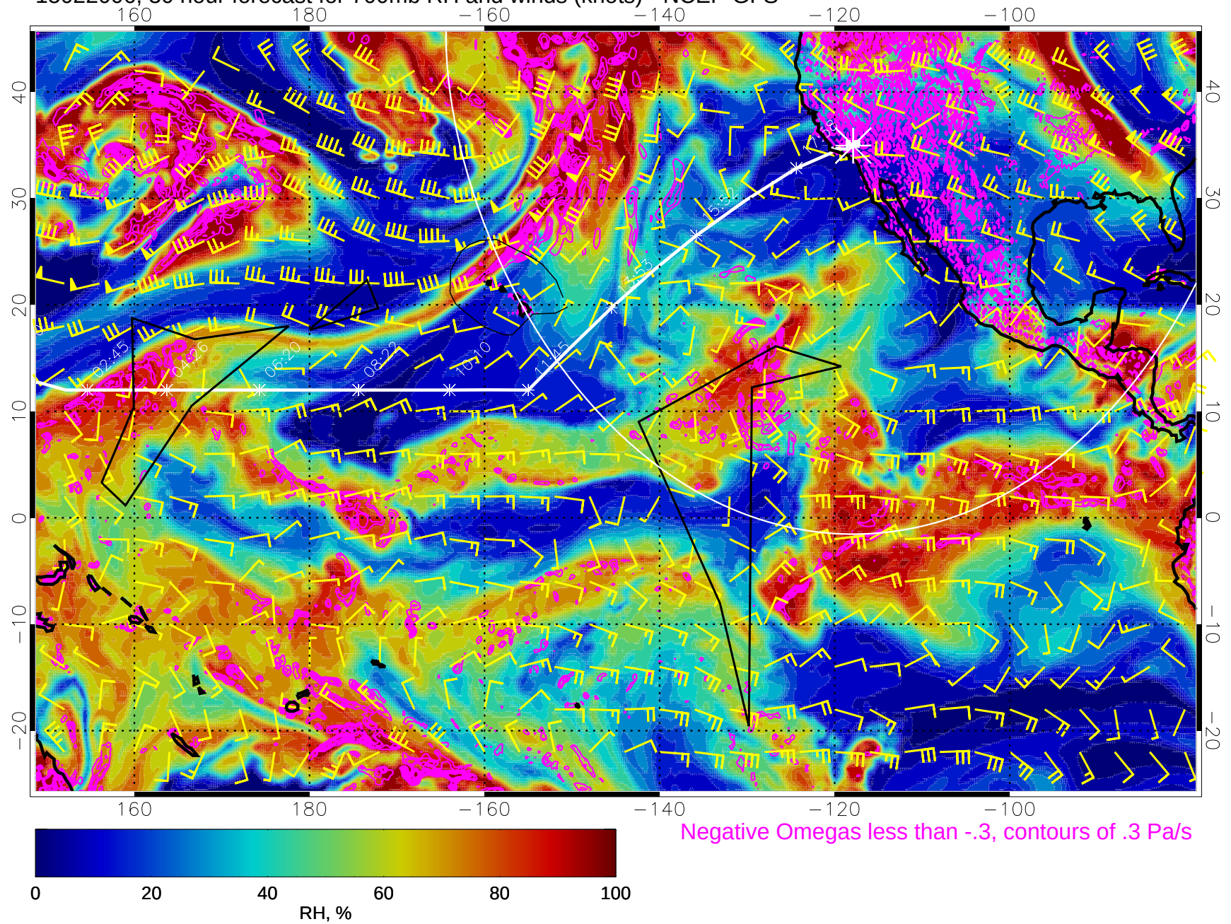
15022006, 30 hour forecast for 700mb RH and winds (knots) - NCEP GFS
