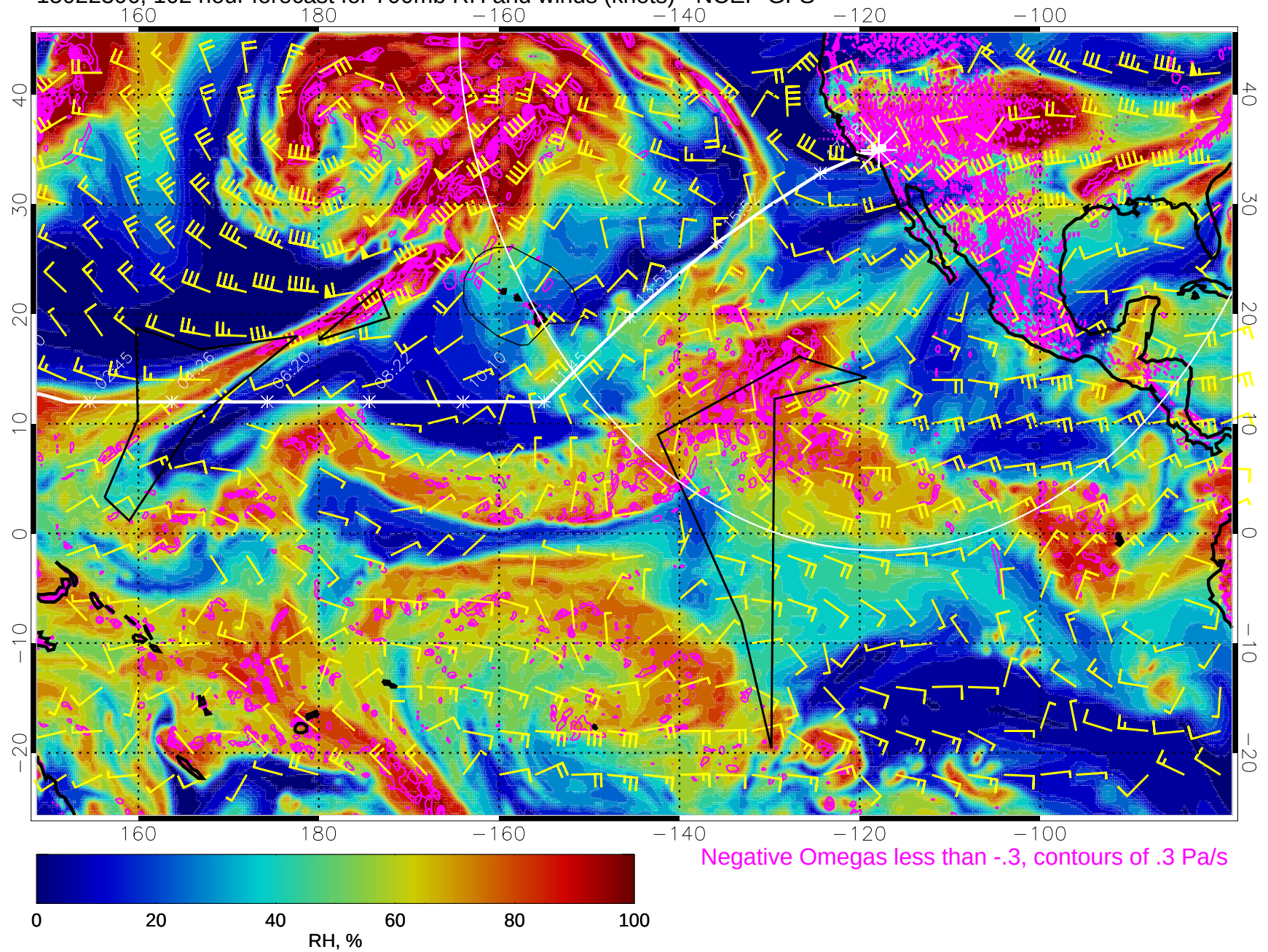
15022306, 102 hour forecast for 700mb RH and winds (knots) - NCEP GFS
