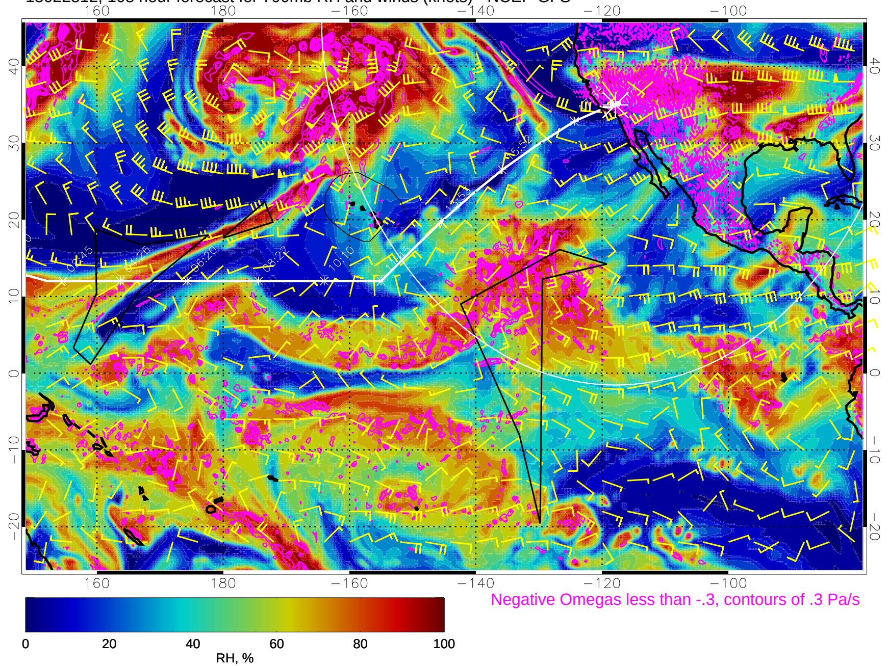
15022312, 108 hour forecast for 700mb RH and winds (knots) - NCEP GFS
