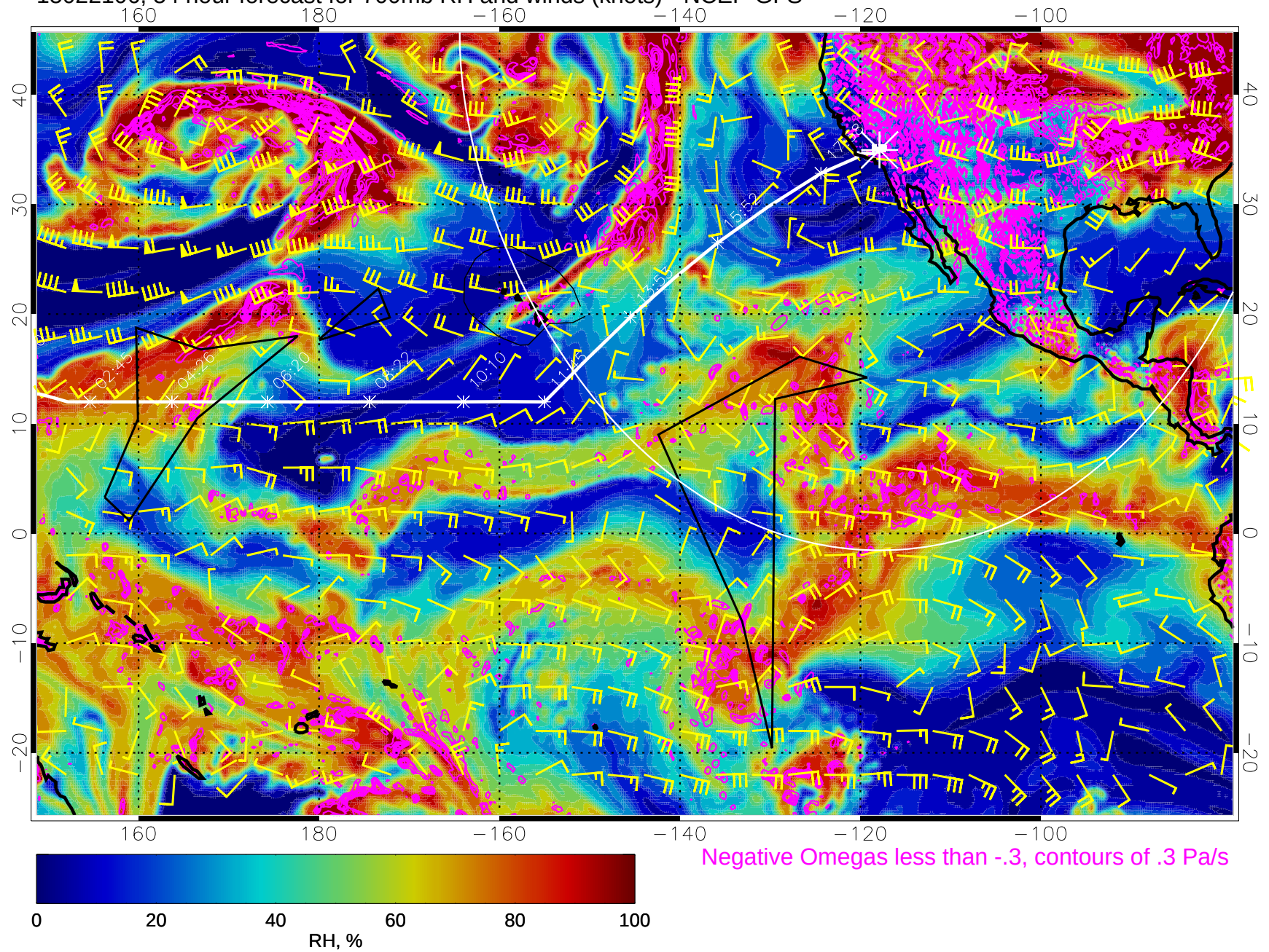
15022106, 54 hour forecast for 700mb RH and winds (knots) - NCEP GFS
