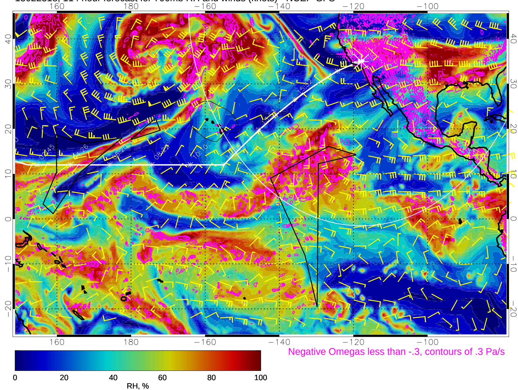
15022318, 114 hour forecast for 700mb RH and winds (knots) - NCEP GFS
