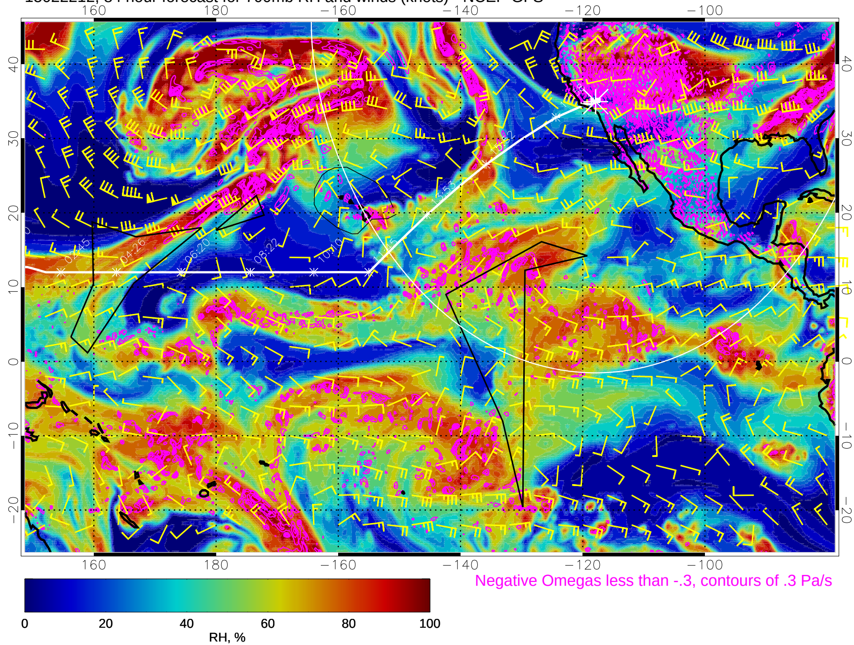
15022212, 84 hour forecast for 700mb RH and winds (knots) - NCEP GFS
