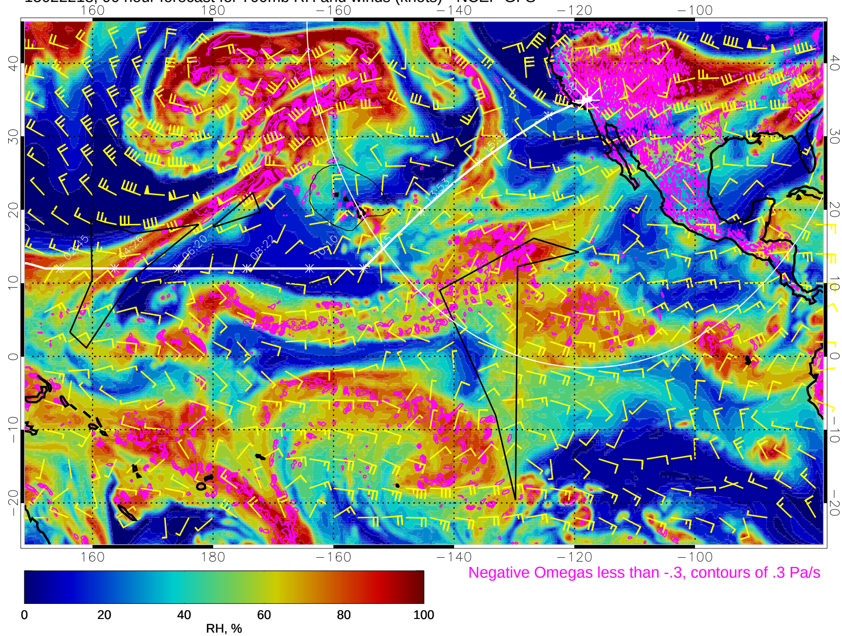
15022218, 90 hour forecast for 700mb RH and winds (knots) - NCEP GFS
