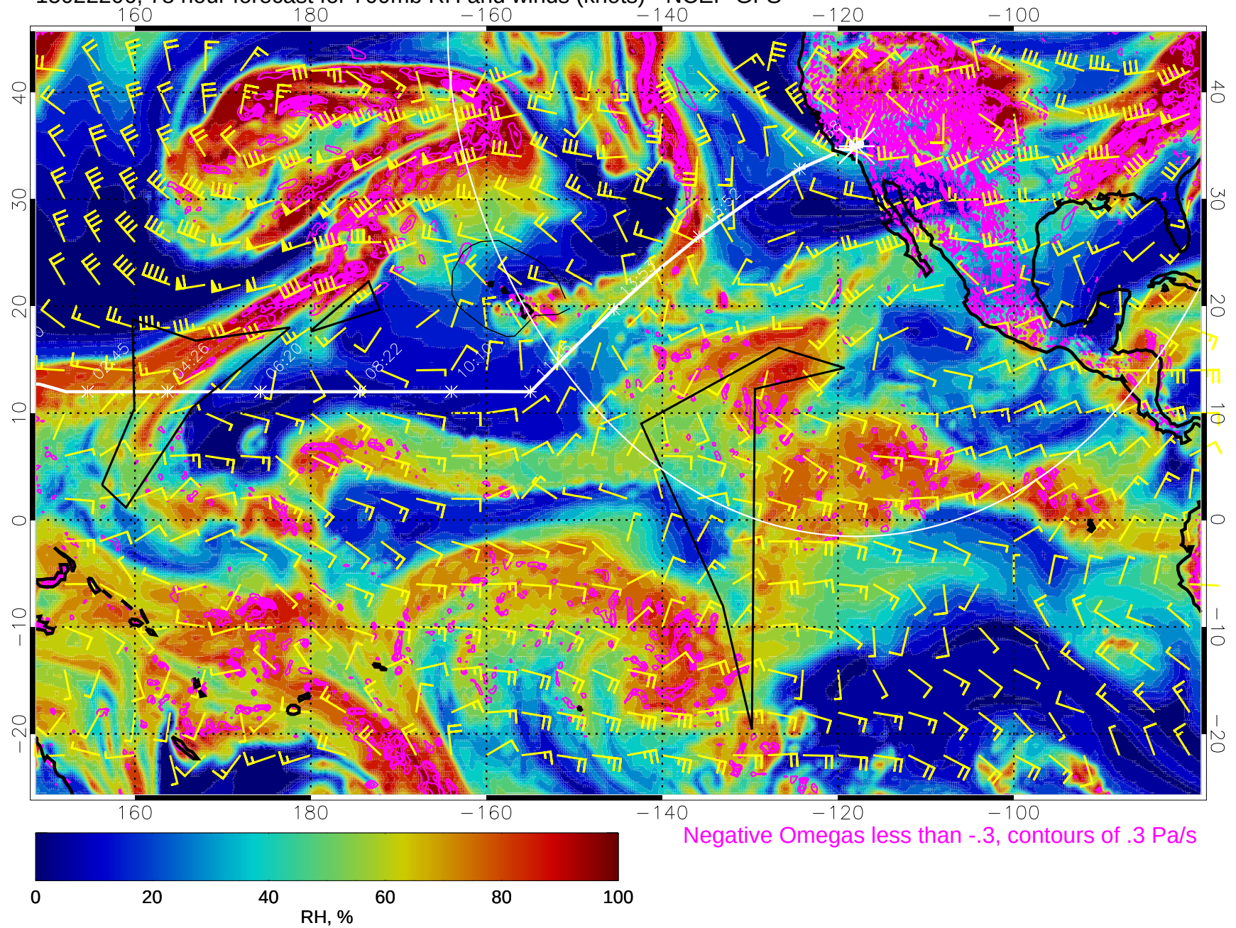
15022206, 78 hour forecast for 700mb RH and winds (knots) - NCEP GFS
