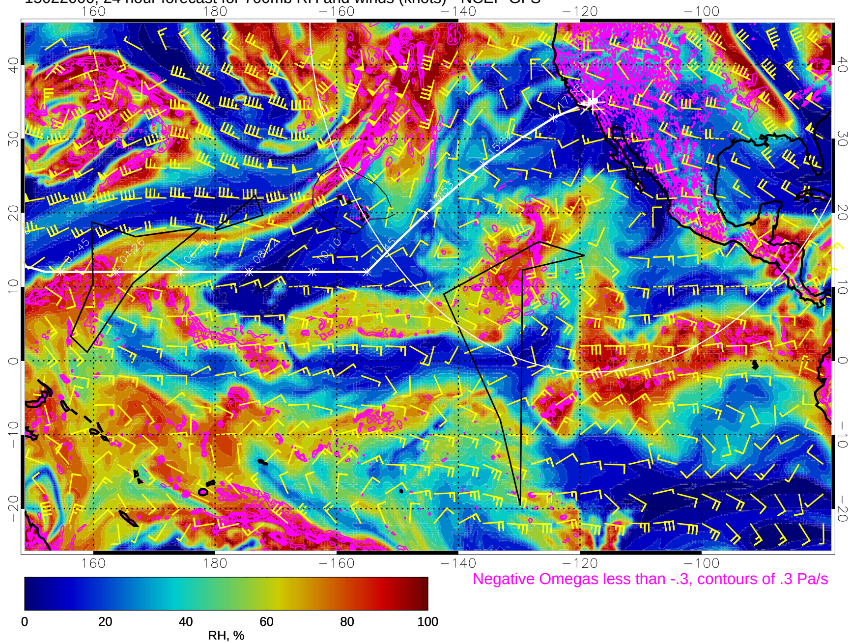
15022000, 24 hour forecast for 700mb RH and winds (knots) - NCEP GFS
