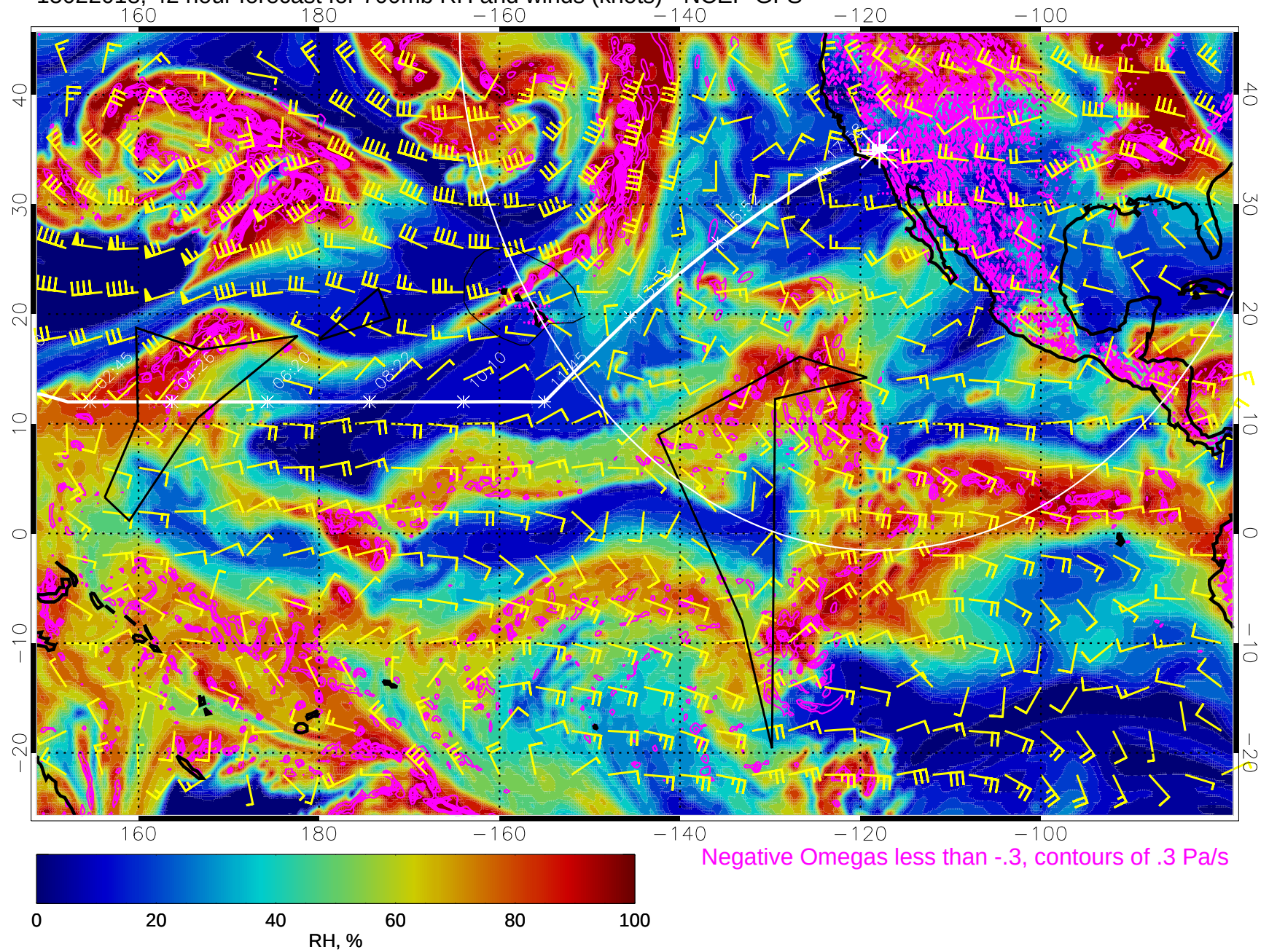
15022018, 42 hour forecast for 700mb RH and winds (knots) - NCEP GFS
