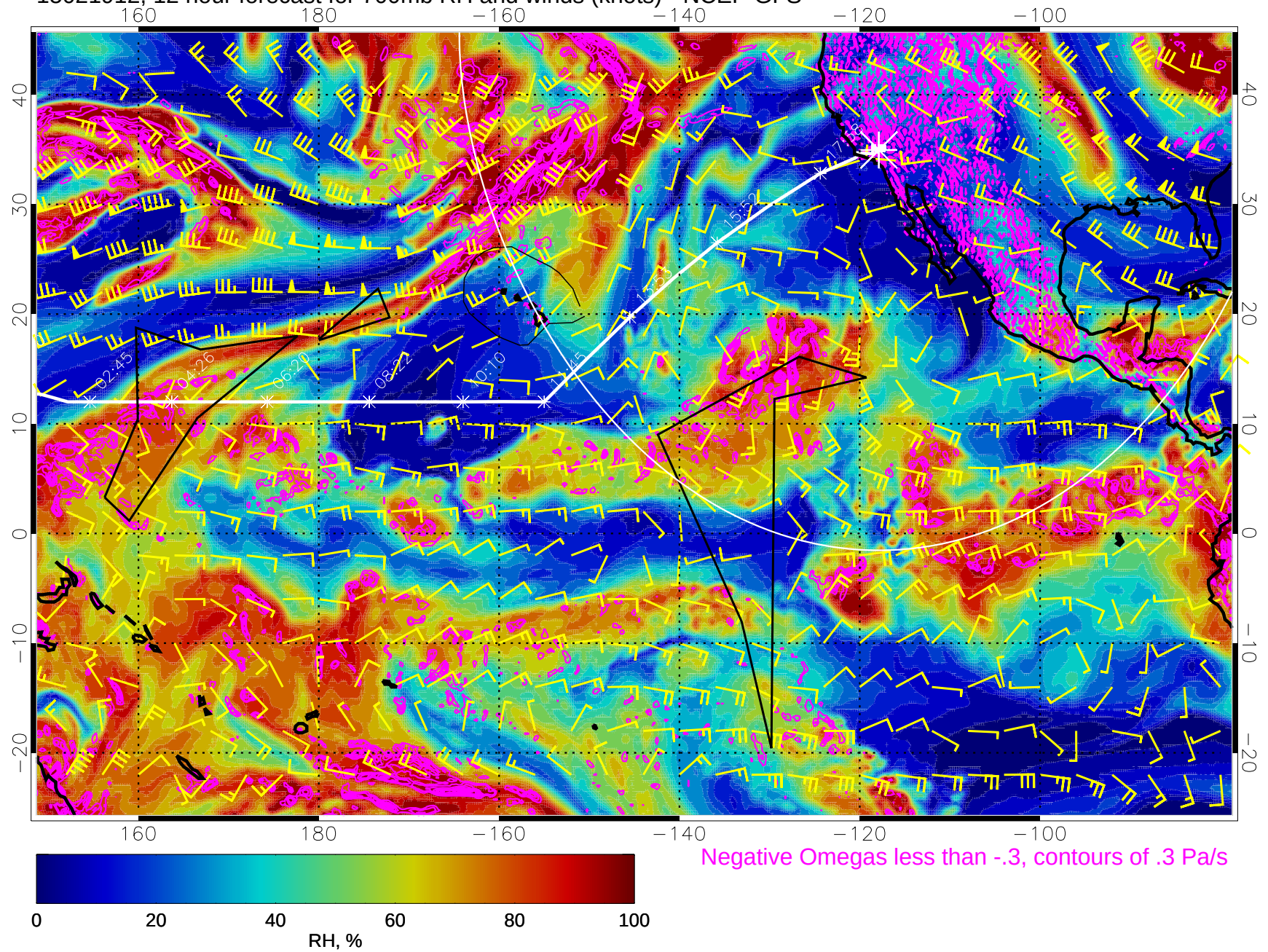
15021912, 12 hour forecast for 700mb RH and winds (knots) - NCEP GFS
