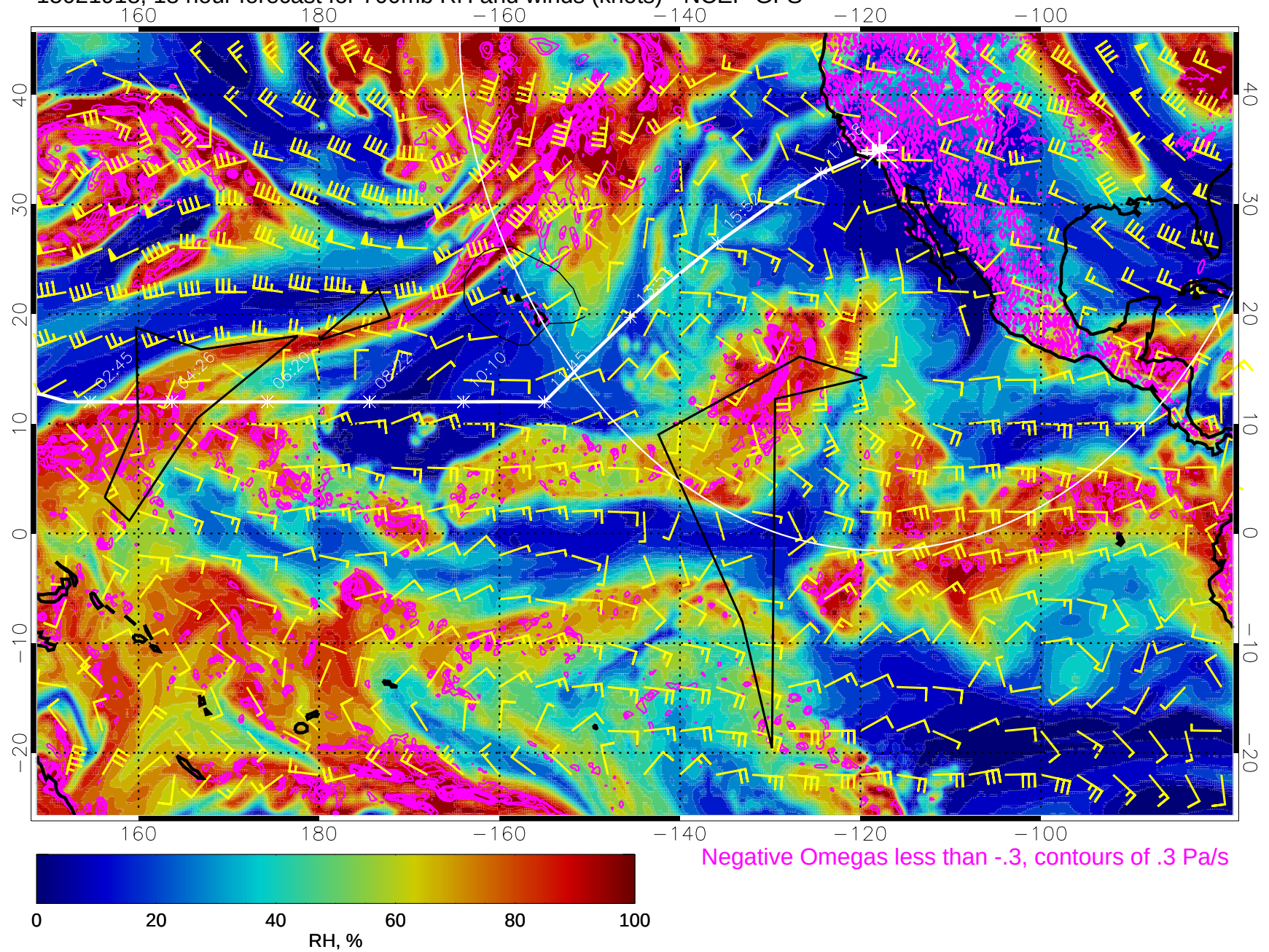
15021918, 18 hour forecast for 700mb RH and winds (knots) - NCEP GFS
