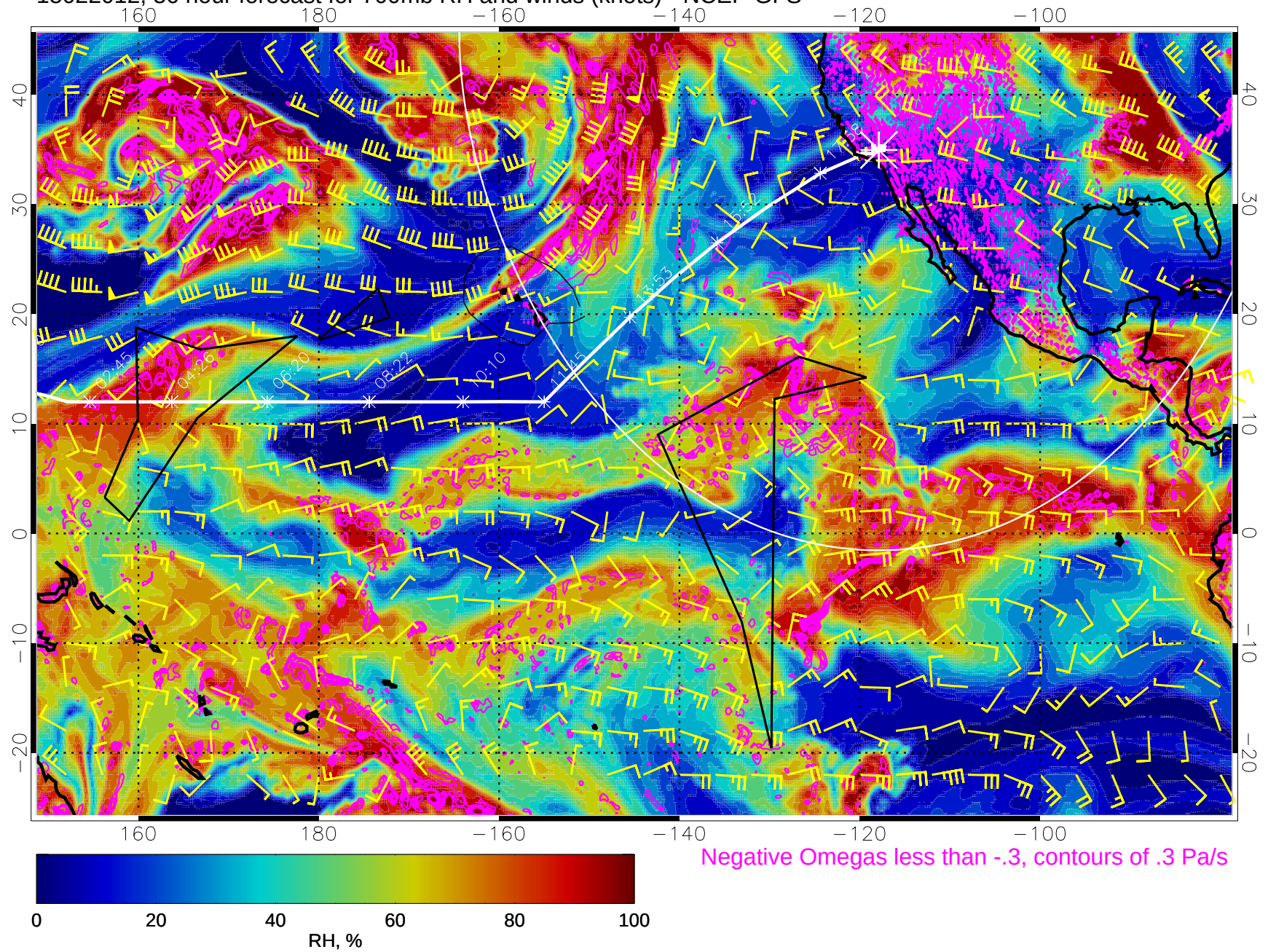
15022012, 36 hour forecast for 700mb RH and winds (knots) - NCEP GFS
