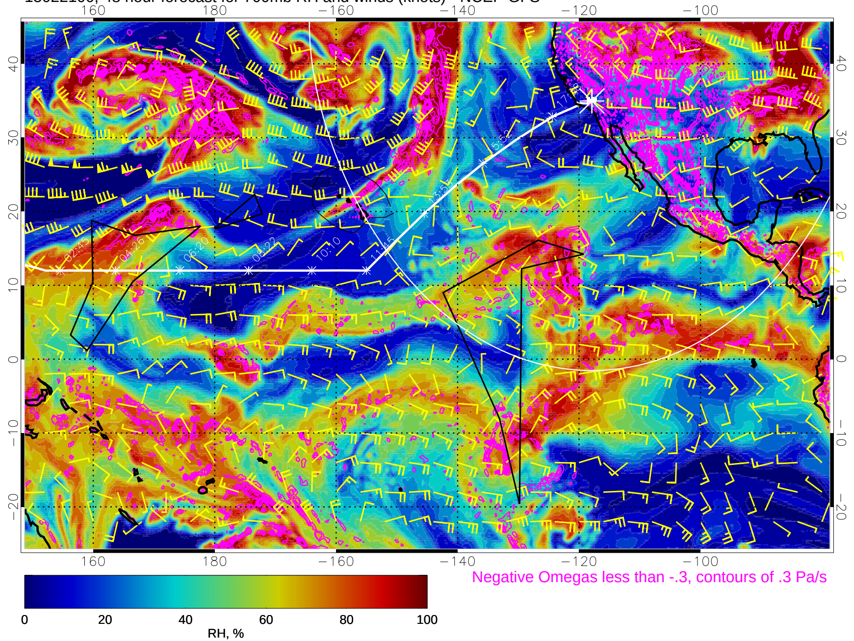
15022100, 48 hour forecast for 700mb RH and winds (knots) - NCEP GFS
