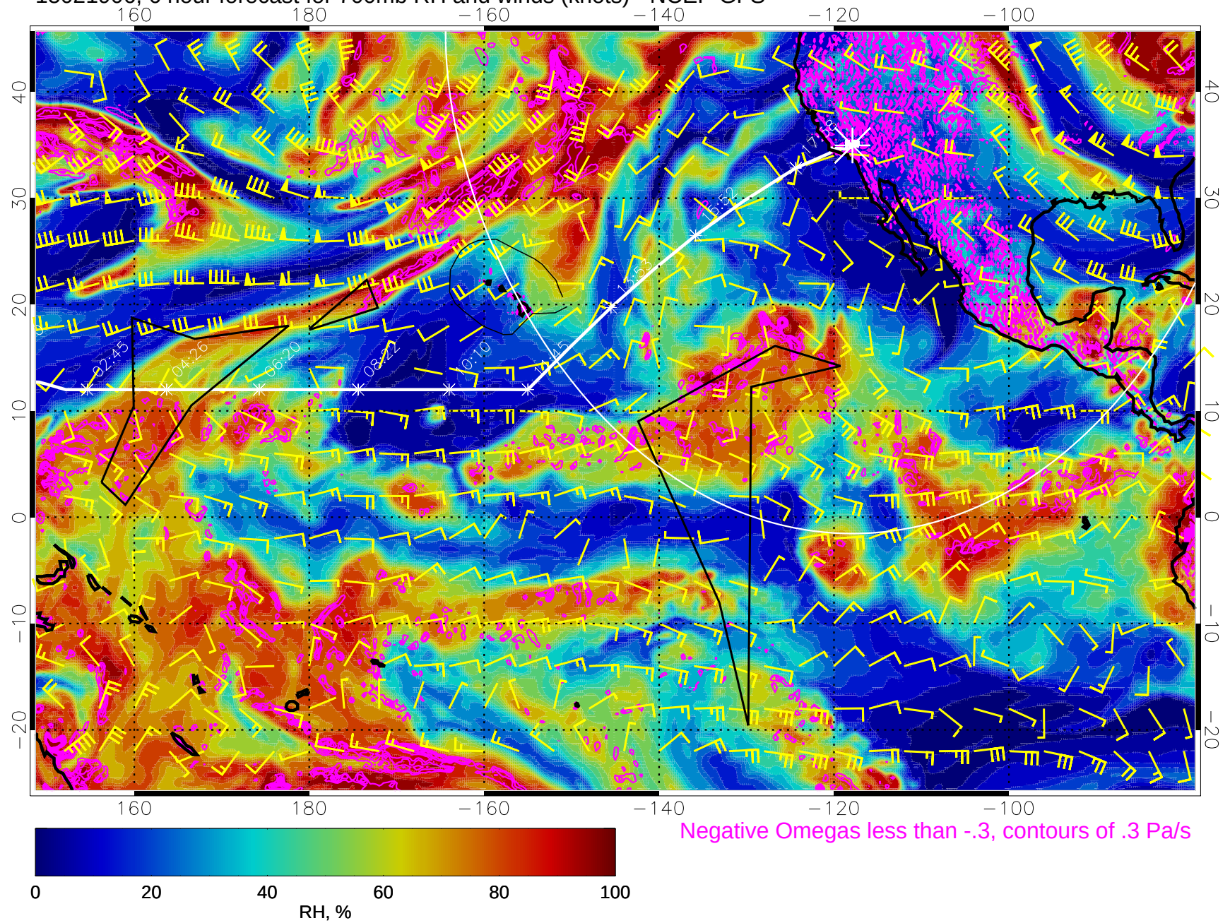
15021906, 6 hour forecast for 700mb RH and winds (knots) - NCEP GFS
