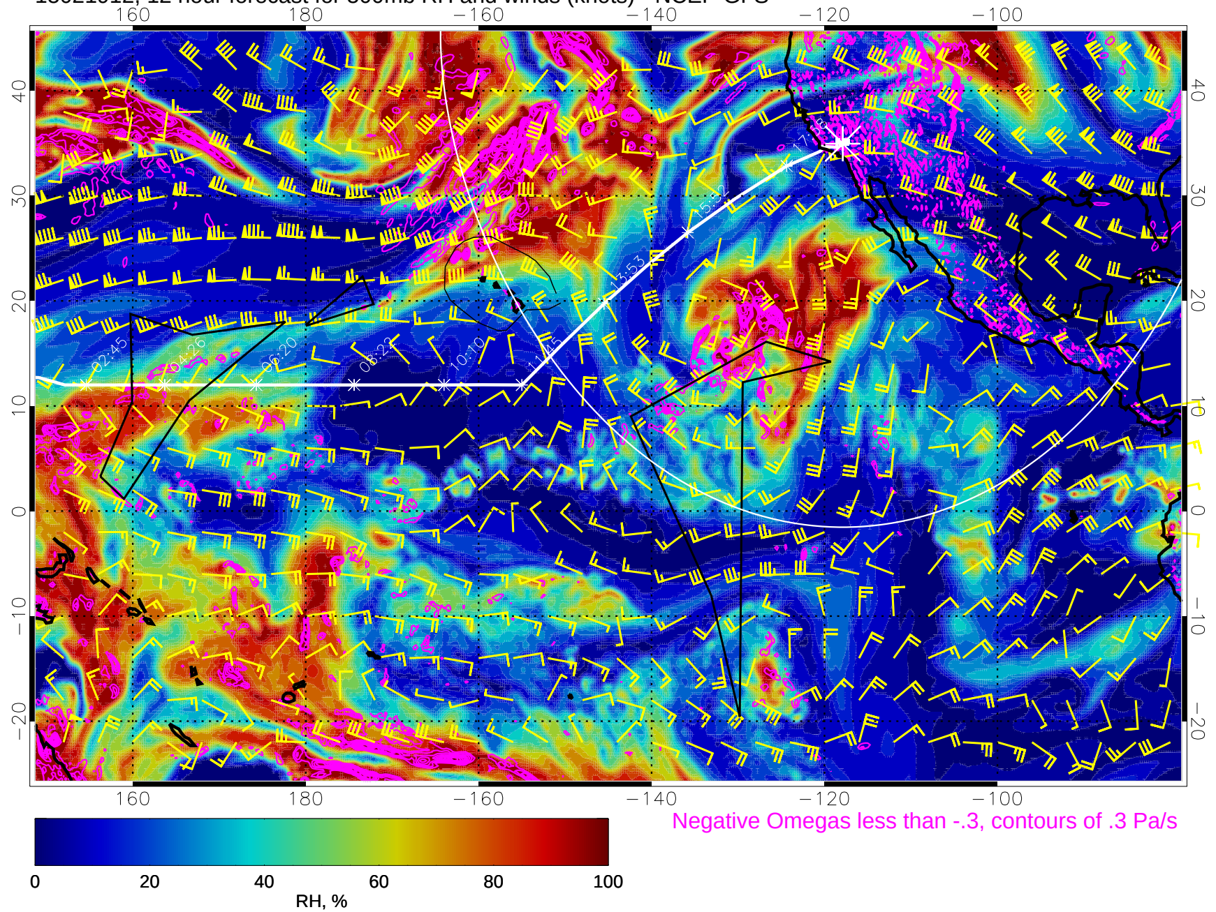
15021912, 12 hour forecast for 500mb RH and winds (knots) - NCEP GFS
