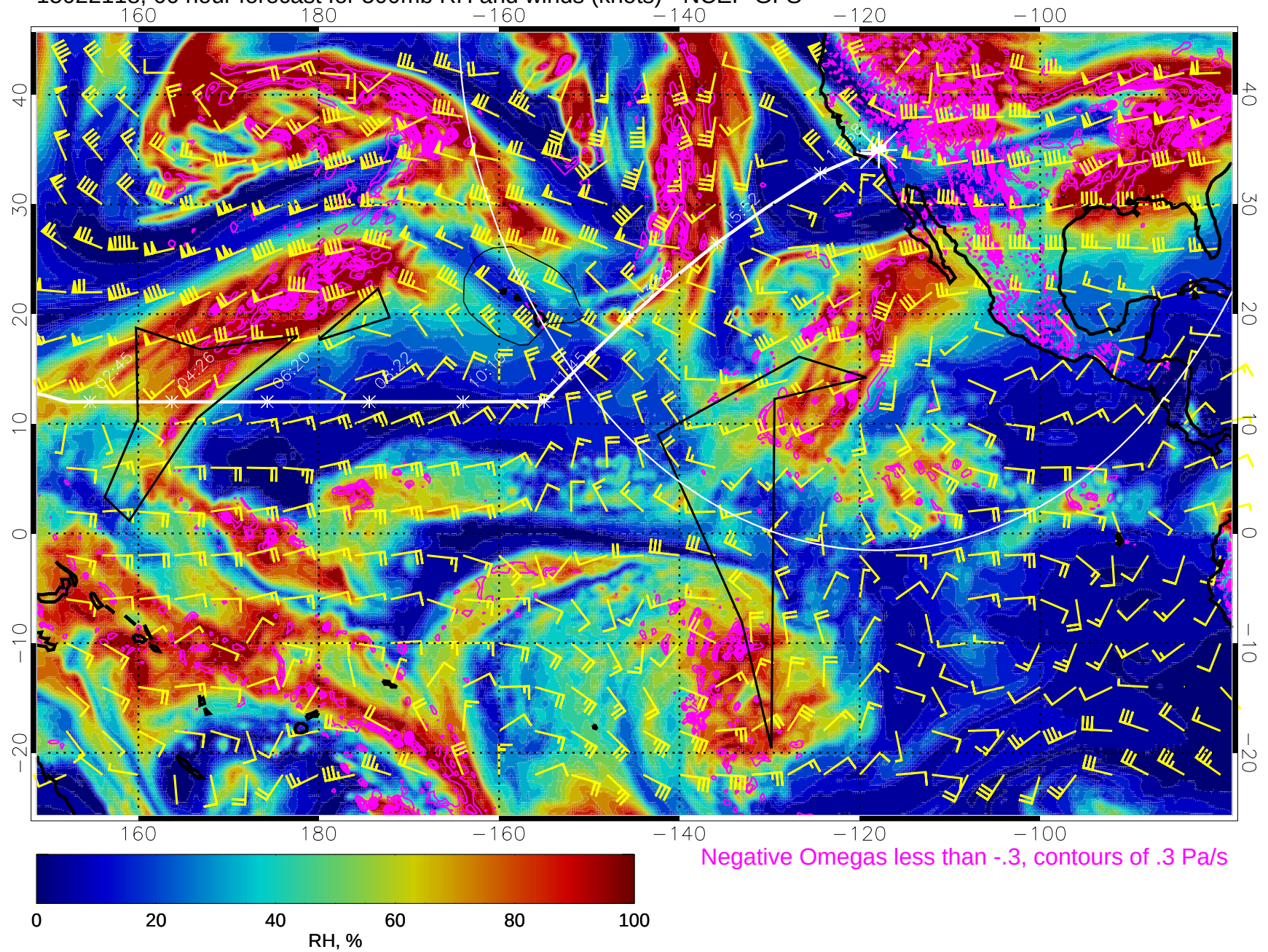
15022118, 66 hour forecast for 500mb RH and winds (knots) - NCEP GFS
