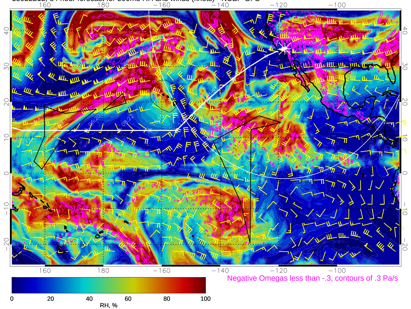
15022212, 84 hour forecast for 500mb RH and winds (knots) - NCEP GFS
