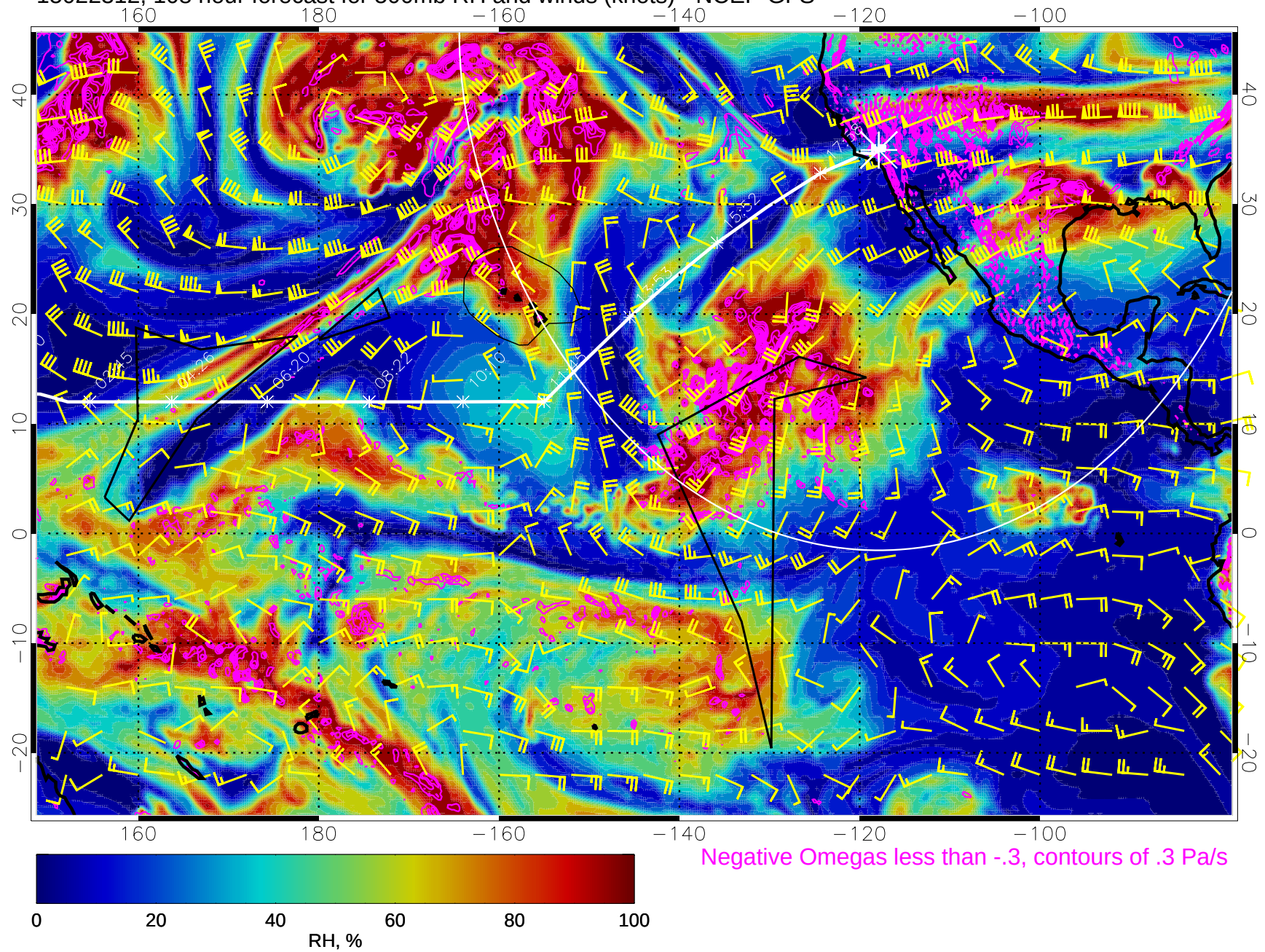
15022312, 108 hour forecast for 500mb RH and winds (knots) - NCEP GFS
