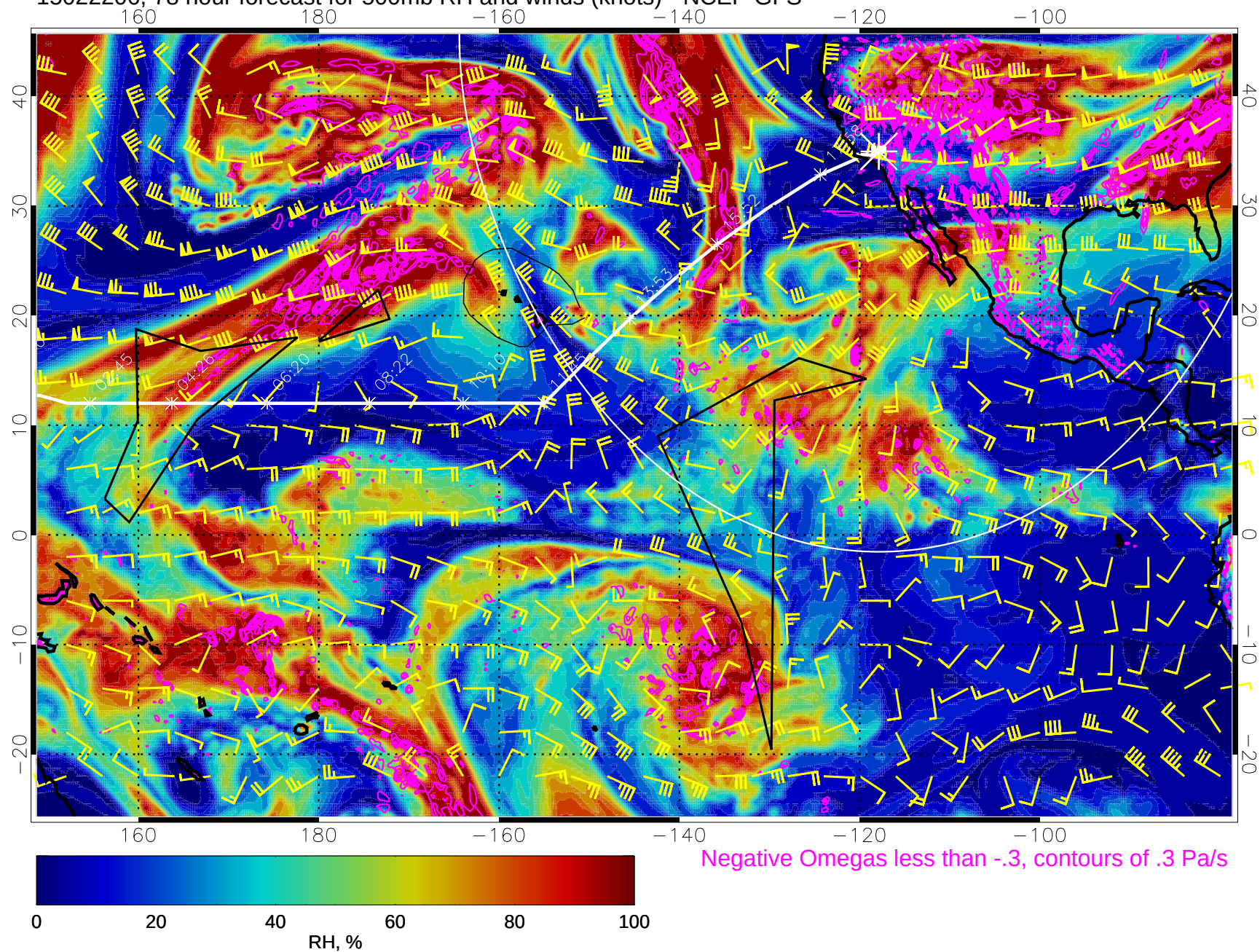
15022206, 78 hour forecast for 500mb RH and winds (knots) - NCEP GFS
