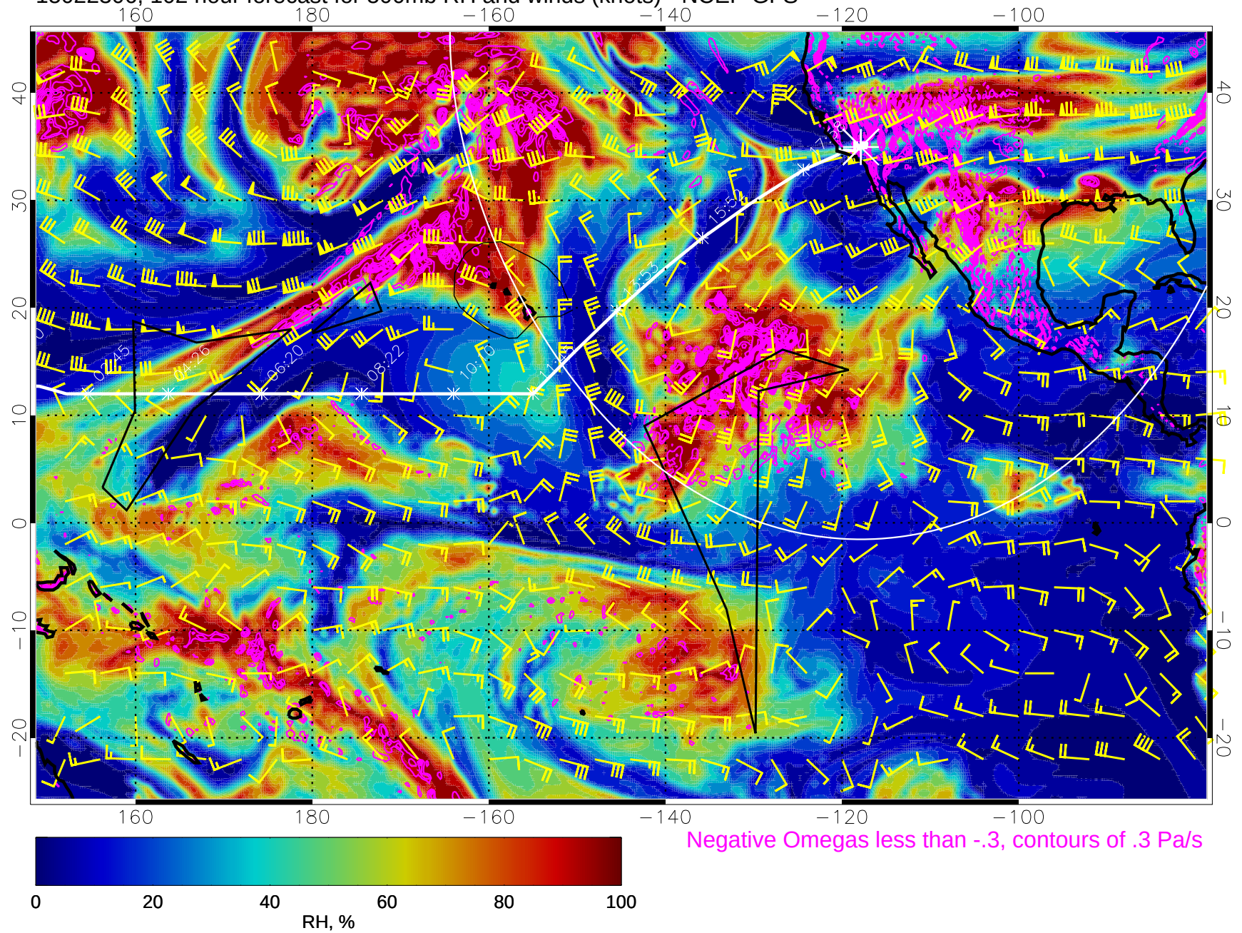
15022306, 102 hour forecast for 500mb RH and winds (knots) - NCEP GFS
