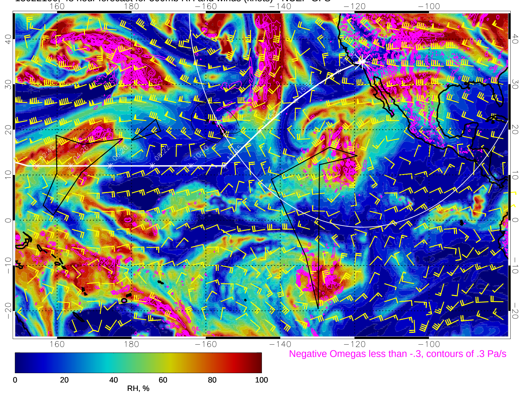
15022100, 48 hour forecast for 500mb RH and winds (knots) - NCEP GFS
