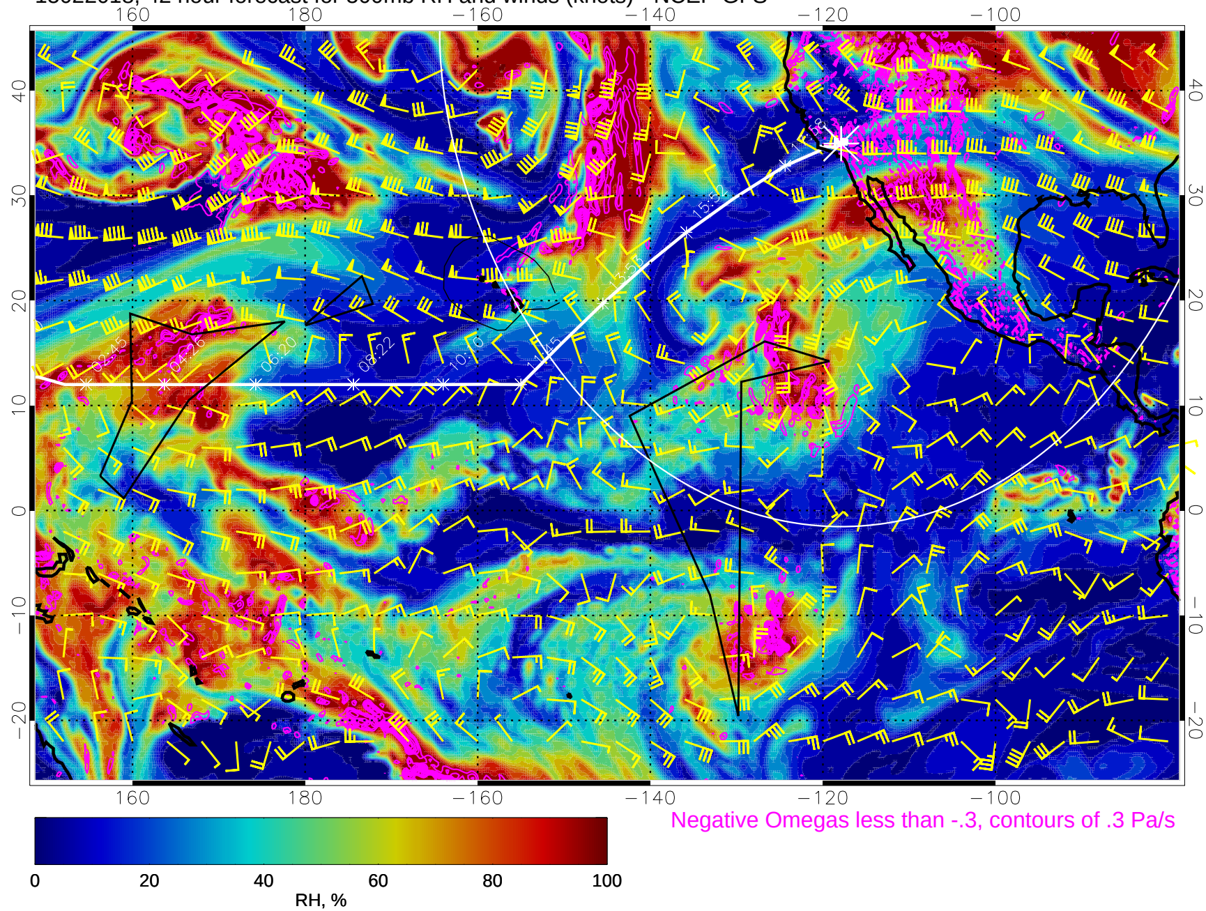
15022018, 42 hour forecast for 500mb RH and winds (knots) - NCEP GFS
