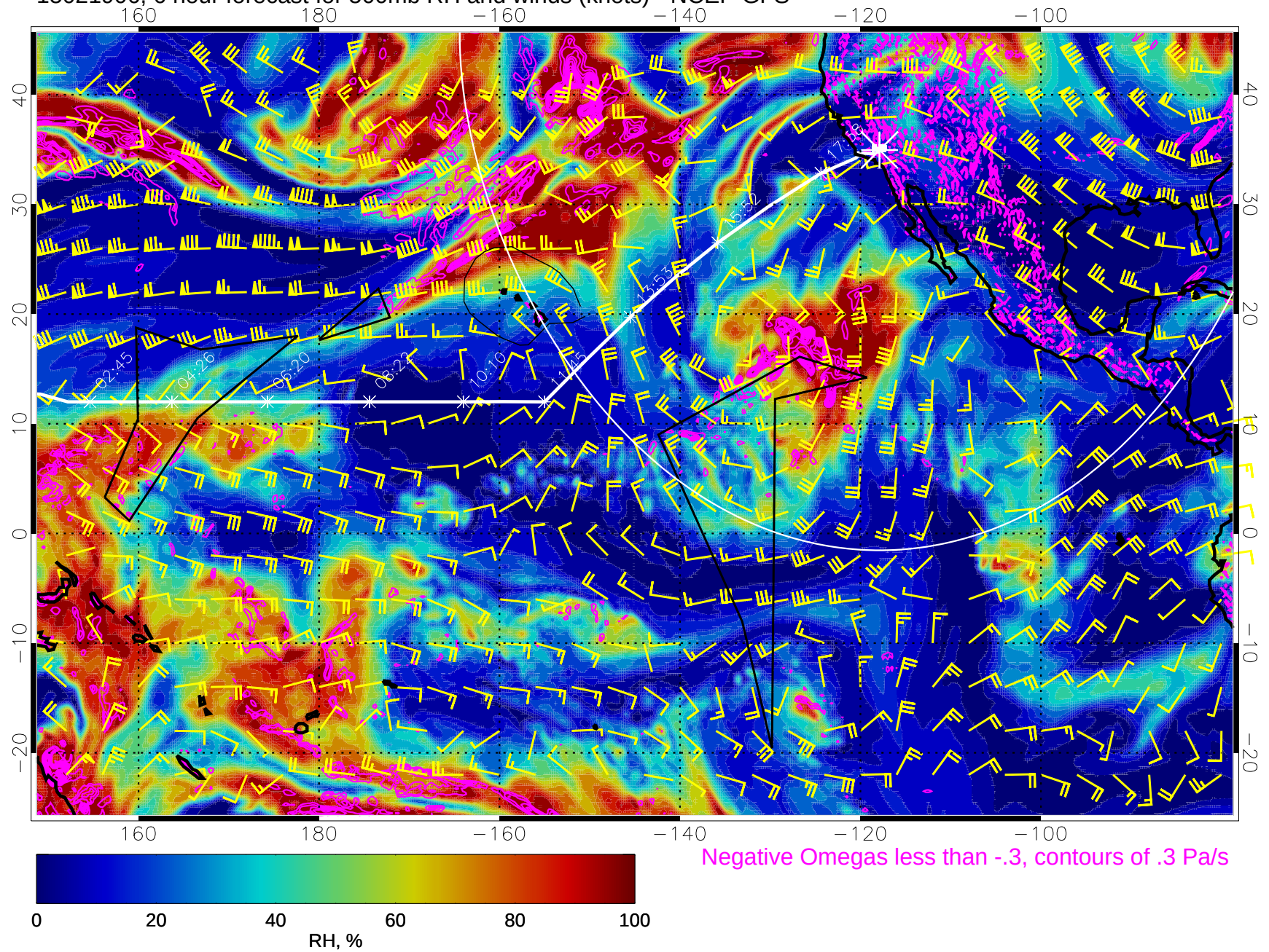
15021906, 6 hour forecast for 500mb RH and winds (knots) - NCEP GFS
