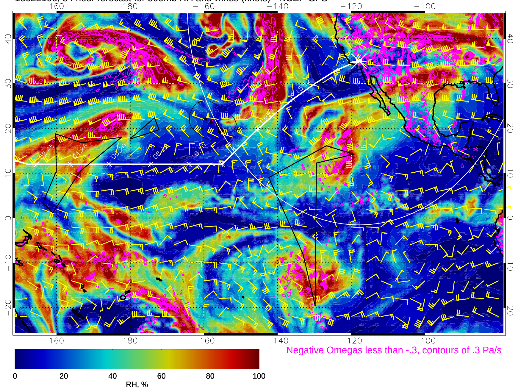
15022106, 54 hour forecast for 500mb RH and winds (knots) - NCEP GFS
