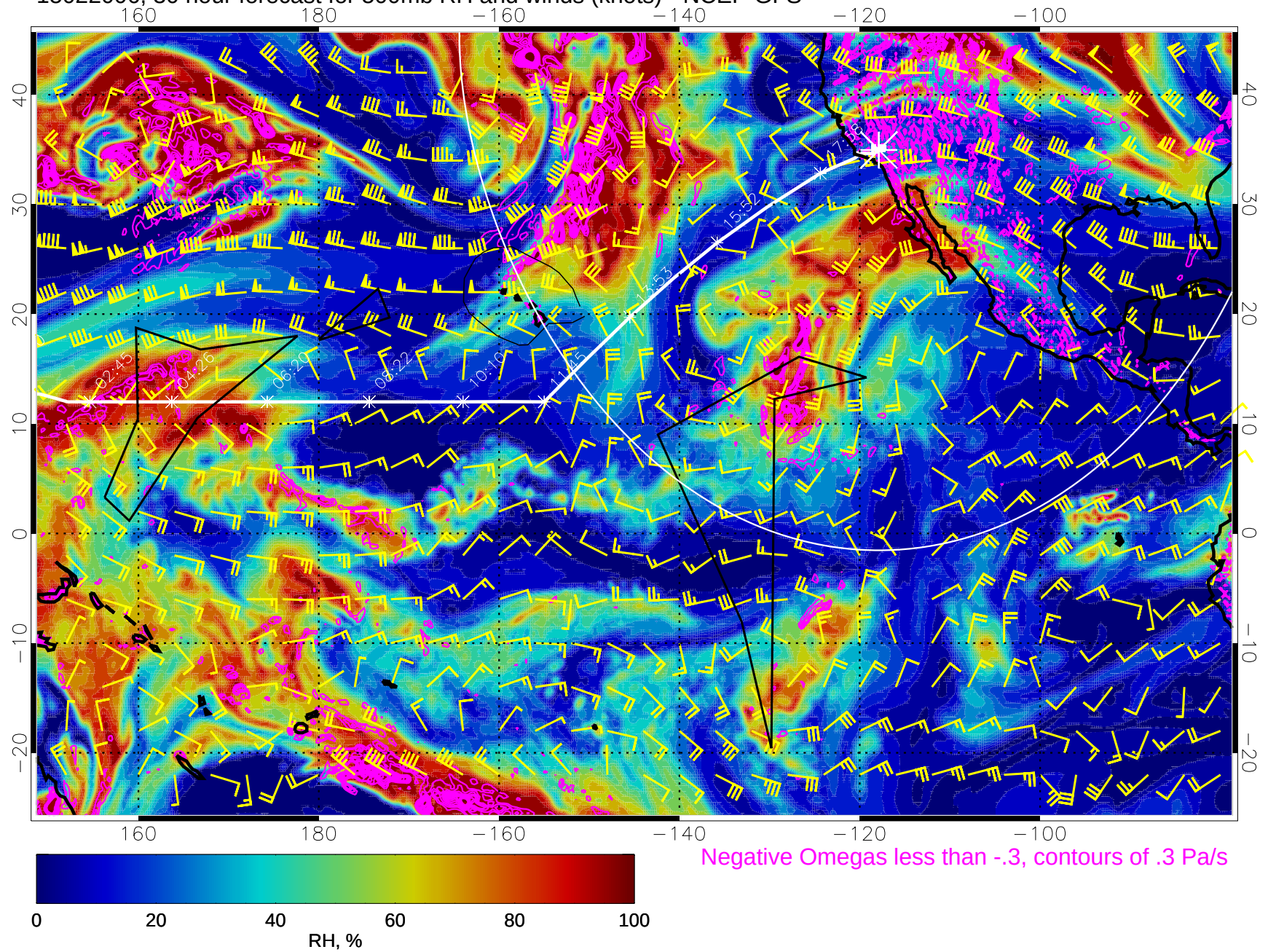
15022006, 30 hour forecast for 500mb RH and winds (knots) - NCEP GFS
