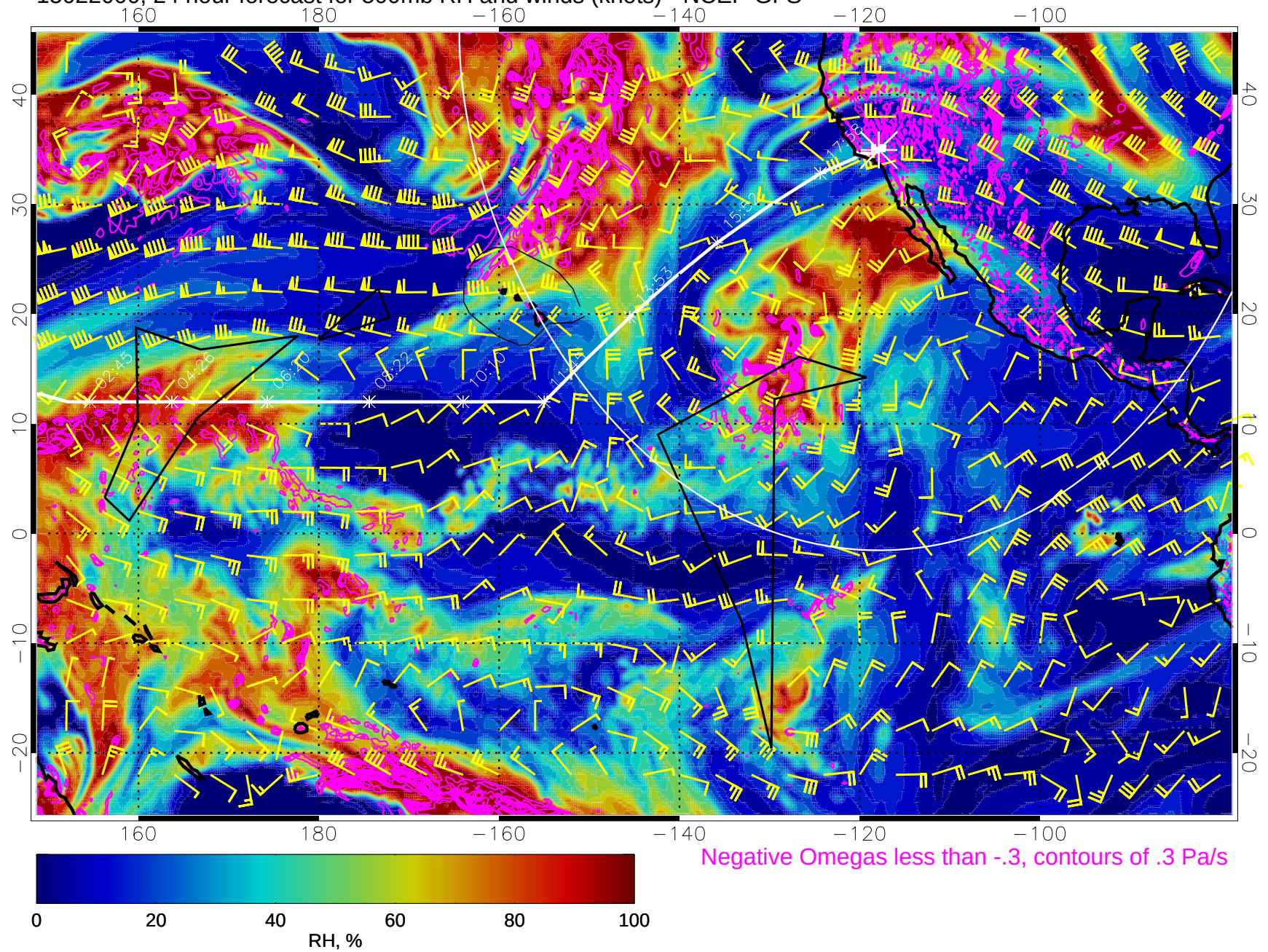
15022000, 24 hour forecast for 500mb RH and winds (knots) - NCEP GFS
