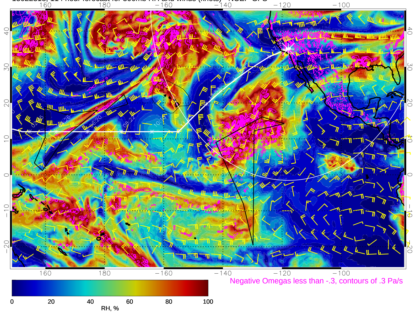
15022318, 114 hour forecast for 500mb RH and winds (knots) - NCEP GFS
