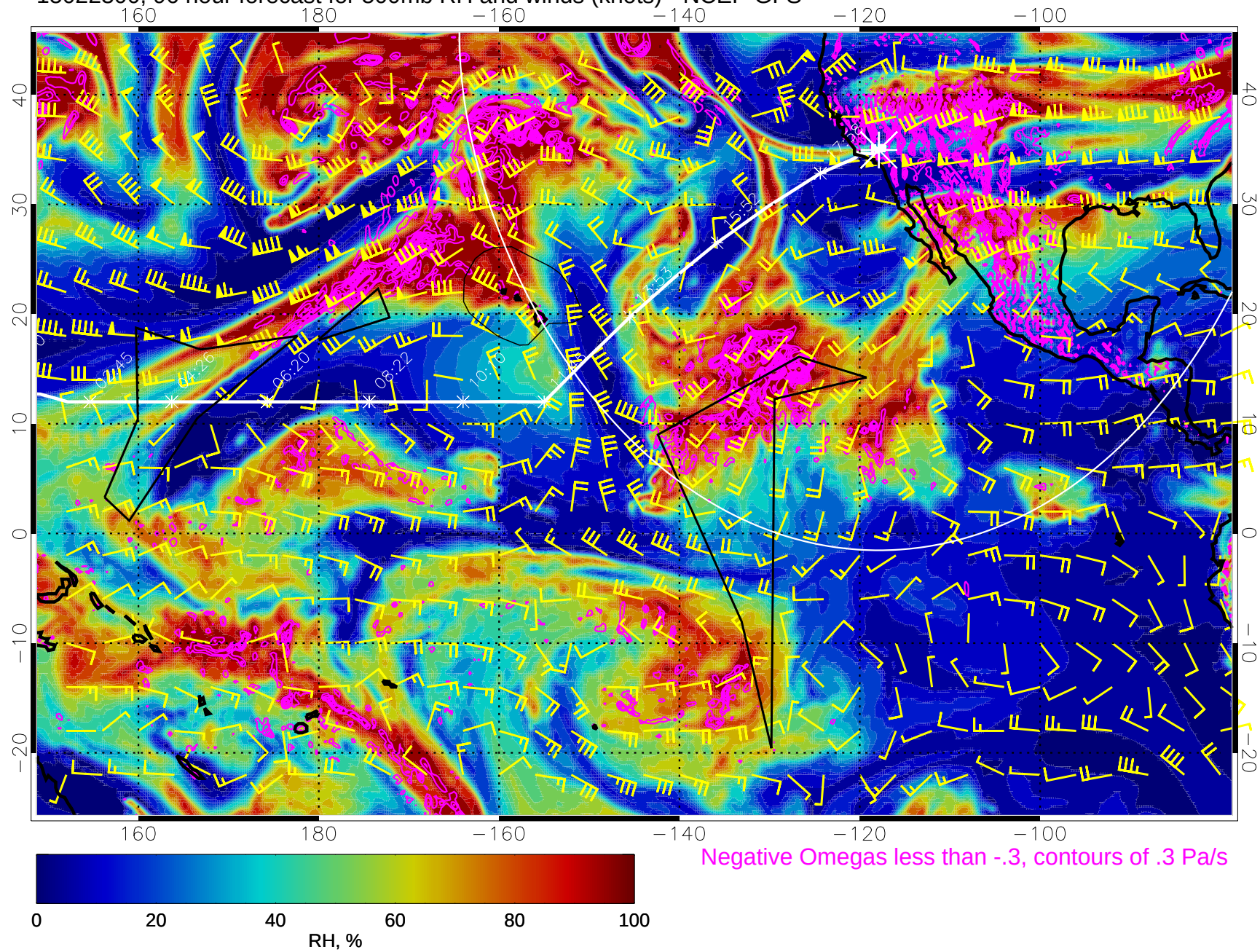
15022300, 96 hour forecast for 500mb RH and winds (knots) - NCEP GFS
