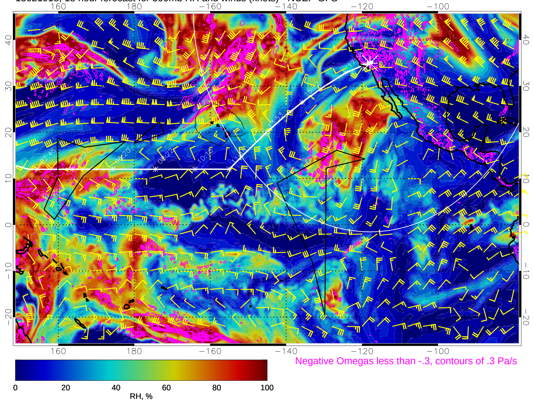
15021918, 18 hour forecast for 500mb RH and winds (knots) - NCEP GFS
