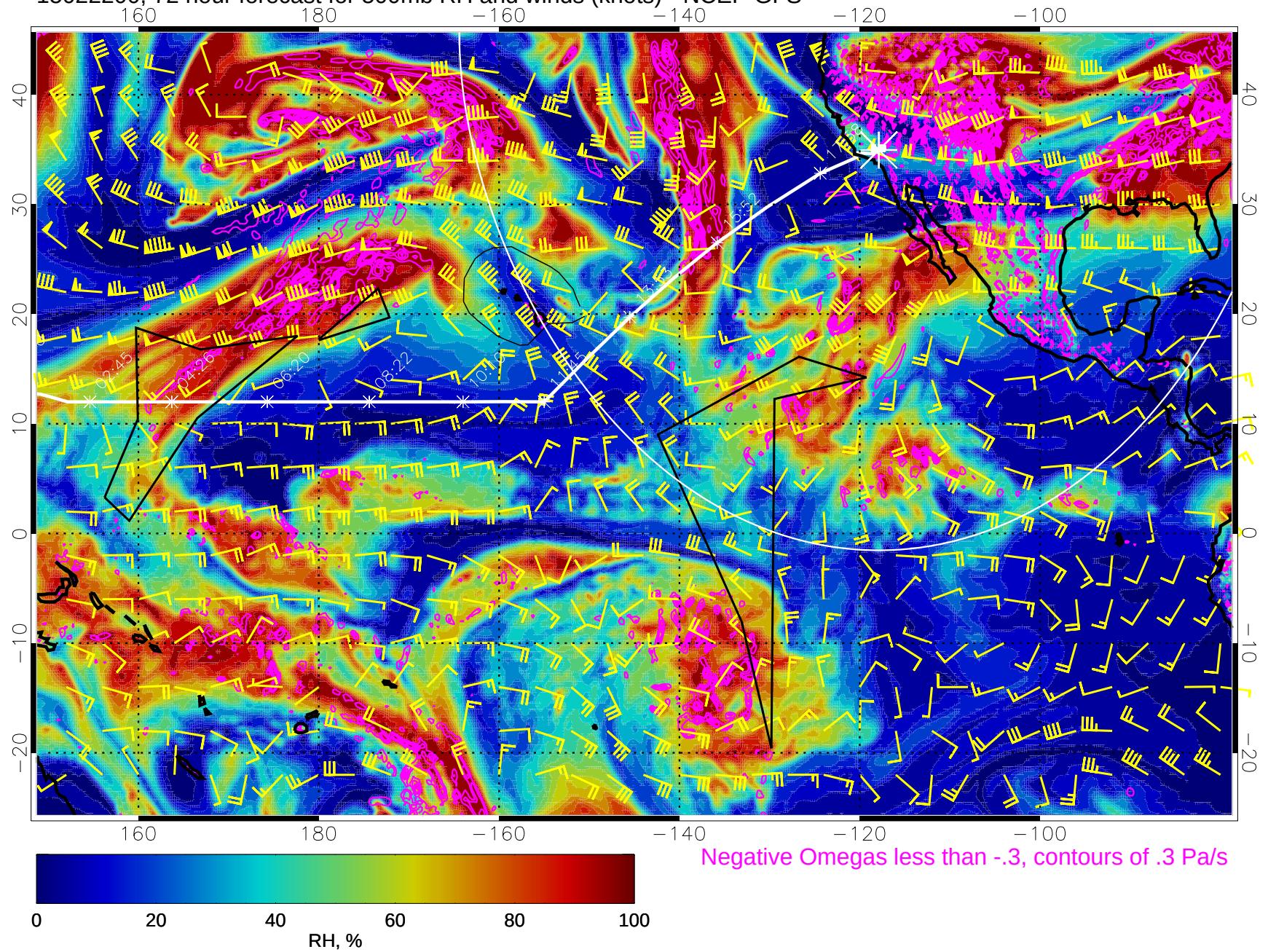
15022200, 72 hour forecast for 500mb RH and winds (knots) - NCEP GFS
