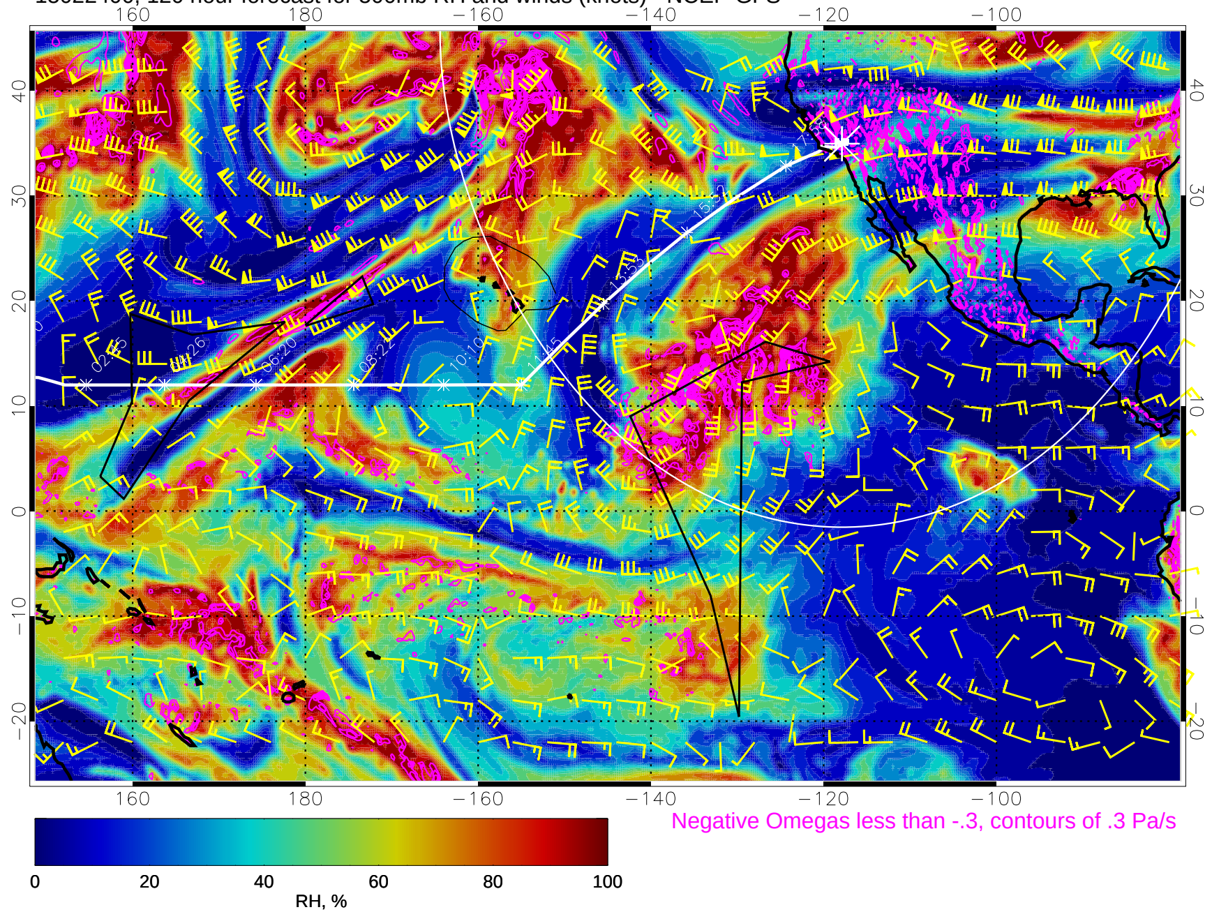
15022400, 120 hour forecast for 500mb RH and winds (knots) - NCEP GFS
