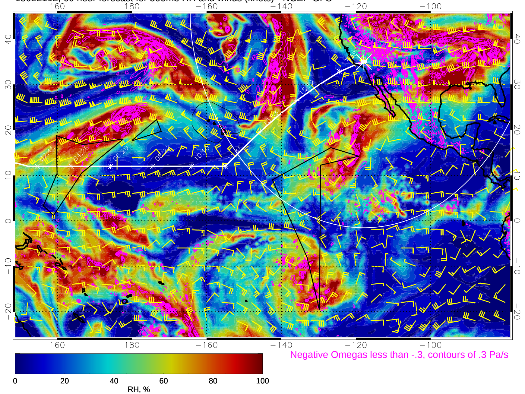
15022112, 60 hour forecast for 500mb RH and winds (knots) - NCEP GFS
