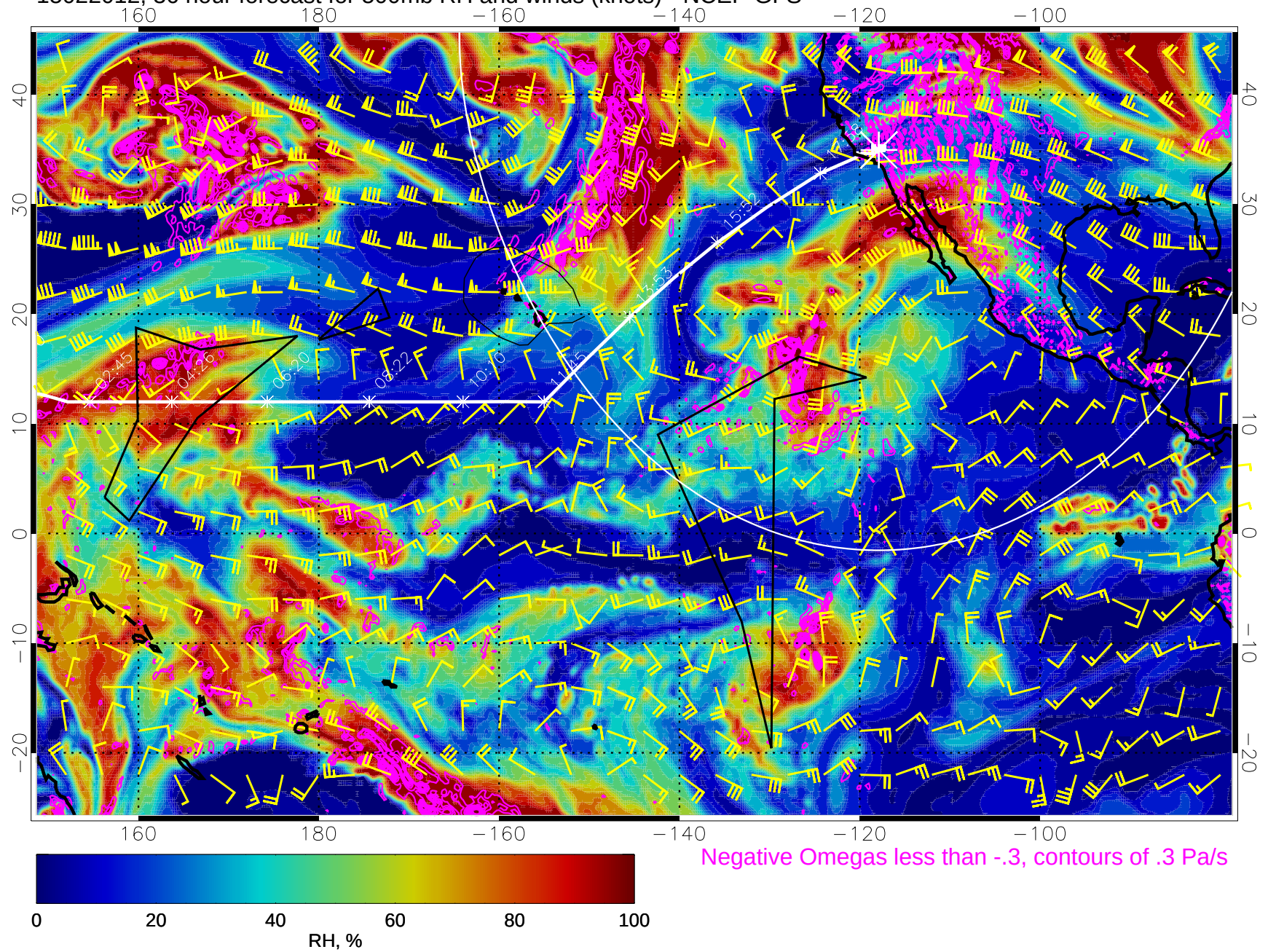
15022012, 36 hour forecast for 500mb RH and winds (knots) - NCEP GFS
